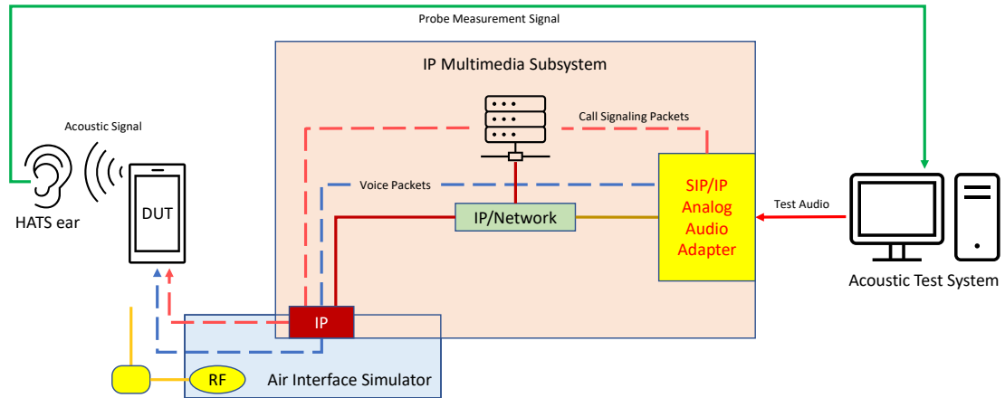
Figure 5-1 Test Setup for VoLTE over IMS Volume Control Measurements
