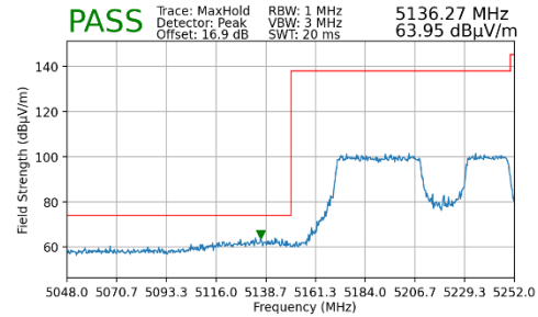
Plot 7-168. Radiated Lower Band Edge Plot MIMO (Peak – UNII Band 1)
