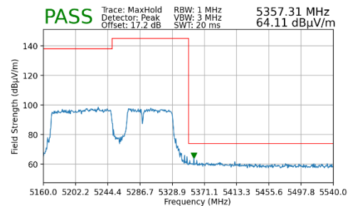
Plot 7-189. Radiated Upper Band Edge Plot MIMO (Peak – UNII Band 2A)
