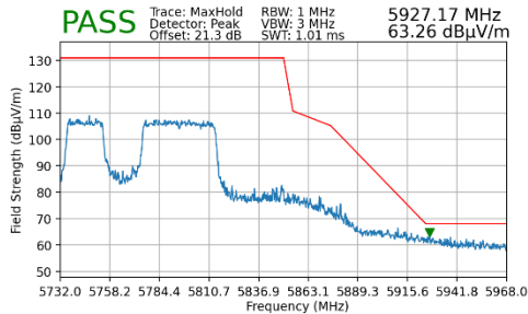
Plot 7-173. Radiated Upper Band Edge Plot MIMO (Peak – UNII Band 3)
