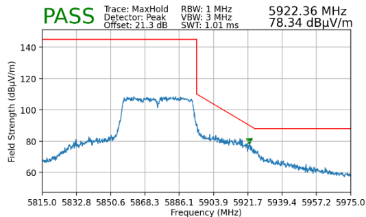
Plot 7-156. Radiated Upper Band Edge Plot MIMO (Peak – UNII Band 4)
