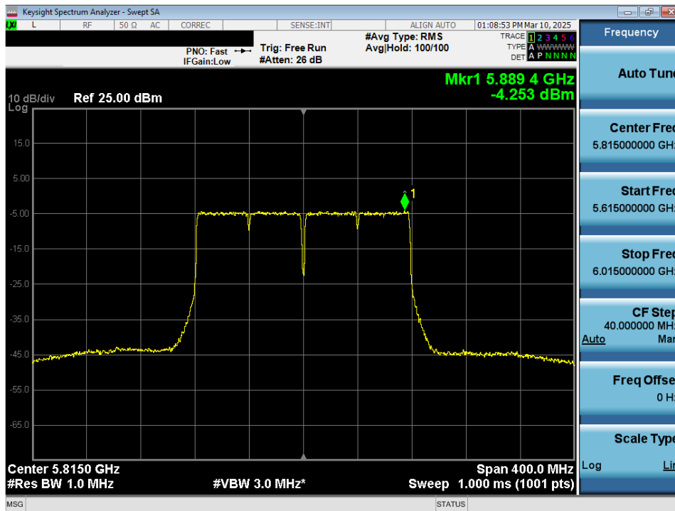
Plot 7-121. Power Spectral Density Plot MIMO ANT2 (160MHz 802.11ac (UNII Band 3/4) – Ch. 163)
