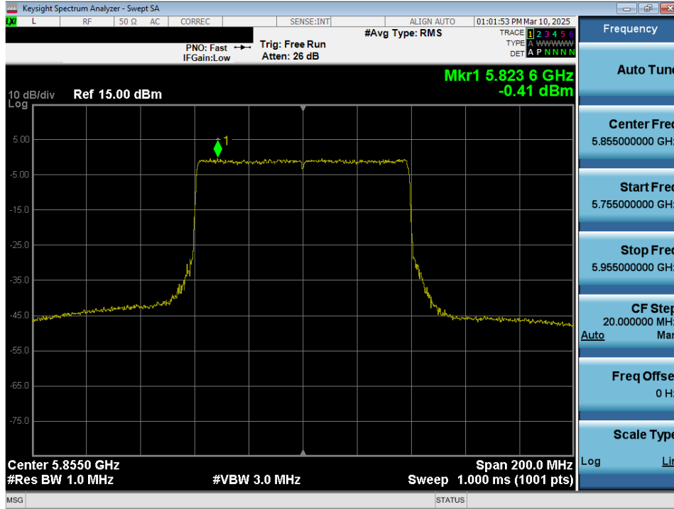
Plot 7-120. Power Spectral Density Plot MIMO ANT2 (80MHz 802.11ax/be (UNII Band 3/4) – Ch. 171)
