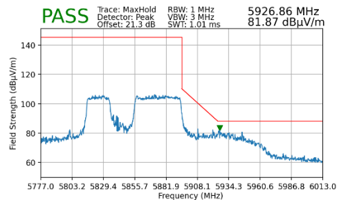
Plot 7-176. Radiated Upper Band Edge Plot MIMO (Peak – UNII Band 4)
