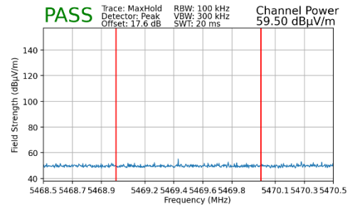
Plot 7-172. Radiated Lower Band Edge Plot MIMO (Peak – UNII Band 2C)
