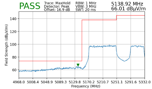
Plot 7-187. Radiated Lower Band Edge Plot MIMO (Peak – UNII Band 1)
