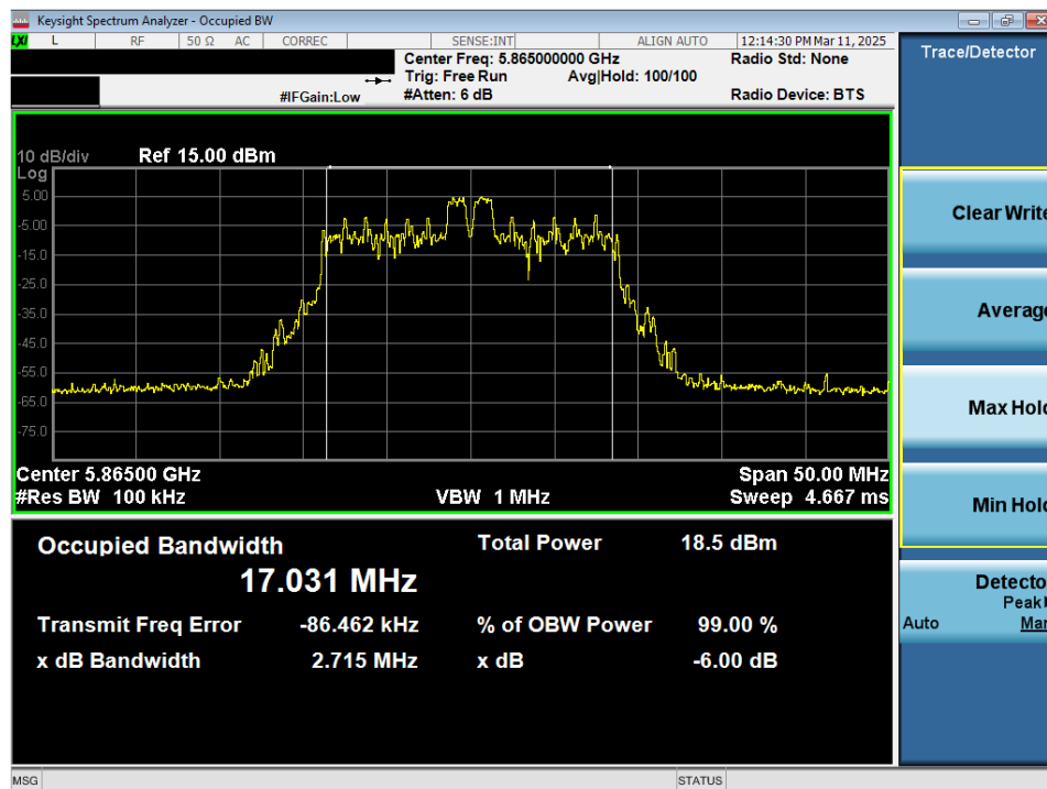
Plot 7-47. 6dB Bandwidth Plot MIMO ANT2 (20MHz 802.11ax/be (26 Tones) (UNII Band 4) – Ch. 173)
