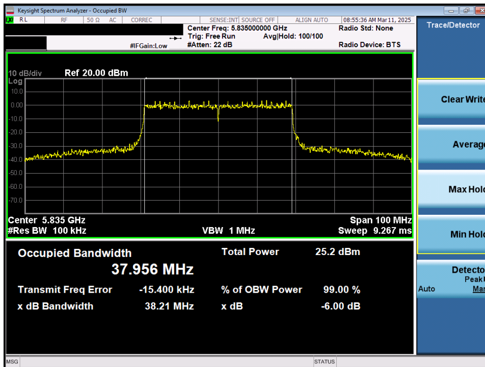
Plot 7-39. 6dB Bandwidth Plot MIMO ANT1 (40MHz 802.11ax/be (Full Tones) (UNII Band 3/4) – Ch. 167)
