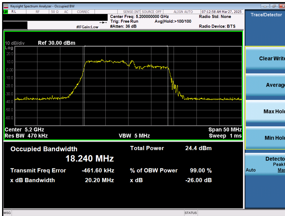
Plot 7-5. 26dB Bandwidth Plot MIMO ANT1 (20MHz 802.11be (106+26 Tones) (UNII Band 1) – Ch. 40)
