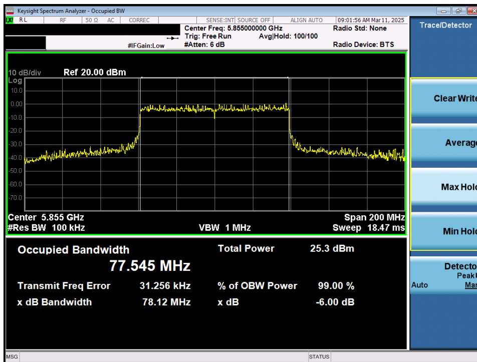
Plot 7-40. 6dB Bandwidth Plot MIMO ANT1 (80MHz 802.11ax/be (Full Tones) (UNII Band 3/4) – Ch. 171)
