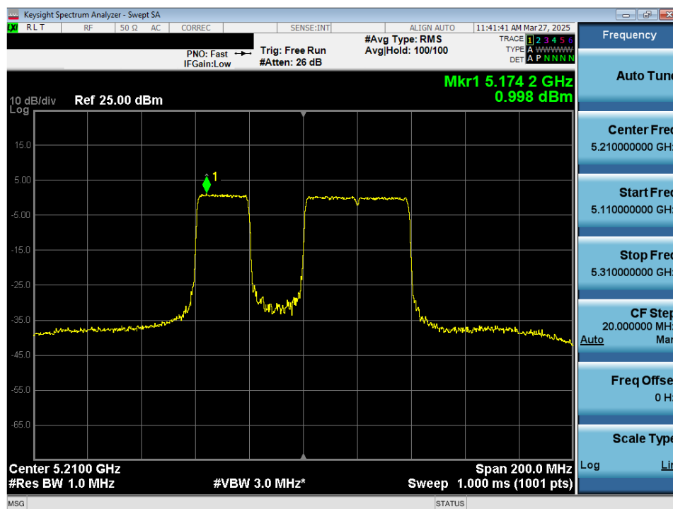
Plot 7-96. Power Spectral Density Plot MIMO ANT2 (80MHz 802.11be (484+242 Tones) (UNII Band 1) – Ch. 42)
