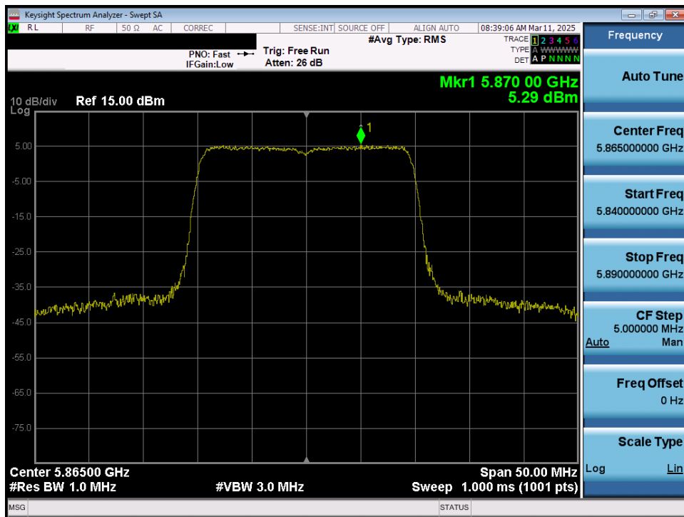
Plot 7-87. Power Spectral Density Plot MIMO ANT1 (20MHz 802.11ax/be (Full Tones) (UNII Band 4) – Ch. 173)
