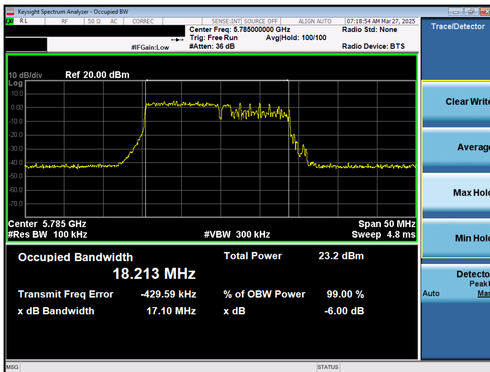
Plot 7-26. 6dB Bandwidth Plot MIMO ANT1 (20MHz 802.11be (106+26 Tones) (UNII Band 3) – Ch. 157)
