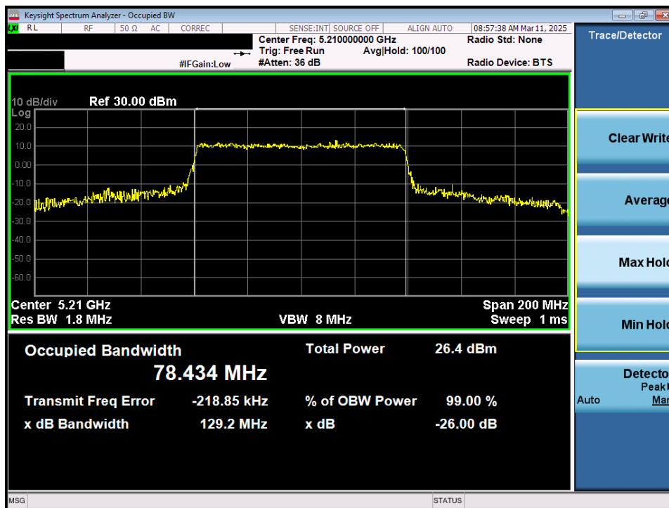
Plot 7-10. 26dB Bandwidth Plot MIMO ANT1 (80MHz 802.11ax/be (Full Tones) (UNII Band 1) – Ch. 42)
