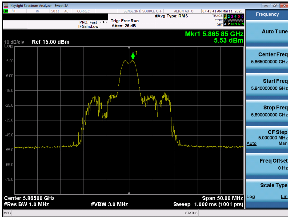
Plot 7-77. Power Spectral Density Plot MIMO ANT1 (20MHz 802.11ax/be (26 Tones) (UNII Band 4) – Ch. 173)
