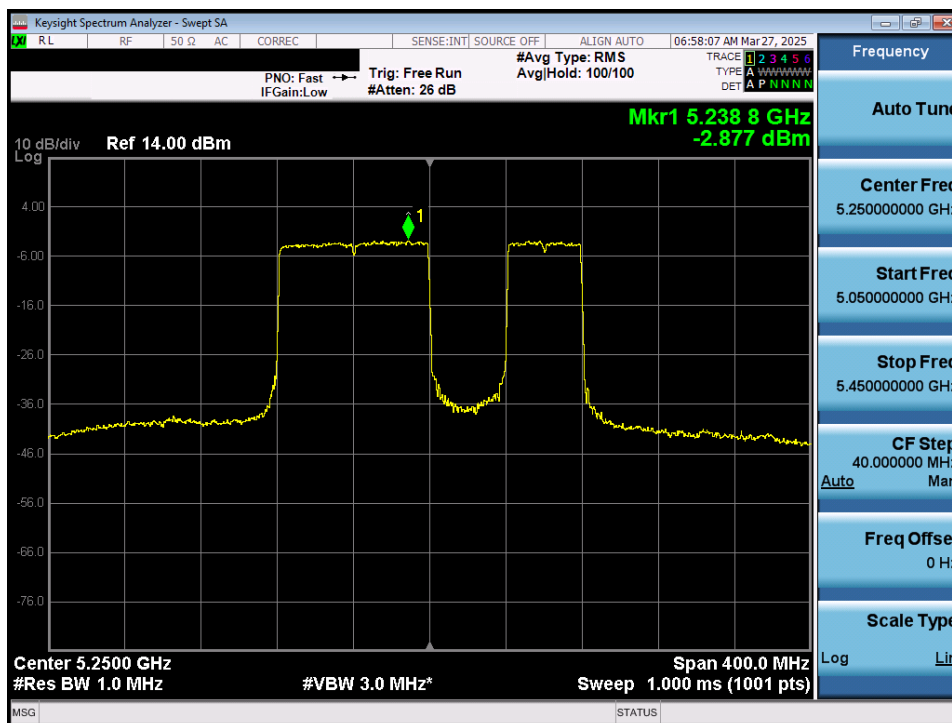
Plot 7-67. Power Spectral Density Plot MIMO ANT1 (160MHz 802.11be (996+484 Tones) (UNII Band 1/2A) – Ch. 50)
