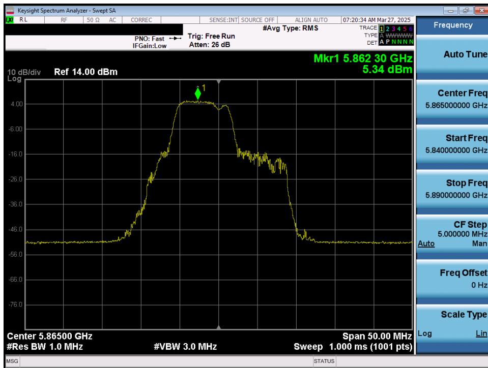
Plot 7-81. Power Spectral Density Plot MIMO ANT1 (20MHz 802.11be (52+26 Tones) (UNII Band 4) – Ch. 173)
