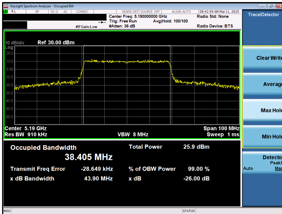
Plot 7-9. 26dB Bandwidth Plot MIMO ANT1 (40MHz 802.11ax/be (Full Tones) (UNII Band 1) – Ch. 38)
