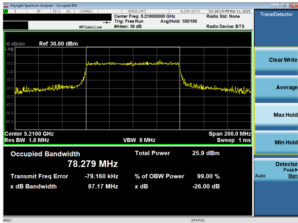
Plot 7-21. 26dB Bandwidth Plot MIMO ANT2 (80MHz 802.11ax/be (Full Tones) (UNII Band 1) – Ch. 42)
