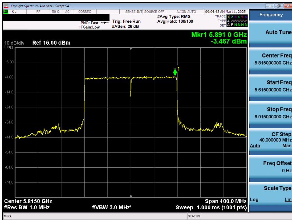
Plot 7-90. Power Spectral Density Plot MIMO ANT1 (160MHz 802.11ax/be (Full Tones) (UNII Band 3/4) – Ch. 163)
