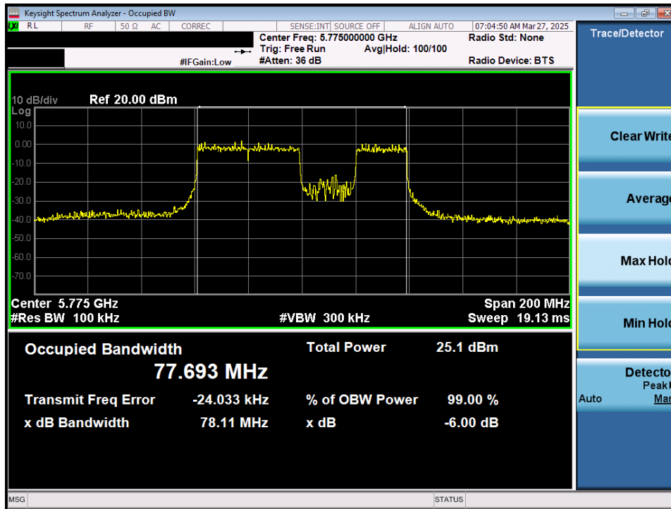
Plot 7-27. 6dB Bandwidth Plot MIMO ANT1 (80MHz 802.11be (484+242 Tones) (UNII Band 3) – Ch. 155)
