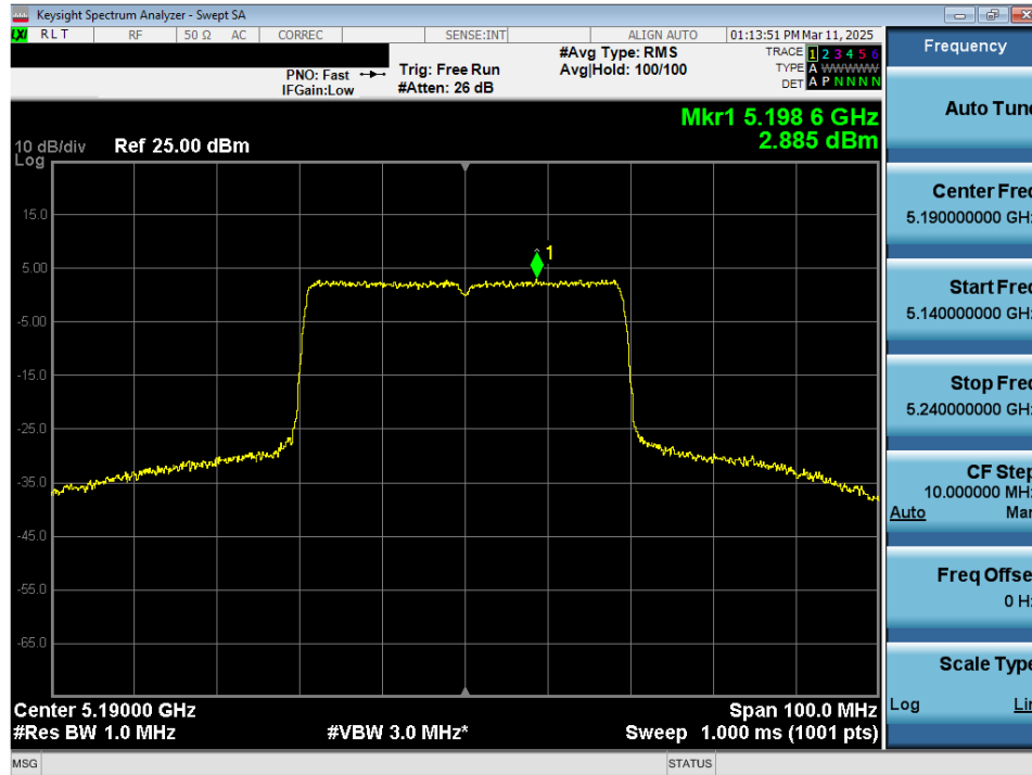
Plot 7-99. Power Spectral Density Plot MIMO ANT2 (40MHz 802.11ax/be (Full Tones) (UNII Band 1) – Ch. 38)
