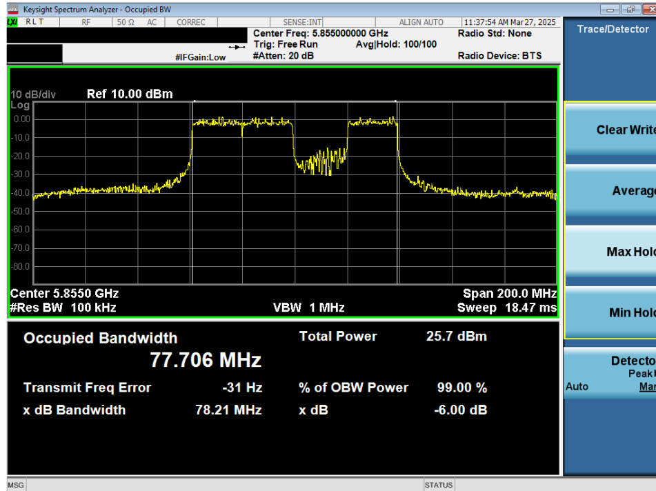
Plot 7-52. 6dB Bandwidth Plot MIMO ANT2 (80MHz 802.11be (484+242 Tones) (UNII Band 3/4) – Ch. 171)
