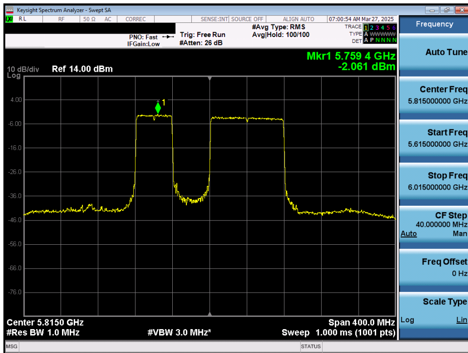
Plot 7-83. Power Spectral Density Plot MIMO ANT1 (160MHz 802.11be (996+484 Tones) (UNII Band 3/4) – Ch. 163)
