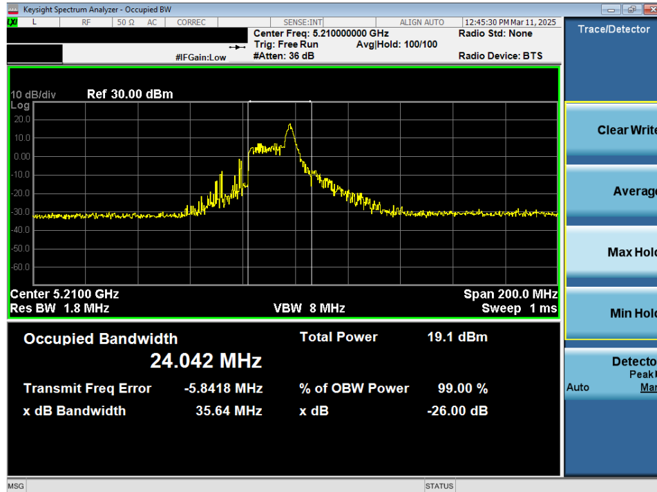
Plot 7-14. 26dB Bandwidth Plot MIMO ANT2 (80MHz 802.11ax/be (26 Tones) (UNII Band 1) – Ch. 42)
