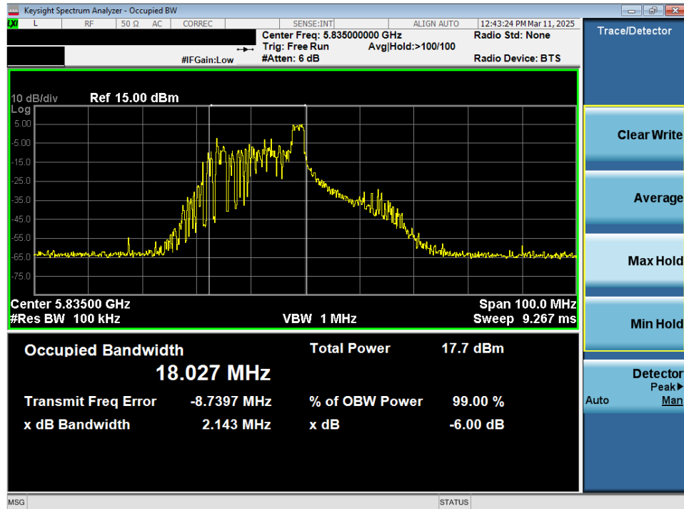
Plot 7-48. 6dB Bandwidth Plot MIMO ANT2 (40MHz 802.11ax/be (26 Tones) (UNII Band 3/4) – Ch. 167)
