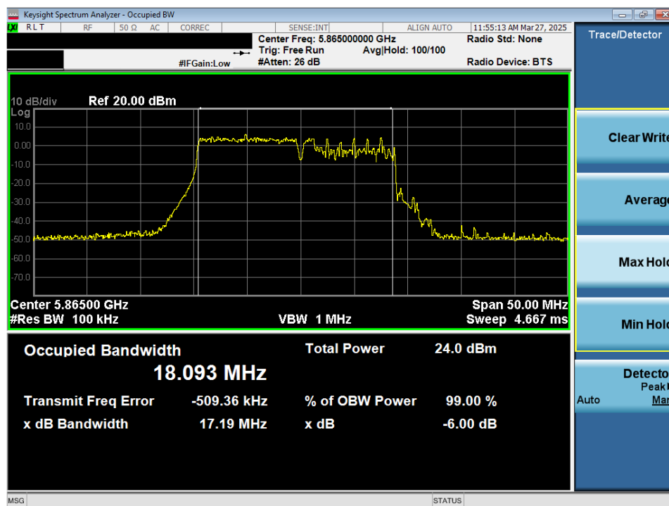
Plot 7-51. 6dB Bandwidth Plot MIMO ANT2 (20MHz 802.11be (106+26 Tones) (UNII Band 4) – Ch. 173)
