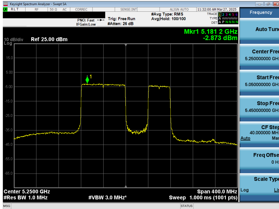
Plot 7-97. Power Spectral Density Plot MIMO ANT2 (160MHz 802.11be (996+484 Tones) (UNII Band 1/2A) – Ch. 50)
