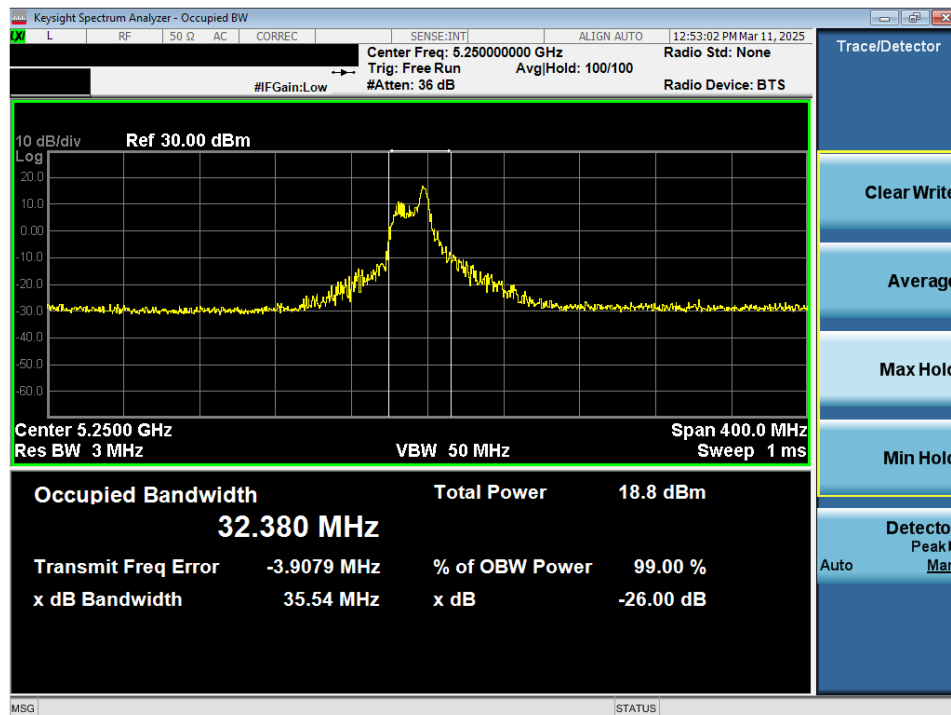
Plot 7-15. 26dB Bandwidth Plot MIMO ANT2 (160MHz 802.11ax/be (26 Tones) (UNII Band 1/2A) – Ch. 50)
