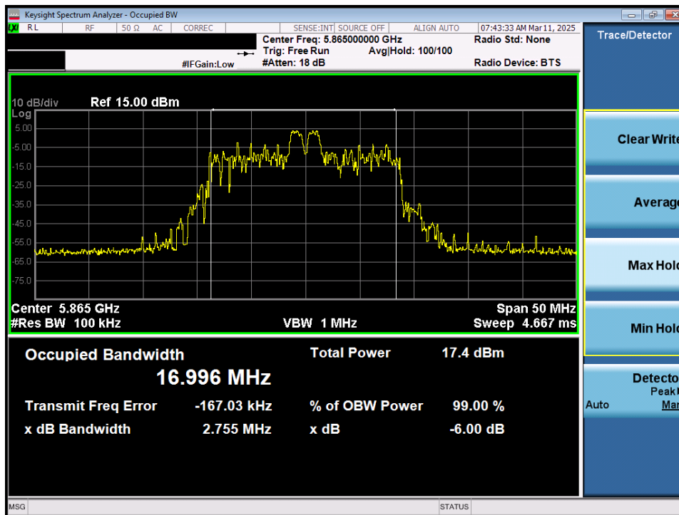
Plot 7-28. 6dB Bandwidth Plot MIMO ANT1 (20MHz 802.11ax/be (26 Tones) (UNII Band 4) – Ch. 173)
