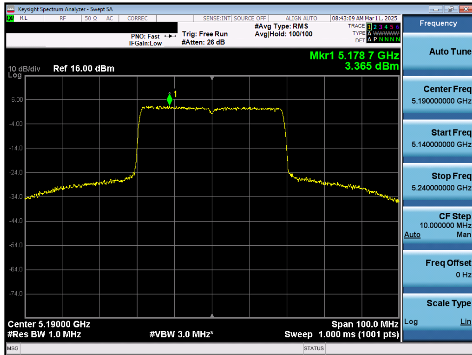
Plot 7-69. Power Spectral Density Plot MIMO ANT1 (40MHz 802.11ax/be (Full Tones) (UNII Band 1) – Ch. 38)
