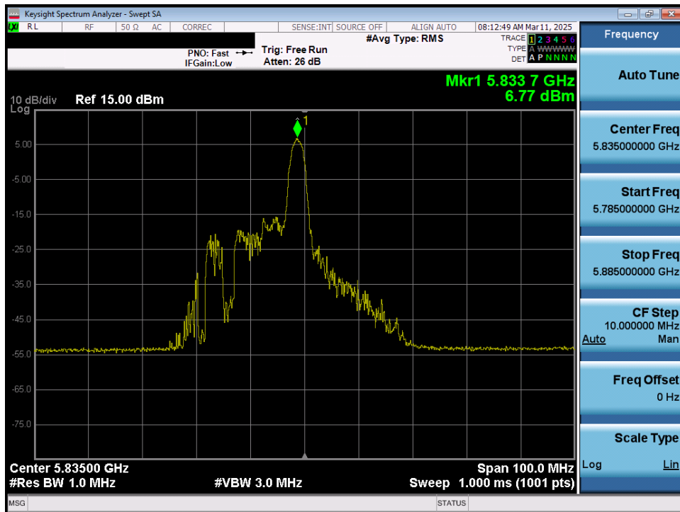
Plot 7-78. Power Spectral Density Plot MIMO ANT1 (40MHz 802.11ax/be (26 Tones) (UNII Band 3/4) – Ch. 167)
