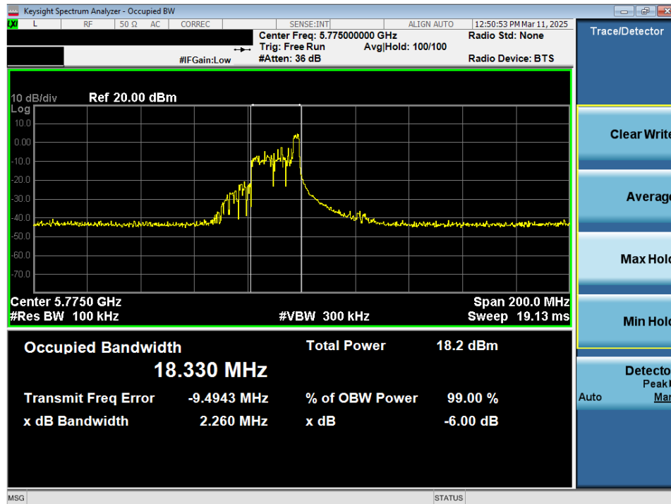
Plot 7-44. 6dB Bandwidth Plot MIMO ANT2 (80MHz 802.11ax/be (26 Tones) (UNII Band 3) – Ch. 155)
