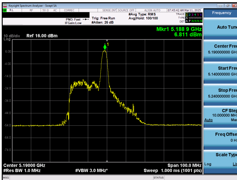
Plot 7-62. Power Spectral Density Plot MIMO ANT1 (40MHz 802.11ax/be (26 Tones) (UNII Band 1) – Ch. 38)
