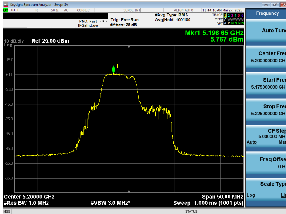
Plot 7-95. Power Spectral Density Plot MIMO ANT2 (20MHz 802.11be (52+26 Tones) (UNII Band 1) – Ch. 40)
