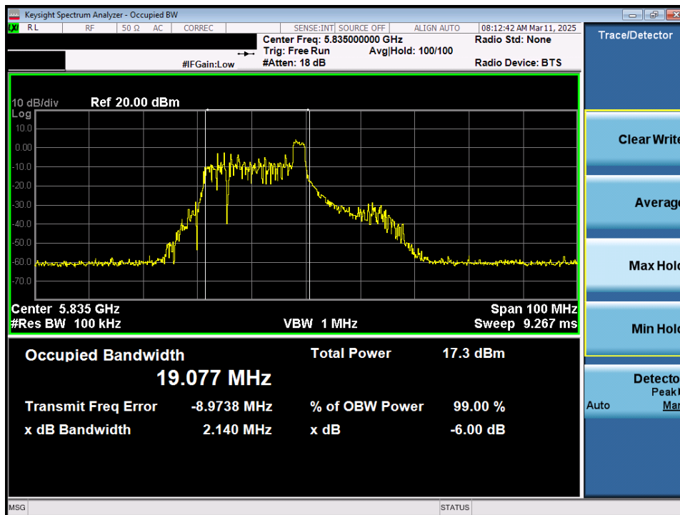
Plot 7-29. 6dB Bandwidth Plot MIMO ANT1 (40MHz 802.11ax/be (26 Tones) (UNII Band 3/4) – Ch. 167)
