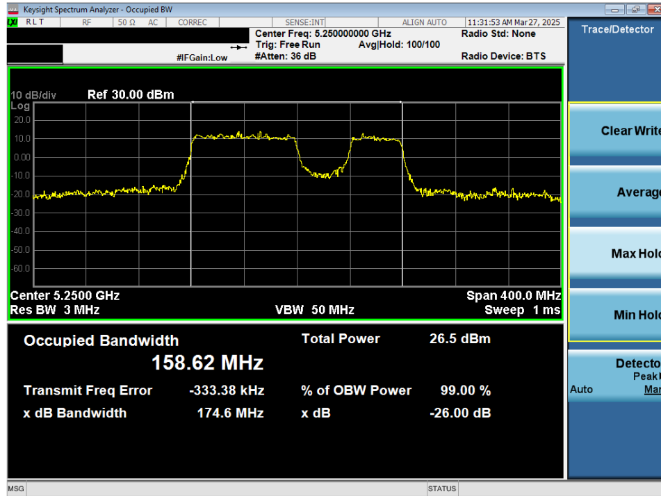
Plot 7-18. 26dB Bandwidth Plot MIMO ANT2 (160MHz 802.11be (996+484 Tones) (UNII Band 1/2A) – Ch. 50)
