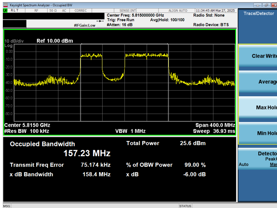
Plot 7-53. 6dB Bandwidth Plot MIMO ANT2 (160MHz 802.11be (996+484 Tones) (UNII Band 3/4) – Ch. 163)
