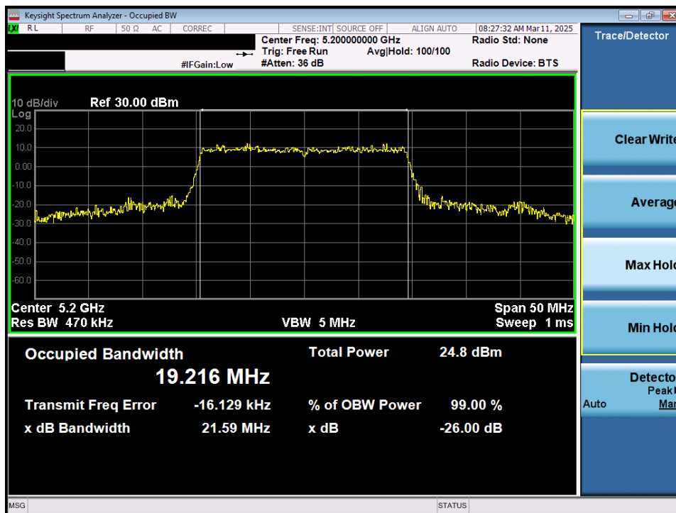
Plot 7-8. 26dB Bandwidth Plot MIMO ANT1 (20MHz 802.11ax/be (Full Tones) (UNII Band 1) – Ch. 40)
