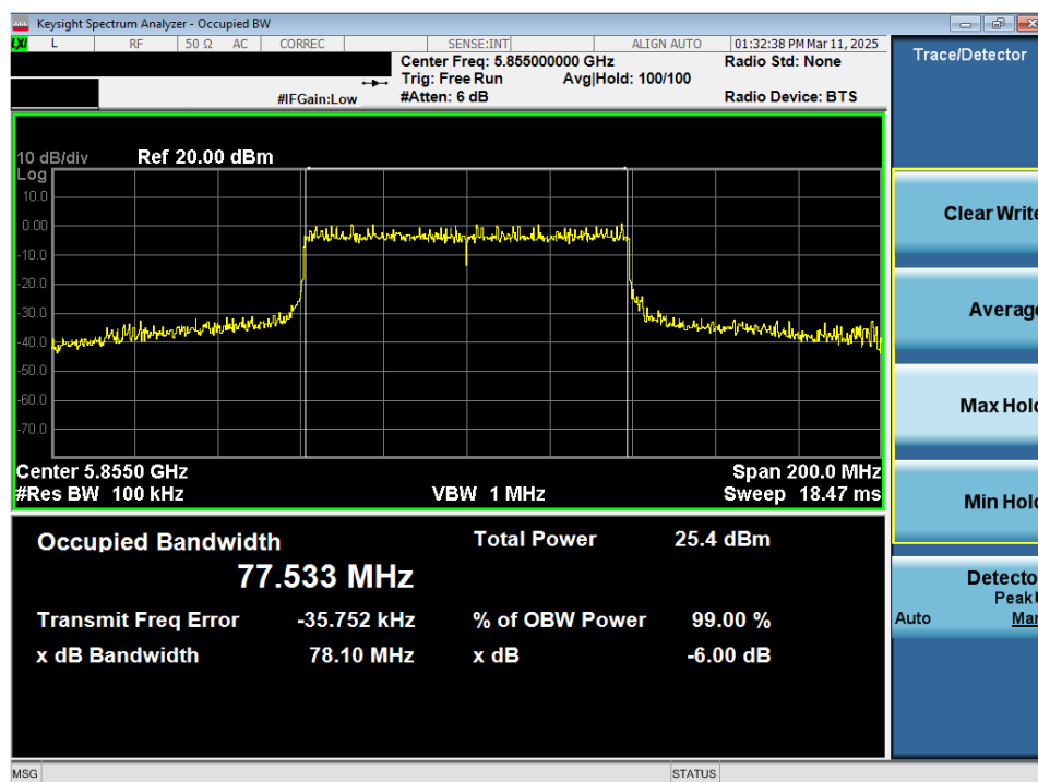
Plot 7-59. 6dB Bandwidth Plot MIMO ANT2 (80MHz 802.11ax/be (Full Tones) (UNII Band 3/4) – Ch. 171)
