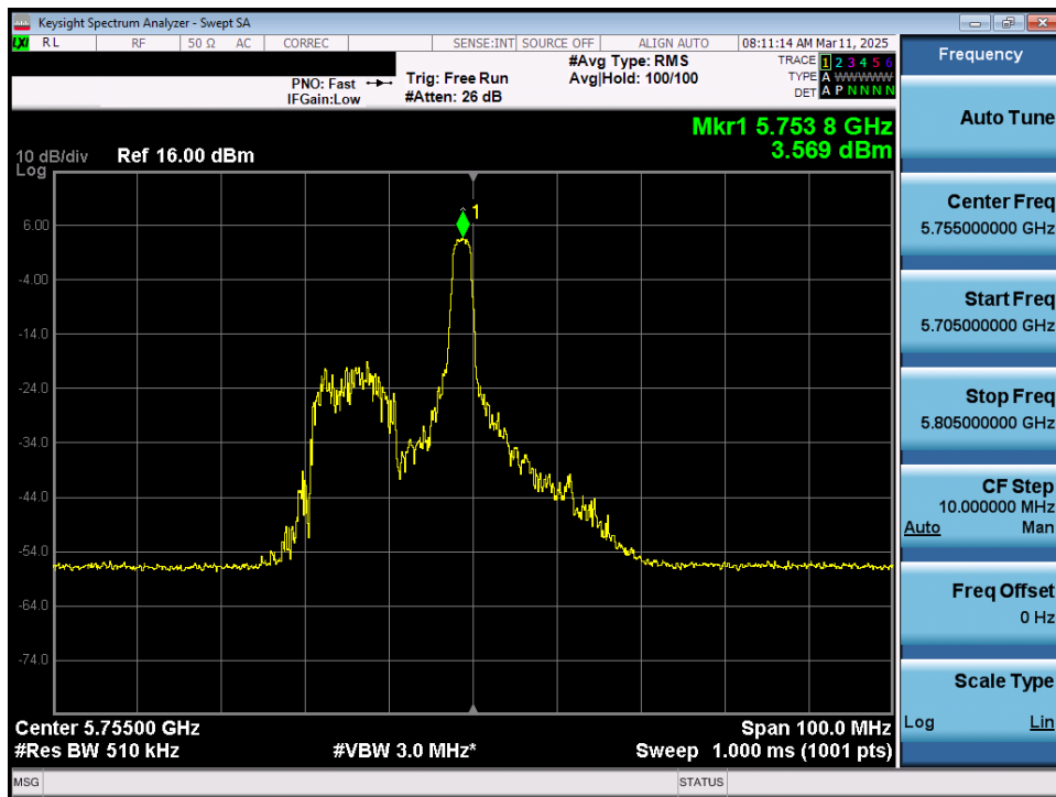
Plot 7-73. Power Spectral Density Plot MIMO ANT1 (40MHz 802.11ax/be (26 Tones) (UNII Band 3) – Ch. 151)
