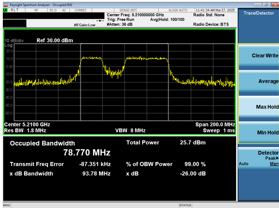
Plot 7-17. 26dB Bandwidth Plot MIMO ANT2 (80MHz 802.11be (484+242 Tones) (UNII Band 1) – Ch. 42)
