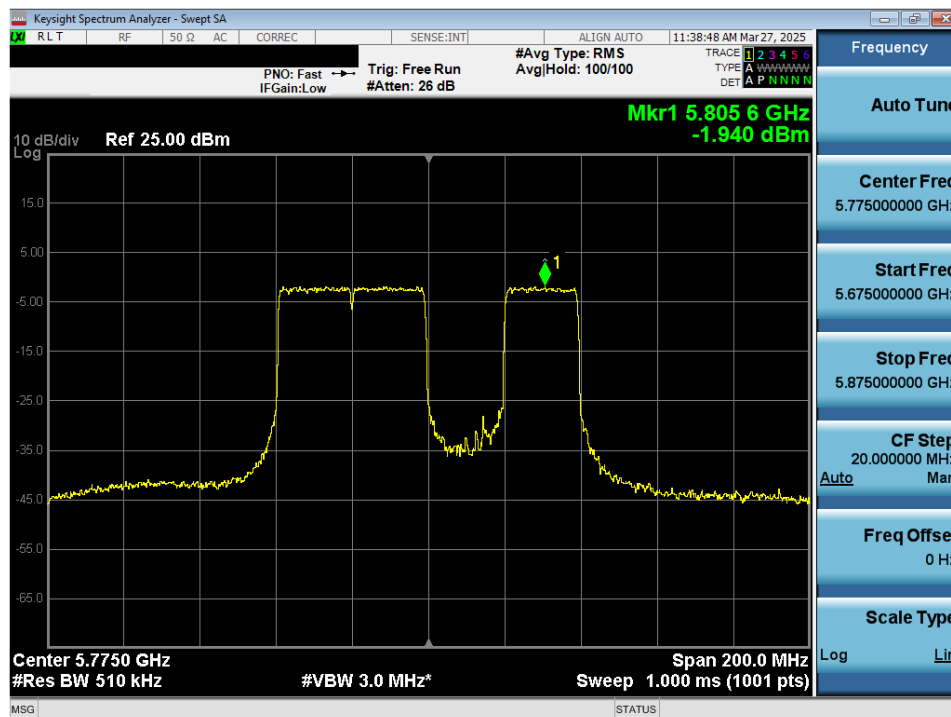
Plot 7-106. Power Spectral Density Plot MIMO ANT2 (80MHz 802.11be (484+242 Tones) (UNII Band 3) – Ch. 155)
