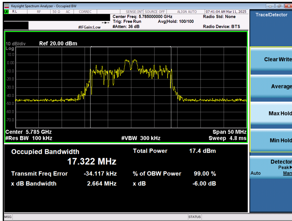
Plot 7-23. 6dB Bandwidth Plot MIMO ANT1 (20MHz 802.11ax/be (26 Tones) (UNII Band 3) – Ch. 157)
