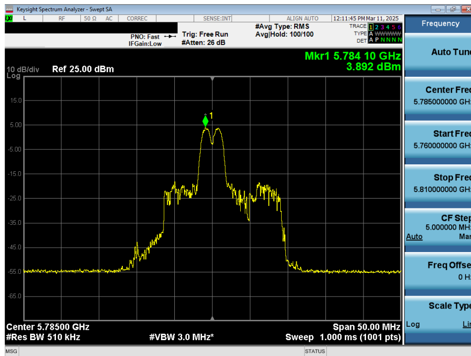
Plot 7-102. Power Spectral Density Plot MIMO ANT2 (20MHz 802.11ax/be (26 Tones) (UNII Band 3) – Ch. 157)
