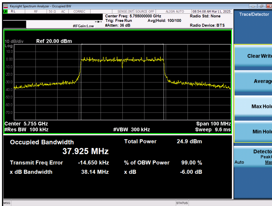
Plot 7-36. 6dB Bandwidth Plot MIMO ANT1 (40MHz 802.11ax/be (Full Tones) (UNII Band 3) – Ch. 151)
