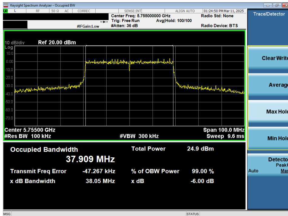
Plot 7-55. 6dB Bandwidth Plot MIMO ANT2 (40MHz 802.11ax/be (Full Tones) (UNII Band 3) – Ch. 151)
