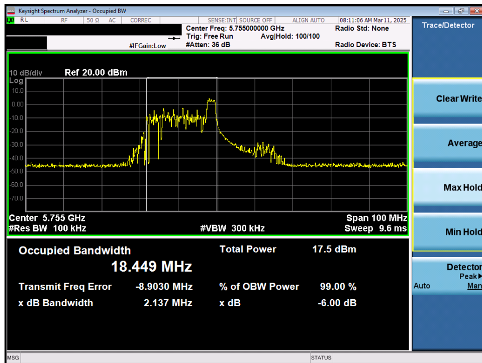
Plot 7-24. 6dB Bandwidth Plot MIMO ANT1 (40MHz 802.11ax/be (26 Tones) (UNII Band 3) – Ch. 151)
