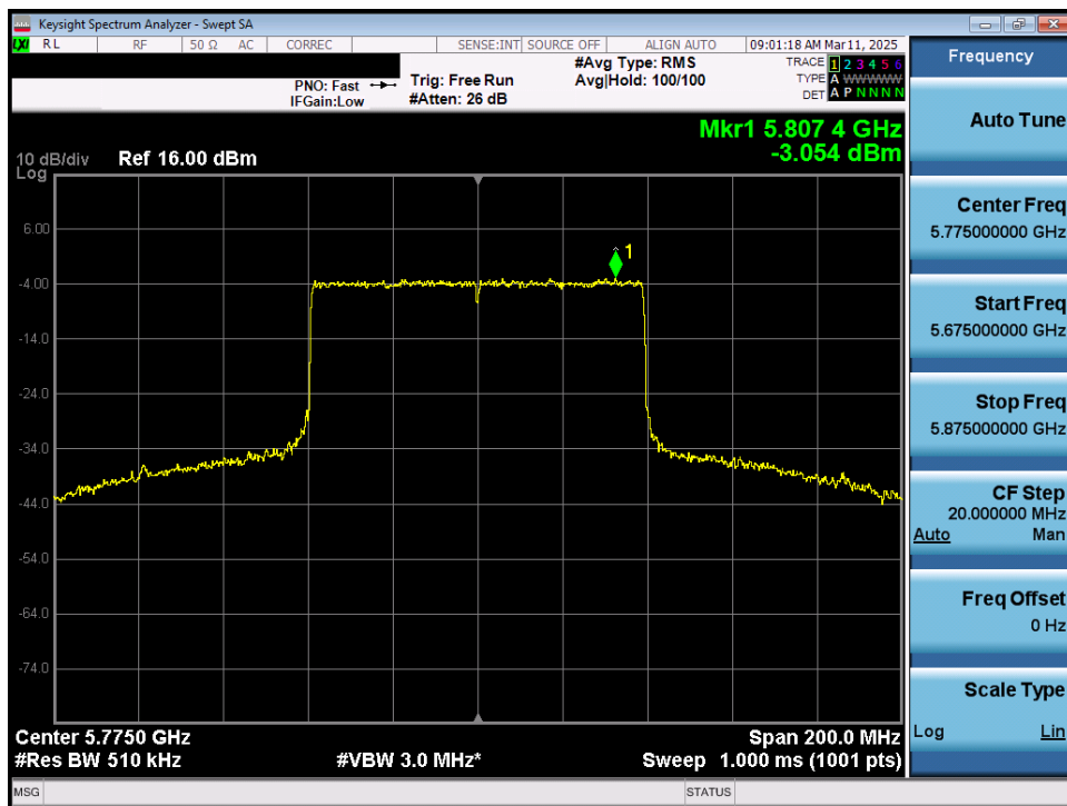
Plot 7-86. Power Spectral Density Plot MIMO ANT1 (80MHz 802.11ax/be (Full Tones) (UNII Band 3) – Ch. 155)
