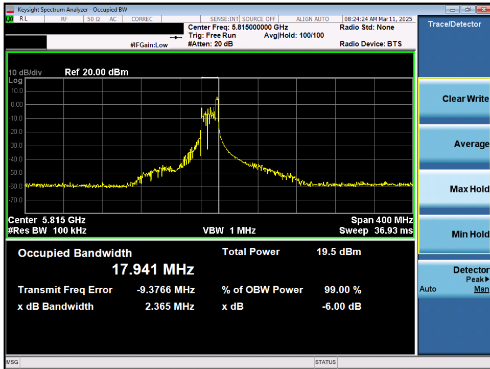
Plot 7-31. 6dB Bandwidth Plot MIMO ANT1 (160MHz 802.11ax/be (26 Tones) (UNII Band 3/4) – Ch. 163)
