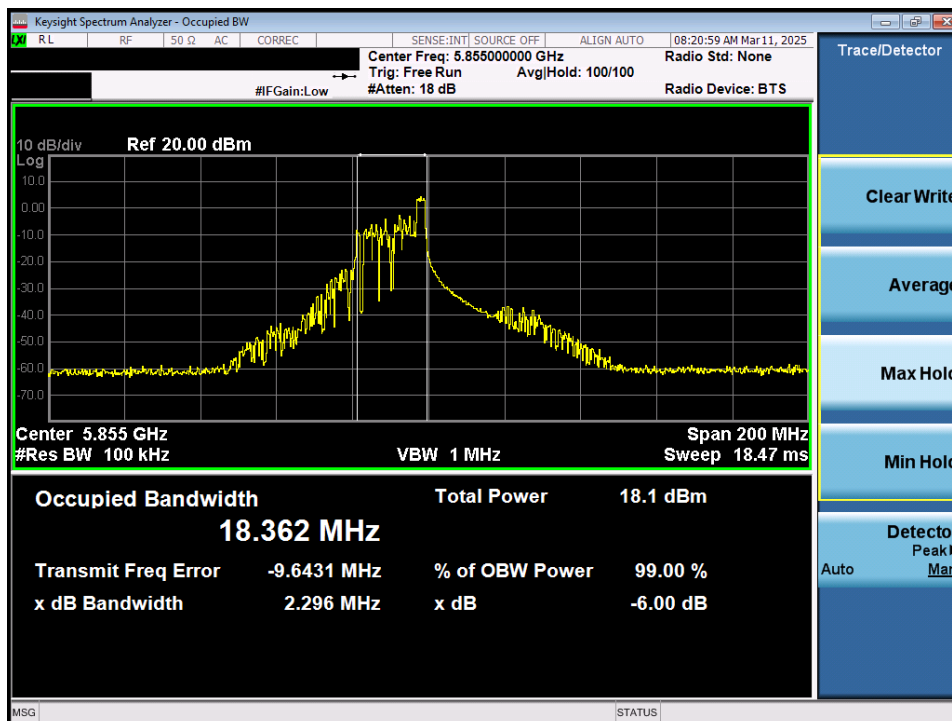
Plot 7-30. 6dB Bandwidth Plot MIMO ANT1 (80MHz 802.11ax/be (26 Tones) (UNII Band 3/4) – Ch. 171)
