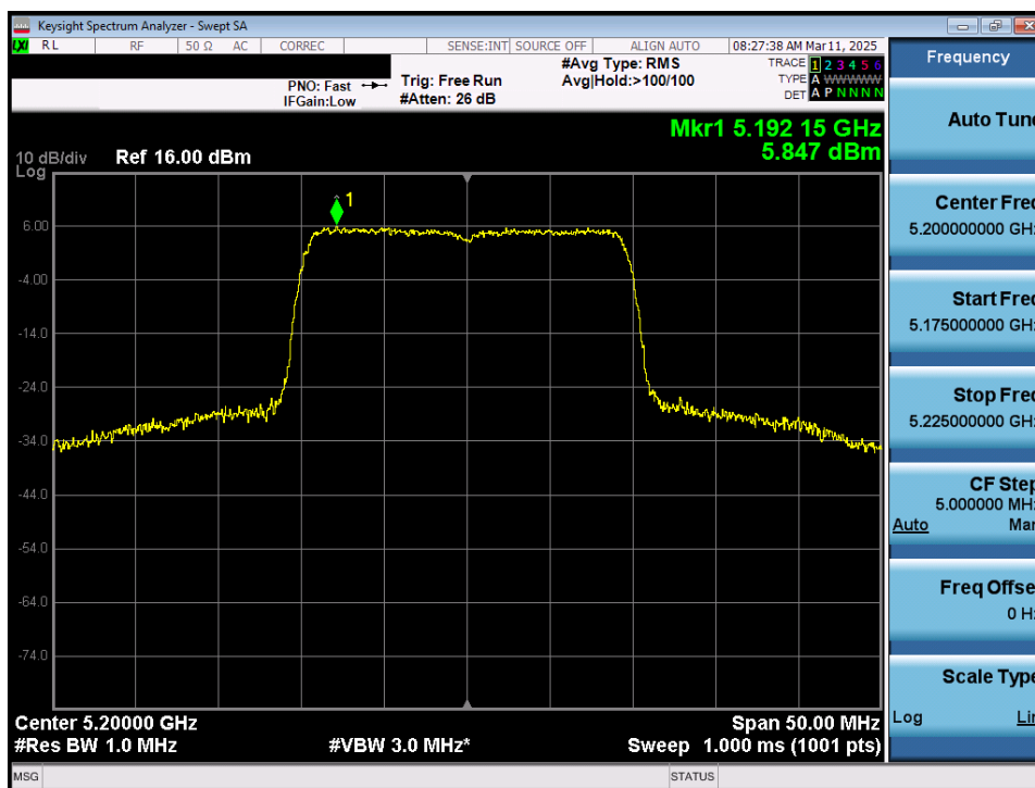
Plot 7-68. Power Spectral Density Plot MIMO ANT1 (20MHz 802.11ax/be (Full Tones) (UNII Band 1) – Ch. 40)
