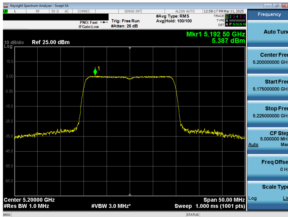
Plot 7-98. Power Spectral Density Plot MIMO ANT2 (20MHz 802.11ax/be (Full Tones) (UNII Band 1) – Ch. 40)
