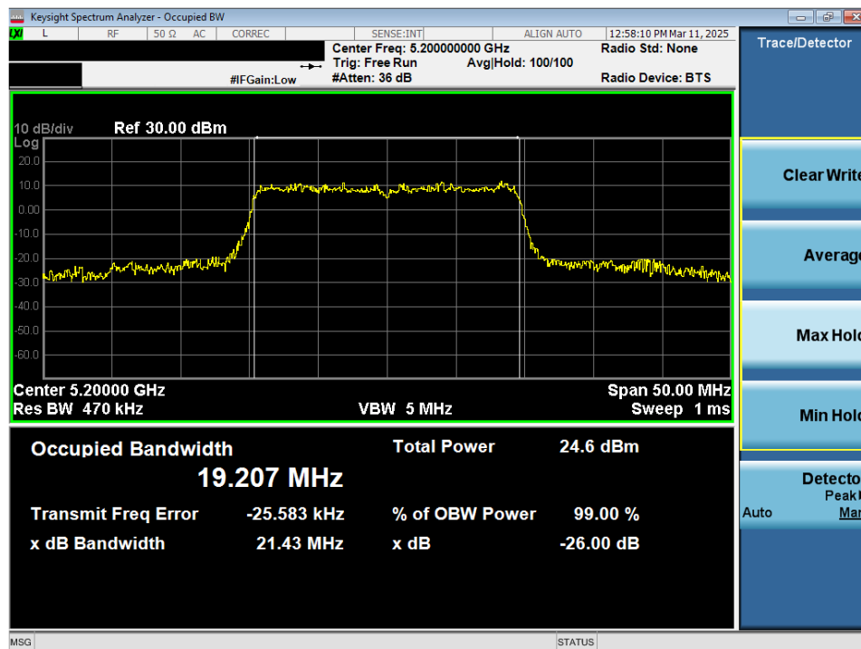
Plot 7-19. 26dB Bandwidth Plot MIMO ANT2 (20MHz 802.11ax/be (Full Tones) (UNII Band 1) – Ch. 40)
