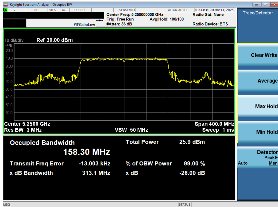
Plot 7-22. 26dB Bandwidth Plot MIMO ANT2 (160MHz 802.11ax/be (Full Tones) (UNII Band 1/2A) – Ch. 50)
