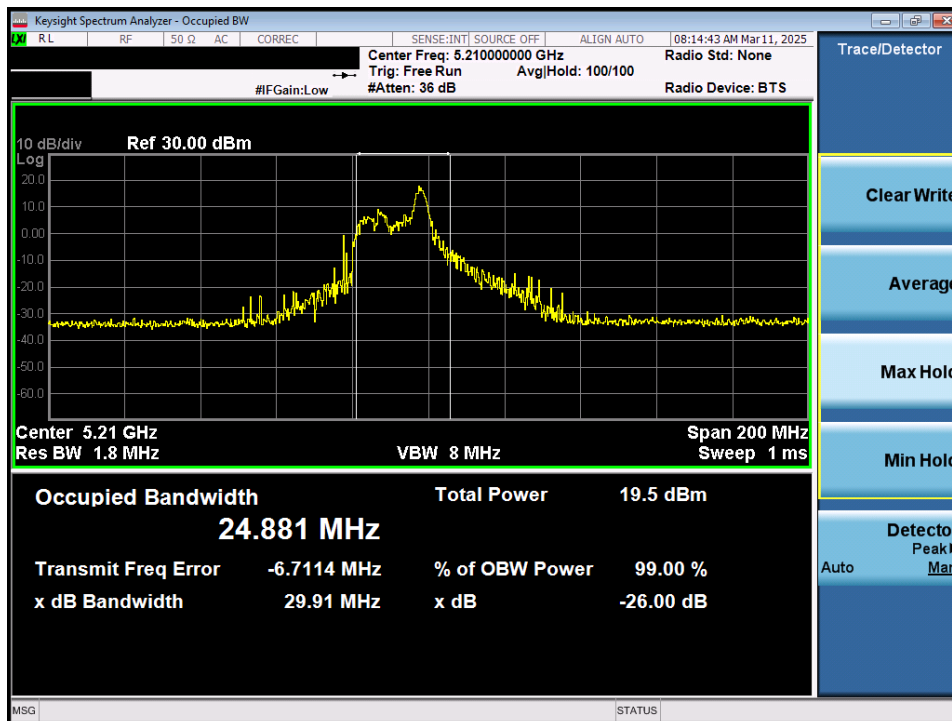
Plot 7-3. 26dB Bandwidth Plot MIMO ANT1 (80MHz 802.11ax/be (26 Tones) (UNII Band 1) – Ch. 42)
