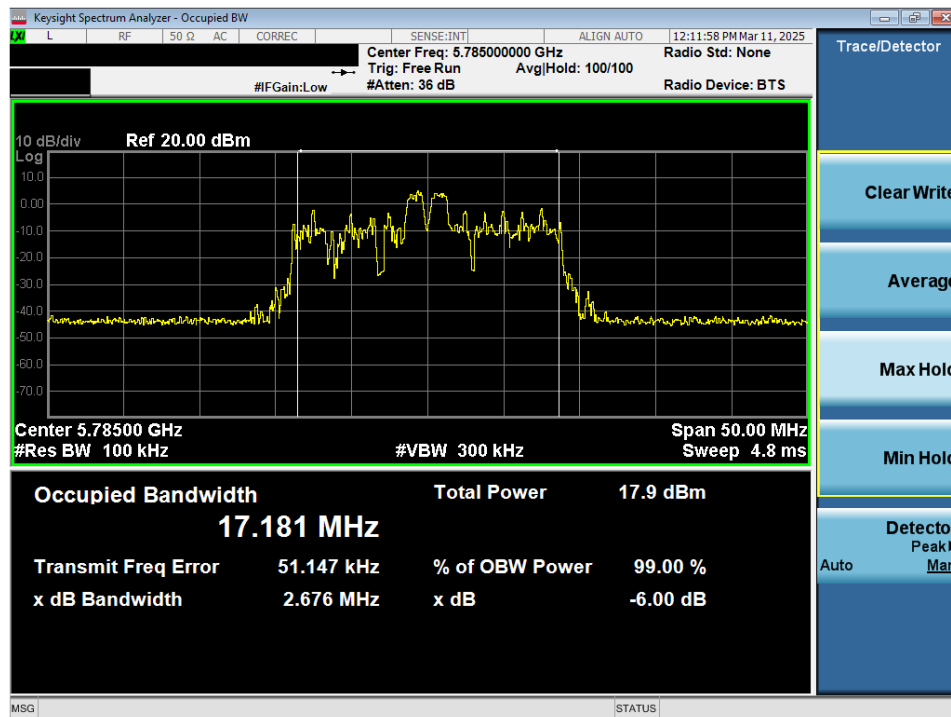
Plot 7-42. 6dB Bandwidth Plot MIMO ANT2 (20MHz 802.11ax/be (26 Tones) (UNII Band 3) – Ch. 157)
