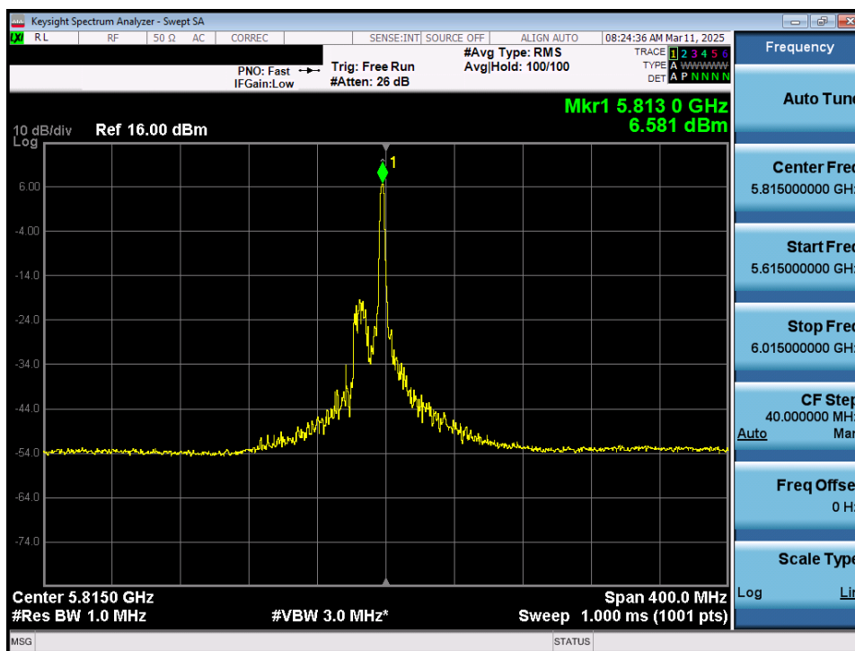
Plot 7-80. Power Spectral Density Plot MIMO ANT1 (160MHz 802.11ax/be (26 Tones) (UNII Band 3/4) – Ch. 163)
