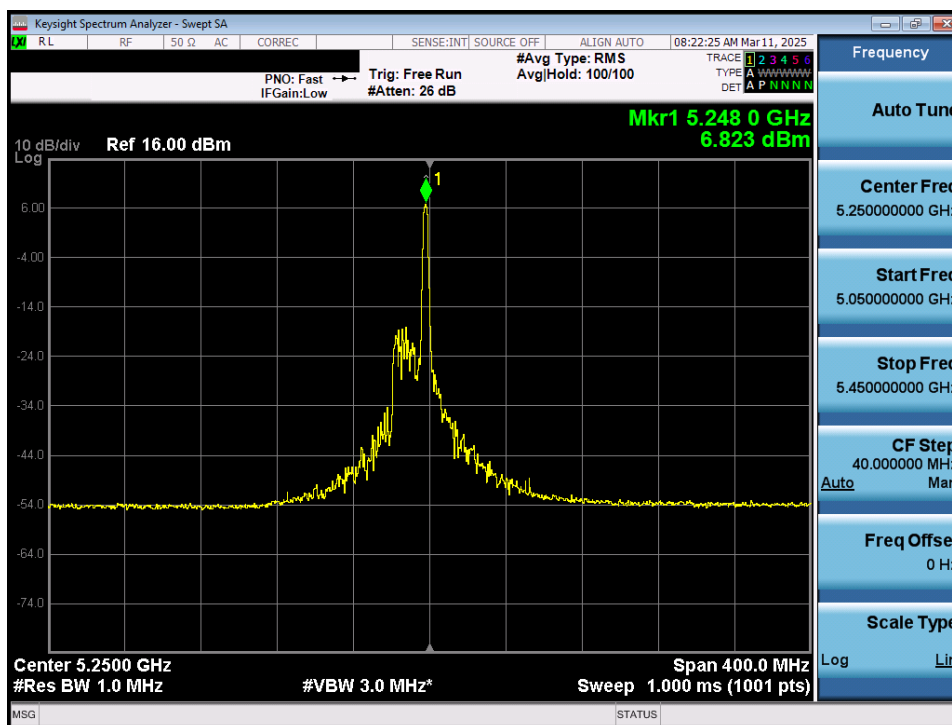
Plot 7-64. Power Spectral Density Plot MIMO ANT1 (160MHz 802.11ax/be (26 Tones) (UNII Band 1/2A) – Ch. 50)
