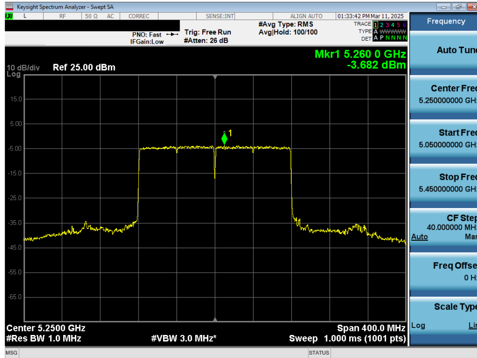
Plot 7-101. Power Spectral Density Plot MIMO ANT2 (160MHz 802.11ax/be (Full Tones) (UNII Band 1/2A) – Ch. 50)
