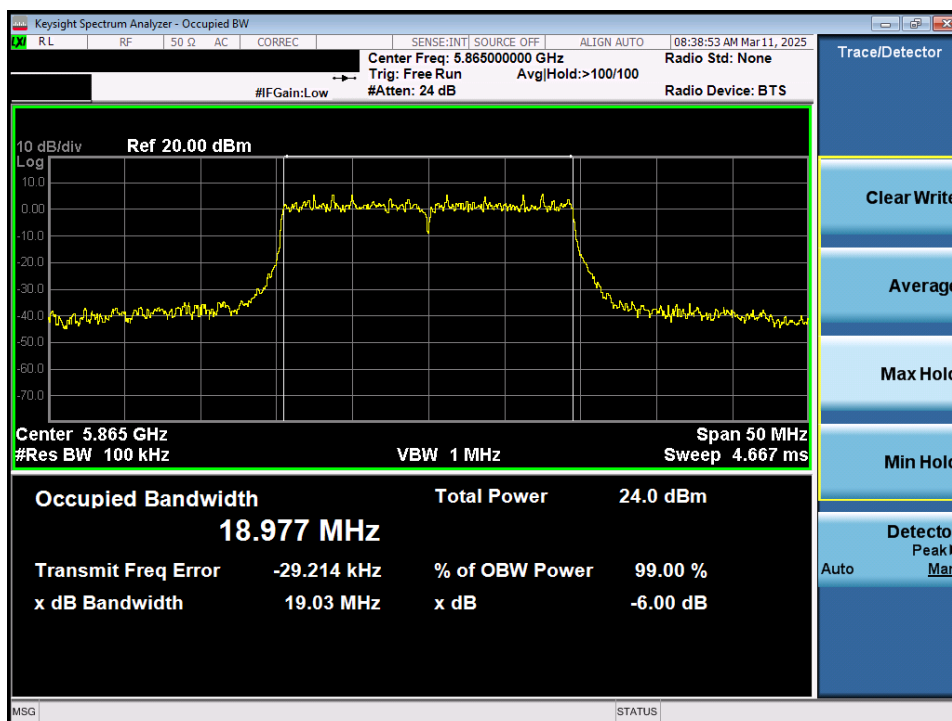
Plot 7-38. 6dB Bandwidth Plot MIMO ANT1 (20MHz 802.11ax/be (Full Tones) (UNII Band 4) – Ch. 173)
