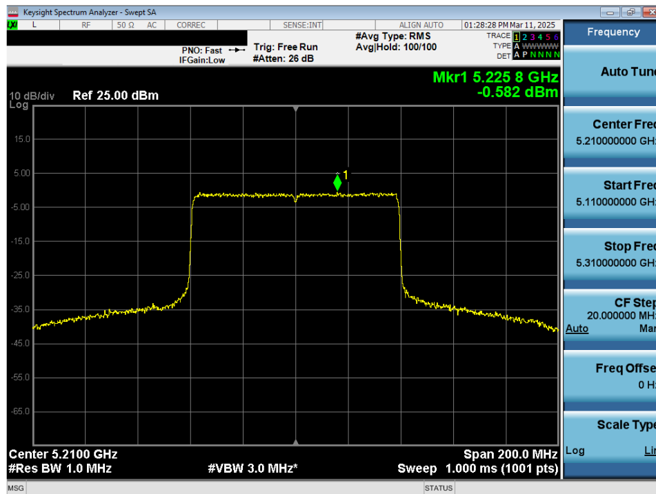
Plot 7-100. Power Spectral Density Plot MIMO ANT2 (80MHz 802.11ax/be (Full Tones) (UNII Band 1) – Ch. 42)
