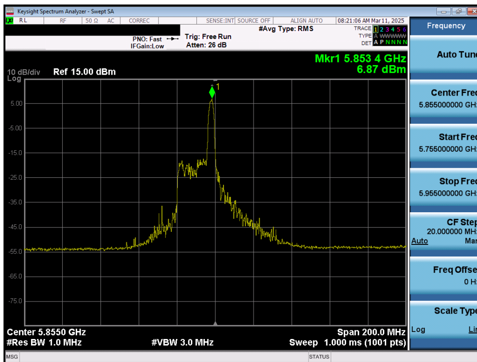
Plot 7-79. Power Spectral Density Plot MIMO ANT1 (80MHz 802.11ax/be (26 Tones) (UNII Band 3/4) – Ch. 171)
