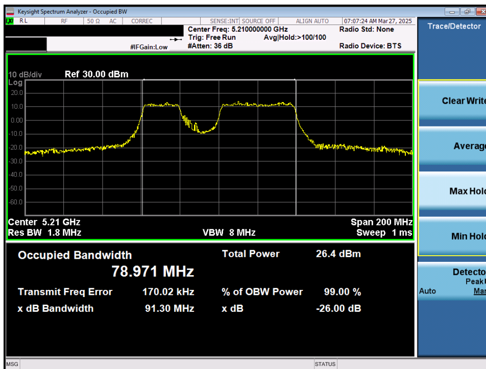
Plot 7-6. 26dB Bandwidth Plot MIMO ANT1 (80MHz 802.11be (484+242 Tones) (UNII Band 1) – Ch. 42)
