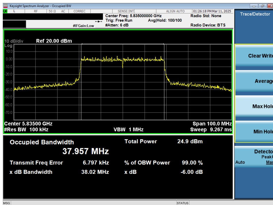
Plot 7-58. 6dB Bandwidth Plot MIMO ANT2 (40MHz 802.11ax/be (Full Tones) (UNII Band 3/4) – Ch. 167)
