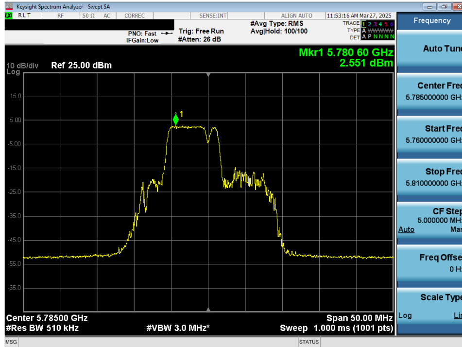
Plot 7-105. Power Spectral Density Plot MIMO ANT2 (20MHz 802.11be (52+26 Tones) (UNII Band 3) – Ch. 157)
