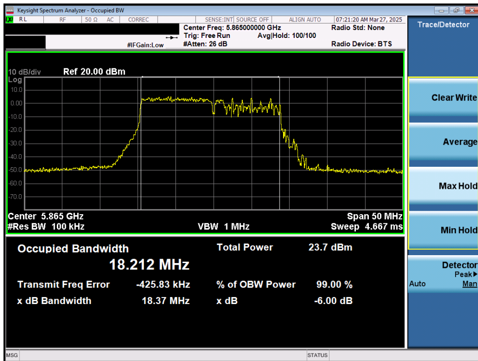
Plot 7-32. 6dB Bandwidth Plot MIMO ANT1 (20MHz 802.11be (106+26 Tones) (UNII Band 4) – Ch. 173)
