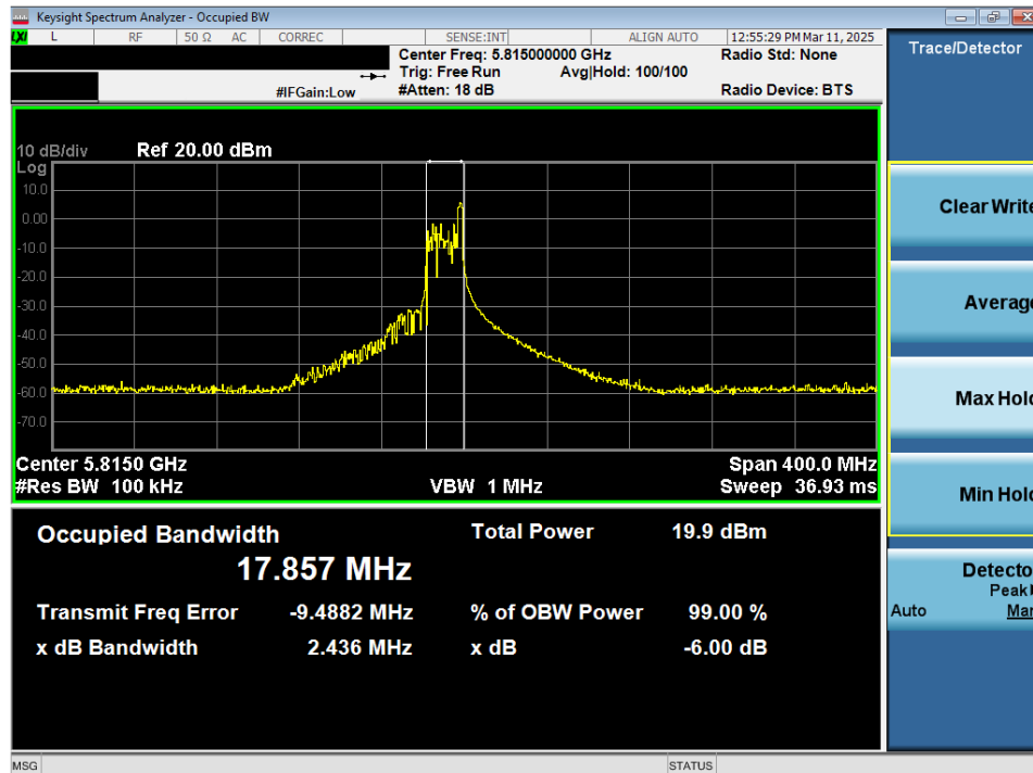
Plot 7-50. 6dB Bandwidth Plot MIMO ANT2 (160MHz 802.11ax/be (26 Tones) (UNII Band 3/4) – Ch. 163)
