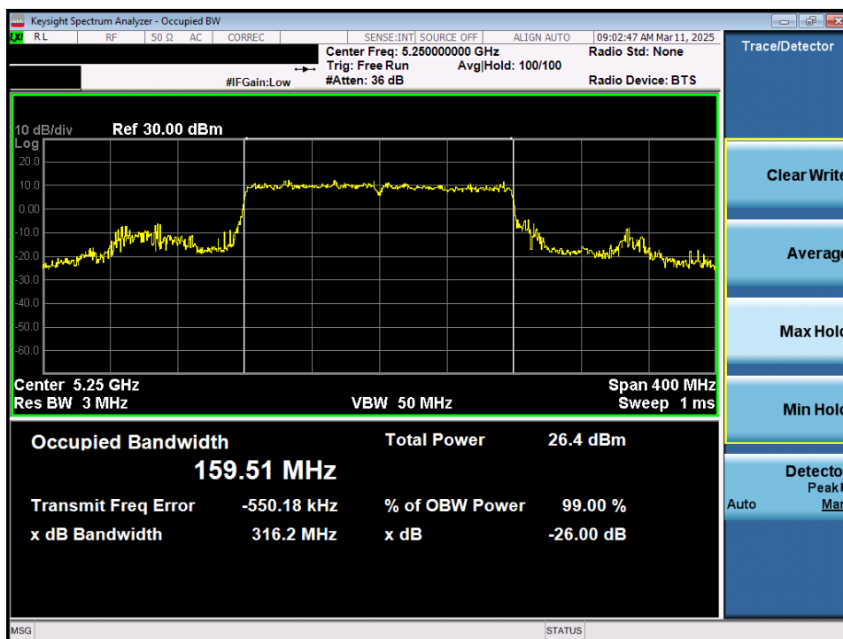
Plot 7-11. 26dB Bandwidth Plot MIMO ANT1 (160MHz 802.11ax/be (Full Tones) (UNII Band 1/2A) – Ch. 50)
