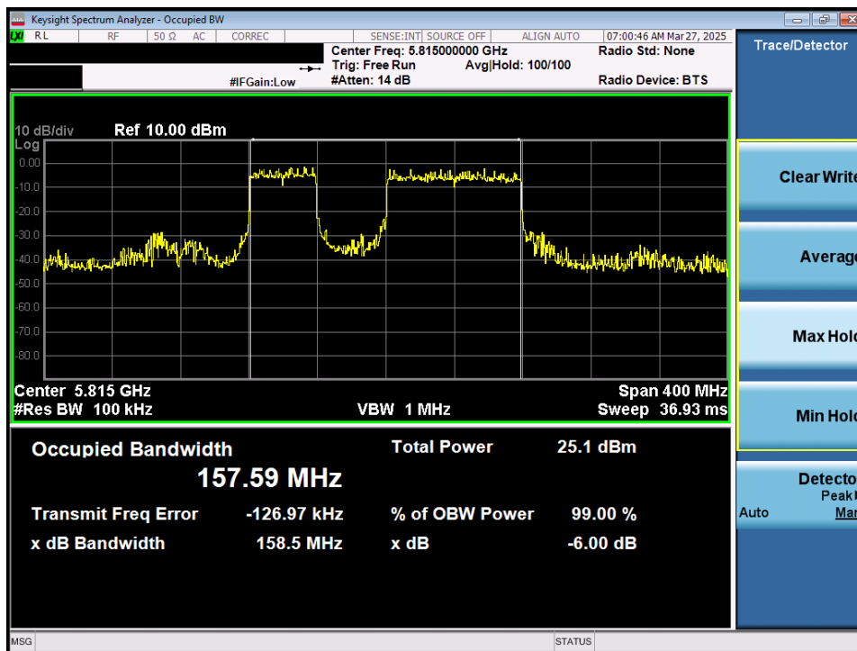
Plot 7-34. 6dB Bandwidth Plot MIMO ANT1 (160MHz 802.11be (996+484 Tones) (UNII Band 3/4) – Ch. 163)
