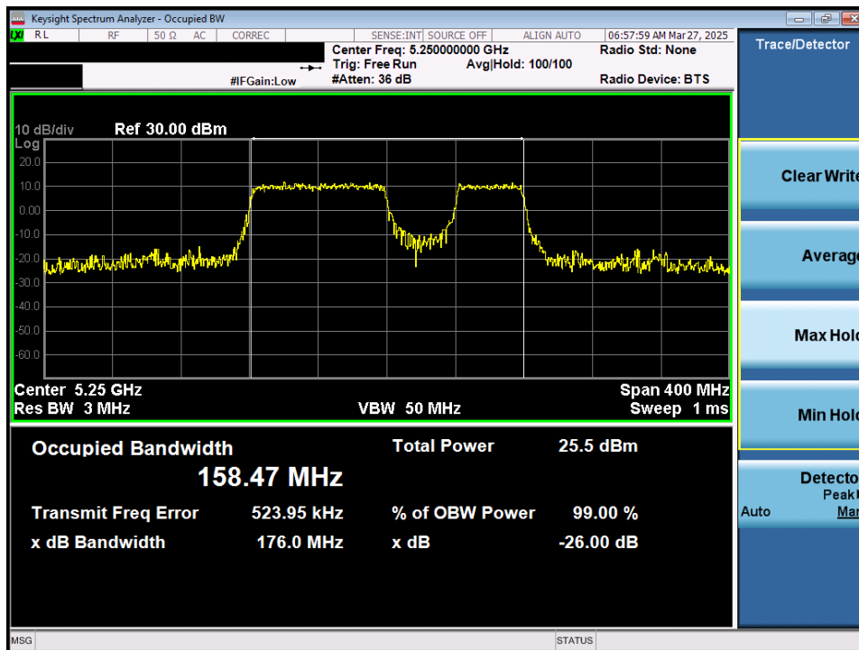
Plot 7-7. 26dB Bandwidth Plot MIMO ANT1 (160MHz 802.11be (996+484 Tones) (UNII Band 1/2A) – Ch. 50)
