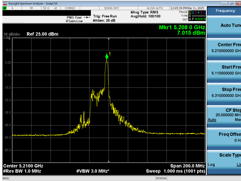
Plot 7-93. Power Spectral Density Plot MIMO ANT2 (80MHz 802.11ax/be (26 Tones) (UNII Band 1) – Ch. 42)
