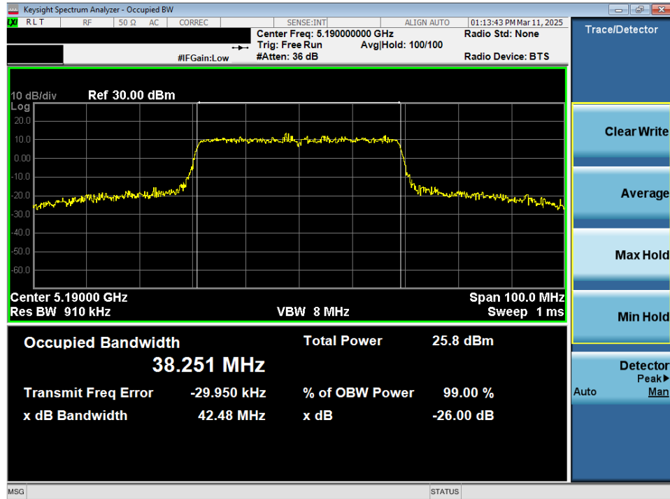
Plot 7-20. 26dB Bandwidth Plot MIMO ANT2 (40MHz 802.11ax/be (Full Tones) (UNII Band 1) – Ch. 38)
