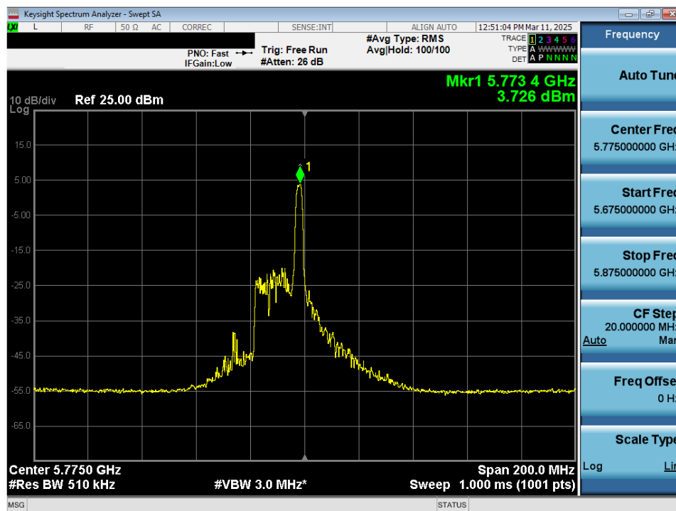
Plot 7-104. Power Spectral Density Plot MIMO ANT2 (80MHz 802.11ax/be (26 Tones) (UNII Band 3) – Ch. 155)
