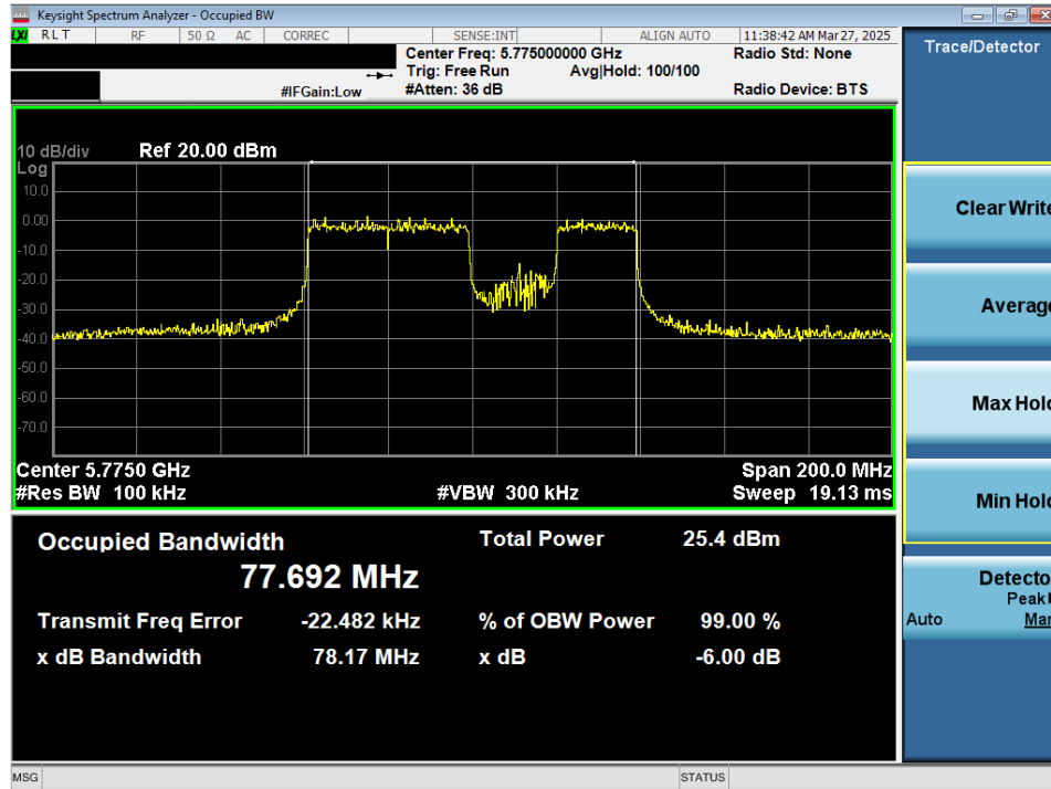
Plot 7-46. 6dB Bandwidth Plot MIMO ANT2 (80MHz 802.11be (484+242 Tones) (UNII Band 3) – Ch. 155)
