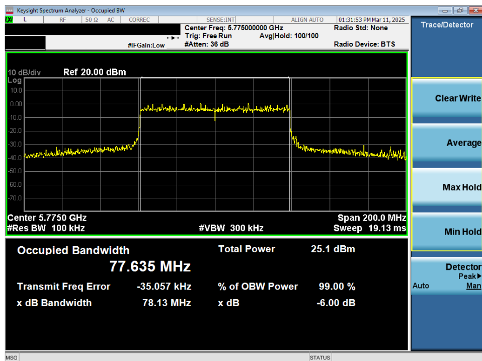
Plot 7-56. 6dB Bandwidth Plot MIMO ANT2 (80MHz 802.11ax/be (Full Tones) (UNII Band 3) – Ch. 155)
