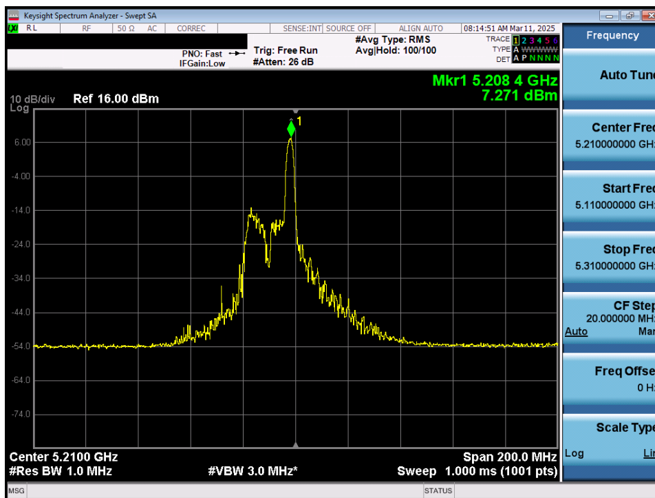
Plot 7-63. Power Spectral Density Plot MIMO ANT1 (80MHz 802.11ax/be (26 Tones) (UNII Band 1) – Ch. 42)
