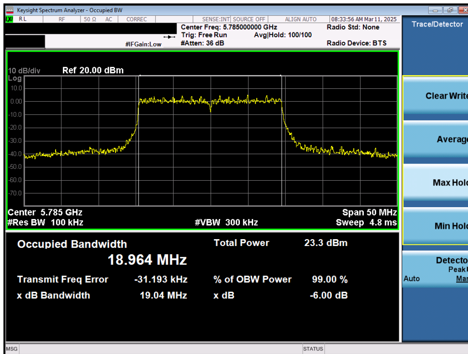
Plot 7-35. 6dB Bandwidth Plot MIMO ANT1 (20MHz 802.11ax/be (Full Tones) (UNII Band 3) – Ch. 157)
