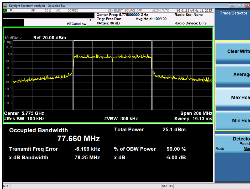
Plot 7-37. 6dB Bandwidth Plot MIMO ANT1 (80MHz 802.11ax/be (Full Tones) (UNII Band 3) – Ch. 155)
