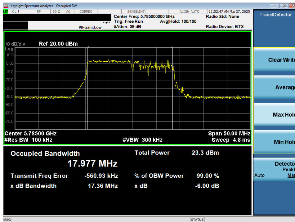
Plot 7-45. 6dB Bandwidth Plot MIMO ANT2 (20MHz 802.11be (106+26 Tones) (UNII Band 3) – Ch. 157)
