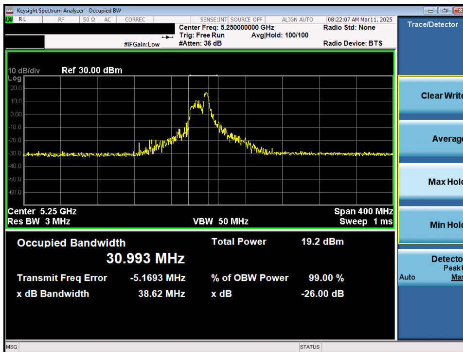
Plot 7-4. 26dB Bandwidth Plot MIMO ANT1 (160MHz 802.11ax/be (26 Tones) (UNII Band 1/2A) – Ch. 50)
