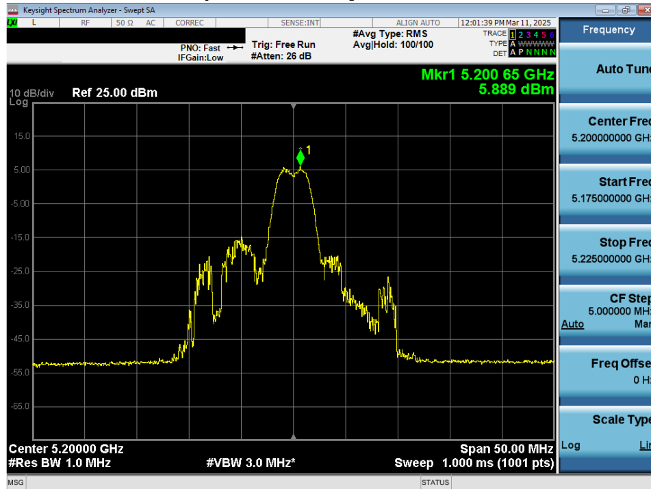
Plot 7-91. Power Spectral Density Plot MIMO ANT2 (20MHz 802.11ax/be (26 Tones) (UNII Band 1) – Ch. 40)
