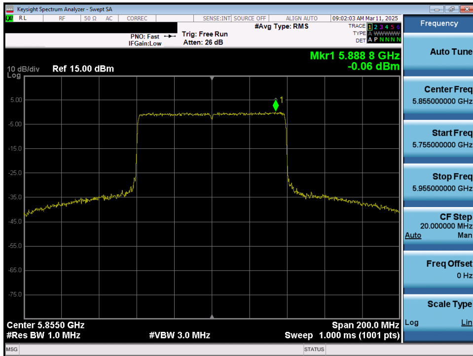
Plot 7-89. Power Spectral Density Plot MIMO ANT1 (80MHz 802.11ax/be (Full Tones) (UNII Band 3/4) – Ch. 171)
