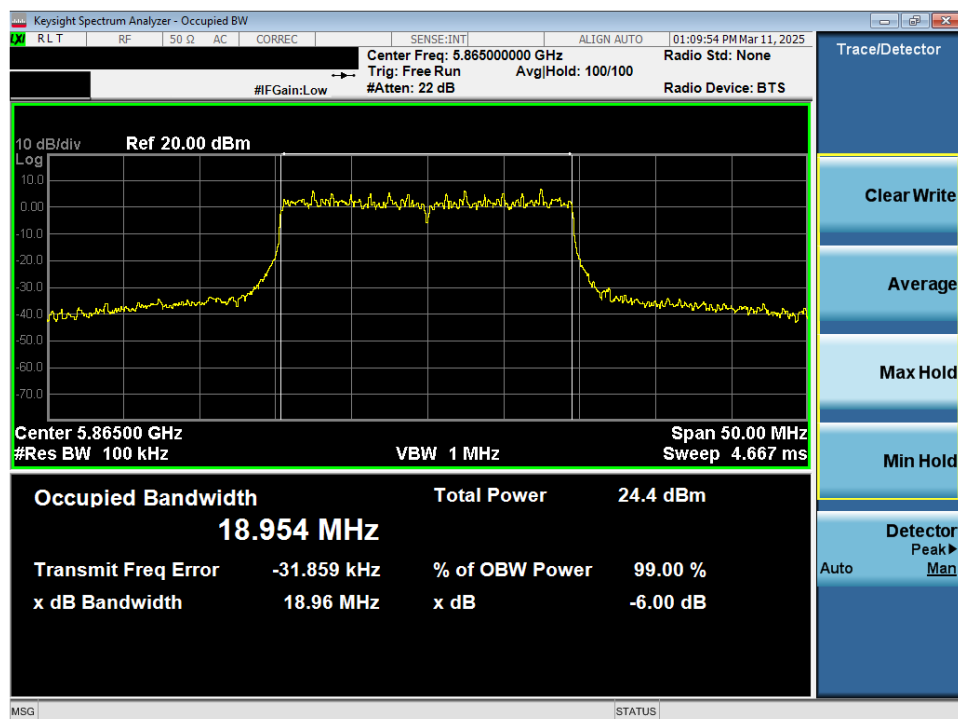
Plot 7-57. 6dB Bandwidth Plot MIMO ANT2 (20MHz 802.11ax/be (Full Tones) (UNII Band 4) – Ch. 173)
