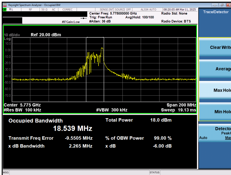
Plot 7-25. 6dB Bandwidth Plot MIMO ANT1 (80MHz 802.11ax/be (26 Tones) (UNII Band 3) – Ch. 155)
