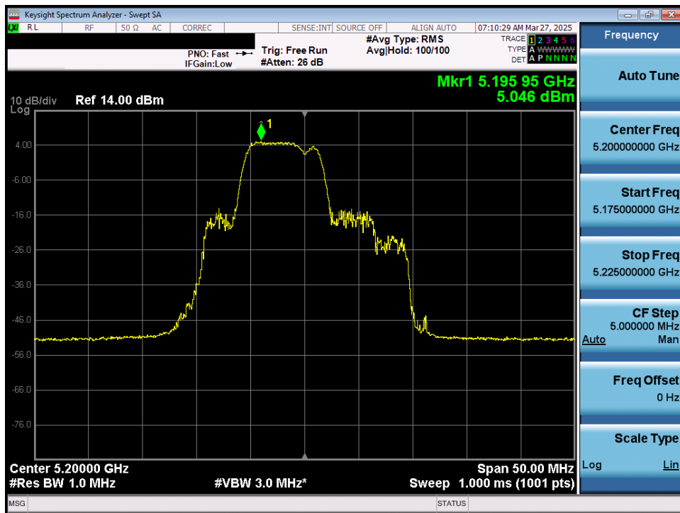
Plot 7-65. Power Spectral Density Plot MIMO ANT1 (20MHz 802.11be (52+26 Tones) (UNII Band 1) – Ch. 40)
