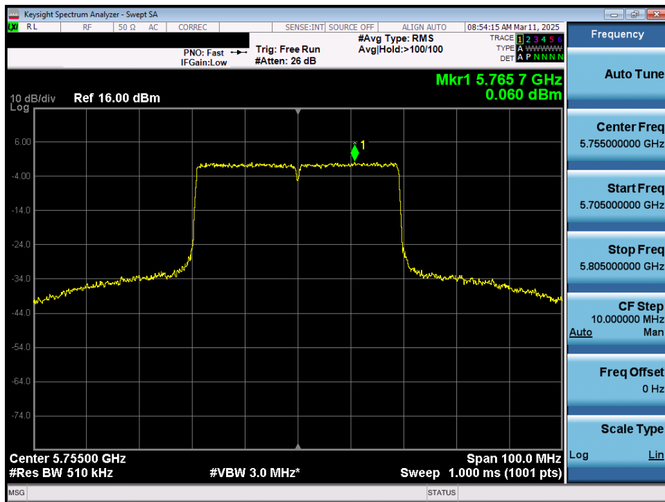
Plot 7-85. Power Spectral Density Plot MIMO ANT1 (40MHz 802.11ax/be (Full Tones) (UNII Band 3) – Ch. 151)
