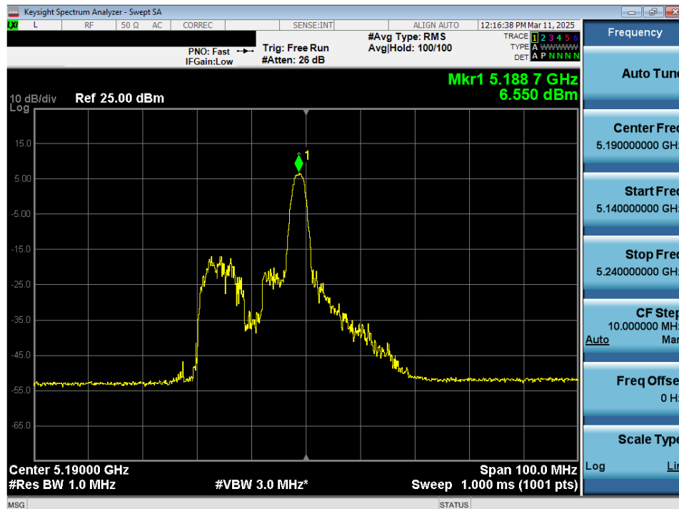
Plot 7-92. Power Spectral Density Plot MIMO ANT2 (40MHz 802.11ax/be (26 Tones) (UNII Band 1) – Ch. 38)
