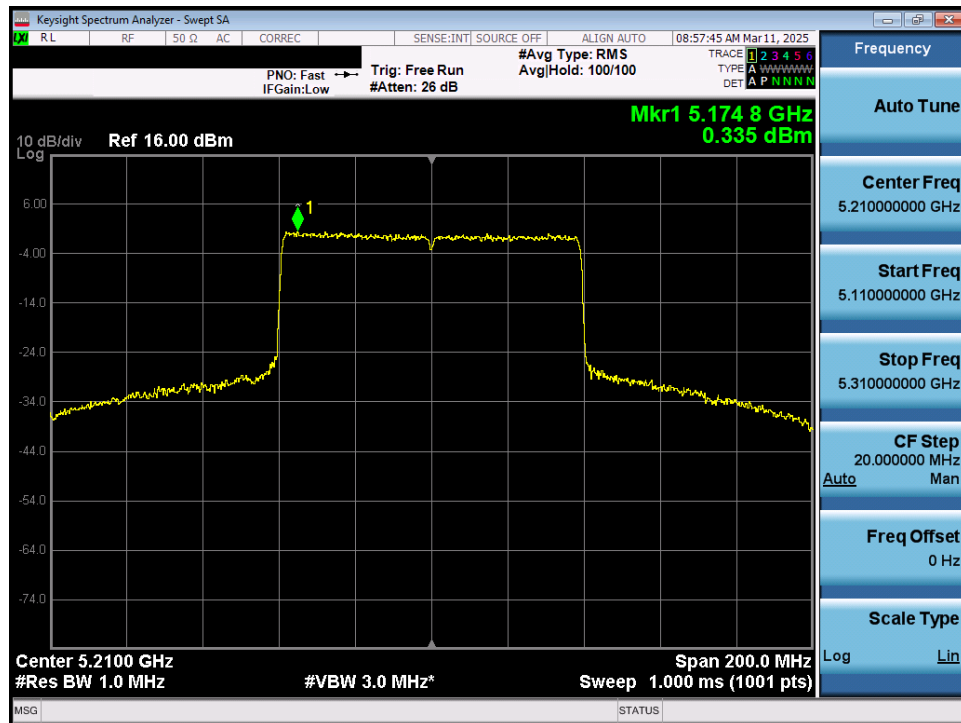
Plot 7-70. Power Spectral Density Plot MIMO ANT1 (80MHz 802.11ax/be (Full Tones) (UNII Band 1) – Ch. 42)
