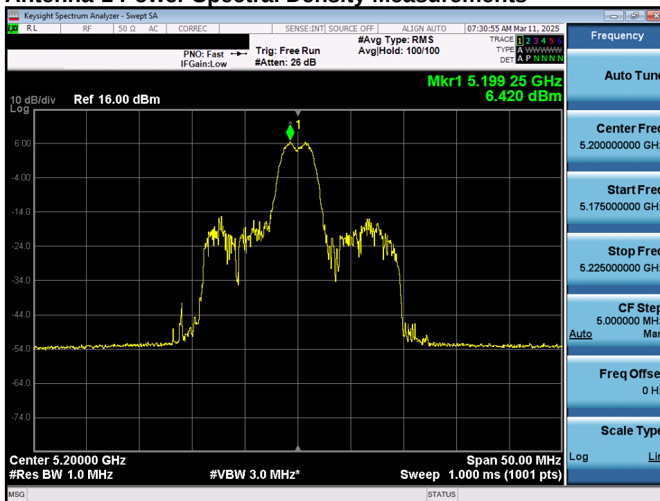
Plot 7-61. Power Spectral Density Plot MIMO ANT1 (20MHz 802.11ax/be (26 Tones) (UNII Band 1) – Ch. 40)
