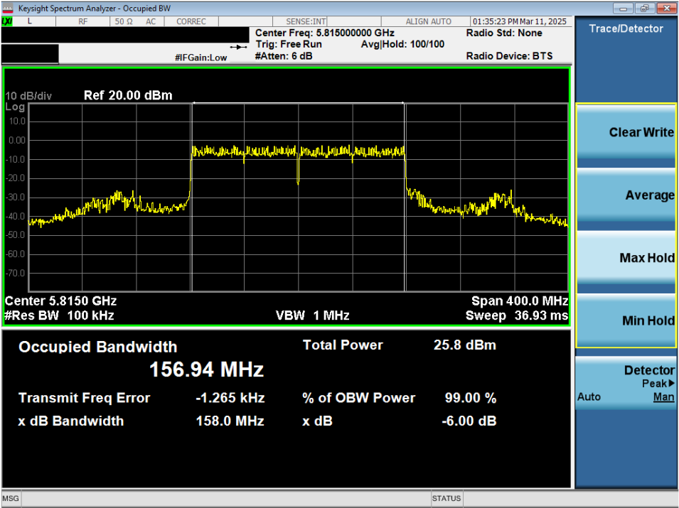
Plot 7-60. 6dB Bandwidth Plot MIMO ANT2 (160MHz 802.11ax/be (Full Tones) (UNII Band 3/4) – Ch. 163)
