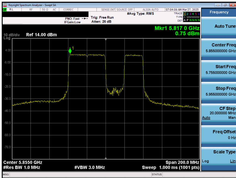
Plot 7-82. Power Spectral Density Plot MIMO ANT1 (80MHz 802.11be (484+242 Tones) (UNII Band 3/4) – Ch. 171)
