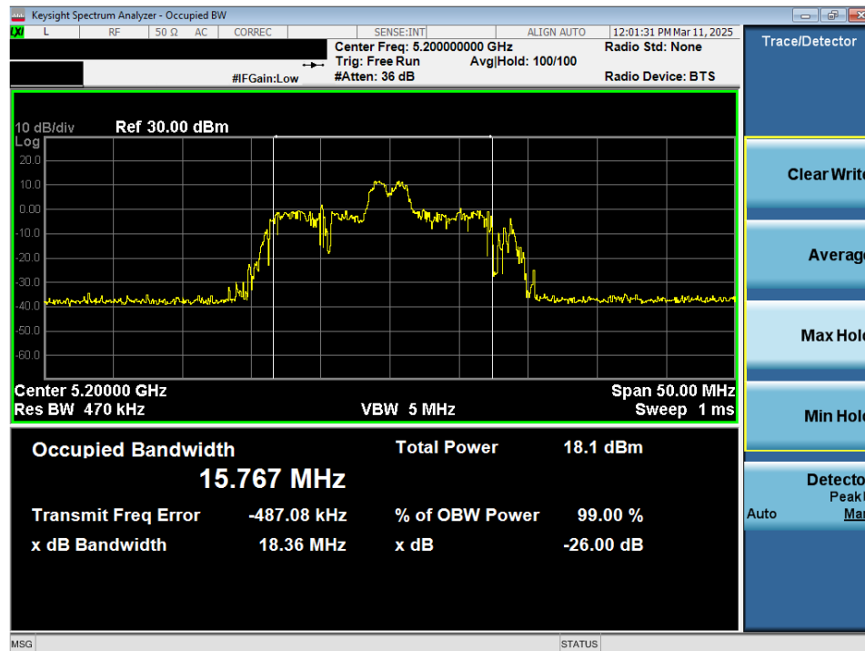
Plot 7-12. 26dB Bandwidth Plot MIMO ANT2 (20MHz 802.11ax/be (26 Tones) (UNII Band 1) – Ch. 40)
