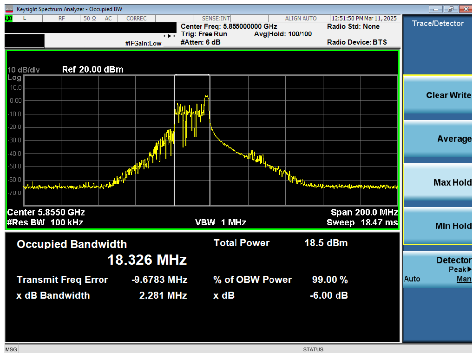
Plot 7-49. 6dB Bandwidth Plot MIMO ANT2 (80MHz 802.11ax/be (26 Tones) (UNII Band 3/4) – Ch. 171)
