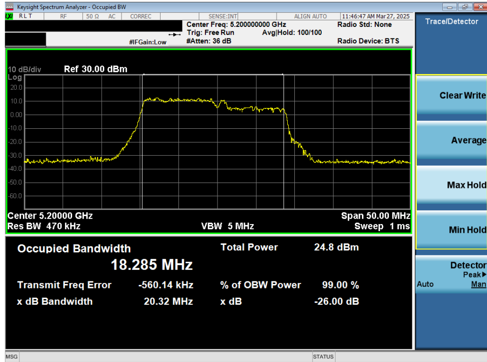
Plot 7-16. 26dB Bandwidth Plot MIMO ANT2 (20MHz 802.11be (106+26 Tones) (UNII Band 1) – Ch. 40)
