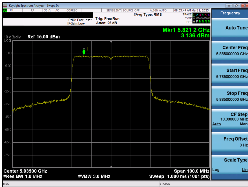
Plot 7-88. Power Spectral Density Plot MIMO ANT1 (40MHz 802.11ax/be (Full Tones) (UNII Band 3/4) – Ch. 167)
