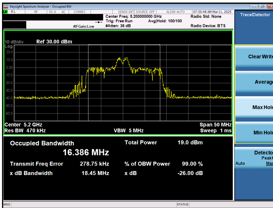
Plot 7-1. 26dB Bandwidth Plot MIMO ANT1 (20MHz 802.11ax/be (26 Tones) (UNII Band 1) – Ch. 40)
