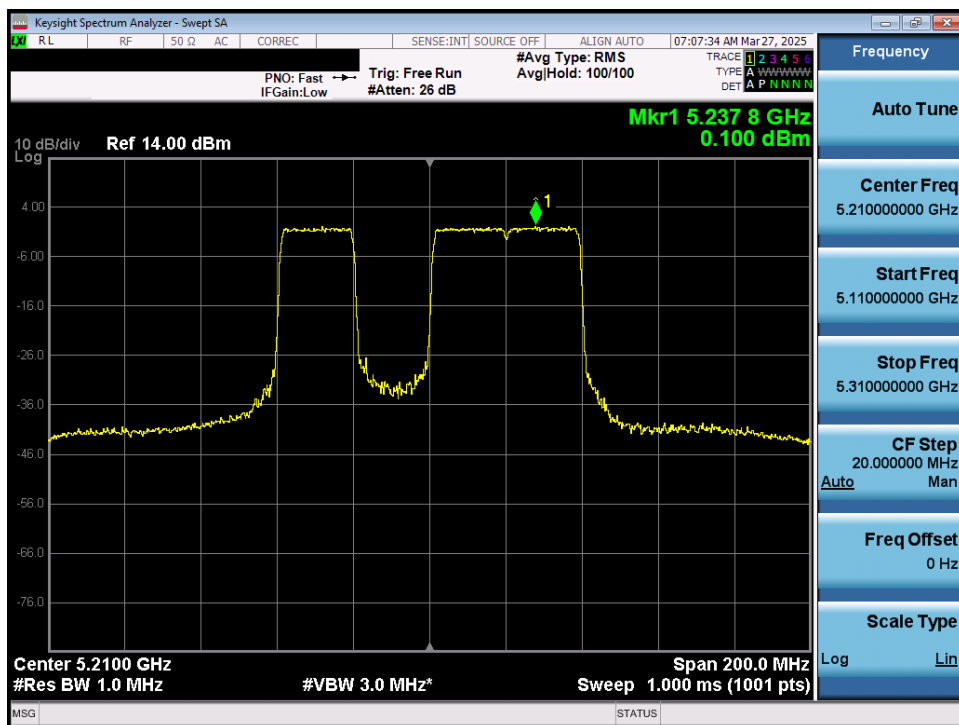
Plot 7-66. Power Spectral Density Plot MIMO ANT1 (80MHz 802.11be (484+242 Tones) (UNII Band 1) – Ch. 42)
