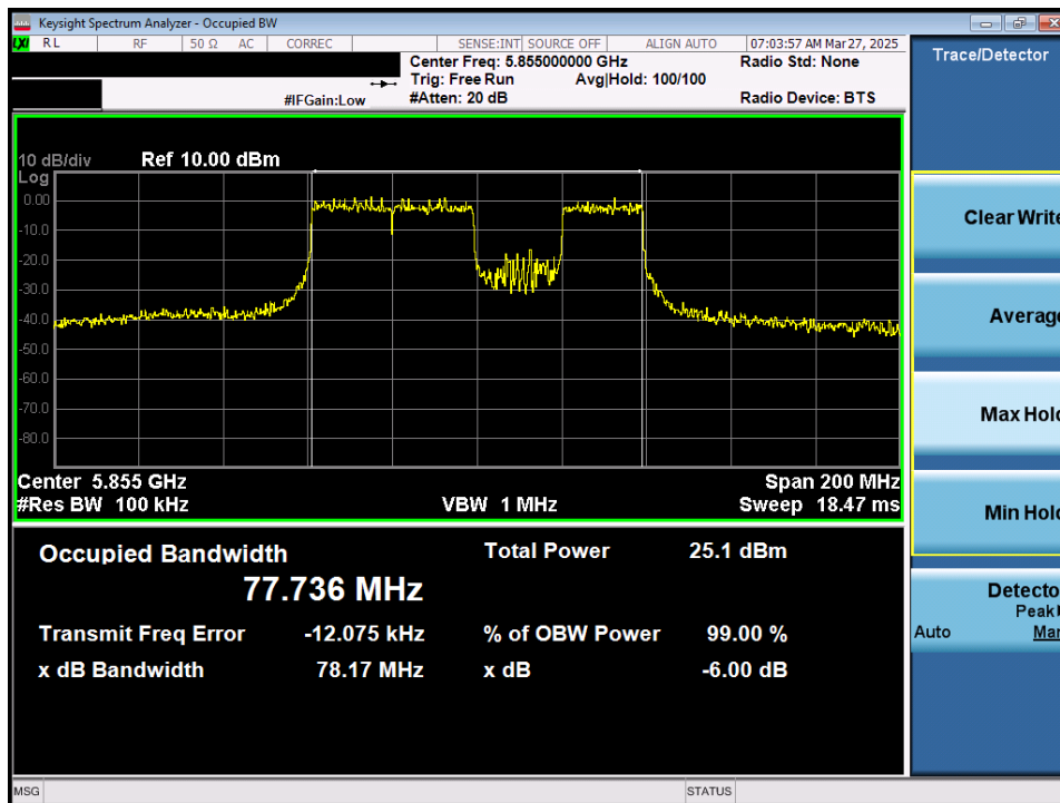
Plot 7-33. 6dB Bandwidth Plot MIMO ANT1 (80MHz 802.11be (484+242 Tones) (UNII Band 3/4) – Ch. 171)
