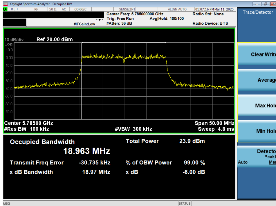
Plot 7-54. 6dB Bandwidth Plot MIMO ANT2 (20MHz 802.11ax/be (Full Tones) (UNII Band 3) – Ch. 157)
