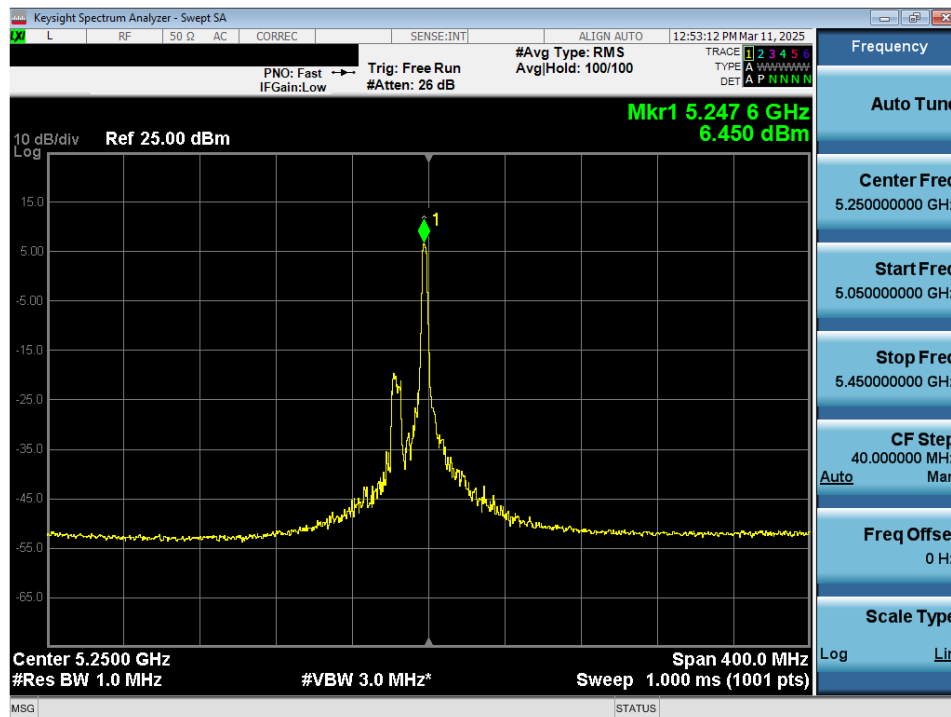
Plot 7-94. Power Spectral Density Plot MIMO ANT2 (160MHz 802.11ax/be (26 Tones) (UNII Band 1/2A) – Ch. 50)
