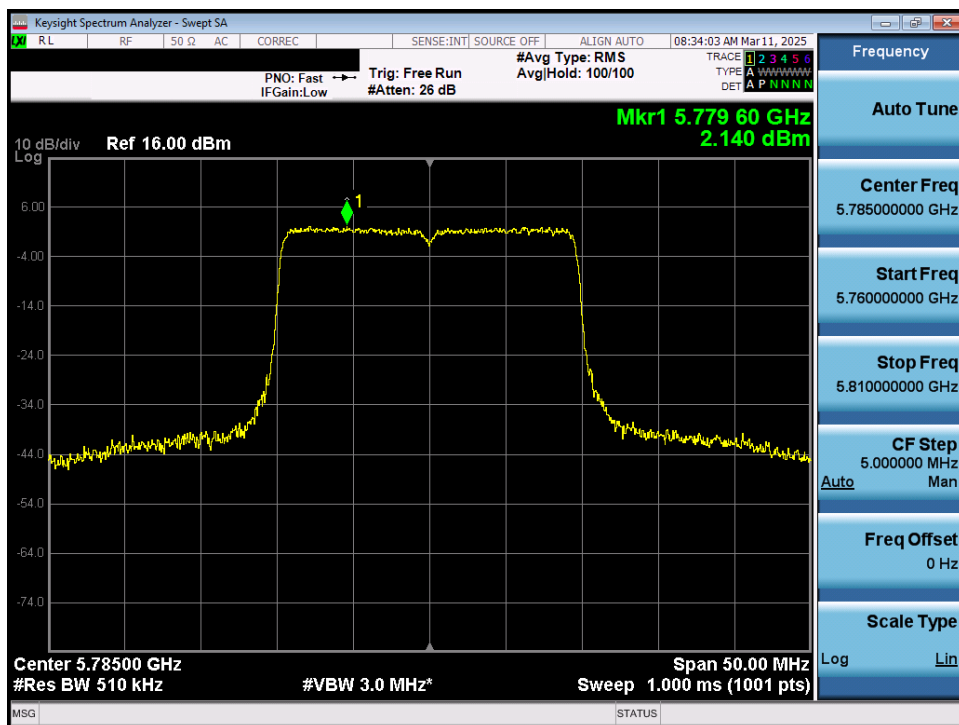
Plot 7-84. Power Spectral Density Plot MIMO ANT1 (20MHz 802.11ax/be (Full Tones) (UNII Band 3) – Ch. 157)
