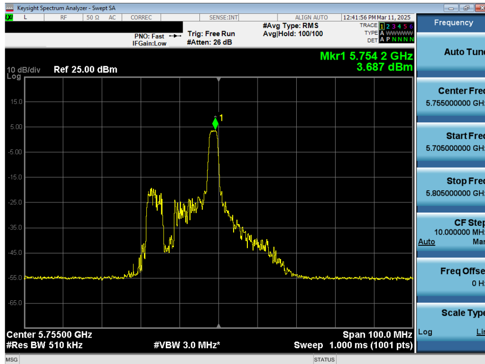
Plot 7-103. Power Spectral Density Plot MIMO ANT2 (40MHz 802.11ax/be (26 Tones) (UNII Band 3) – Ch. 151)
