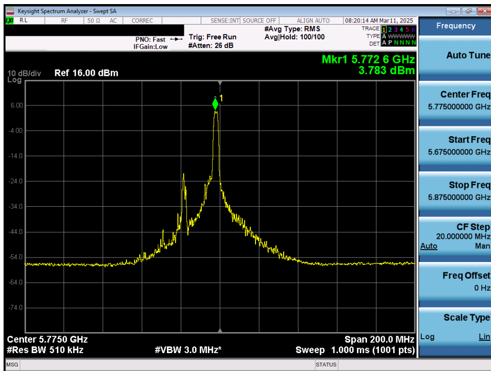
Plot 7-74. Power Spectral Density Plot MIMO ANT1 (80MHz 802.11ax/be (26 Tones) (UNII Band 3) – Ch. 155)
