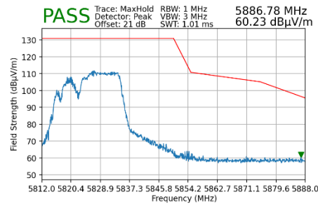
Plot 7-151. Radiated Upper Band Edge Plot MIMO (Peak – UNII Band 3 – 106+26 Tones)
