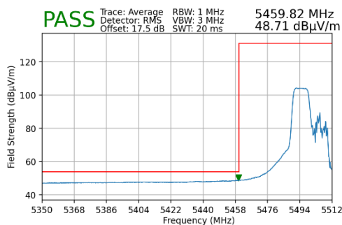
Plot 7-139. Radiated Lower Band Edge Plot MIMO (Average – UNII Band 2C – 106 Tones)
