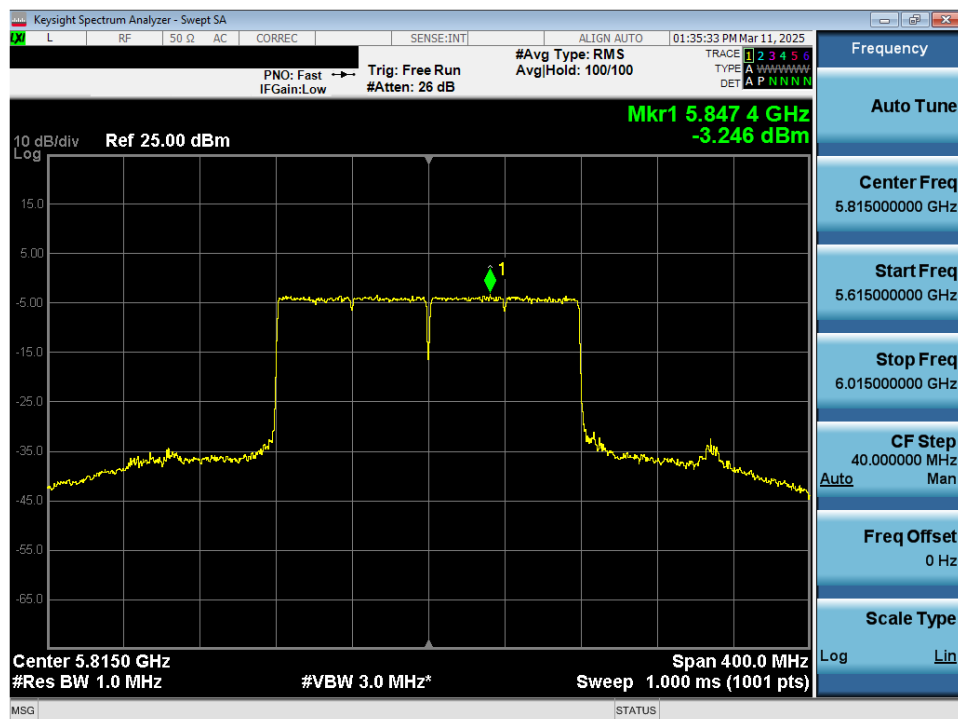
Plot 7-120. Power Spectral Density Plot MIMO ANT2 (160MHz 802.11ax/be (Full Tones) (UNII Band 3/4) – Ch. 163)
