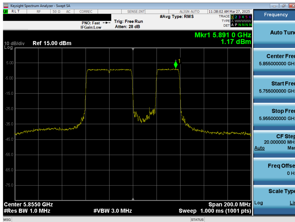
Plot 7-112. Power Spectral Density Plot MIMO ANT2 (80MHz 802.11be (484+242 Tones) (UNII Band 3/4) – Ch. 171)
