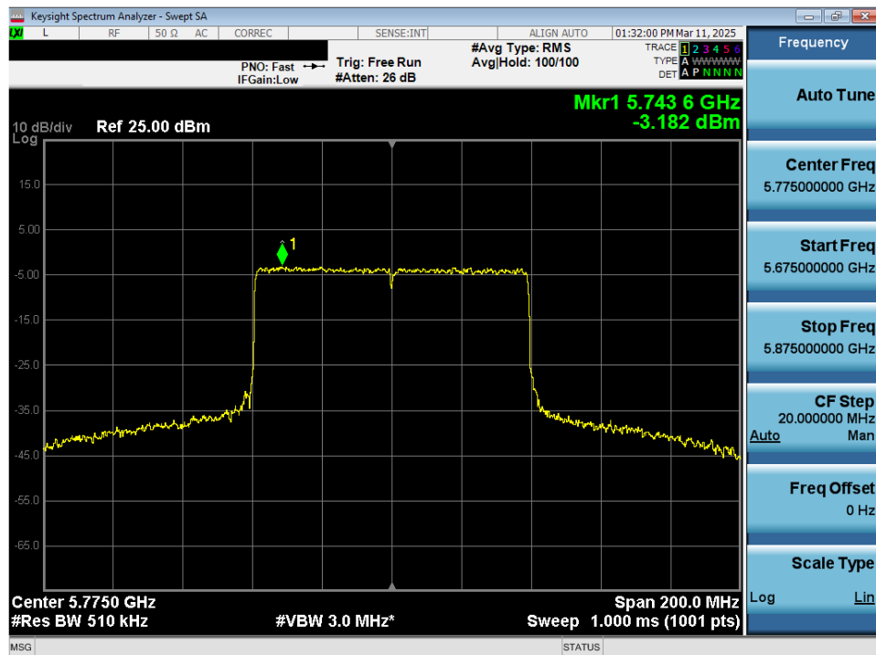
Plot 7-116. Power Spectral Density Plot MIMO ANT2 (80MHz 802.11ax/be (Full Tones) (UNII Band 3) – Ch. 155)
