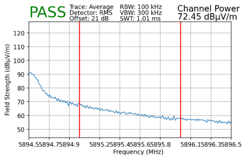
Plot 7-143. Radiated Upper Band Edge Plot MIMO (Average – UNII Band 4 – 106 Tones)
