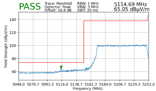
Plot 7-186. Radiated Lower Band Edge Plot MIMO (Peak – UNII Band 1 – 996 Tones)
