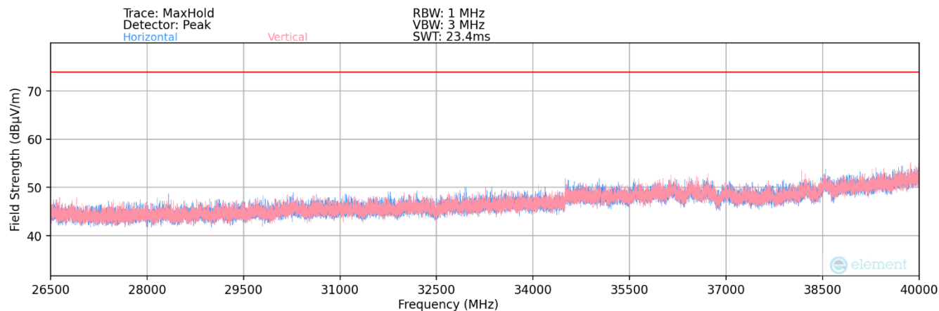
Plot 7-127. Radiated Spurious Plot 26.5GHz - 40GHz (802.11ax)
