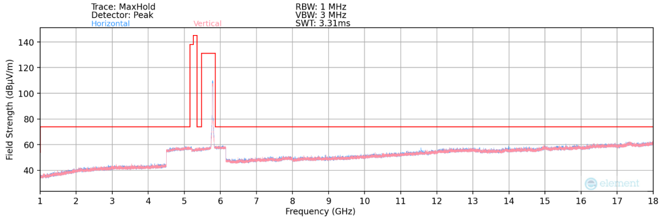
Plot 7-131. Radiated Spurious Plot above 1GHz MIMO (802.11ax – UNII 3 Ch. 157)
