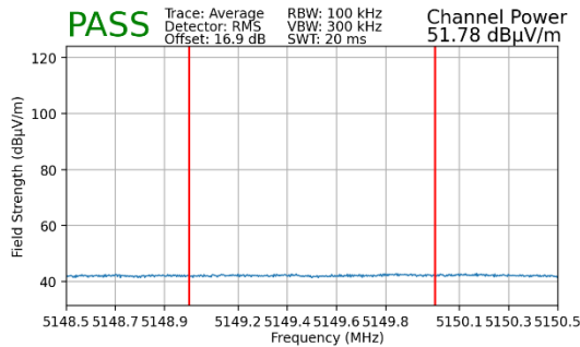
Plot 7-165. Radiated Lower Band Edge Plot MIMO (Average – UNII Band 1 – 484 Tones)
