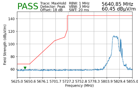
Plot 7-152. Radiated Lower Band Edge Plot MIMO (Peak - UNII Band 4 - 106+26 Tones)
