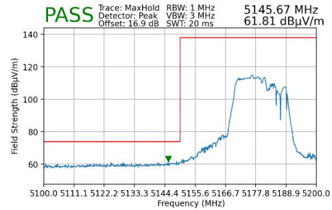
Plot 7-146. Radiated Lower Band Edge Plot MIMO (Peak – UNII Band 1 – 106+26 Tones)
