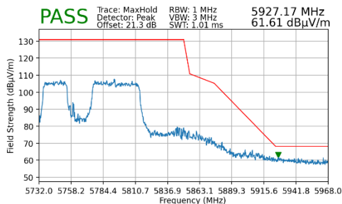
Plot 7-181. Radiated Upper Band Edge Plot MIMO (Peak – UNII Band 3 – 484+242 Tones)
