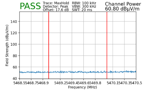
Plot 7-150. Radiated Lower Band Edge Plot MIMO (Peak – UNII Band 2C – 106+26 Tones)
