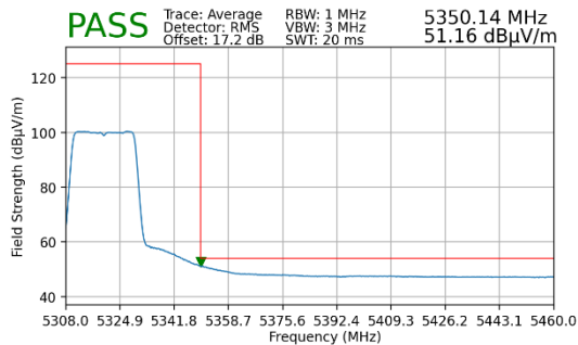
Plot 7-157. Radiated Upper Band Edge Plot MIMO (Average – UNII Band 2A – 242 Tones)
