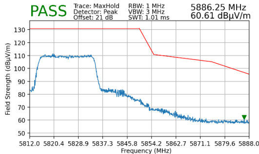
Plot 7-161. Radiated Upper Band Edge Plot MIMO (Peak – UNII Band 3 – 242 Tones)
