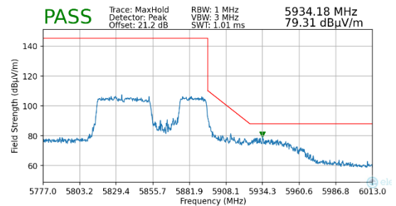
Plot 7-184. Radiated Upper Band Edge Plot MIMO (Peak – UNII Band 4 – 484+242 Tones)
