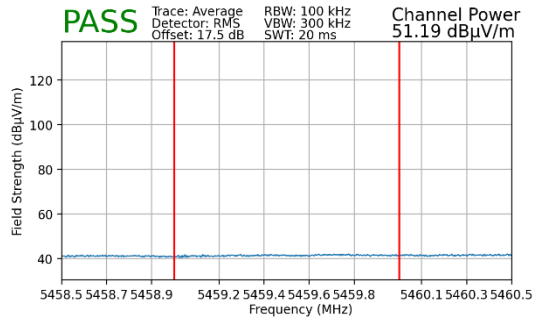
Plot 7-159. Radiated Lower Band Edge Plot MIMO (Average – UNII Band 2C – 242 Tones)
