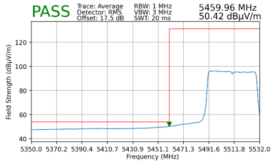
Plot 7-169. Radiated Lower Band Edge Plot MIMO (Average – UNII Band 2C – 484 Tones)
