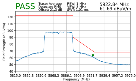
Plot 7-173. Radiated Upper Band Edge Plot MIMO (Average – UNII Band 4 – 484 Tones)
