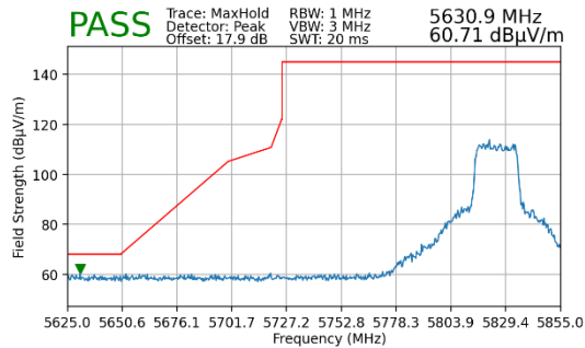
Plot 7-162. Radiated Lower Band Edge Plot MIMO (Peak – UNII Band 4 – 242 Tones)
