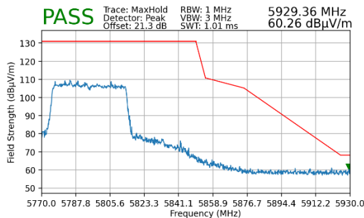
Plot 7-171. Radiated Upper Band Edge Plot MIMO (Peak – UNII Band 3 – 484 Tones)
