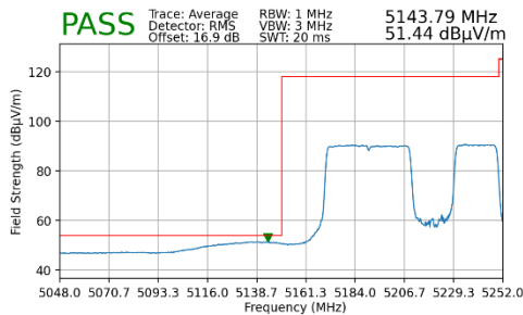
Plot 7-175. Radiated Lower Band Edge Plot MIMO (Average – UNII Band 1 – 484+242 Tones)
