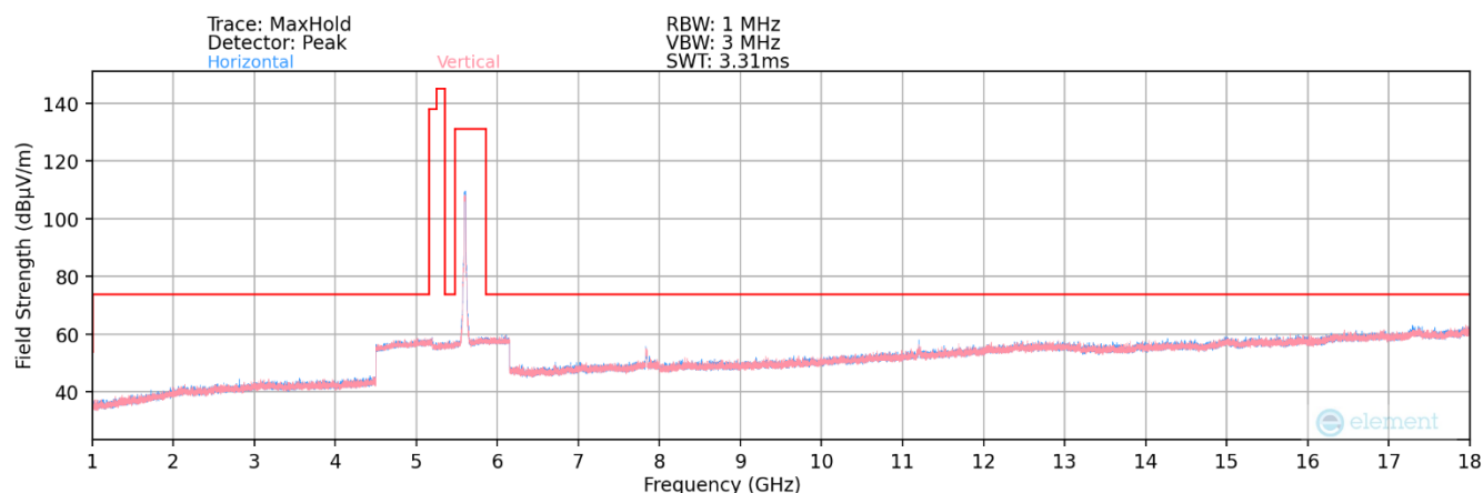
Plot 7-130. Radiated Spurious Plot above 1GHz MIMO (802.11ax – UNII 2C Ch. 120)
