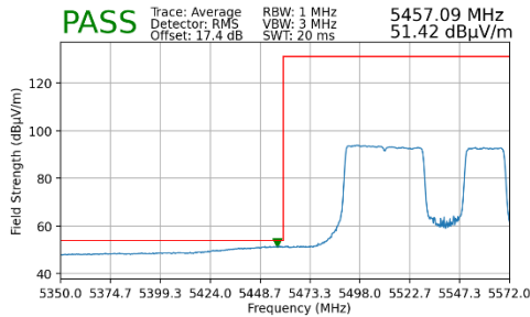
Plot 7-179. Radiated Lower Band Edge Plot MIMO (Average – UNII Band 2C – 484+242 Tones)
