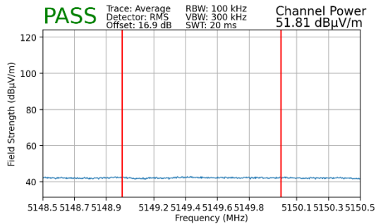
Plot 7-185. Radiated Lower Band Edge Plot MIMO (Average – UNII Band 1 – 996 Tones)
