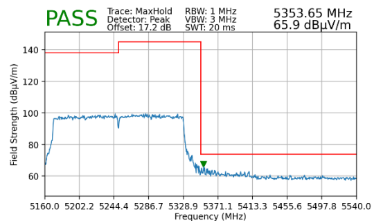
Plot 7-207. Radiated Upper Band Edge Plot MIMO (Peak – UNII Band 2A – 2x996 Tones)
