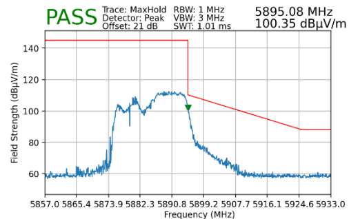
Plot 7-144. Radiated Upper Band Edge Plot MIMO (Peak – UNII Band 4 – 106 Tones)
