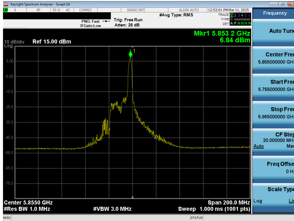
Plot 7-109. Power Spectral Density Plot MIMO ANT2 (80MHz 802.11ax/be (26 Tones) (UNII Band 3/4) – Ch. 171)
