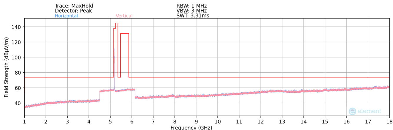
Plot 7-121. Radiated Spurious Plot above 1GHz MIMO (802.11ax – UNII 1 Ch. 40)
