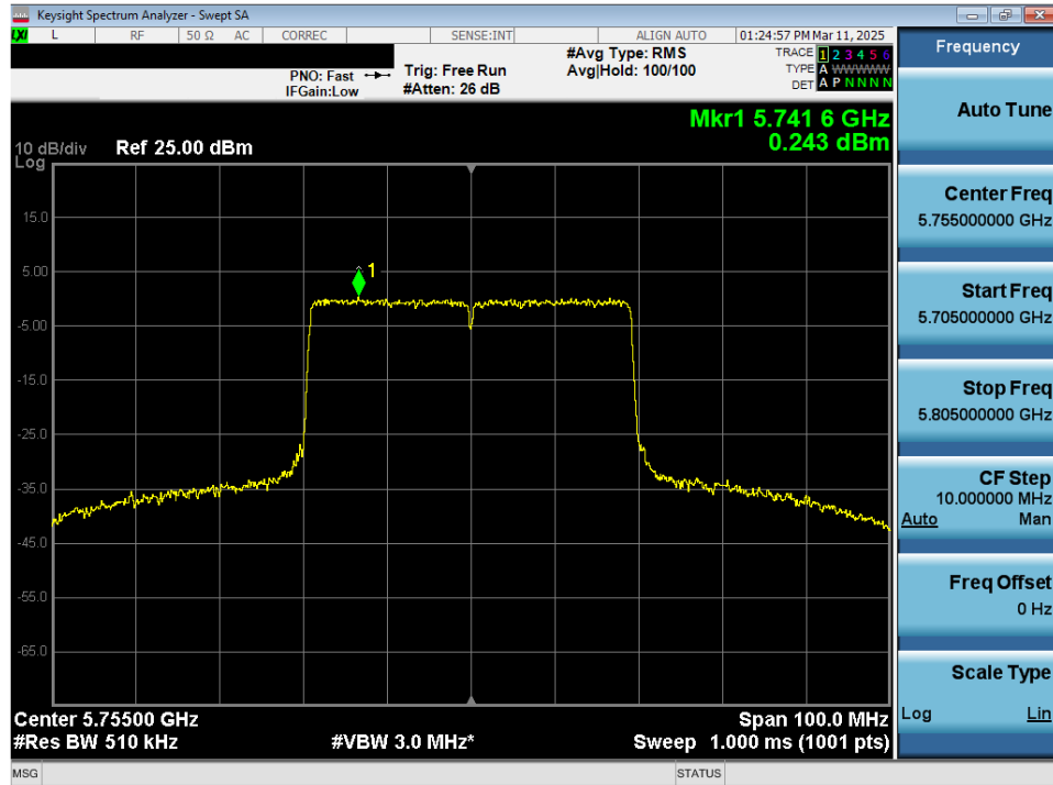
Plot 7-115. Power Spectral Density Plot MIMO ANT2 (40MHz 802.11ax/be (Full Tones) (UNII Band 3) – Ch. 151)
