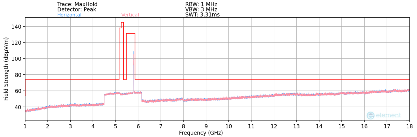
Plot 7-124. Radiated Spurious Plot above 1GHz MIMO (802.11ax – UNII 3 Ch. 157)
