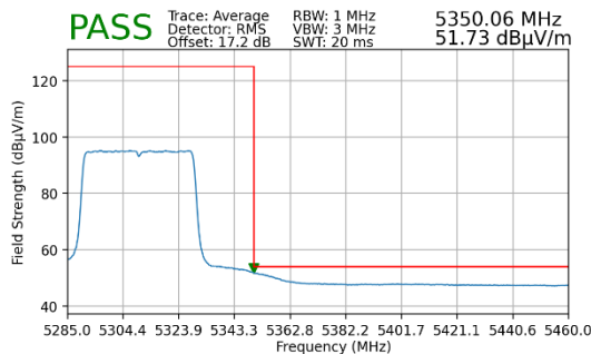
Plot 7-167. Radiated Upper Band Edge Plot MIMO (Average – UNII Band 2A – 484 Tones)
