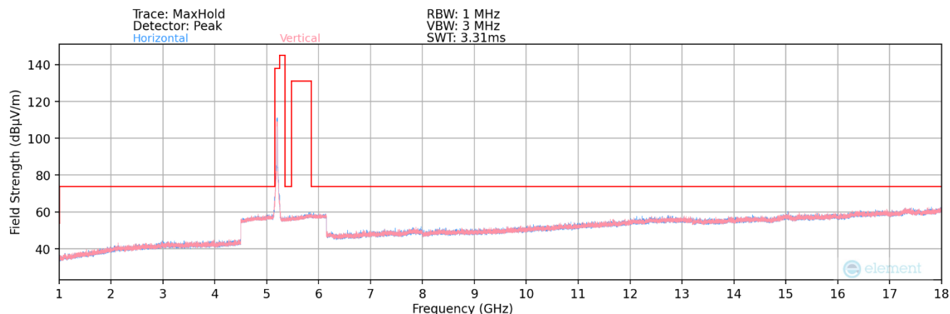
Plot 7-128. Radiated Spurious Plot above 1GHz MIMO (802.11ax – UNII 1 Ch. 40)
