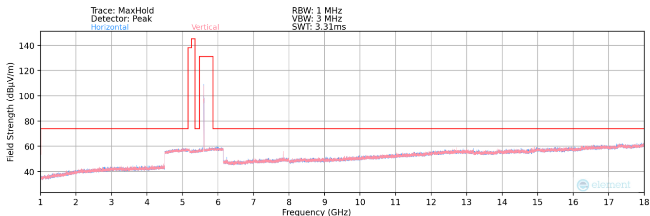
Plot 7-123. Radiated Spurious Plot above 1GHz MIMO (802.11ax – UNII 2C Ch. 120)
