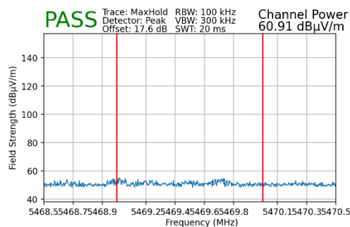
Plot 7-140. Radiated Lower Band Edge Plot MIMO (Peak – UNII Band 2C – 106 Tones)
