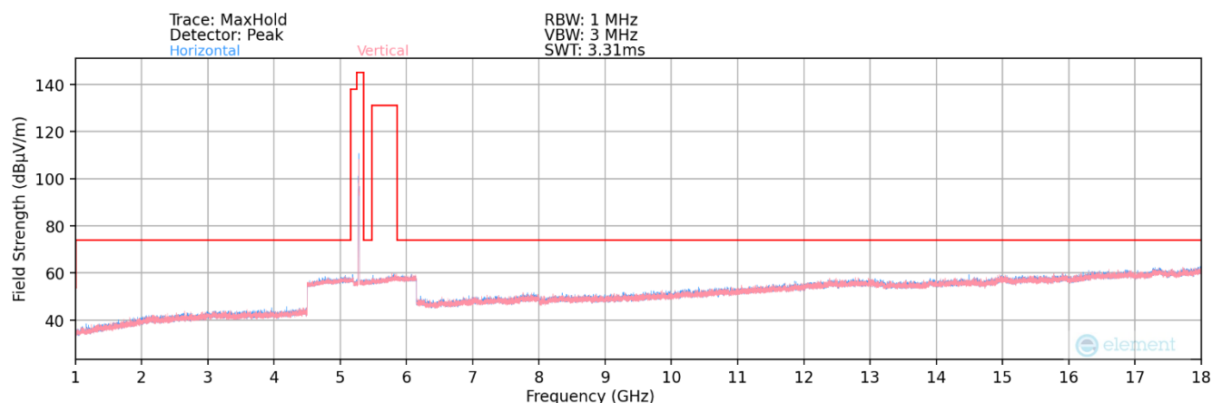
Plot 7-122. Radiated Spurious Plot above 1GHz MIMO (802.11ax – UNII 2A Ch. 56)
