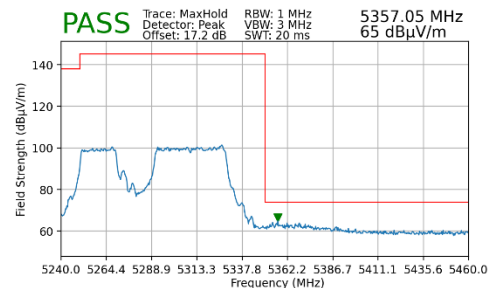
Plot 7-178. Radiated Upper Band Edge Plot MIMO (Peak – UNII Band 2A – 484+242 Tones)
