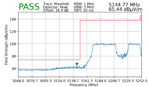
Plot 7-176. Radiated Lower Band Edge Plot MIMO (Peak – UNII Band 1 – 484+242 Tones)
