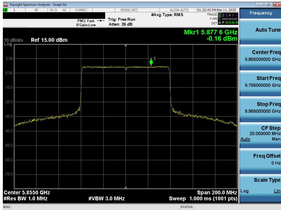
Plot 7-119. Power Spectral Density Plot MIMO ANT2 (80MHz 802.11ax/be (Full Tones) (UNII Band 3/4) – Ch. 171)
