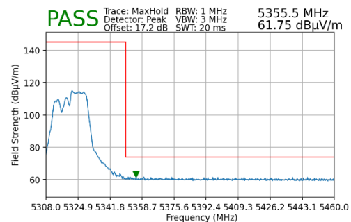
Plot 7-138. Radiated Upper Band Edge Plot MIMO (Peak – UNII Band 2A – 106 Tones)
