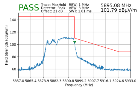
Plot 7-154. Radiated Upper Band Edge Plot MIMO (Peak - UNII Band 4 - 106+26 Tones)
