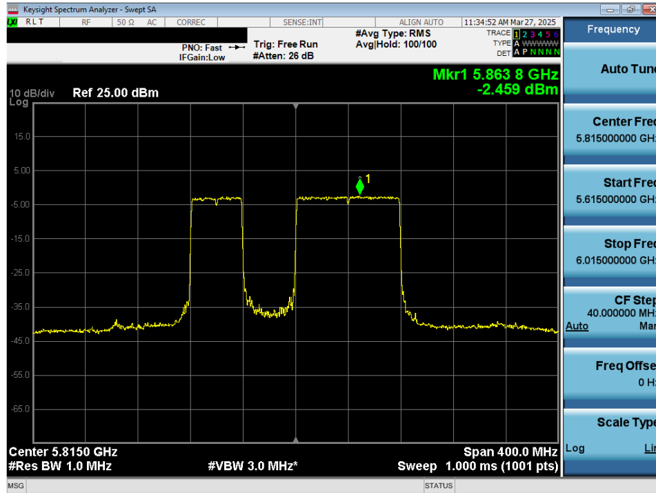
Plot 7-113. Power Spectral Density Plot MIMO ANT2 (160MHz 802.11be (996+484 Tones) (UNII Band 3/4) – Ch. 163)
