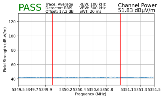
Plot 7-187. Radiated Upper Band Edge Plot MIMO (Average – UNII Band 2A – 996 Tones)
