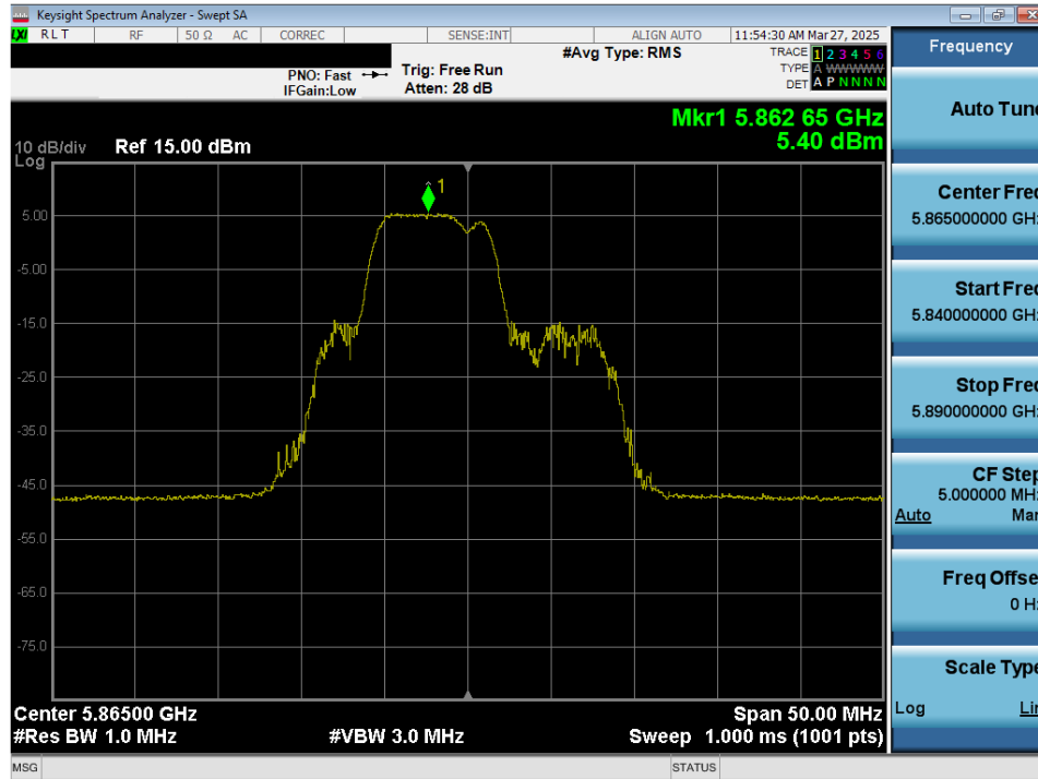
Plot 7-111. Power Spectral Density Plot MIMO ANT2 (20MHz 802.11be (52+26 Tones) (UNII Band 4) – Ch. 173)
