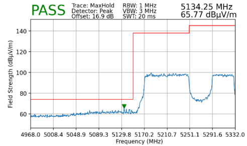
Plot 7-196. Radiated Lower Band Edge Plot MIMO (Peak – UNII Band 1 – 996+484 Tones)
