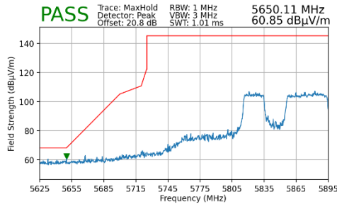
Plot 7-182. Radiated Lower Band Edge Plot MIMO (Peak – UNII Band 4 – 484+242 Tones)
