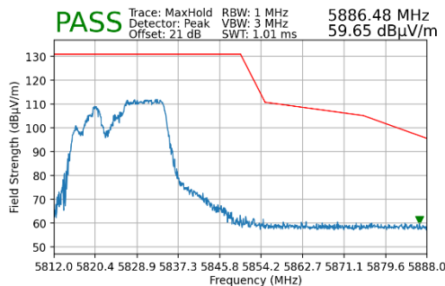
Plot 7-141. Radiated Upper Band Edge Plot MIMO (Peak – UNII Band 3 – 106 Tones)
