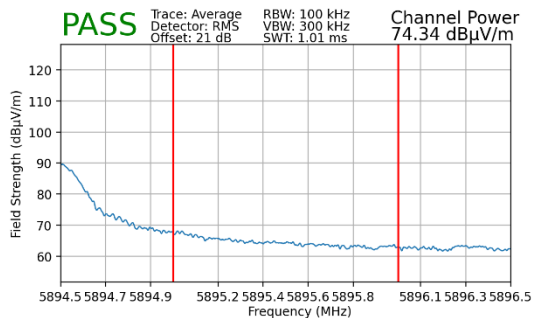
Plot 7-163. Radiated Upper Band Edge Plot MIMO (Average – UNII Band 4 – 242 Tones)
