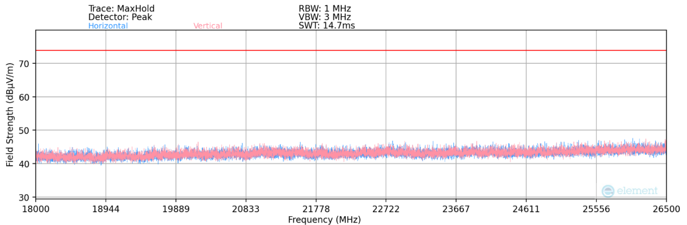
Plot 7-126. Radiated Spurious Plot 18GHz - 26.5GHz (802.11ax)
