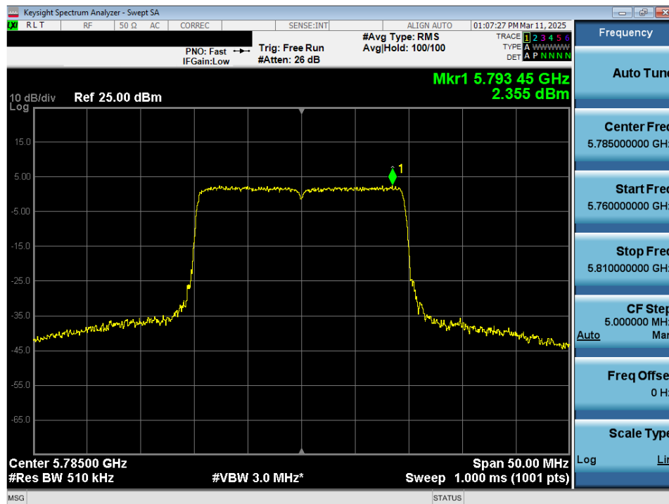
Plot 7-114. Power Spectral Density Plot MIMO ANT2 (20MHz 802.11ax/be (Full Tones) (UNII Band 3) – Ch. 157)
