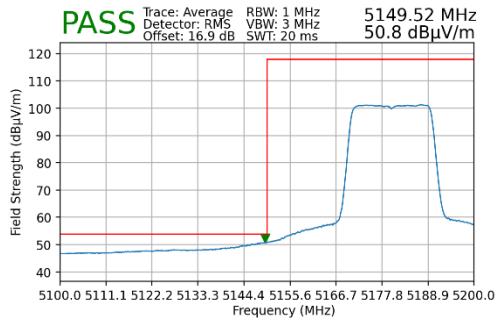
Plot 7-155. Radiated Lower Band Edge Plot MIMO (Average – UNII Band 1 – 242 Tones)
