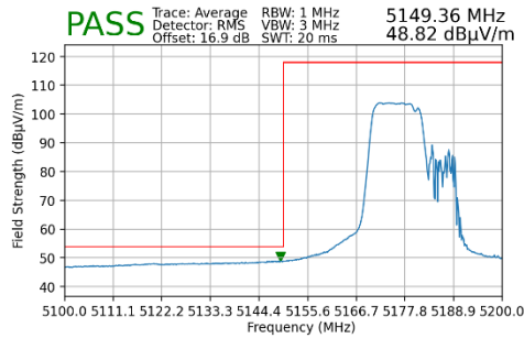
Plot 7-145. Radiated Lower Band Edge Plot MIMO (Average – UNII Band 1 – 106+26 Tones)
