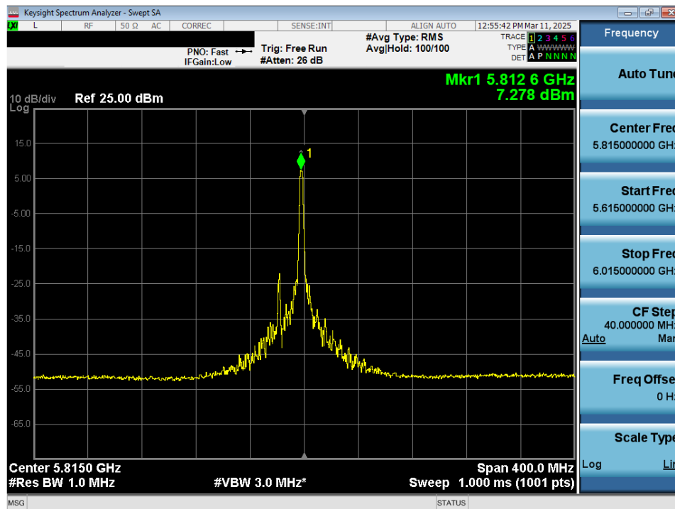
Plot 7-110. Power Spectral Density Plot MIMO ANT2 (160MHz 802.11ax/be (26 Tones) (UNII Band 3/4) – Ch. 163)
