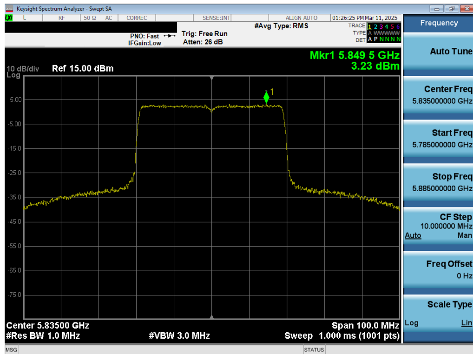
Plot 7-118. Power Spectral Density Plot MIMO ANT2 (40MHz 802.11ax/be (Full Tones) (UNII Band 3/4) – Ch. 167)
