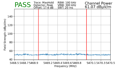
Plot 7-180. Radiated Lower Band Edge Plot MIMO (Peak – UNII Band 2C – 484+242 Tones)
