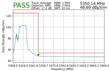
Plot 7-147. Radiated Upper Band Edge Plot MIMO (Average – UNII Band 2A – 106+26 Tones)
