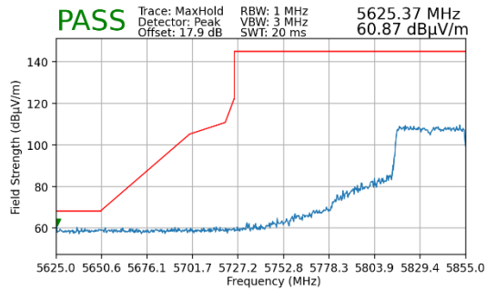
Plot 7-172. Radiated Lower Band Edge Plot MIMO (Peak – UNII Band 4 – 484 Tones)
