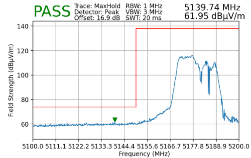
Plot 7-136. Radiated Lower Band Edge Plot MIMO (Peak – UNII Band 1 – 106 Tones)
