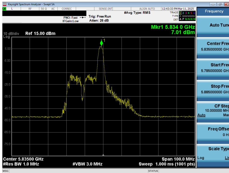
Plot 7-108. Power Spectral Density Plot MIMO ANT2 (40MHz 802.11ax/be (26 Tones) (UNII Band 3/4) – Ch. 167)
