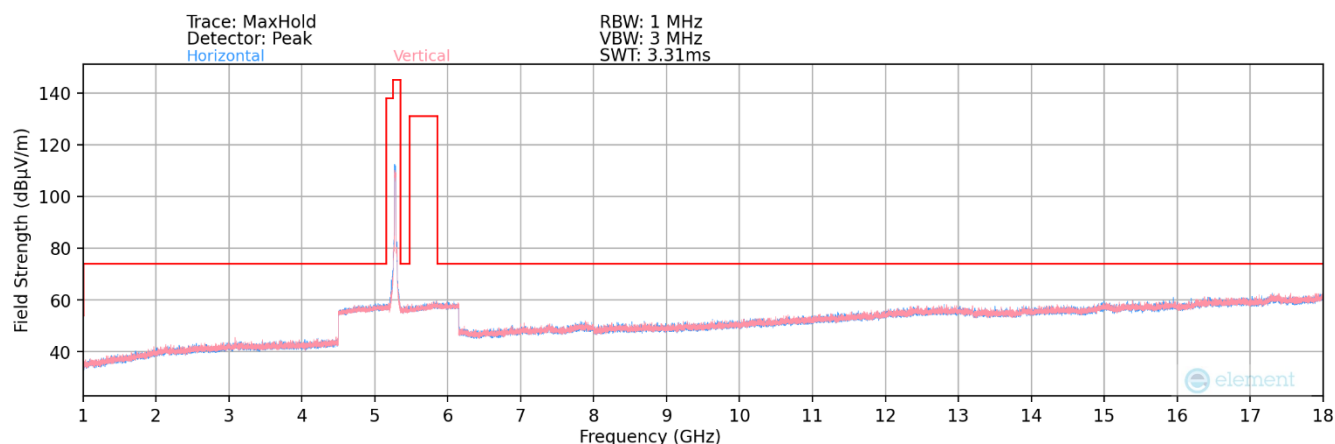
Plot 7-129. Radiated Spurious Plot above 1GHz MIMO (802.11ax – UNII 2A Ch. 56)
