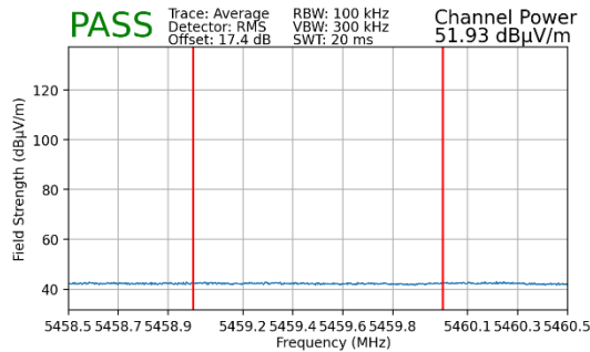
Plot 7-189. Radiated Lower Band Edge Plot MIMO (Average – UNII Band 2C – 996 Tones)
