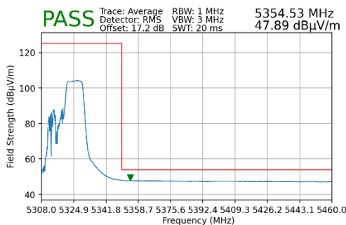
Plot 7-137. Radiated Upper Band Edge Plot MIMO (Average – UNII Band 2A – 106 Tones)
