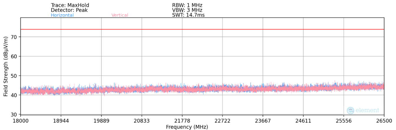
Plot 7-133. Radiated Spurious Plot 18GHz - 26.5GHz (802.11ax)
