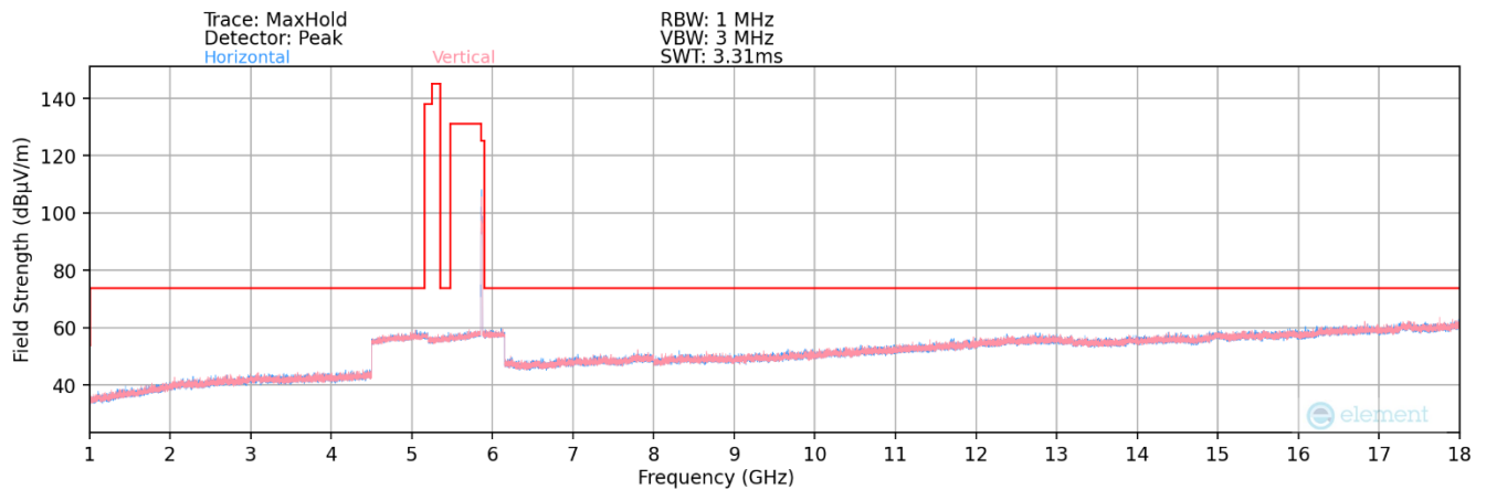
Plot 7-125. Radiated Spurious Plot above 1GHz MIMO (802.11ax – UNII 4 Ch. 173)
