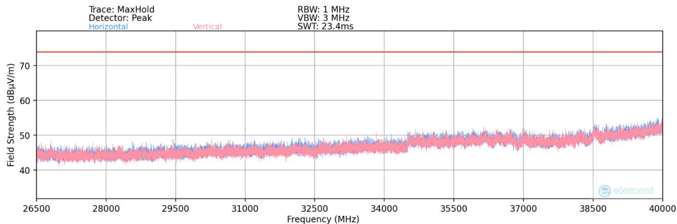
Plot 7-134. Radiated Spurious Plot 26.5GHz - 40GHz (802.11ax)
