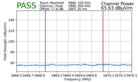
Plot 7-160. Radiated Lower Band Edge Plot MIMO (Peak – UNII Band 2C – 242 Tones)
