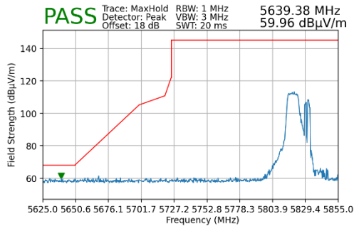
Plot 7-142. Radiated Lower Band Edge Plot MIMO (Peak – UNII Band 4 – 106 Tones)
