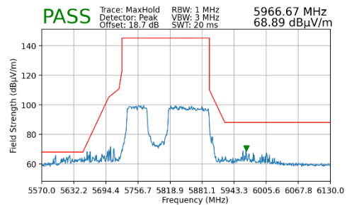
Plot 7-203. Radiated Upper Band Edge Plot MIMO (Peak – UNII Band 4 – 996+484 Tones)
