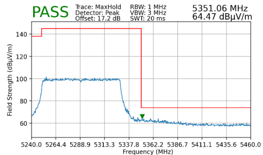
Plot 7-188. Radiated Upper Band Edge Plot MIMO (Peak – UNII Band 2A – 996 Tones)
