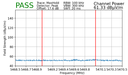
Plot 7-170. Radiated Lower Band Edge Plot MIMO (Peak – UNII Band 2C – 484 Tones)
