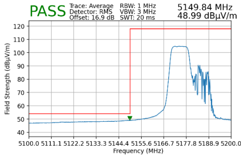
Plot 7-135. Radiated Lower Band Edge Plot MIMO (Average – UNII Band 1 – 106 Tones)
