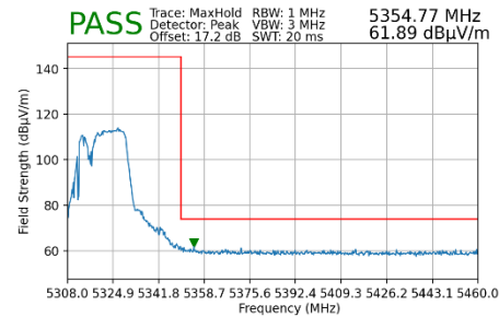
Plot 7-148. Radiated Upper Band Edge Plot MIMO (Peak – UNII Band 2A – 106+26 Tones)
