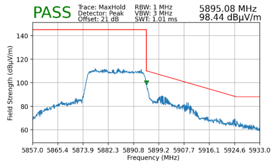
Plot 7-164. Radiated Upper Band Edge Plot MIMO (Peak – UNII Band 4 – 242 Tones)
