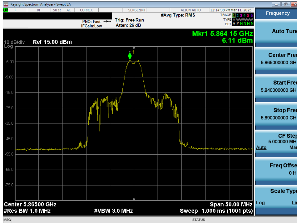
Plot 7-107. Power Spectral Density Plot MIMO ANT2 (20MHz 802.11ax/be (26 Tones) (UNII Band 4) – Ch. 173)
