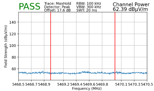
Plot 7-190. Radiated Lower Band Edge Plot MIMO (Peak – UNII Band 2C – 996 Tones)
