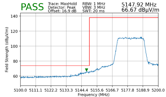
Plot 7-156. Radiated Lower Band Edge Plot MIMO (Peak – UNII Band 1 – 242 Tones)
