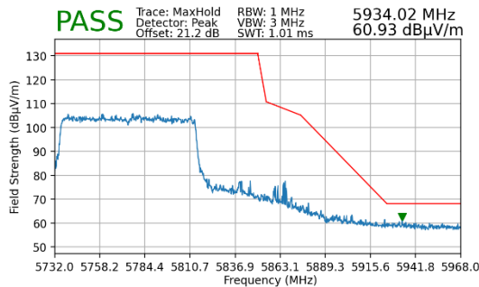
Plot 7-191. Radiated Upper Band Edge Plot MIMO (Peak – UNII Band 3 – 996 Tones)
