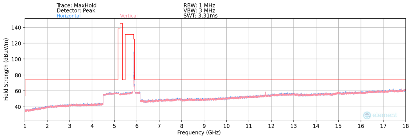
Plot 7-132. Radiated Spurious Plot above 1GHz MIMO (802.11ax – UNII 4 Ch. 173)
