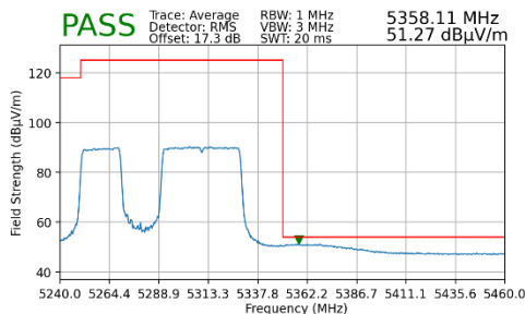
Plot 7-177. Radiated Upper Band Edge Plot MIMO (Average – UNII Band 2A – 484+242 Tones)
