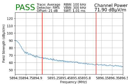
Plot 7-153. Radiated Upper Band Edge Plot MIMO (Average - UNII Band 4 - 106+26 Tones)
