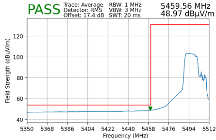
Plot 7-149. Radiated Lower Band Edge Plot MIMO (Average – UNII Band 2C – 106+26 Tones)
