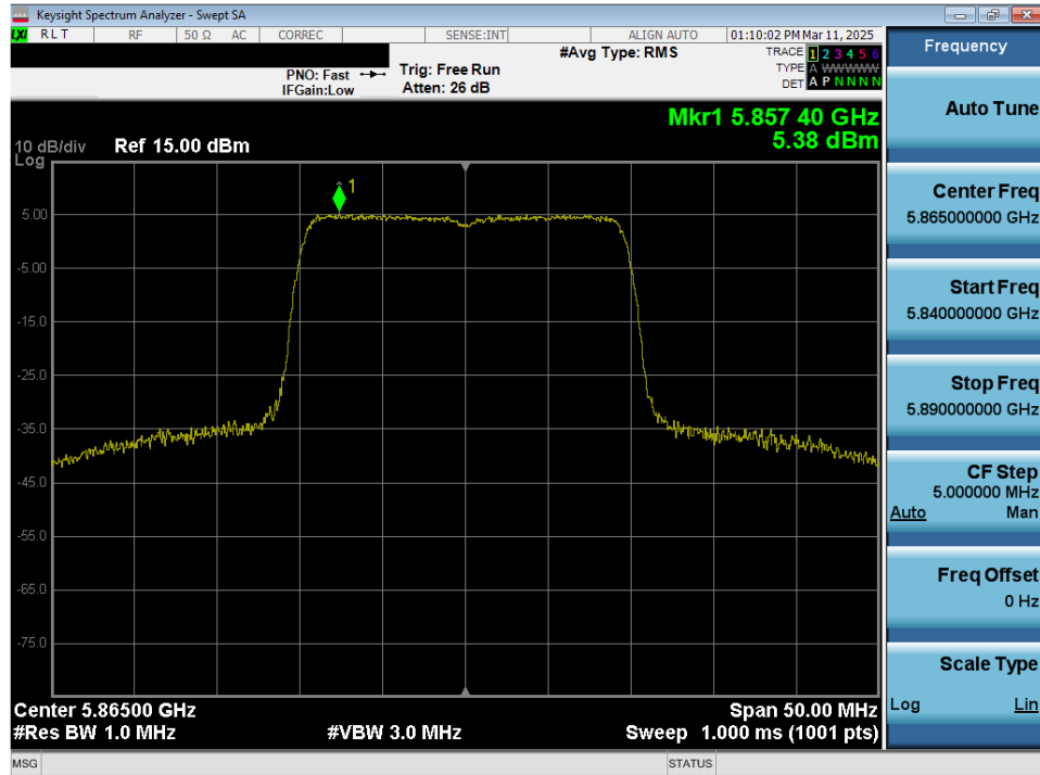
Plot 7-117. Power Spectral Density Plot MIMO ANT2 (20MHz 802.11ax/be (Full Tones) (UNII Band 4) – Ch. 173)
