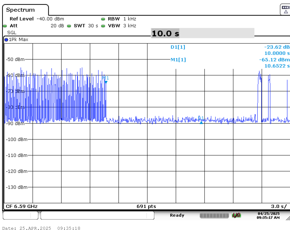
Plot 7-61. Contention Based Protocol Timing Plot (320MHz (UNII Band 7) – Ch. 159 Low)
