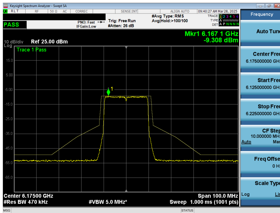
Plot 7-47. In Band Emissions Plot MIMO ANT2 (20MHz 802.11ax/be (UNII Band 5) – Ch. 45) - VLP
