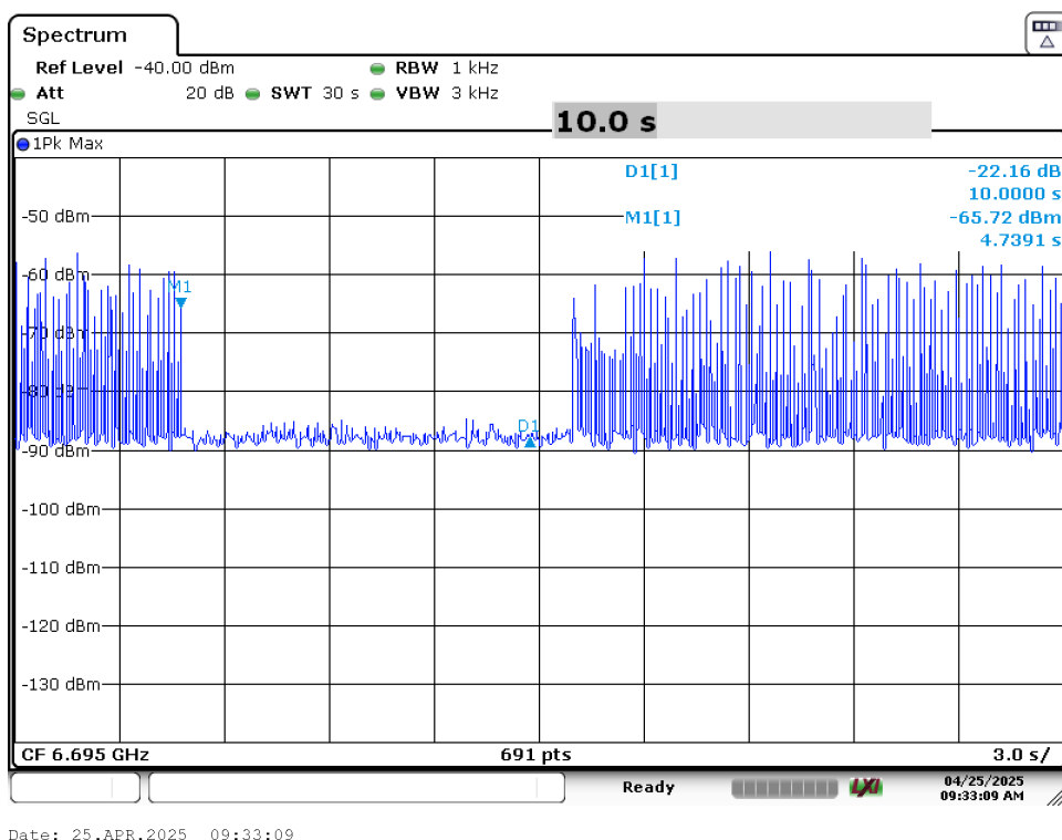
Plot 7-60. Contention Based Protocol Timing Plot (20MHz (UNII Band 7) – Ch. 149)
