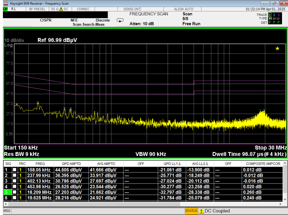
Plot 7-144. Line Conducted Plot with 802.11a UNII Band 8 (L1)
