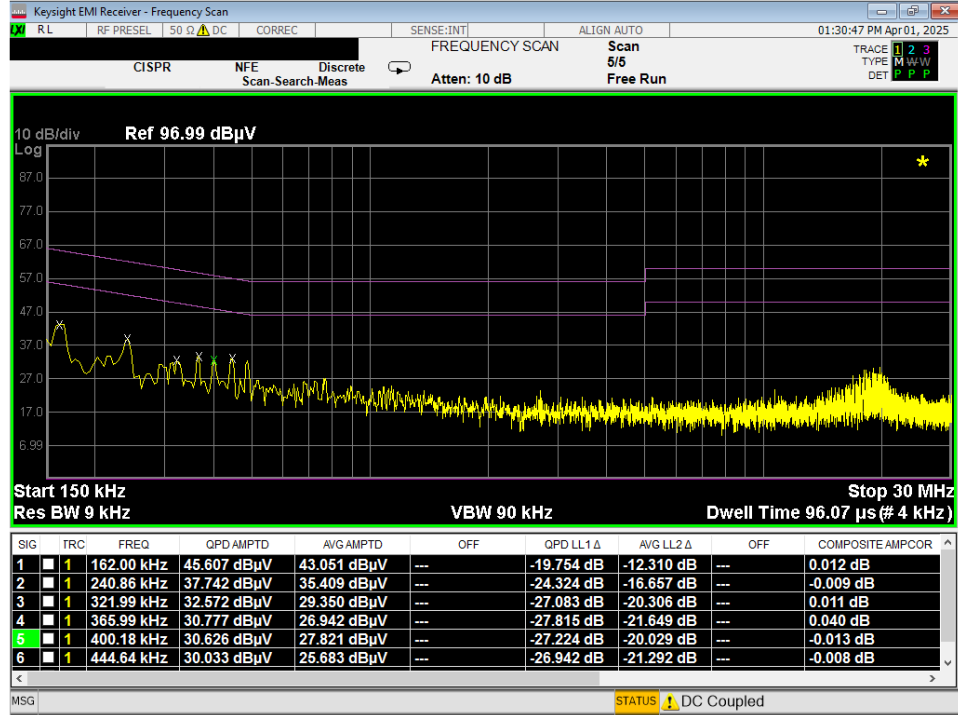
Plot 7-142. Line Conducted Plot with 802.11a UNII Band 7 (L1)
