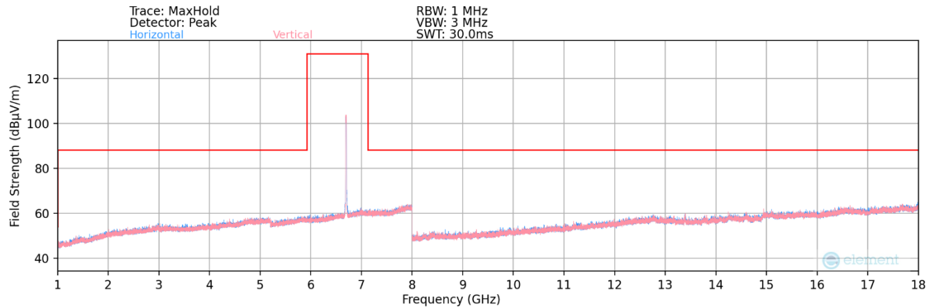
Plot 7-96. Radiated Spurious Plot 1GHz – 18GHz MIMO (802.11a – UNII Band 7 Ch. 149)
