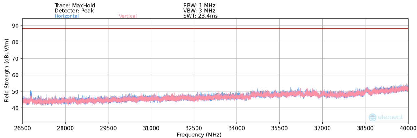
Plot 7-99. Radiated Spurious Plot 26.5GHz - 40GHz (802.11a) – Ch. 149
