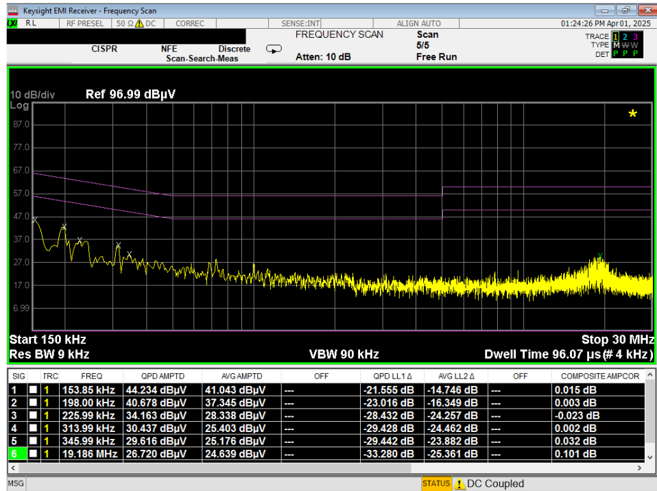
Plot 7-138. Line Conducted Plot with 802.11a UNII Band 5 (L1)
