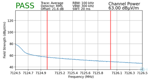
Plot 7-106. Radiated Upper Band Edge Plot MIMO (Average – UNII Band 8)
