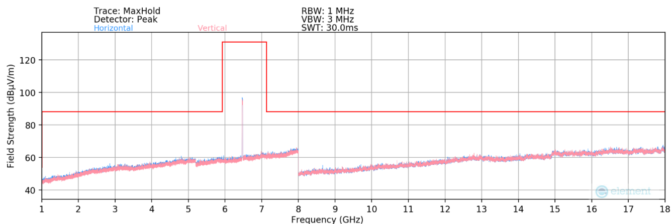
Plot 7-95. Radiated Spurious Plot 1GHz – 18GHz MIMO (802.11a – UNII Band 6 Ch. 105)
