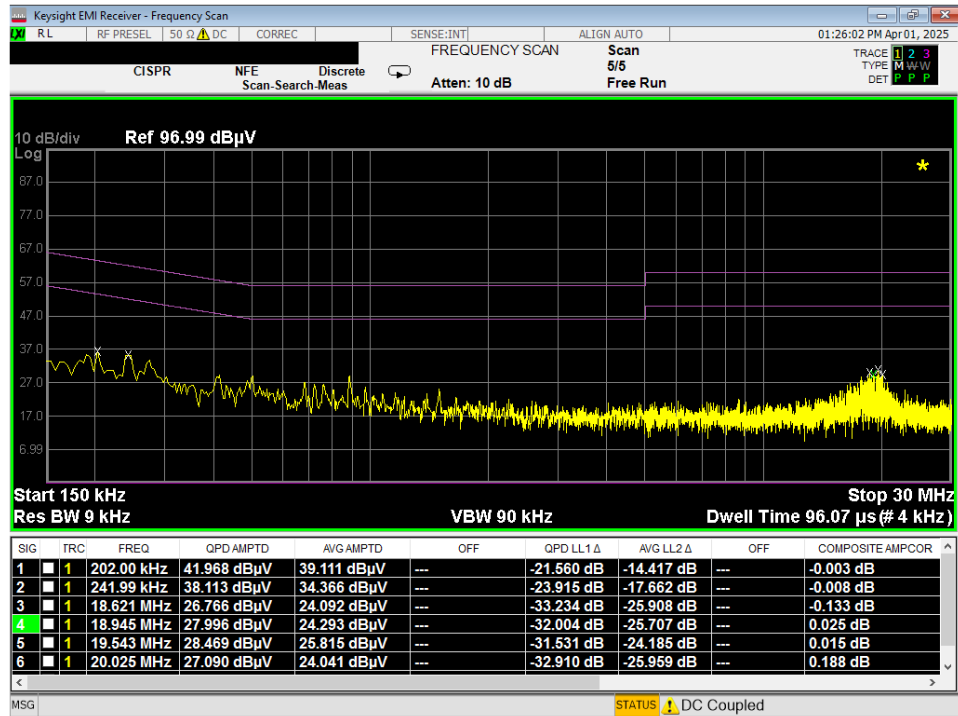
Plot 7-140. Line Conducted Plot with 802.11a UNII Band 6 (L1)
