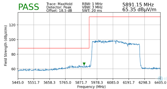
Plot 7-131. Radiated Lower Band Edge Plot MIMO (Peak – UNII Band 5)
