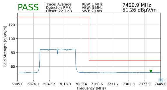
Plot 7-124. Radiated Upper Band Edge Plot MIMO (Average – UNII Band 8)
