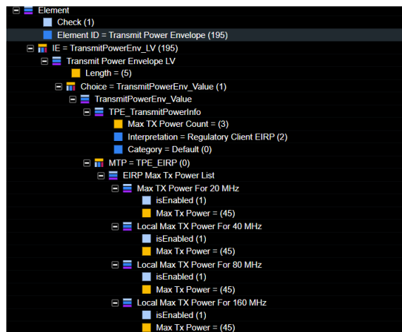
Figure 7-8. Callbox Power Authorization – 22.50dBm
