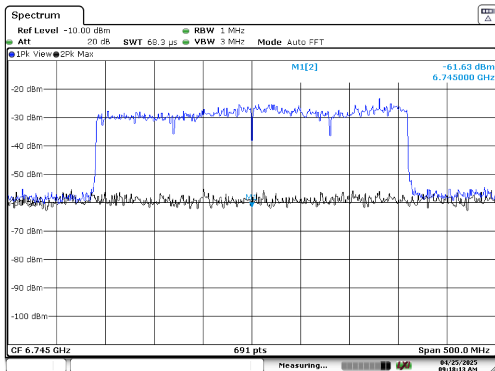
Plot 7-91. CBP 320MHz Channel - Injection Center – [6745 MHz]
