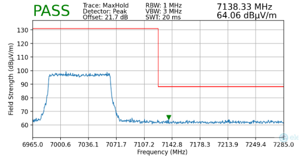
Plot 7-117. Radiated Upper Band Edge Plot MIMO (Peak – UNII Band 8)
