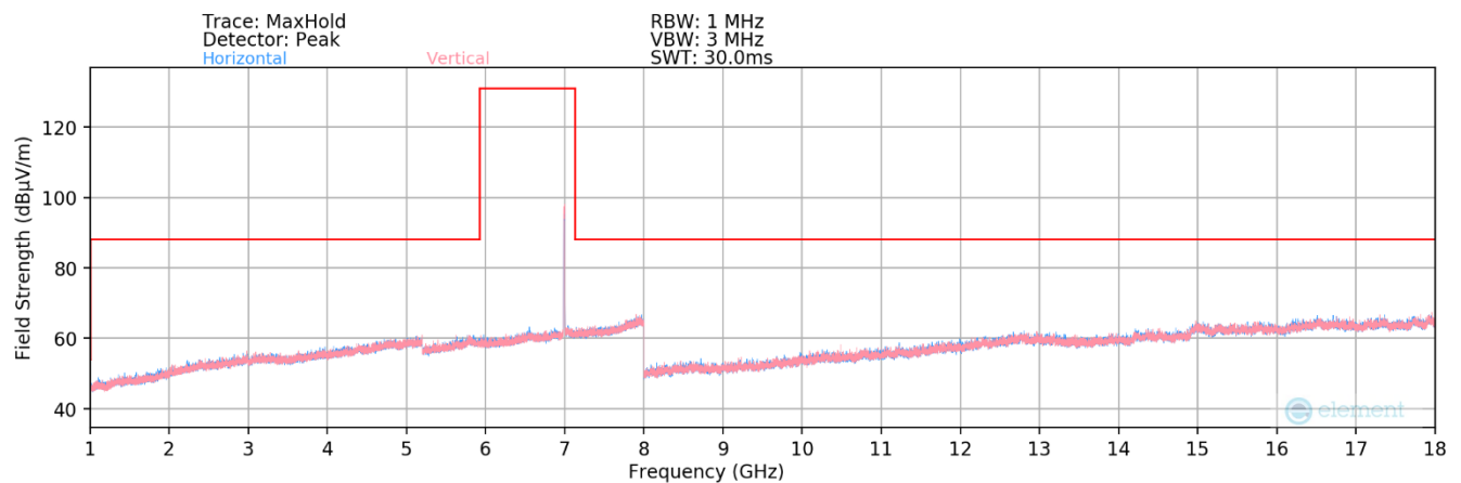
Plot 7-97. Radiated Spurious Plot 1GHz – 18GHz MIMO (802.11a – U Band 8 Ch. 209)
