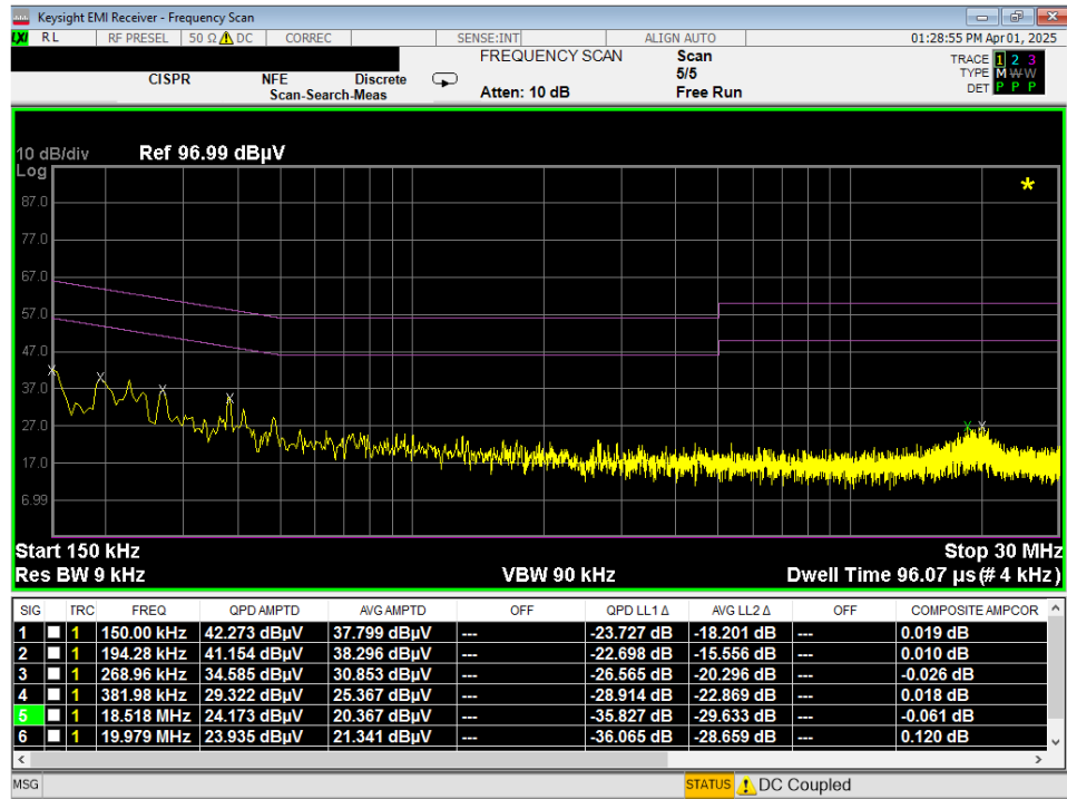
Plot 7-143. Line Conducted Plot with 802.11a UNII Band 7 (N)
