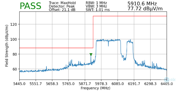
Plot 7-135. Radiated Lower Band Edge Plot MIMO (Peak – UNII Band 5)
