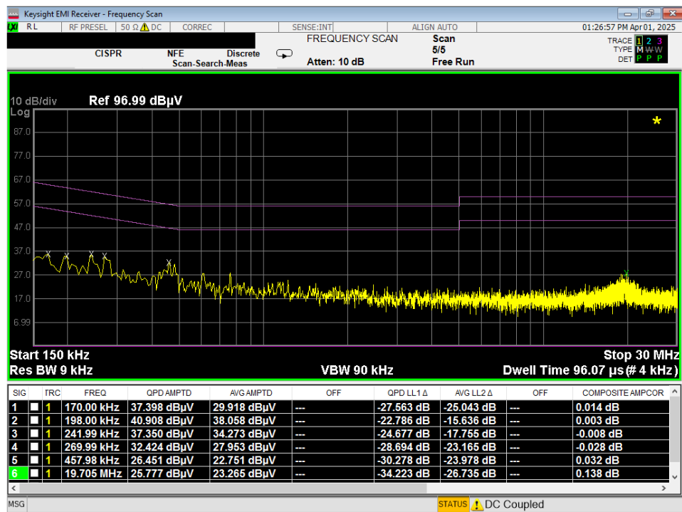
Plot 7-141. Line Conducted Plot with 802.11a UNII Band 6 (N)
