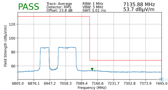
Plot 7-128. Radiated Upper Band Edge Plot MIMO (Average – UNII Band 8)
