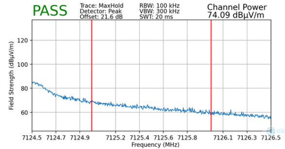
Plot 7-107. Radiated Upper Band Edge Plot MIMO (Peak – UNII Band 8)
