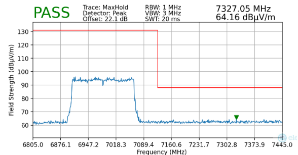
Plot 7-125. Radiated Upper Band Edge Plot MIMO (Peak – UNII Band 8)
