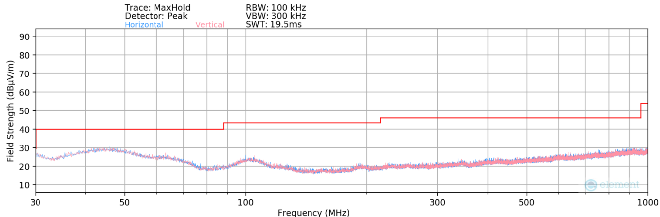
Plot 7-93. Radiated Spurious Plot below 1GHz MIMO (802.11a)
