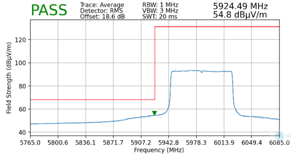
Plot 7-114. Radiated Lower Band Edge Plot MIMO (Average – UNII Band 5)
