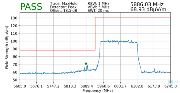
Plot 7-123. Radiated Lower Band Edge Plot MIMO (Peak – UNII Band 5)
