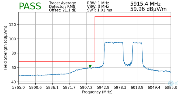
Plot 7-118. Radiated Lower Band Edge Plot MIMO (Average – UNII Band 5)
