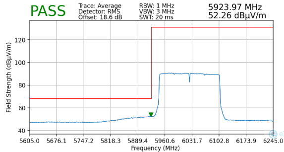
Plot 7-122. Radiated Lower Band Edge Plot MIMO (Average – UNII Band 5)
