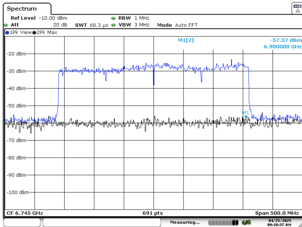
Plot 7-92. CBP 320MHz Channel - Injection Upper Edge – [6900 MHz]
