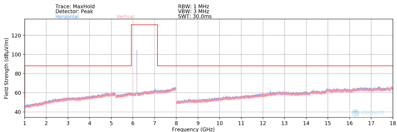
Plot 7-94. Radiated Spurious Plot 1GHz – 18GHz MIMO (802.11a – UNII Band 5 Ch. 45)
