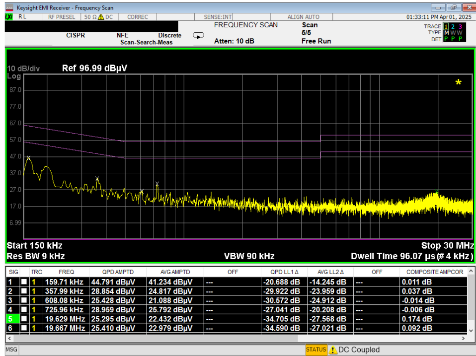
Plot 7-145. Line Conducted Plot with 802.11a UNII Band 8 (N)
