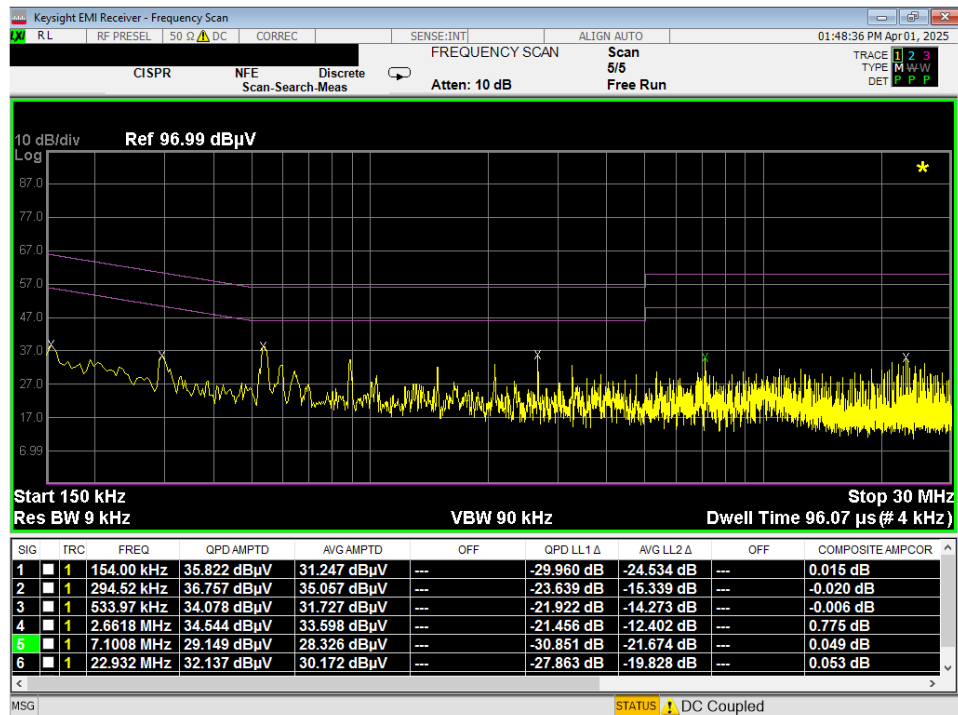
Plot 7-147. Line Conducted Plot with 802.11a UNII Band 5 (N) with WCP
