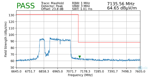
Plot 7-137. Radiated Upper Band Edge Plot MIMO (Peak – UNII Band 8)
