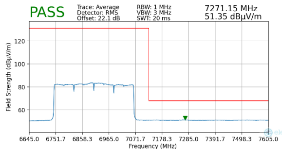
Plot 7-132. Radiated Upper Band Edge Plot MIMO (Average – UNII Band 8)
