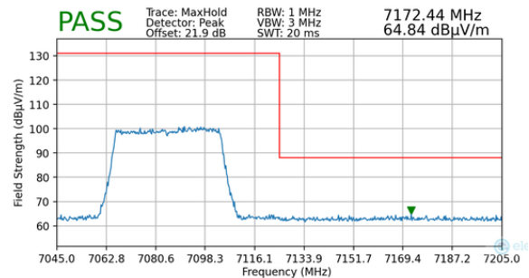
Plot 7-113. Radiated Upper Band Edge Plot MIMO (Peak – UNII Band 8)
