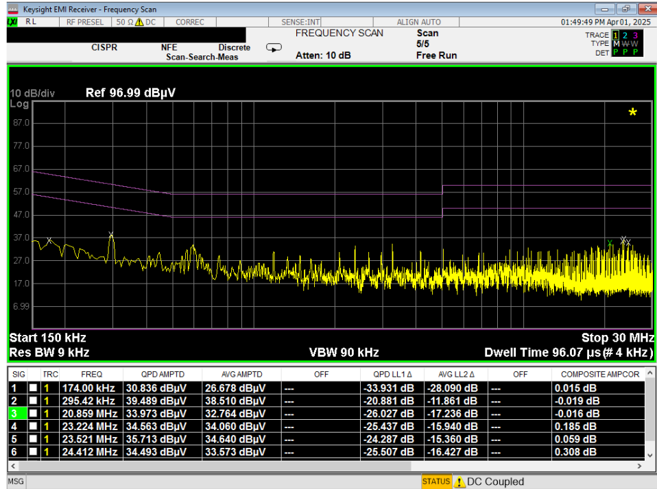
Plot 7-146. Line Conducted Plot with 802.11a UNII Band 5 (L1) with WCP
