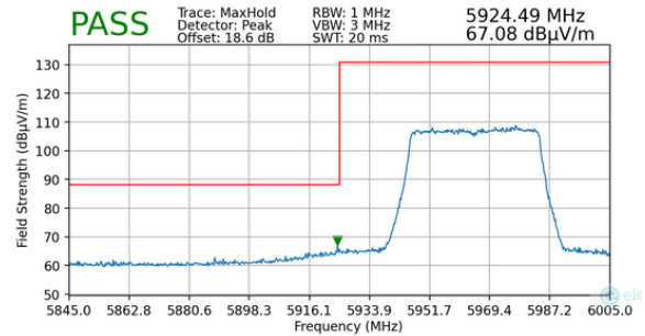
Plot 7-111. Radiated Lower Band Edge Plot MIMO (Peak – UNII Band 5)
