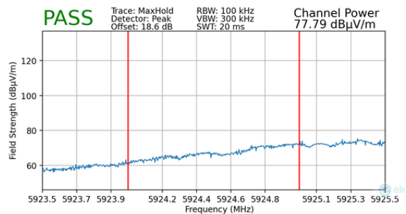
Plot 7-109. Radiated Lower Band Edge Plot MIMO (Peak – UNII Band 5) with WCP
