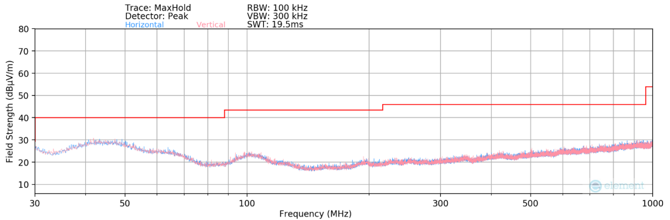
Plot 7-100. Radiated Spurious Plot below 1GHz MIMO 802.11b (2.4GHz – Ch.6) + MIMO 802.11a (6GHz – Ch.1)
