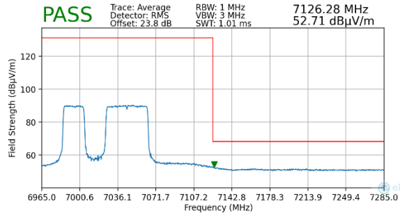
Plot 7-120. Radiated Upper Band Edge Plot MIMO (Average – UNII Band 8)
