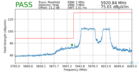
Plot 7-119. Radiated Lower Band Edge Plot MIMO (Peak – UNII Band 5)
