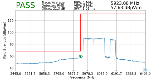
Plot 7-134. Radiated Lower Band Edge Plot MIMO (Average – UNII Band 5)
