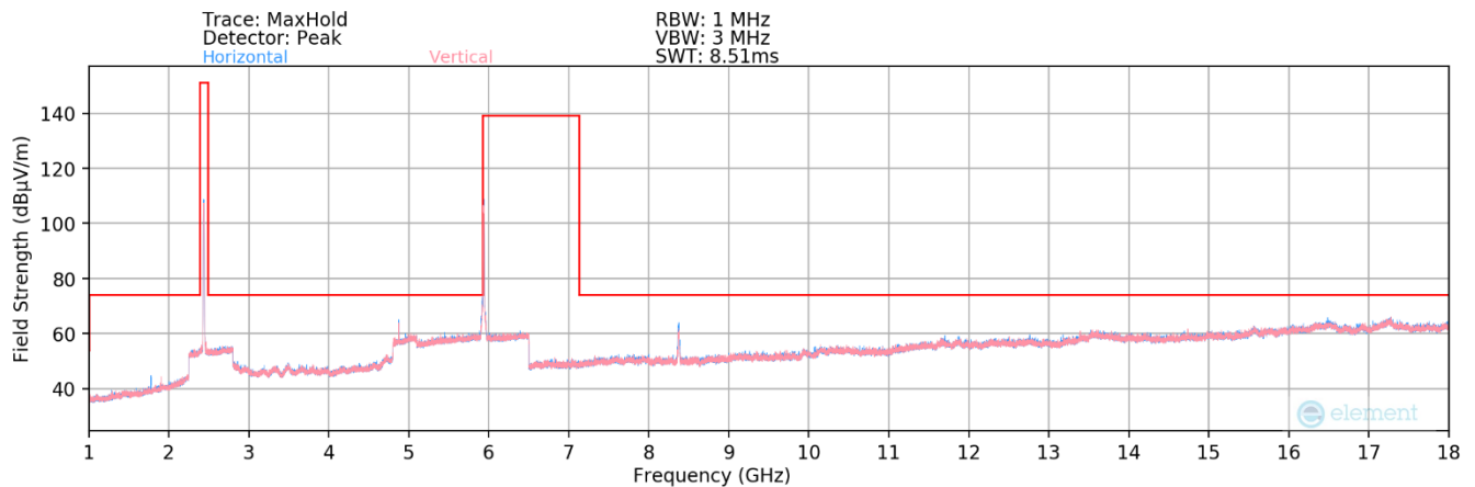
Plot 7-101. Radiated Spurious Plot above 1GHz MIMO 802.11b (2.4GHz – Ch.6) + MIMO 802.11a (6GHz – Ch.1)
