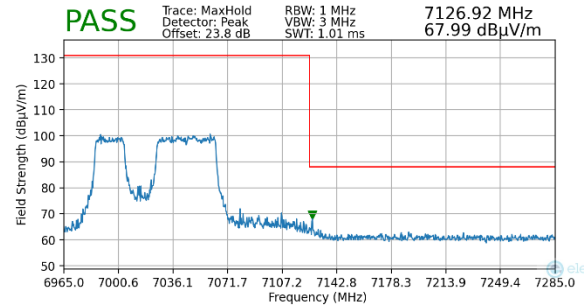
Plot 7-121. Radiated Upper Band Edge Plot MIMO (Peak – UNII Band 8)
