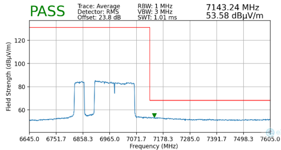
Plot 7-136. Radiated Upper Band Edge Plot MIMO (Average – UNII Band 8)
