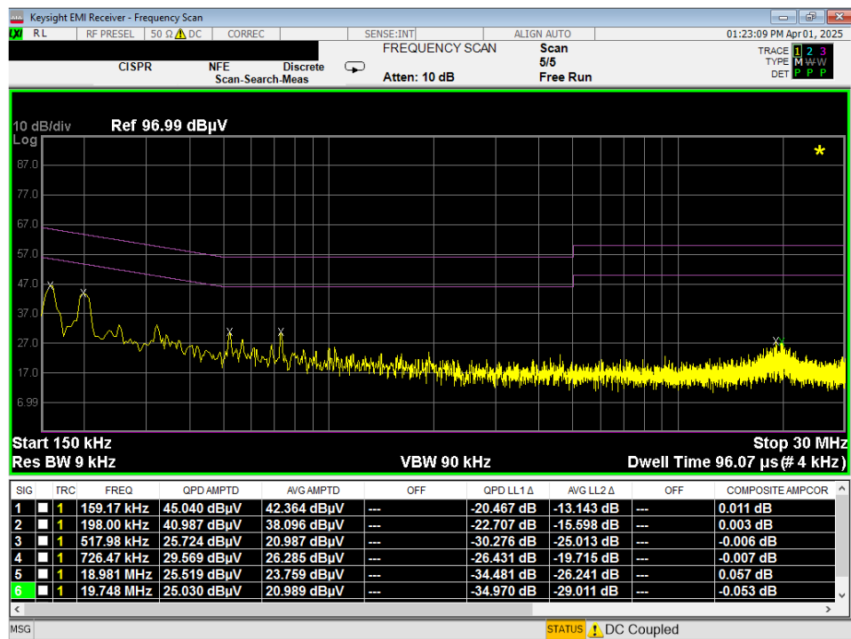
Plot 7-139. Line Conducted Plot with 802.11a UNII Band 5 (N)
