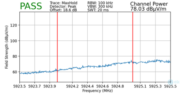
Plot 7-105. Radiated Lower Band Edge Plot MIMO (Peak – UNII Band 5)
