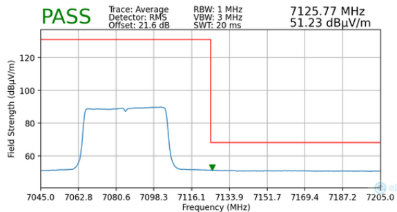
Plot 7-112. Radiated Upper Band Edge Plot MIMO (Average – UNII Band 8)
