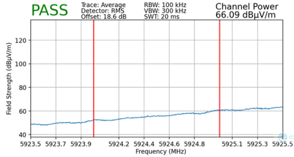
Plot 7-104. Radiated Lower Band Edge Plot MIMO (Average – UNII Band 5)
