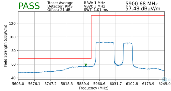
Plot 7-126. Radiated Lower Band Edge Plot MIMO (Average – UNII Band 5)
