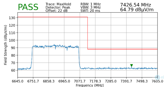
Plot 7-133. Radiated Upper Band Edge Plot MIMO (Peak – UNII Band 8)
