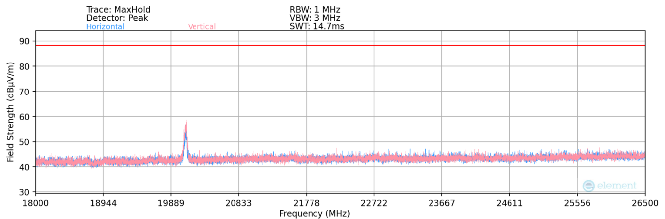
Plot 7-98. Radiated Spurious Plot 18GHz - 26.5GHz (802.11a) – Ch. 149
