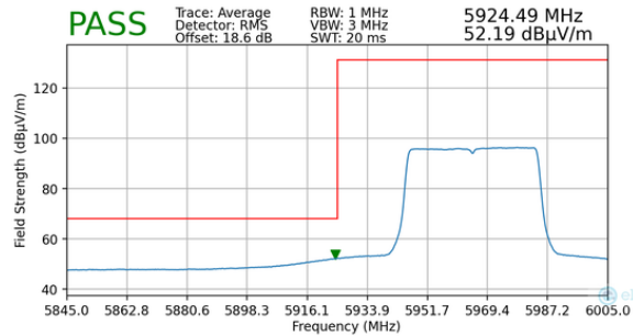
Plot 7-110. Radiated Lower Band Edge Plot MIMO (Average – UNII Band 5)
