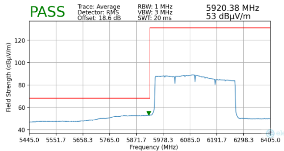
Plot 7-130. Radiated Lower Band Edge Plot MIMO (Average – UNII Band 5)
