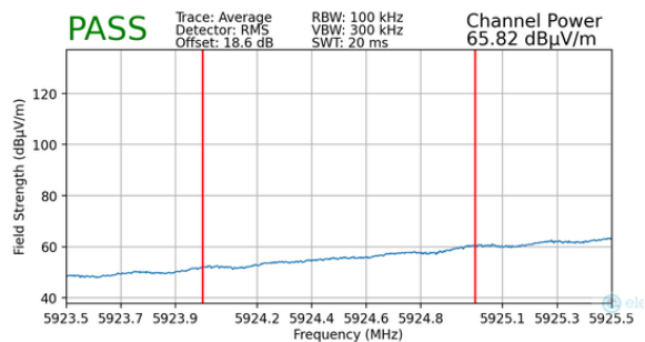
Plot 7-108. Radiated Lower Band Edge Plot MIMO (Average – UNII Band 5) with WCP
