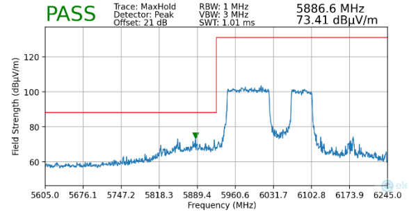
Plot 7-127. Radiated Lower Band Edge Plot MIMO (Peak – UNII Band 5)
