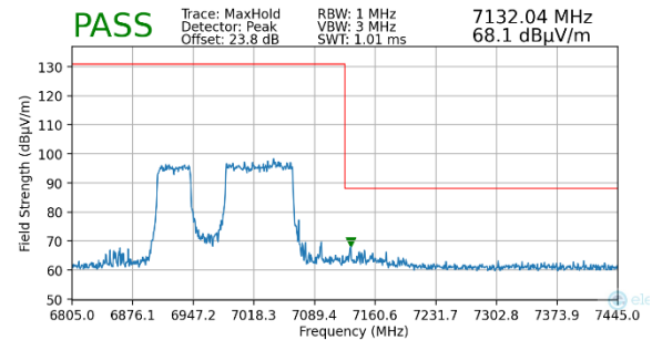
Plot 7-129. Radiated Upper Band Edge Plot MIMO (Peak – UNII Band 8)
