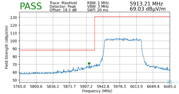
Plot 7-115. Radiated Lower Band Edge Plot MIMO (Peak – UNII Band 5)
