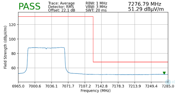
Plot 7-116. Radiated Upper Band Edge Plot MIMO (Average – UNII Band 8)
