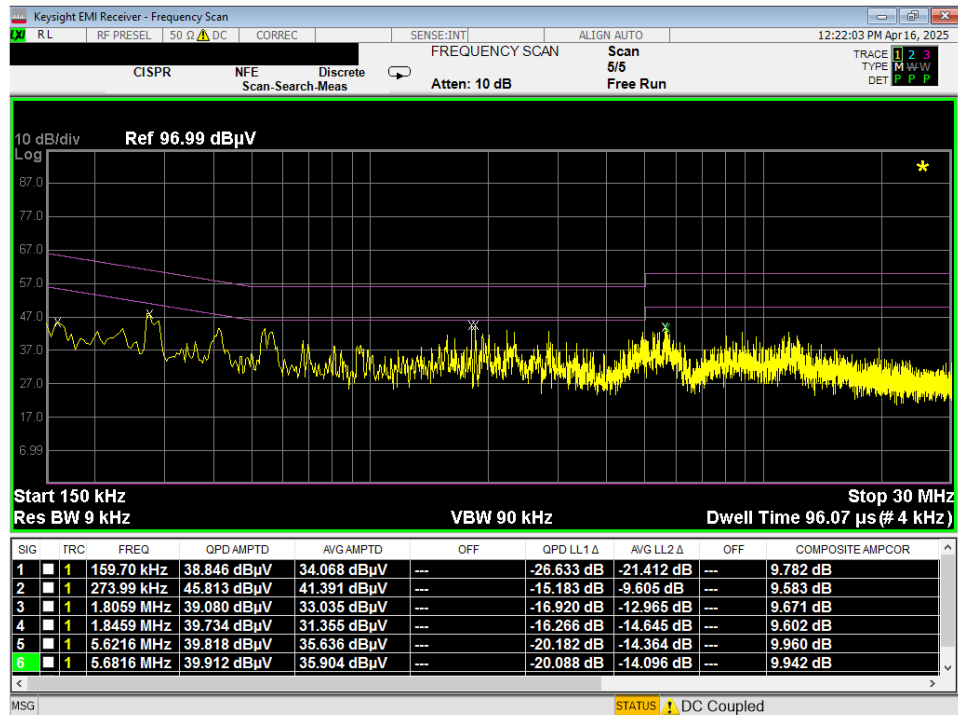
Plot 7-6. Line-Conducted Test Plot (L1) – Device to Device
