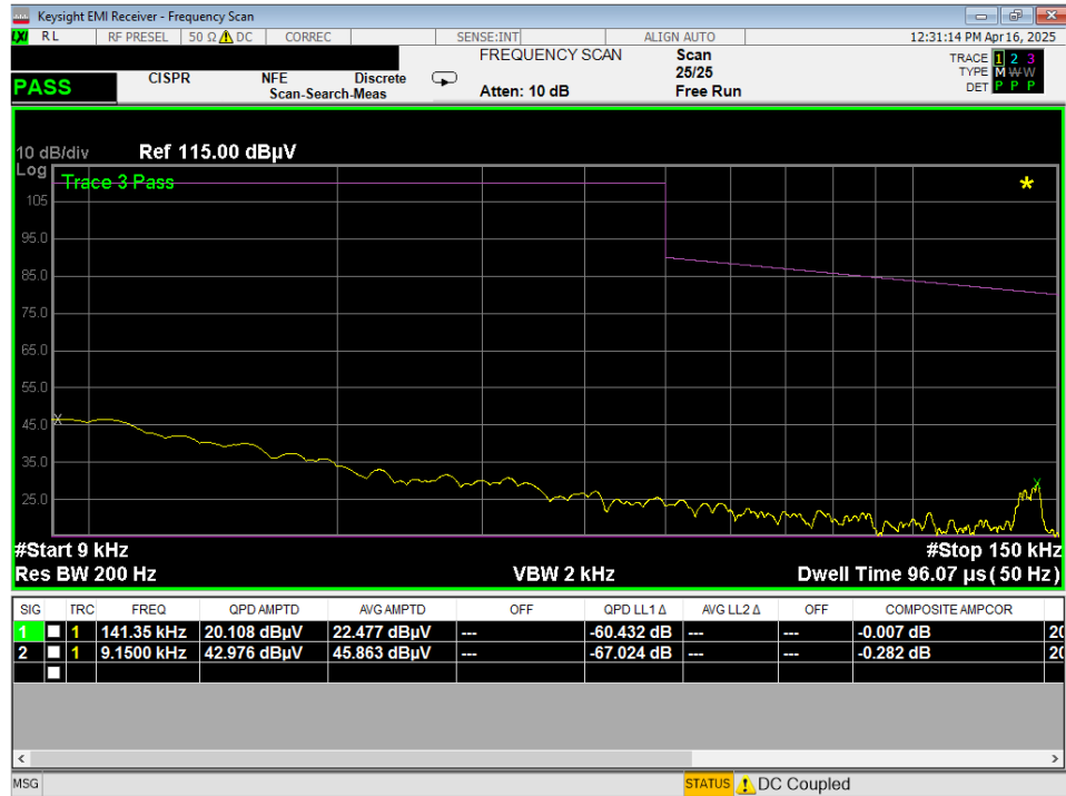
Plot 7-7. Line-Conducted Test Plot (N) – Device to Device
