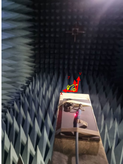
Figure 1: Geometry for SM-F966U for Radiation patterns.
