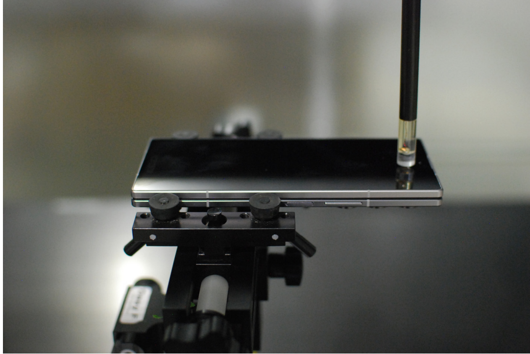
Figure 18-1 Test Setup for Wireless Device
