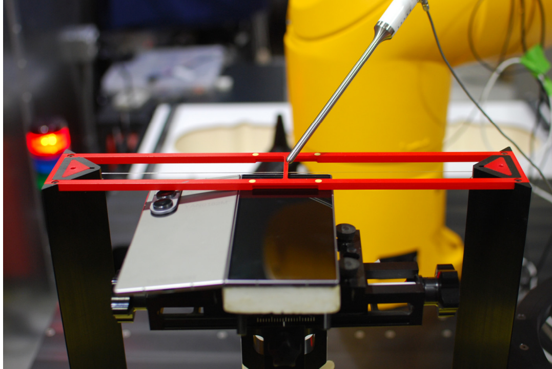
Figure 18-7 Test Setup for Wireless Device
