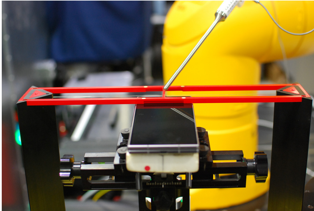
Figure 18-3 Test Setup for Wireless Device
