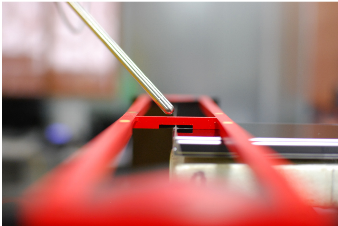
Figure 18-4 Test Setup for Wireless Device
