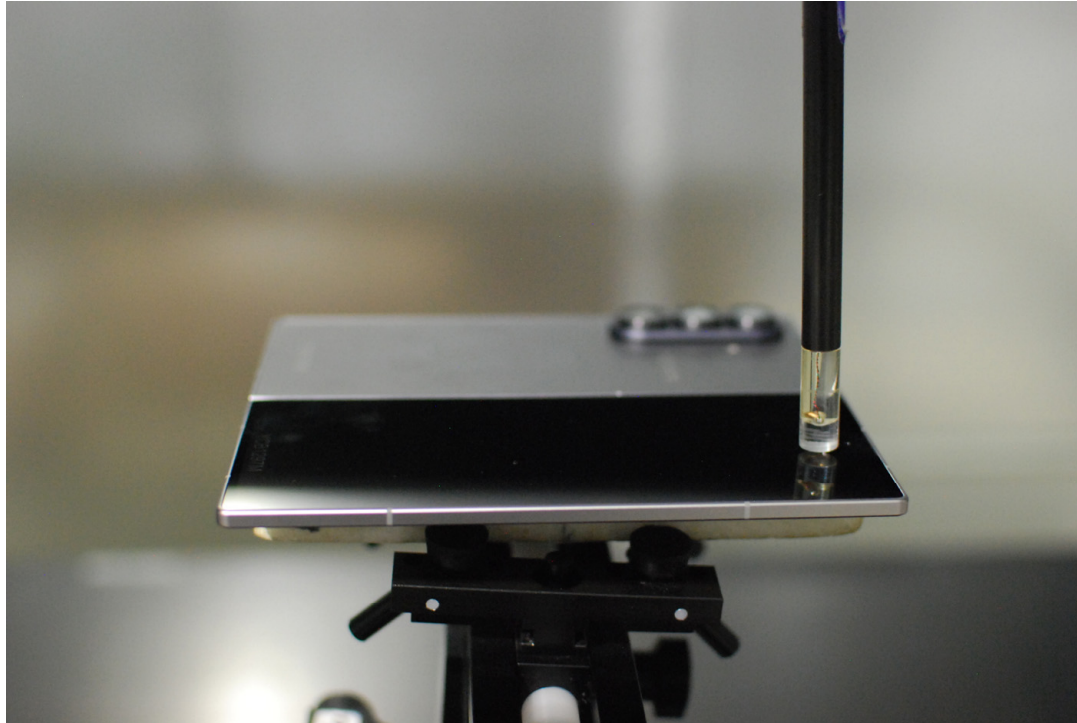
Figure 18-5 Test Setup for Wireless Device
