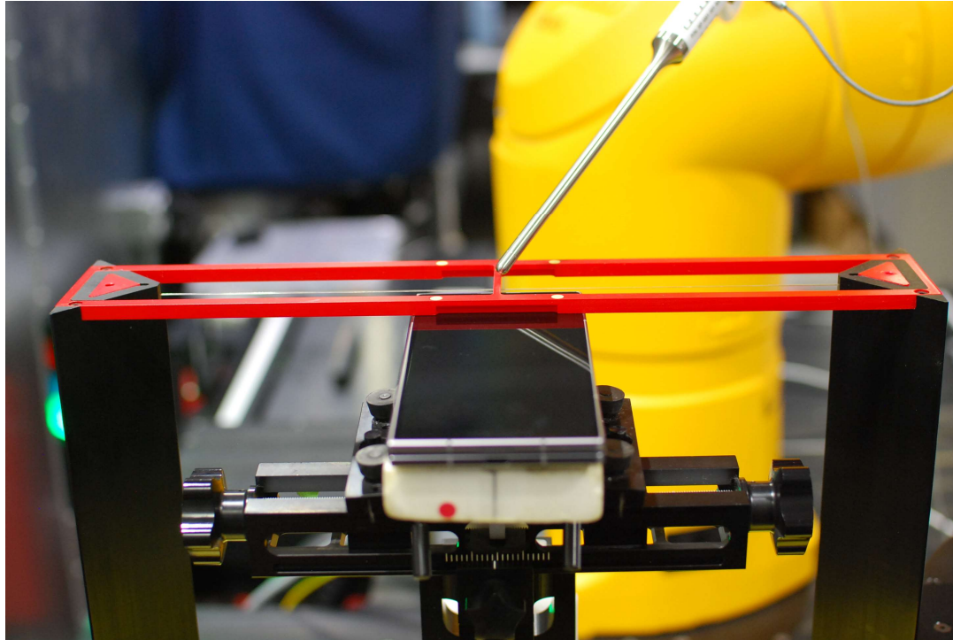
Figure 16-3 Test Setup for Wireless Device
