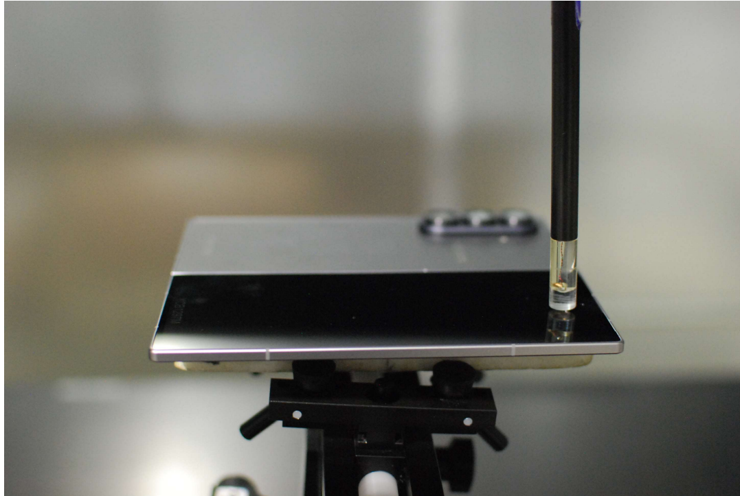
Figure 16-5 Test Setup for Wireless Device
