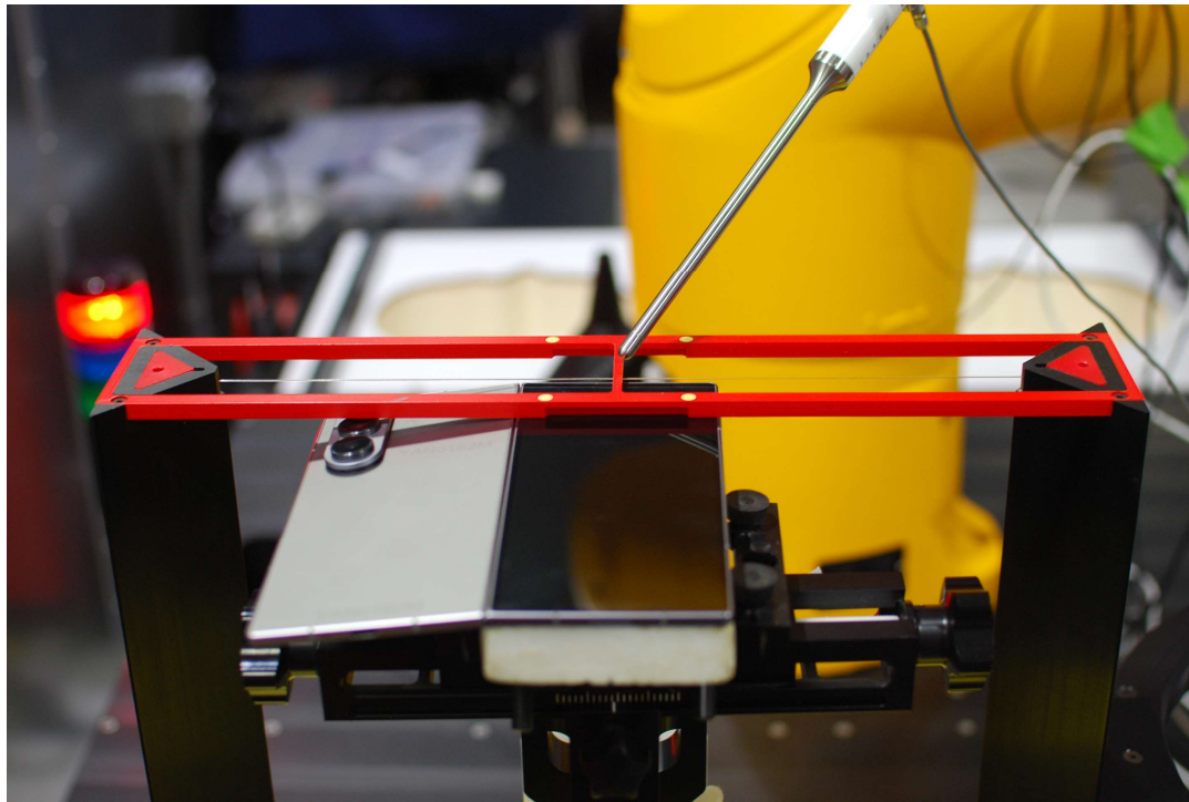
Figure 16-7 Test Setup for Wireless Device
