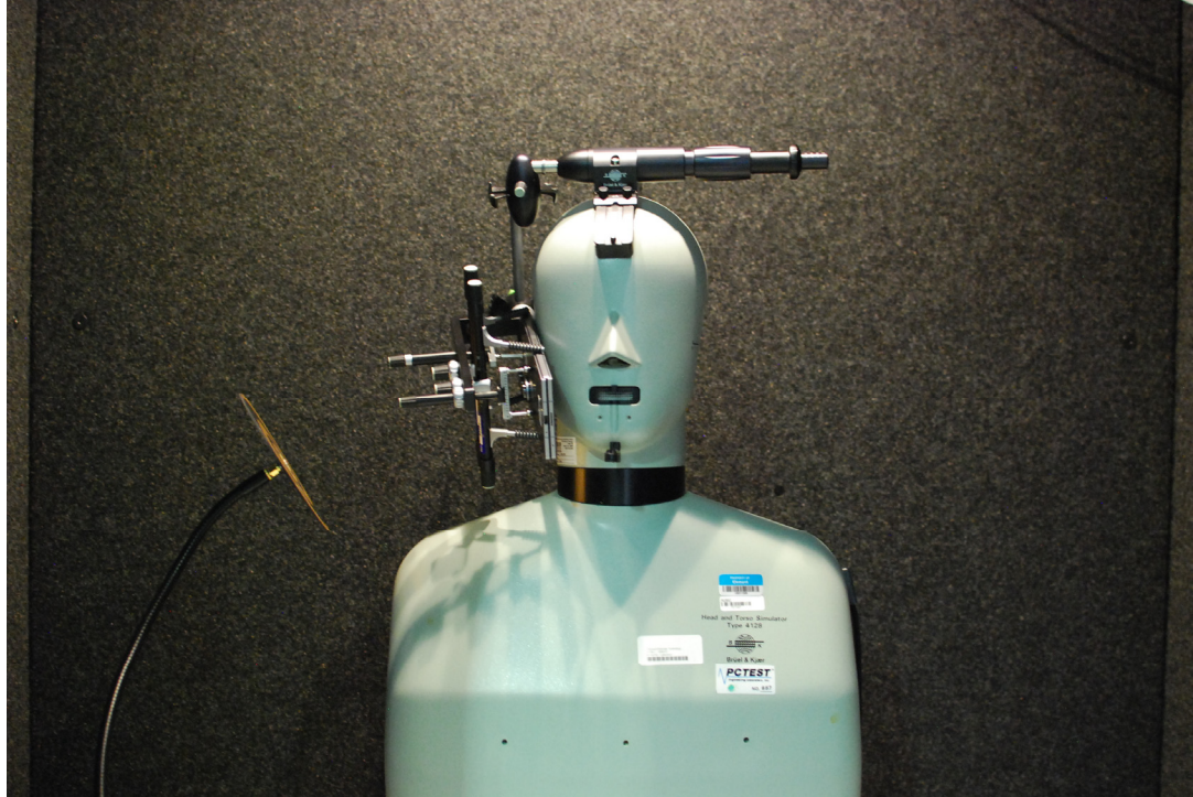
Figure 17-1 Test Setup for Wireless Device – Folder Closed
