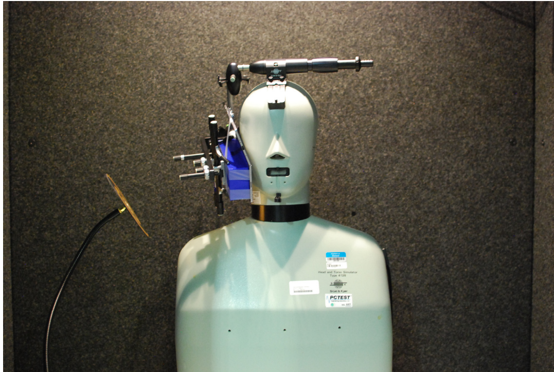
Figure 17-3 Test Setup for Wireless Device – Folder Open
