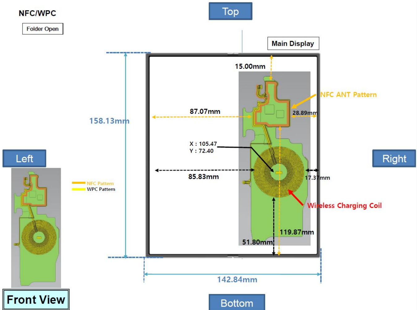
Figure H-4 NFC Antenna Locations – Folder Open
