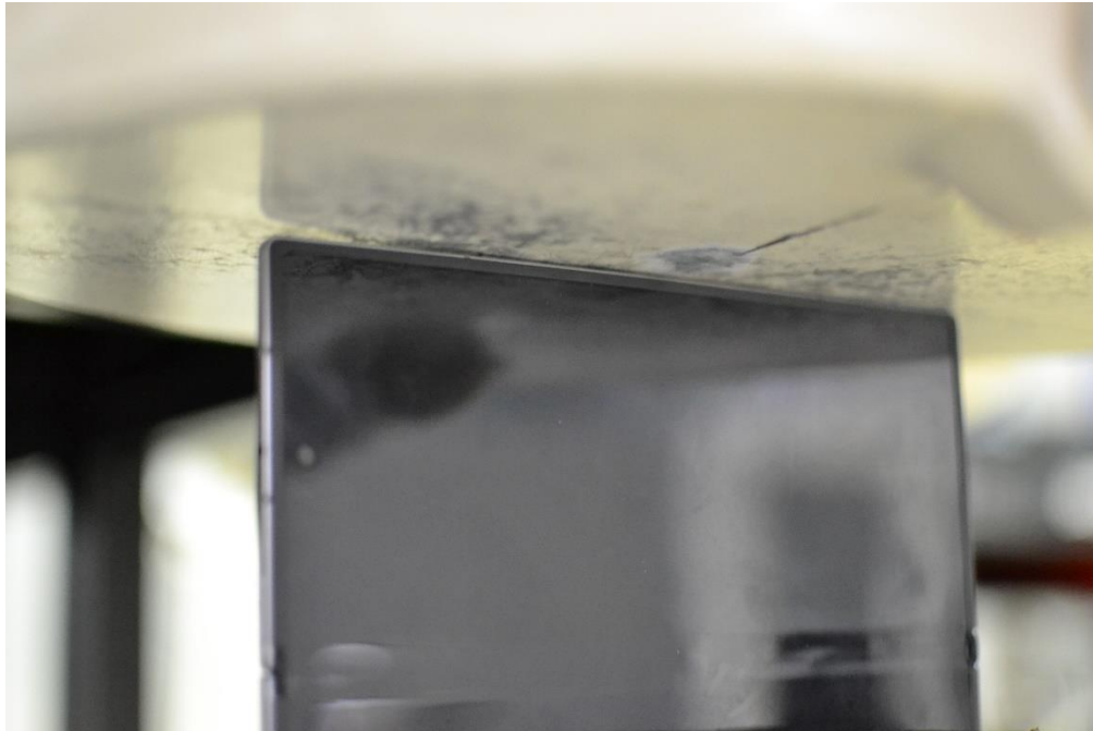
SAR Test Setup Photo 27 – Tablet, Folder Open, Right Edge at 0mm
