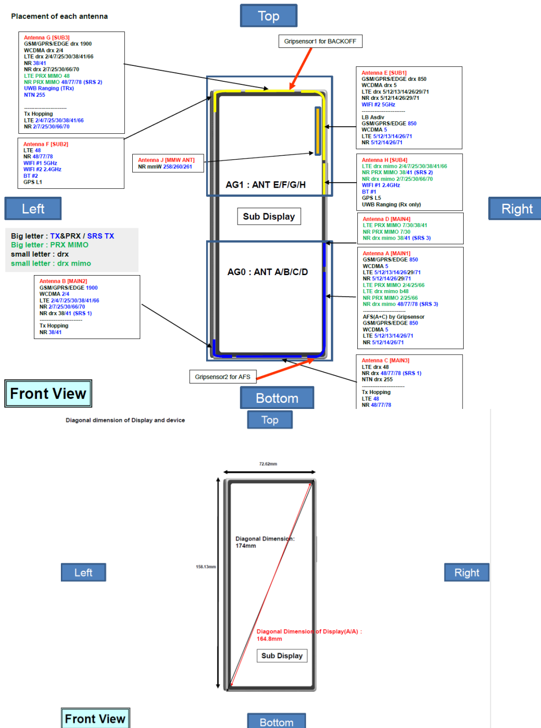
Figure H-1 DUT Antenna Locations – Folder Closed
