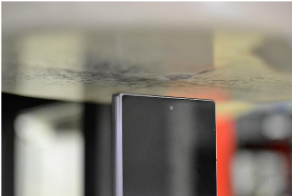
SAR Test Setup Photo 15 – Hotspot, Folder Closed, Top Edge at 10mm
