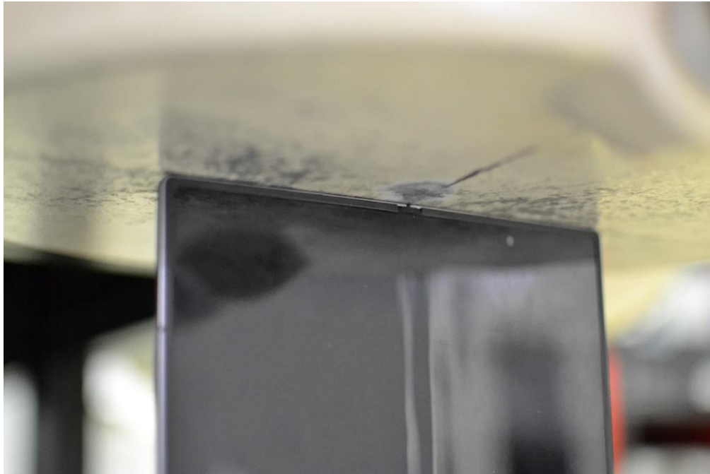
SAR Test Setup Photo 25 – Tablet, Folder Open, Top Edge at 0mm
