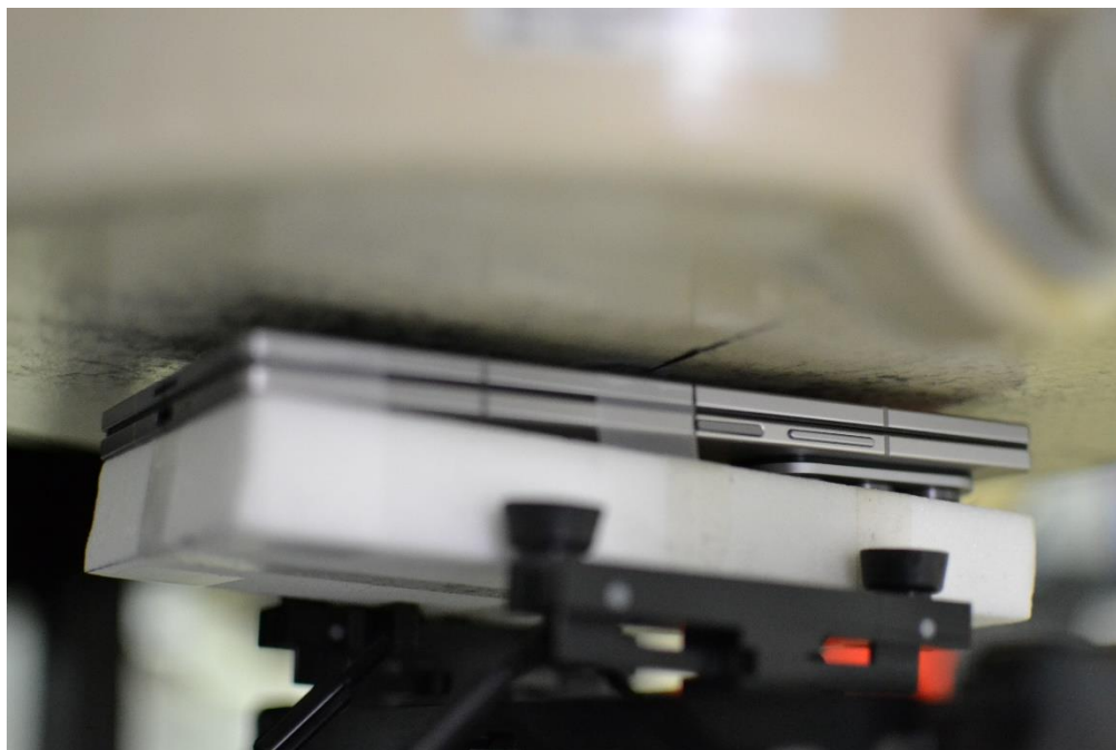
SAR Test Setup Photo 11 – Body-worn/Hotspot, Folder Closed, Front Side at 5mm
