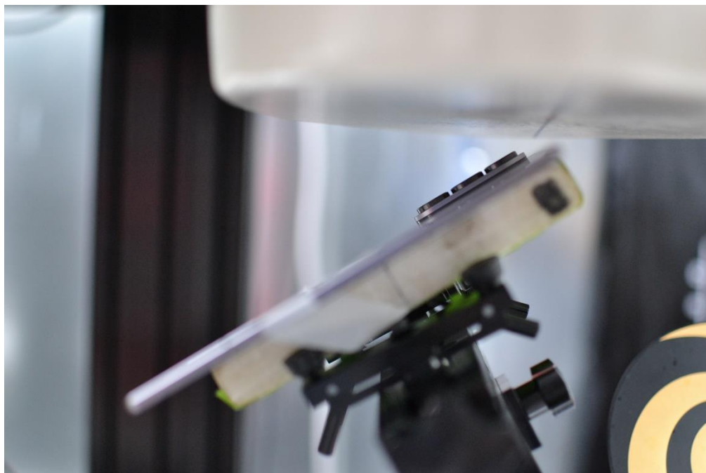
SAR Test Setup Photo 21 – Tablet, Folder Open, Back Side at 10mm (for AG1)
