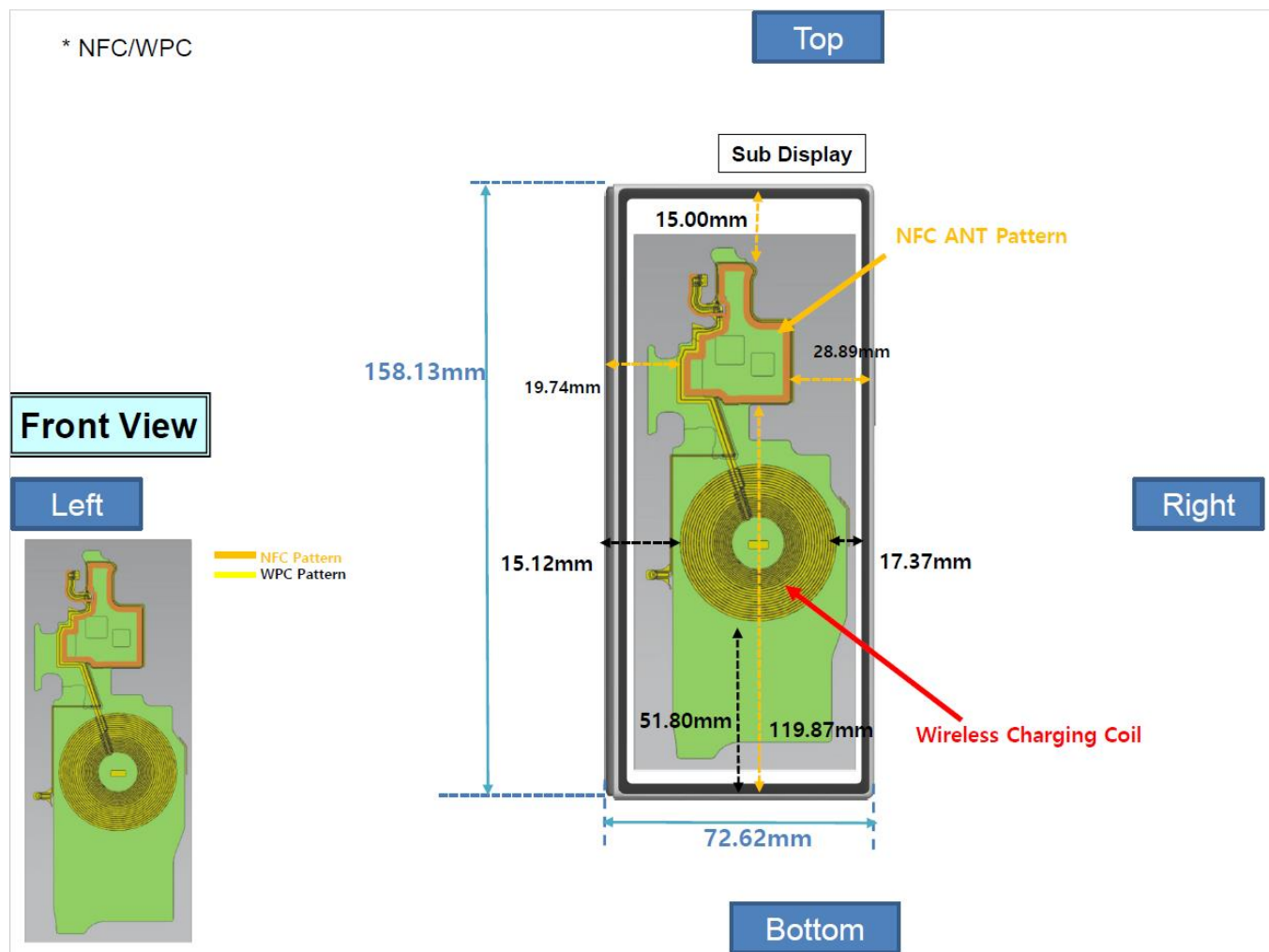
Figure H-3 NFC Antenna Locations – Folder Closed
