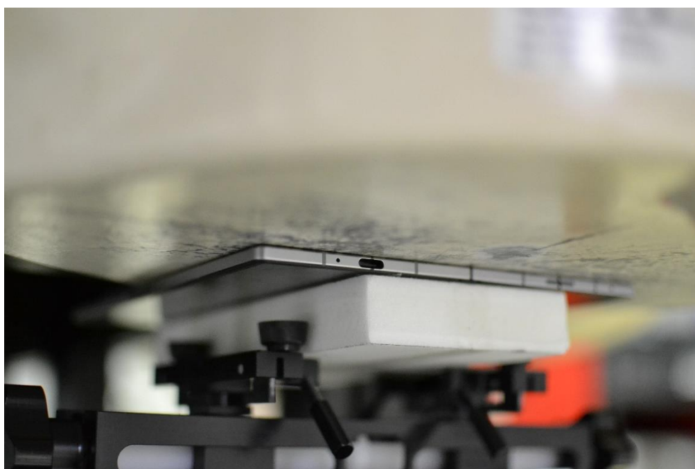
SAR Test Setup Photo 20 – Tablet, Folder Open, Back Side at 0mm (for AG0)
