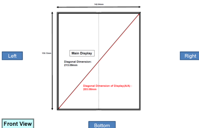
Figure H-2 DUT Antenna Locations – Folder Open
