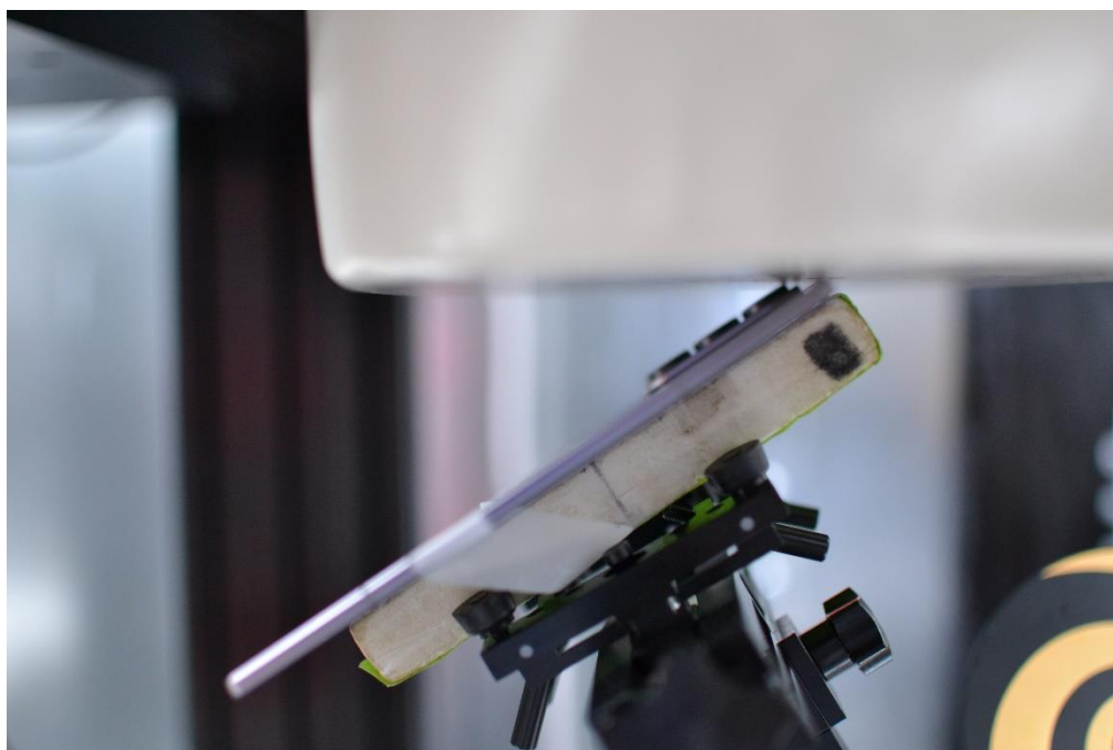
SAR Test Setup Photo 22 – Tablet, Folder Open, Back Side at 0mm (for AG1)
