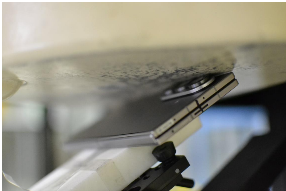
SAR Test Setup Photo 11 – Phablet, Folder Closed, Back Side at 0mm (for Antenna H)
