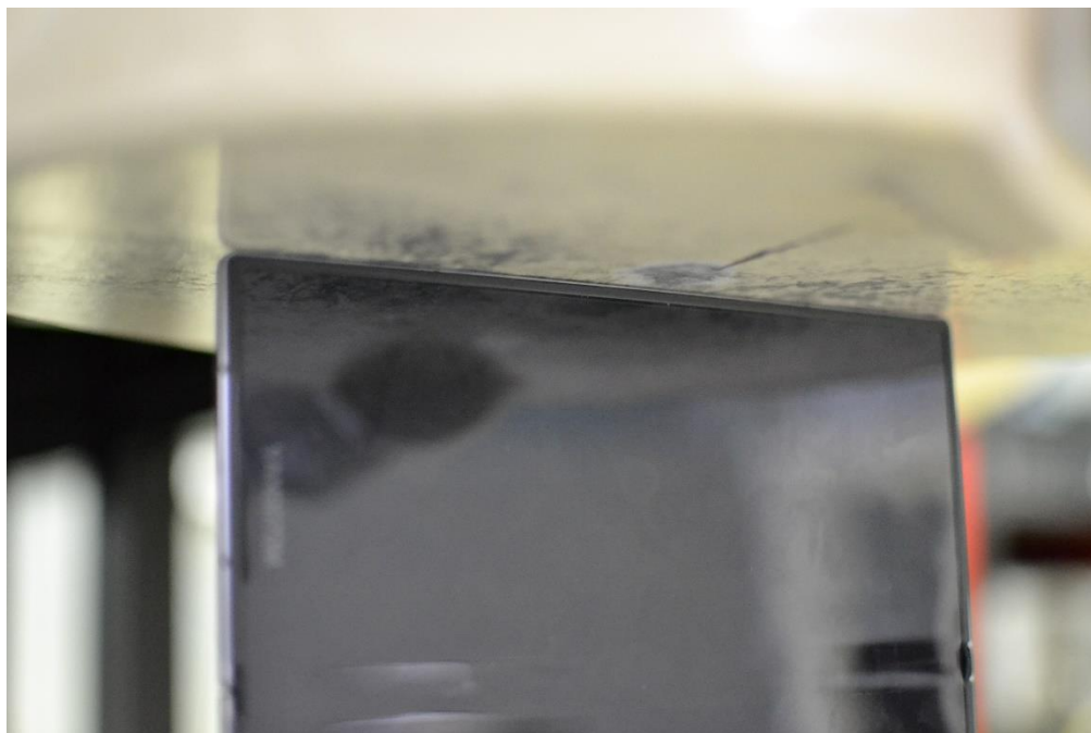
SAR Test Setup Photo 31 – Tablet, Folder Open, Left Edge at 0mm
