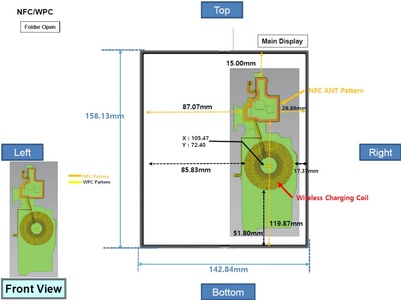
Figure J-4 NFC Antenna Locations – Folder Open
