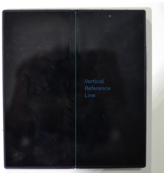
SAR Test Setup Photo 42 –Reference Lines Open
