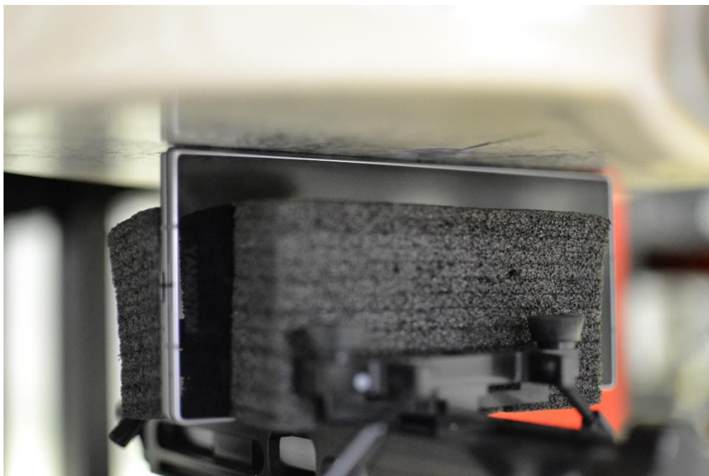
SAR Test Setup Photo 22 – Phablet, Folder Closed, Left Edge at 0mm
