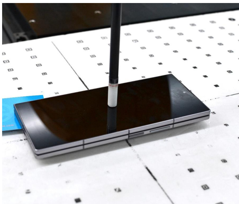
PD Test Setup Photo 47 – PD, Closed Front Side at 2mm
