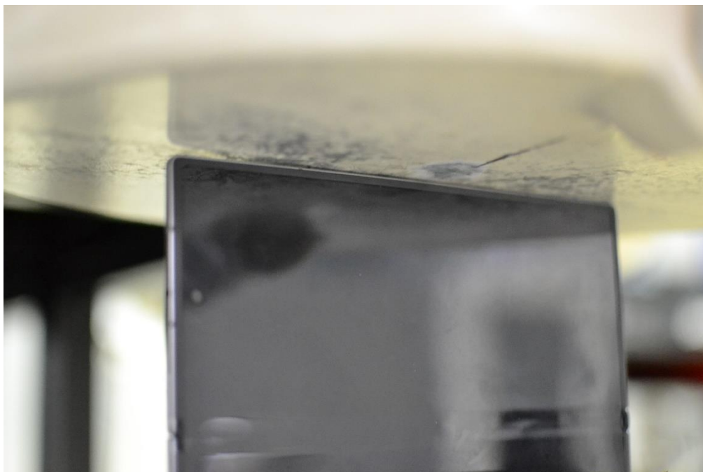
SAR Test Setup Photo 30 – Tablet, Folder Open, Right Edge at 0mm
