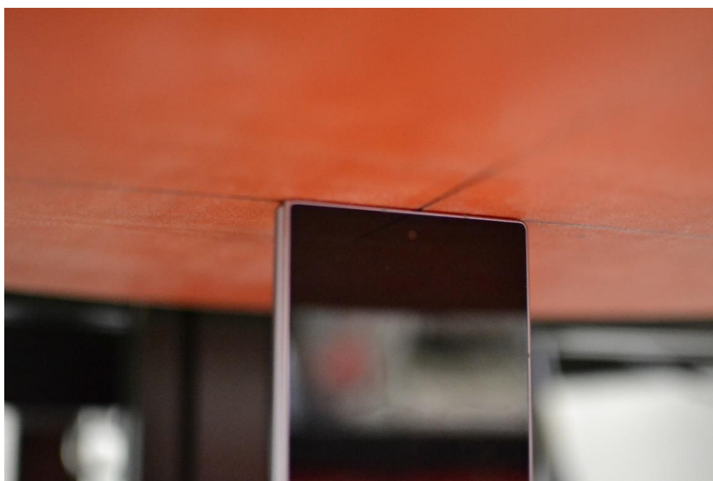
SAR Test Setup Photo 34 – NFC Phablet, Folder Closed, Top Edge at 0mm
