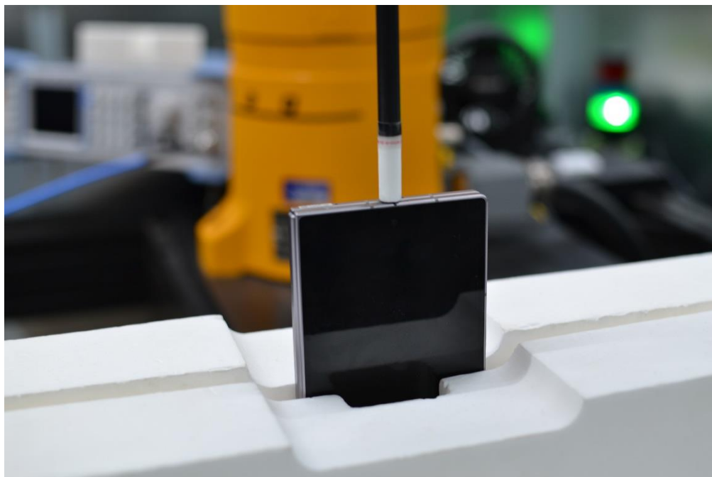
PD Test Setup Photo 48 – PD, Closed Top Edge at 2mm
