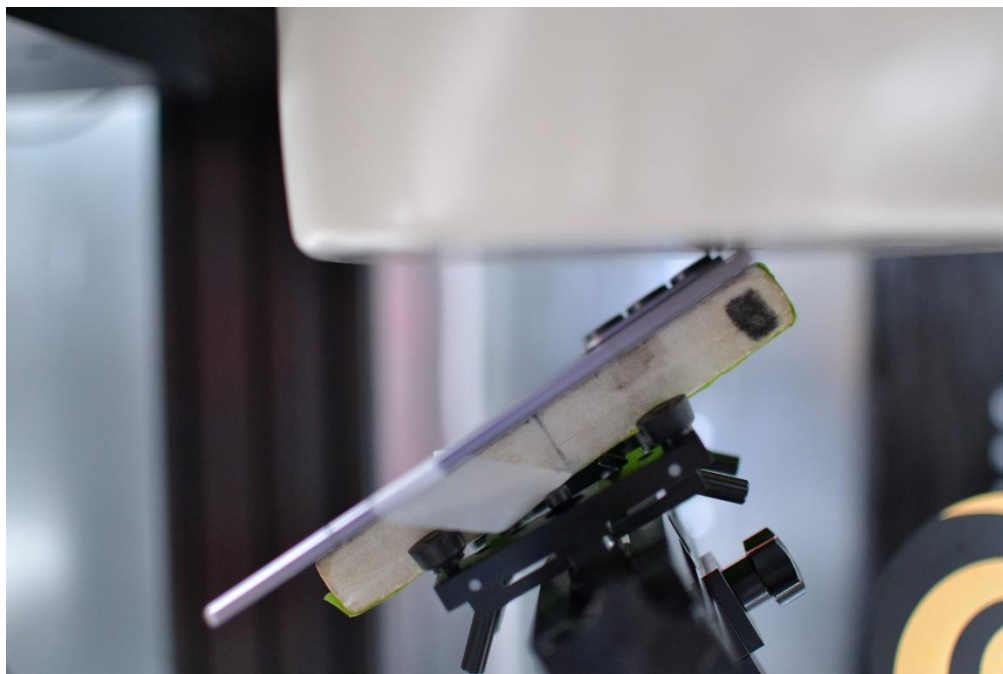
SAR Test Setup Photo 25 – Tablet, Folder Open, Back Side at 0mm (for AG1)
