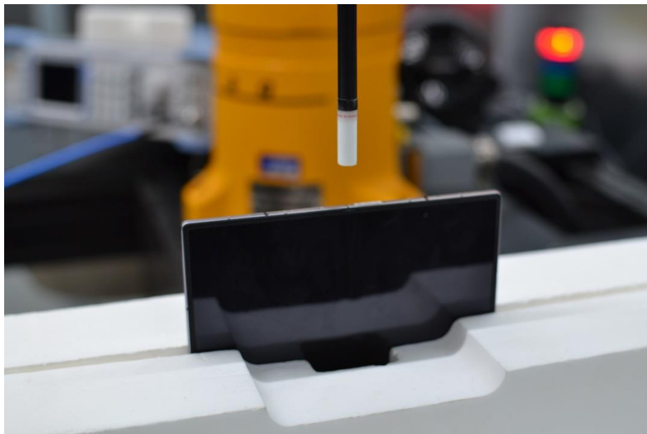
PD Test Setup Photo 50 – PD, Open Top Edge at 9.22mm
