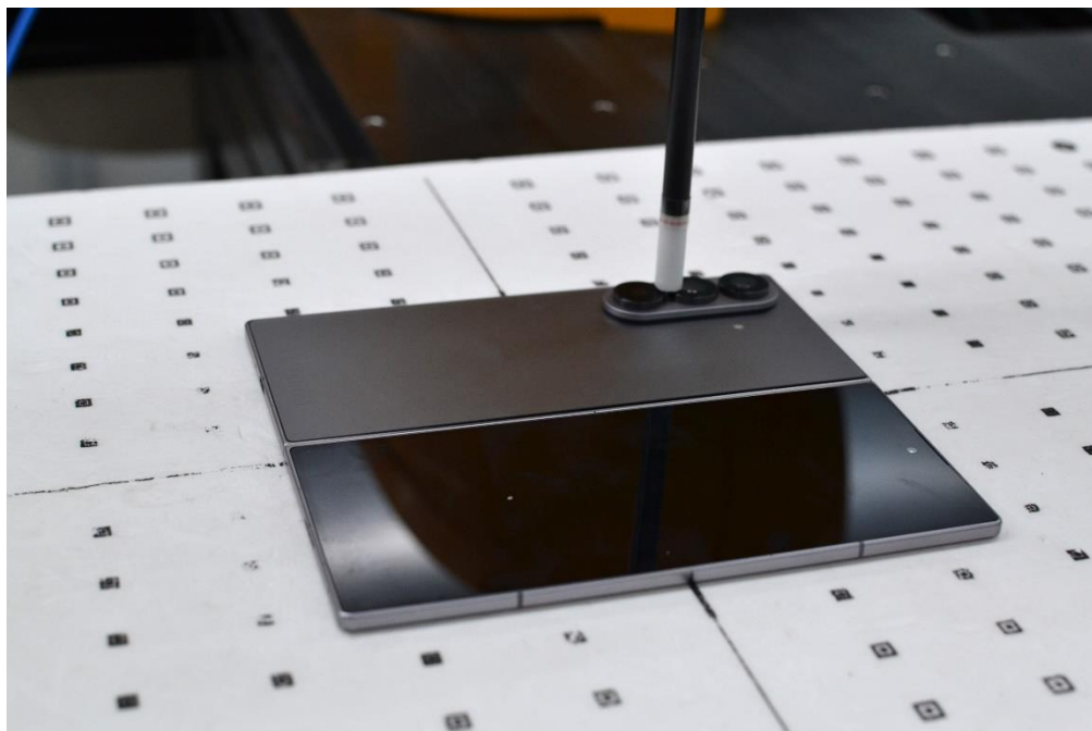
PD Test Setup Photo 46 – PD, Open Back Side at 2mm
