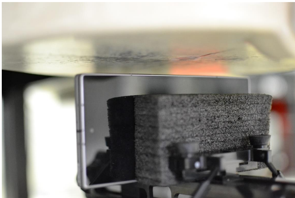
SAR Test Setup Photo 19 – Hotspot, Folder Closed, Right Edge at 10mm
