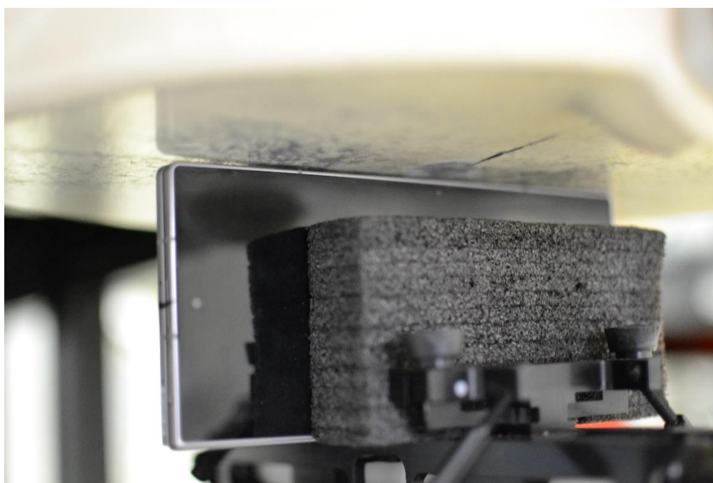
SAR Test Setup Photo 20 – Phablet, Folder Closed, Right Edge at 0mm
