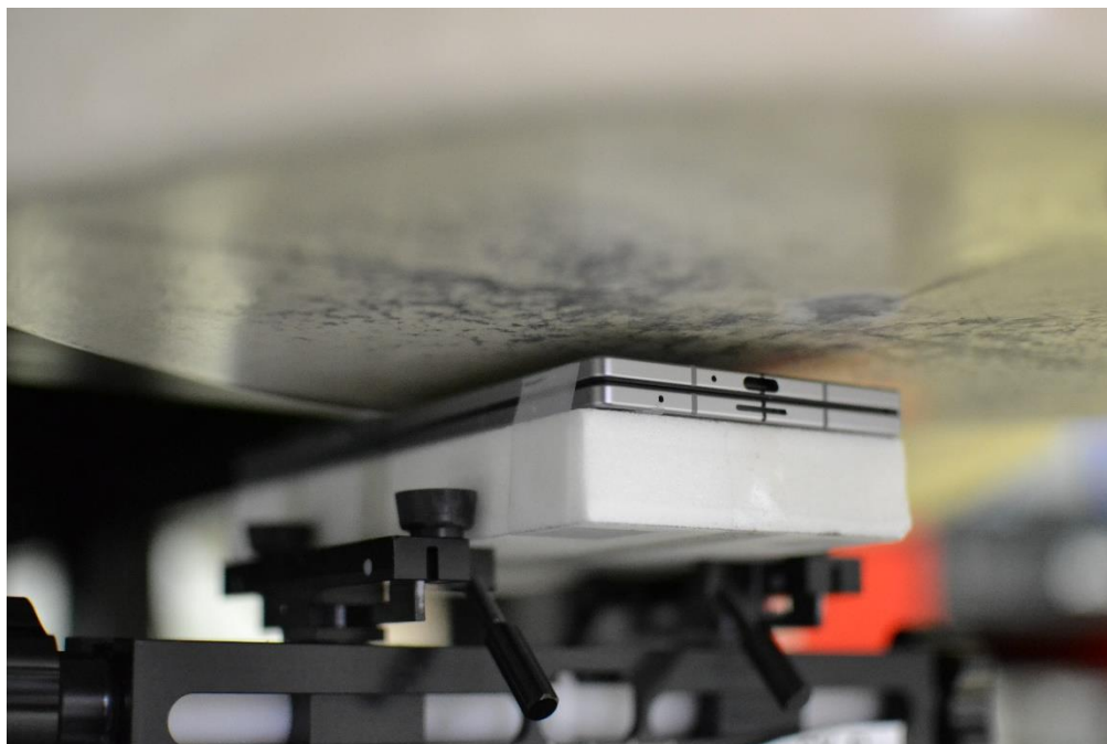
SAR Test Setup Photo 5 – Body-worn/Hotspot, Folder Closed, Back Side at 5mm (for AG0)
