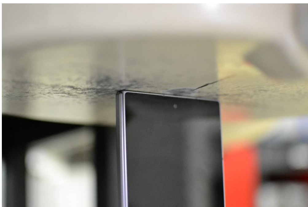
SAR Test Setup Photo 18 – Phablet, Folder Closed, Top Edge at 0mm
