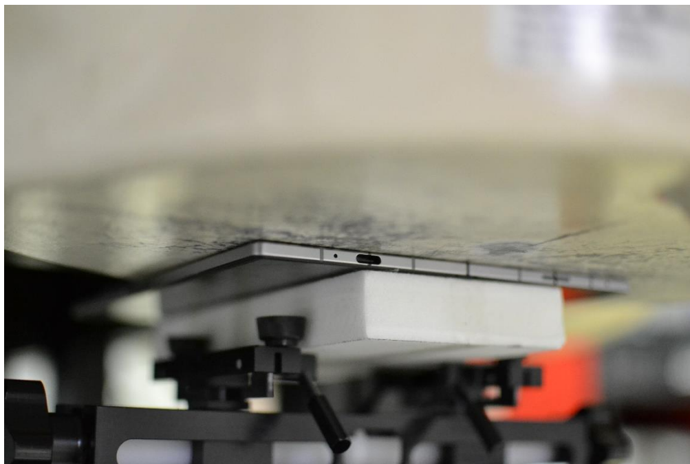
SAR Test Setup Photo 23 – Tablet, Folder Open, Back Side at 0mm (for AG0)
