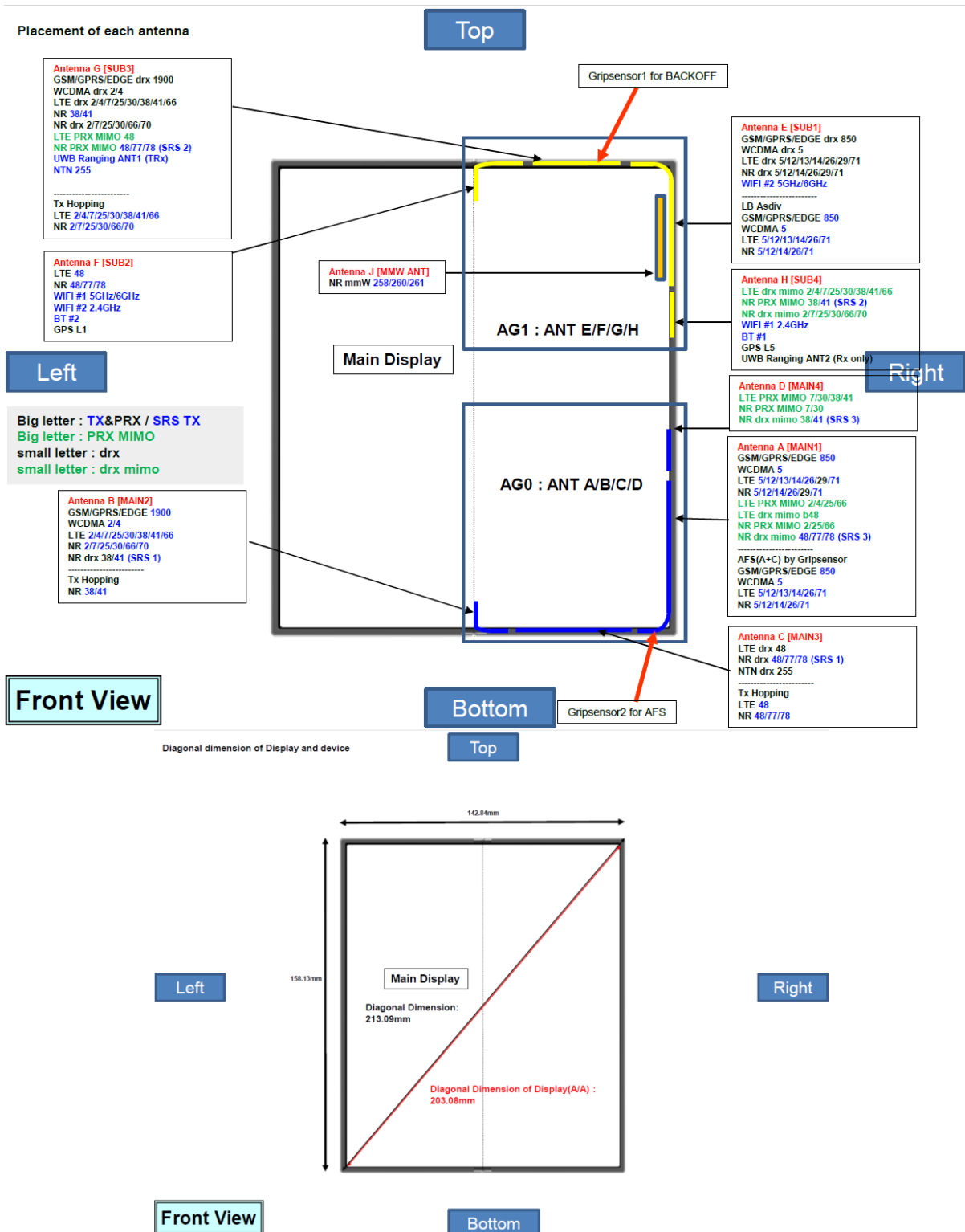
Figure J-2 DUT Antenna Locations – Folder Open
