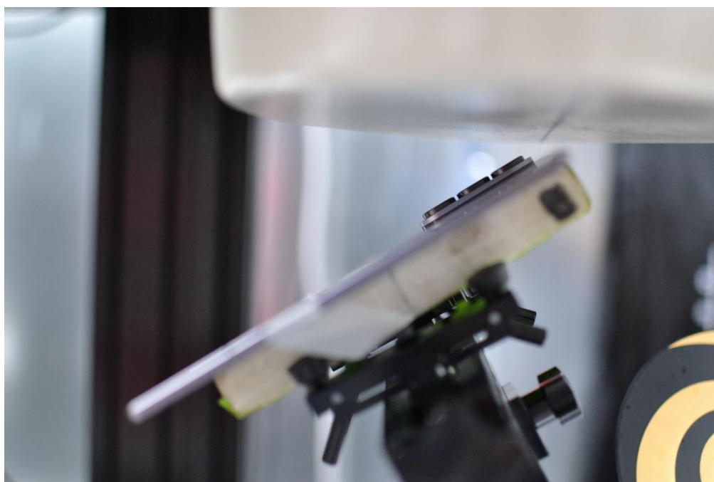
SAR Test Setup Photo 24 – Tablet, Folder Open, Back Side at 10mm (for AG1)
