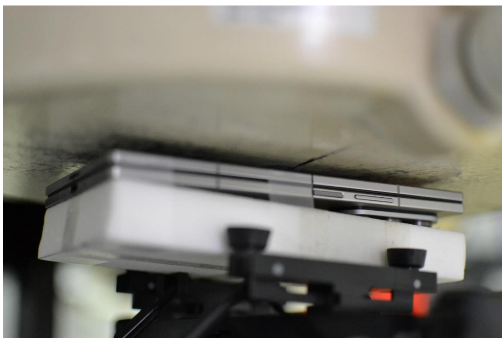
SAR Test Setup Photo 12 – Body-worn/Hotspot, Folder Closed, Front Side at 5mm
