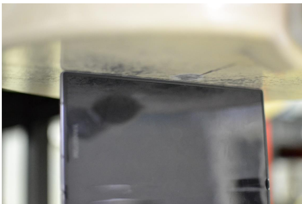
SAR Test Setup Photo 40 – NFC Tablet, Folder Open, Left Edge at 0mm
