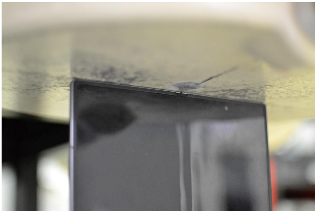
SAR Test Setup Photo 28 – Tablet, Folder Open, Top Edge at 0mm
