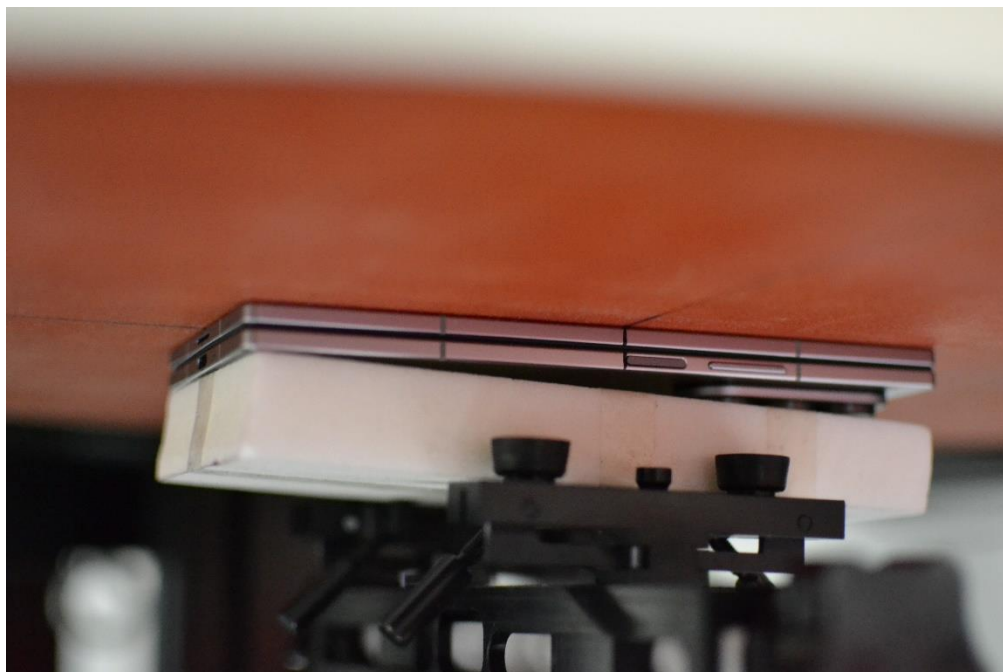
SAR Test Setup Photo 33 – NFC Phablet, Folder Closed, Front Side at 0mm
