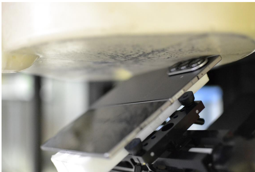
SAR Test Setup Photo 26 – Tablet, Folder Open, Back Side at 0mm (for Antenna H)
