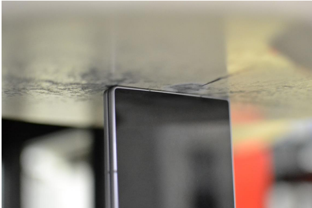
SAR Test Setup Photo 15 – Phablet, Folder Closed, Bottom Edge at 0mm
