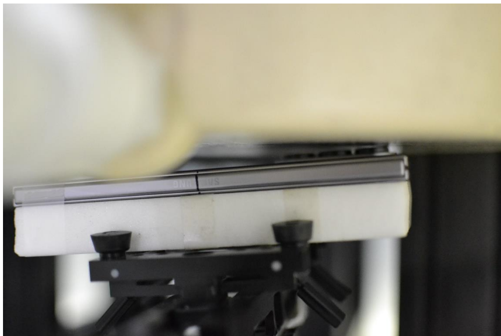
SAR Test Setup Photo 7 – Body-worn/Hotspot, Folder Closed, Back Side at 5mm (for AG1)
