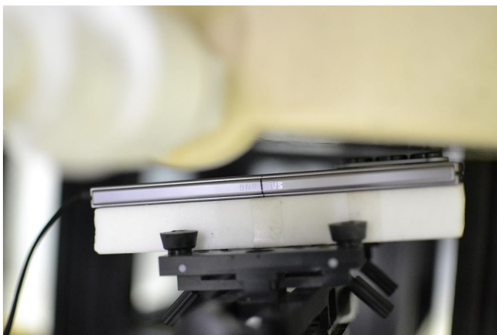
SAR Test Setup Photo 8 – Body-worn/Hotspot, Folder Closed, Back Side at 5mm with headset (for AG1)
