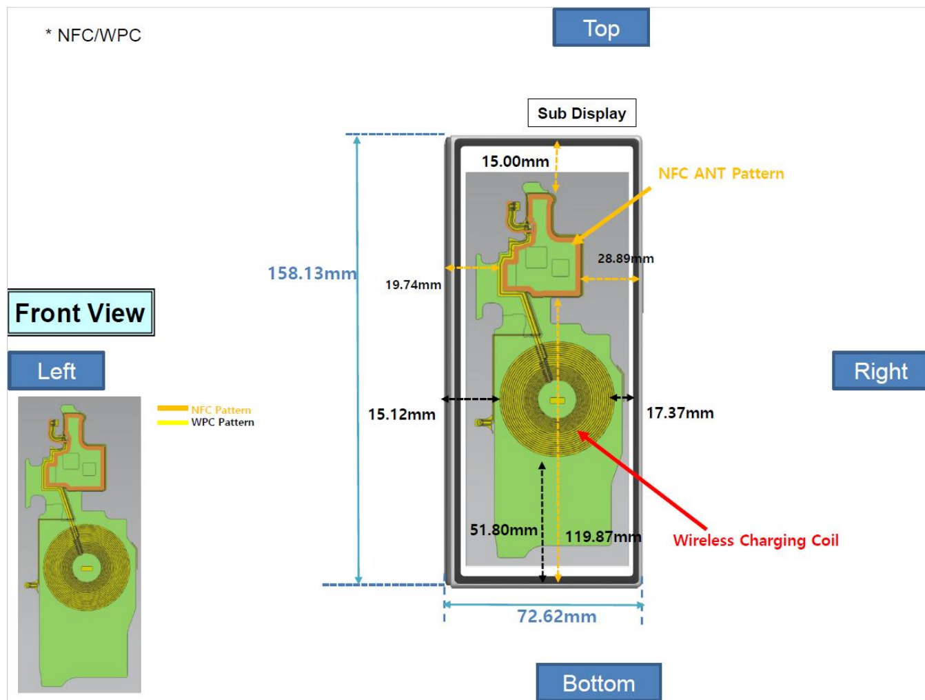
Figure J-3 NFC Antenna Locations – Folder Closed
