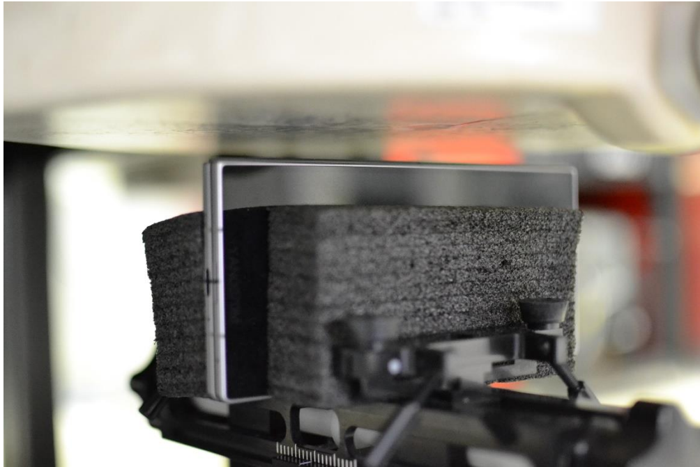
SAR Test Setup Photo 21 – Hotspot, Folder Closed, Left Edge at 10mm
