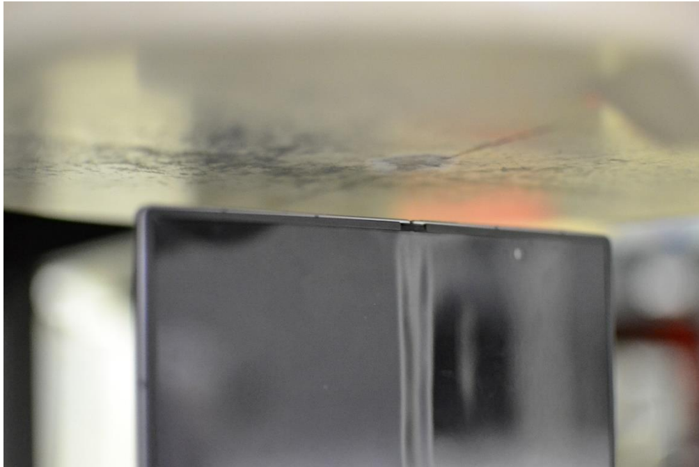
SAR Test Setup Photo 27 – Tablet, Folder Open, Top Edge at 13mm
