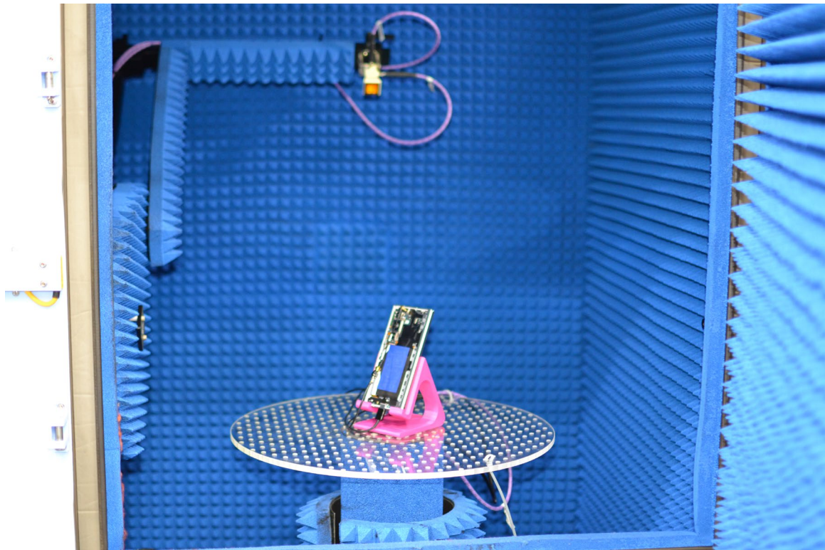
Test Setup Photo 11 – Conducted Test Setup (Figure 8-1)
