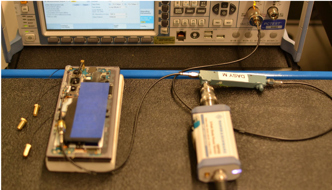
Test Setup Photo 3 – Conducted Test Setup (Figure 7-1a)
