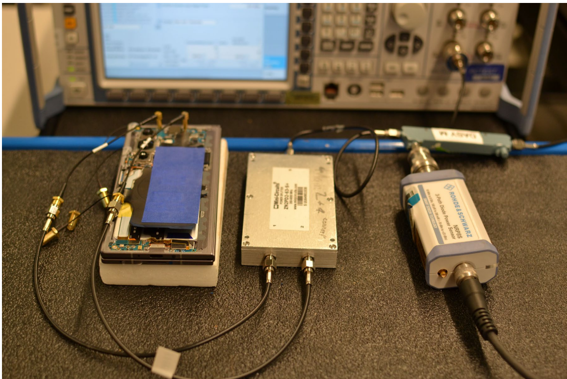
Test Setup Photo 6 – Conducted Test Setup (Figure 7-1b)
