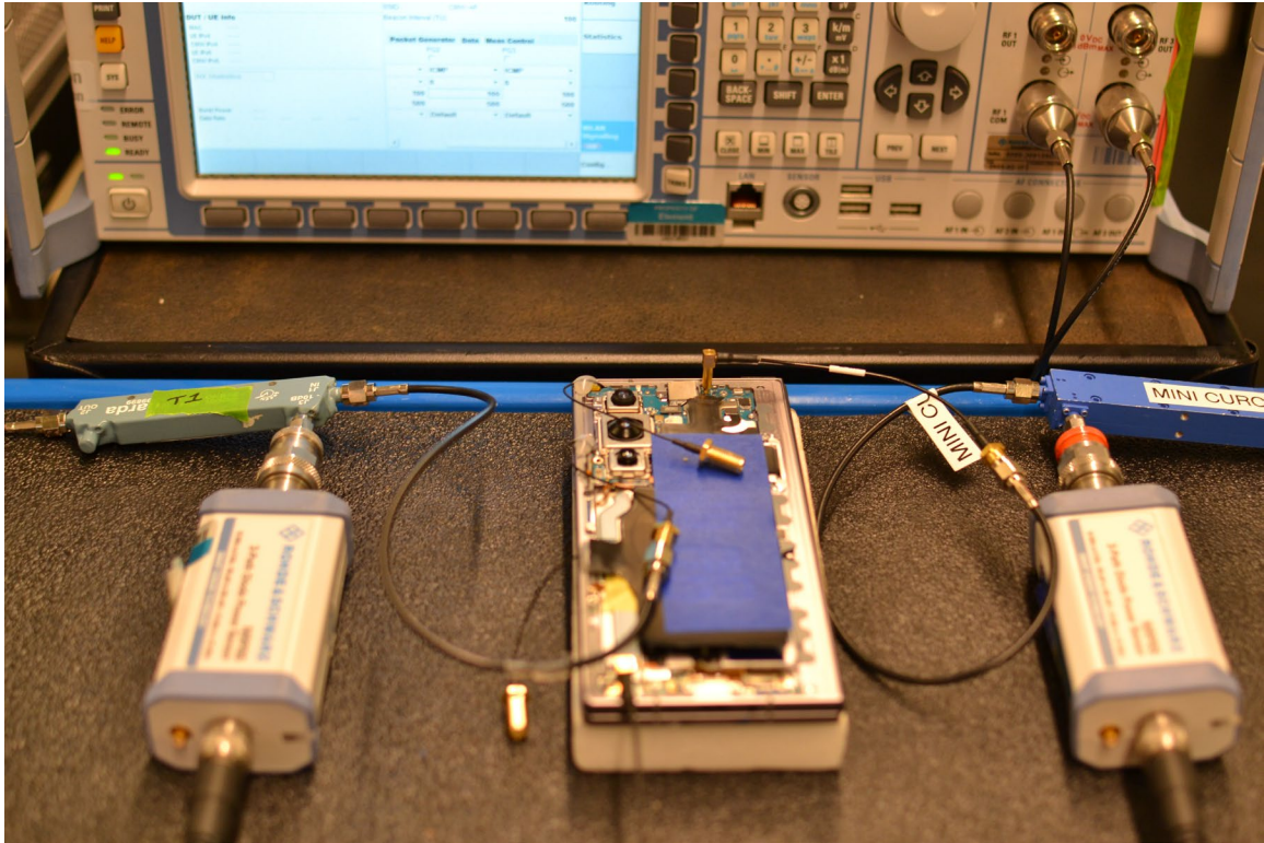
Test Setup Photo 9 – Conducted Test Setup (Figure 7-1d)
