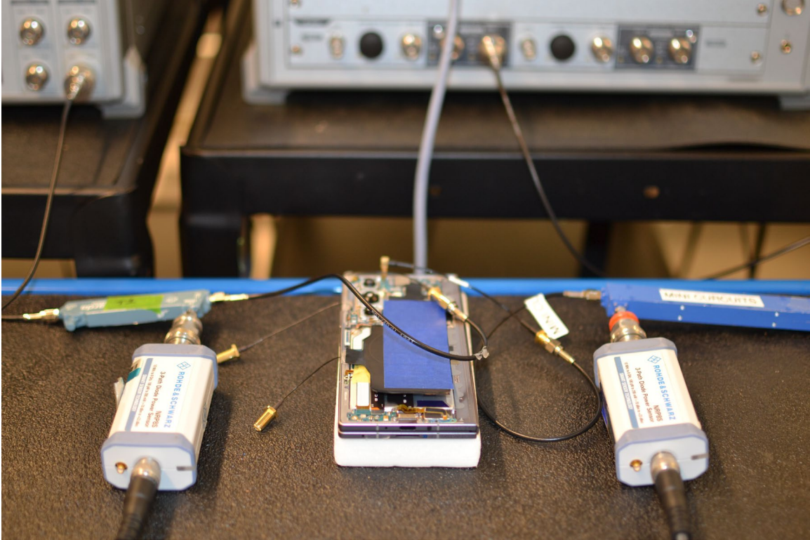
Test Setup Photo 7 – Conducted Test Setup (Figure 7-1c)
