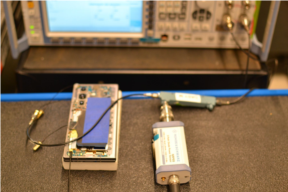
Test Setup Photo 8 – Conducted Test Setup (Figure 7-1d)
