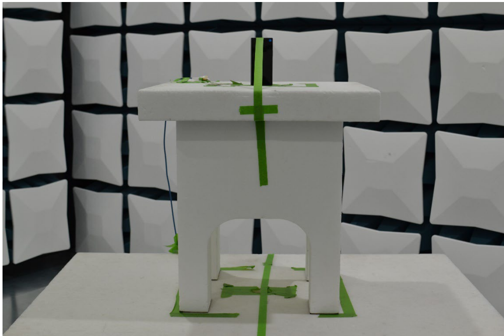
Figure 14. Test Setup – Y Position – 1GHz-40GHz – Closed
