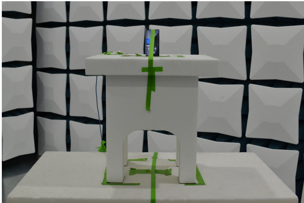
Figure 16. Test Setup – Z Position – 1GHz-40GHz – Half Open
