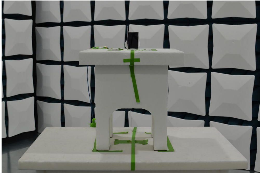
Figure 19. Test Setup – WCP – Half Open
