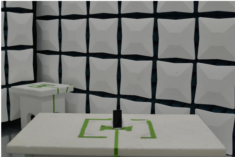
Figure 34. Test Setup – WCP – 30MHz-18GHz – Closed
