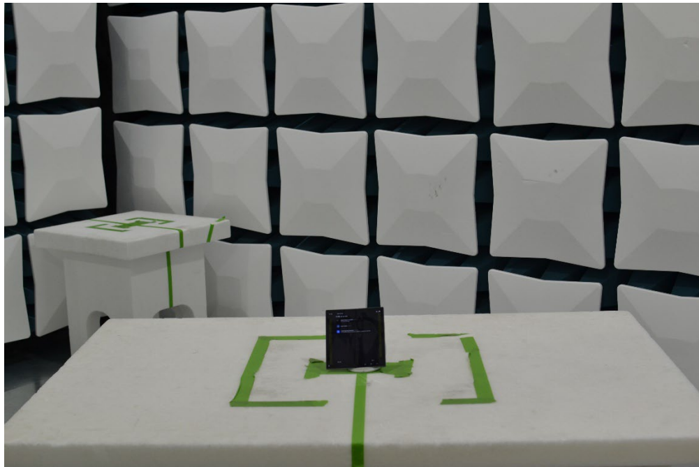
Figure 32. Test Setup – WCP – 30MHz-18GHz – Open
