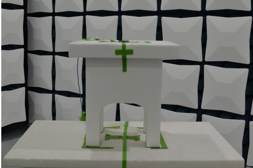
Figure 11. Test Setup – X Position – 1GHz-40GHz – Closed
