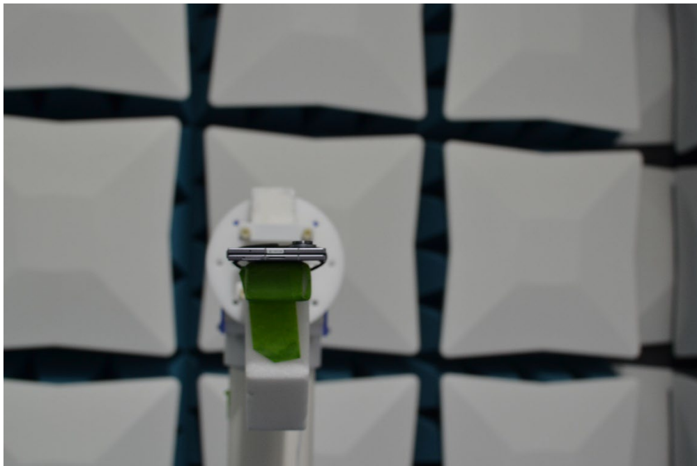
Figure 2. Test Setup – X Down Position - >18GHz – Closed
