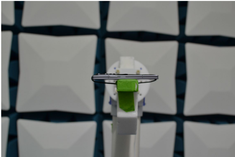
Figure 4. Test Setup – Y Down Position - >18GHz – Closed
