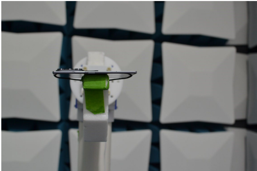
Figure 8. Test Setup – Y Down – Position - >18GHz – Open
