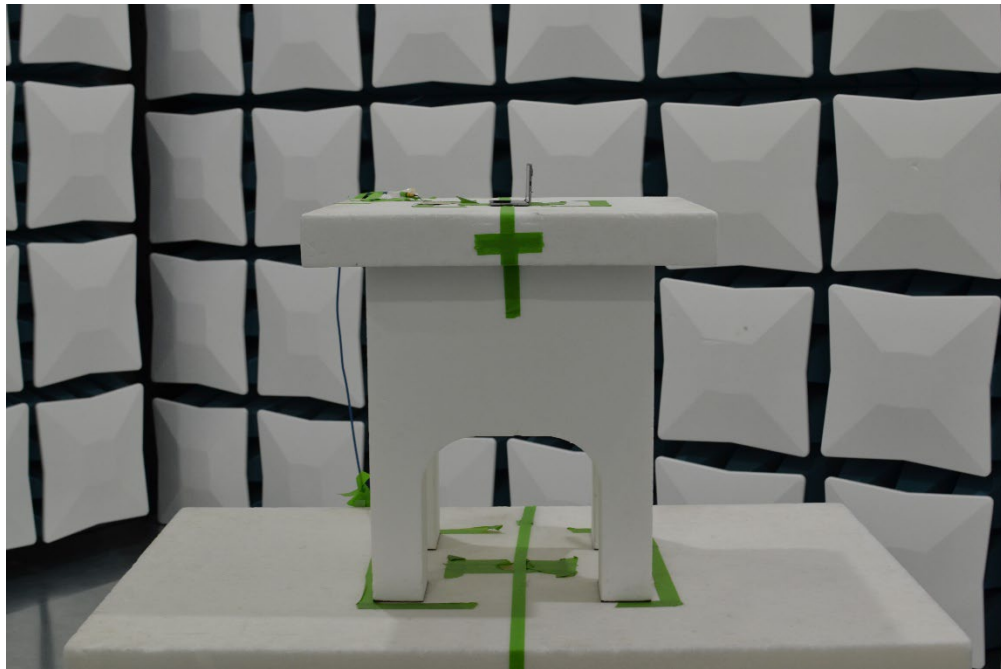
Figure 10. Test Setup – X Position – 1GHz-40GHz – Half Open
