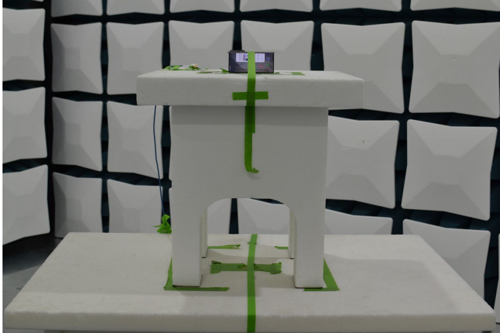
Figure 13. Test Setup – Y Position – 1GHz-40GHz – Half Open
