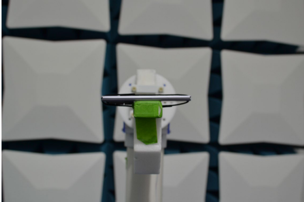
Figure 3. Test Setup – Y Position - >18GHz – Closed
