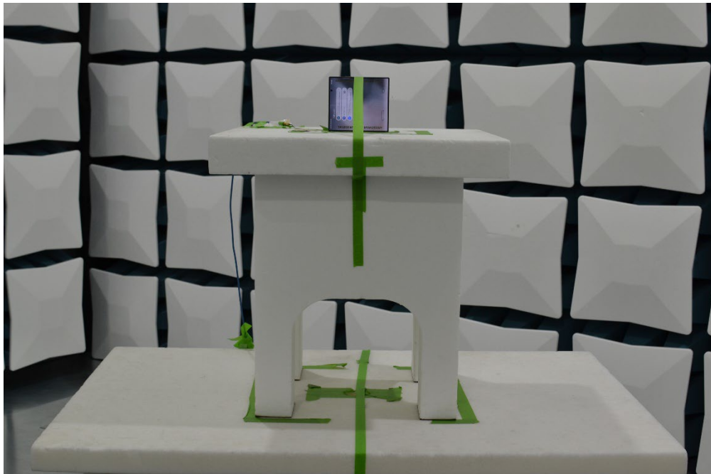
Figure 12. Test Setup – Y Position – 1GHz-40GHz – Open
