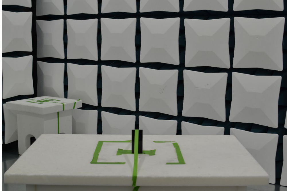
Figure 31. Test Setup – Z Position – 30MHz-18GHz – Closed
