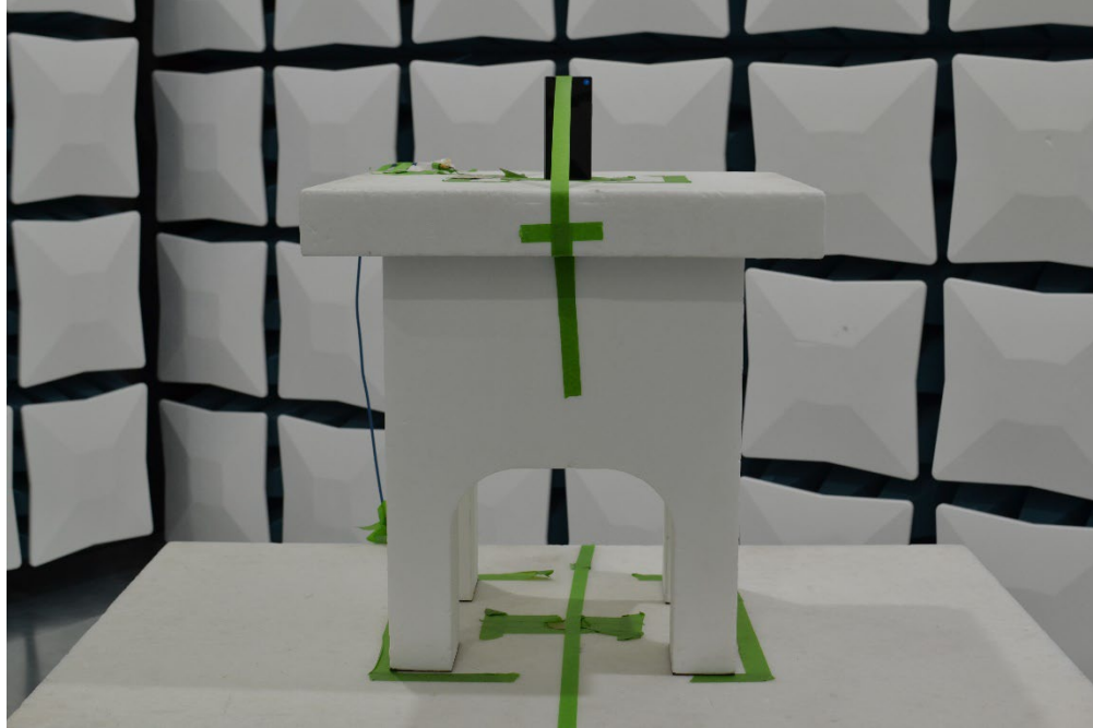
Figure 17. Test Setup – Z Position – 1GHz-40GHz – Closed
