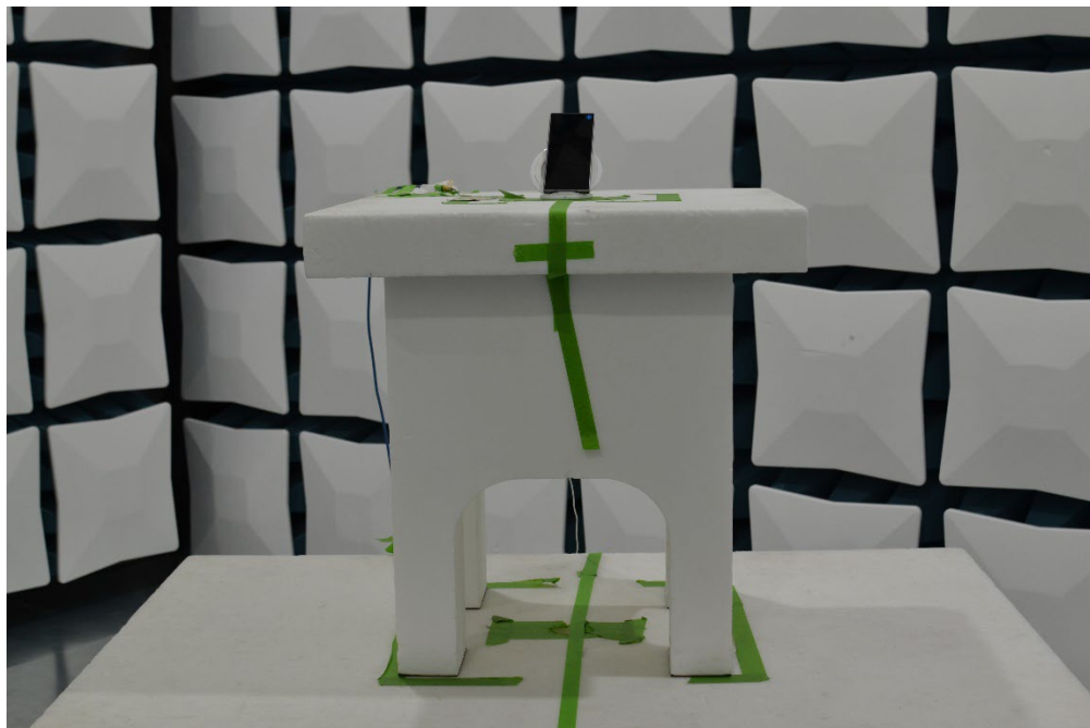
Figure 20. Test Setup – WCP – Closed
