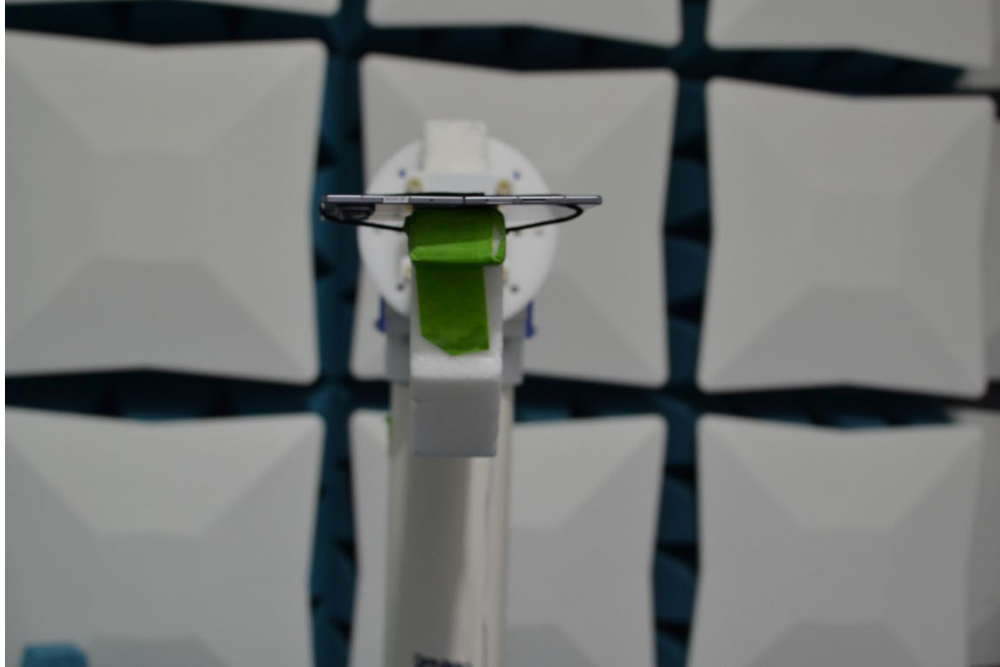
Figure 5. Test Setup – X Position - >18GHz – Open
