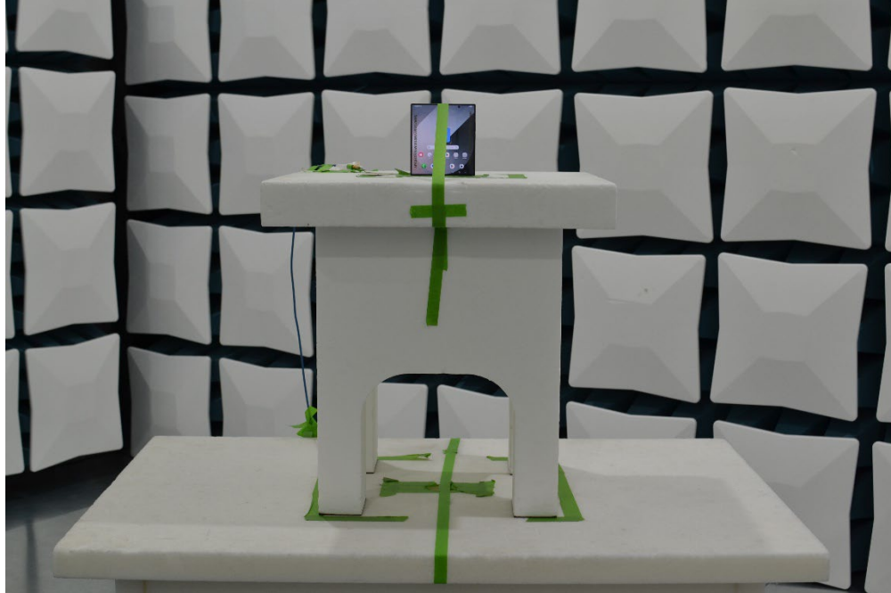
Figure 15. Test Setup – Z Position – 1GHz-40GHz – Open
