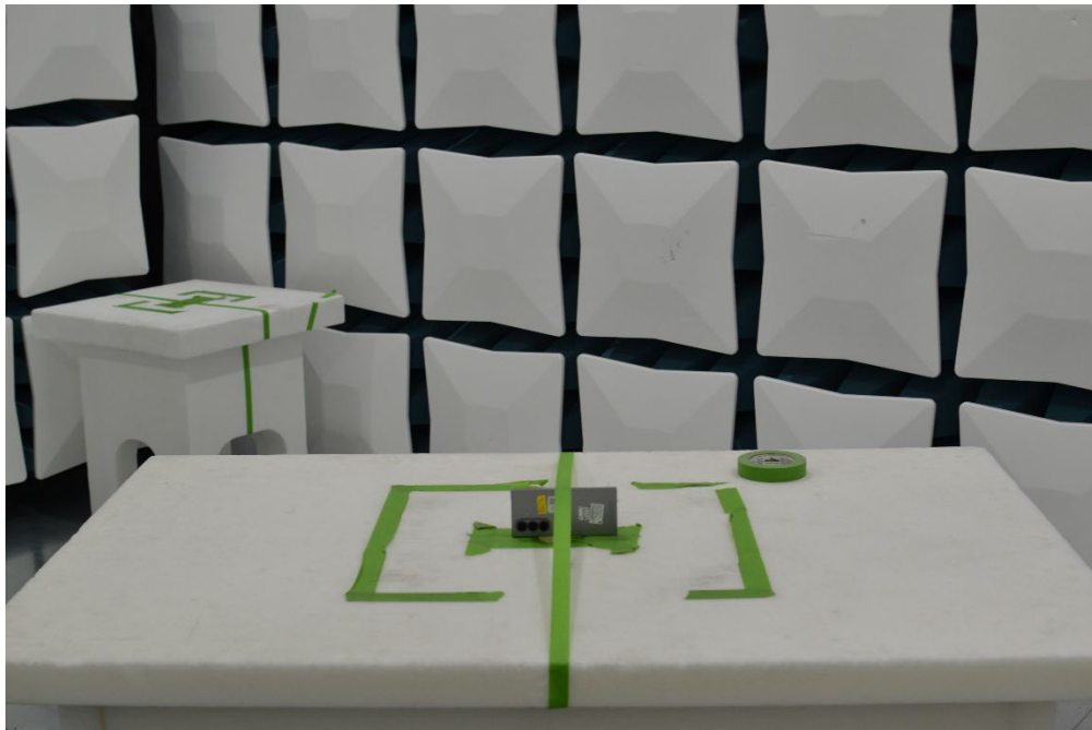
Figure 28. Test Setup – Y Position – 30MHz-18GHz – Closed
