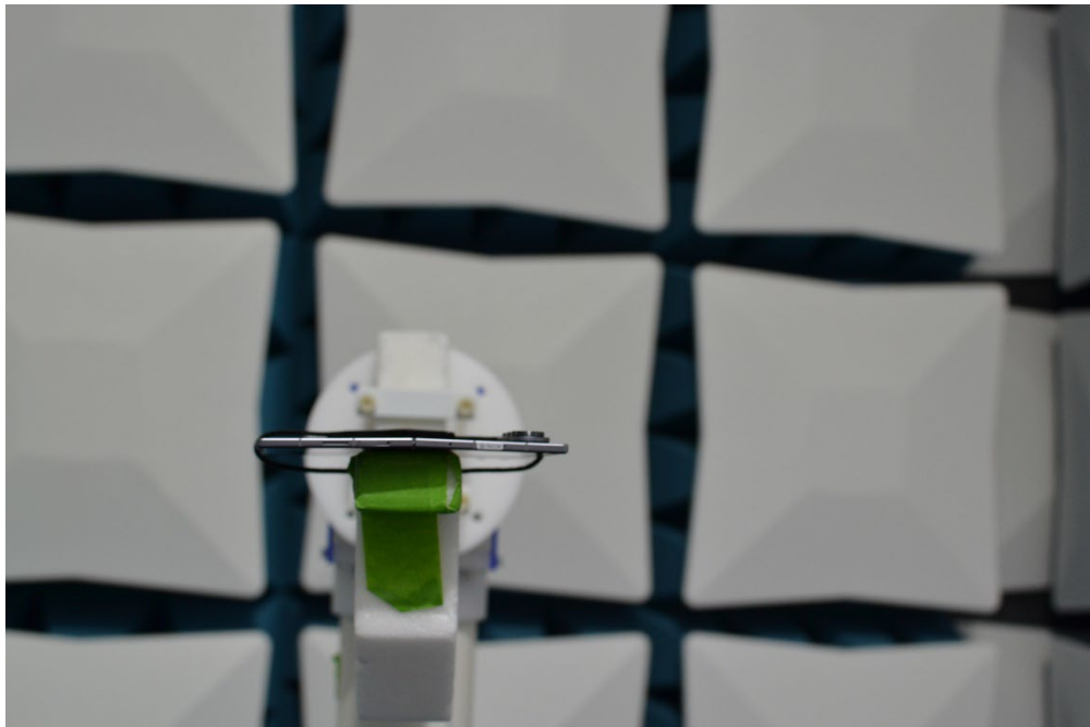
Figure 6. Test Setup – X Down Position - >18GHz – Open
