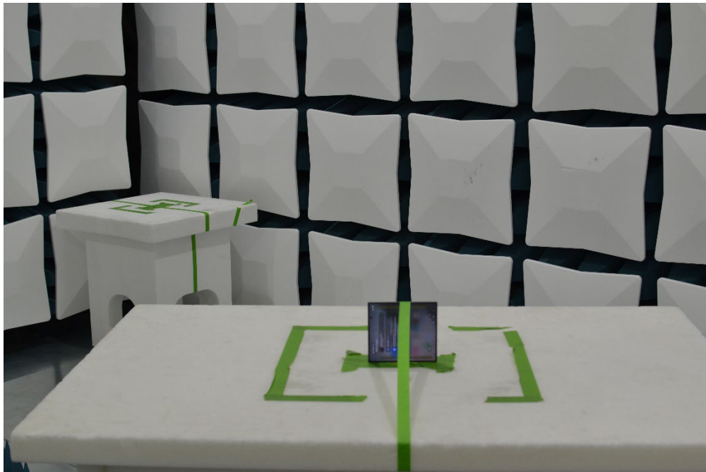
Figure 26. Test Setup – Y Position – 30MHz-18GHz – Open
