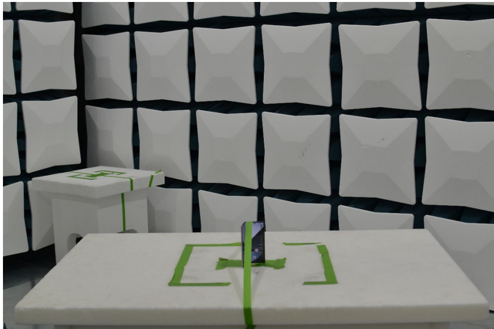
Figure 30. Test Setup – Z Position – 30MHz-18GHz – Half-Open
