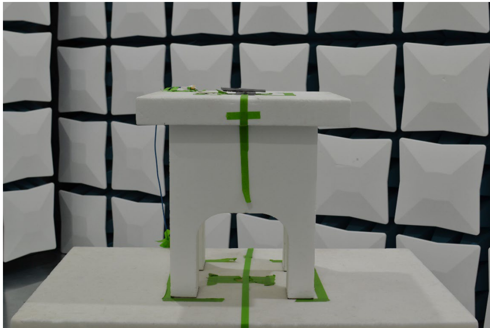
Figure 22. Test Setup – WPT
