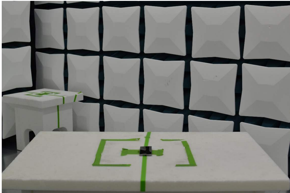
Figure 14. Test Setup – X Position – 30MHz-18GHz – Closed
