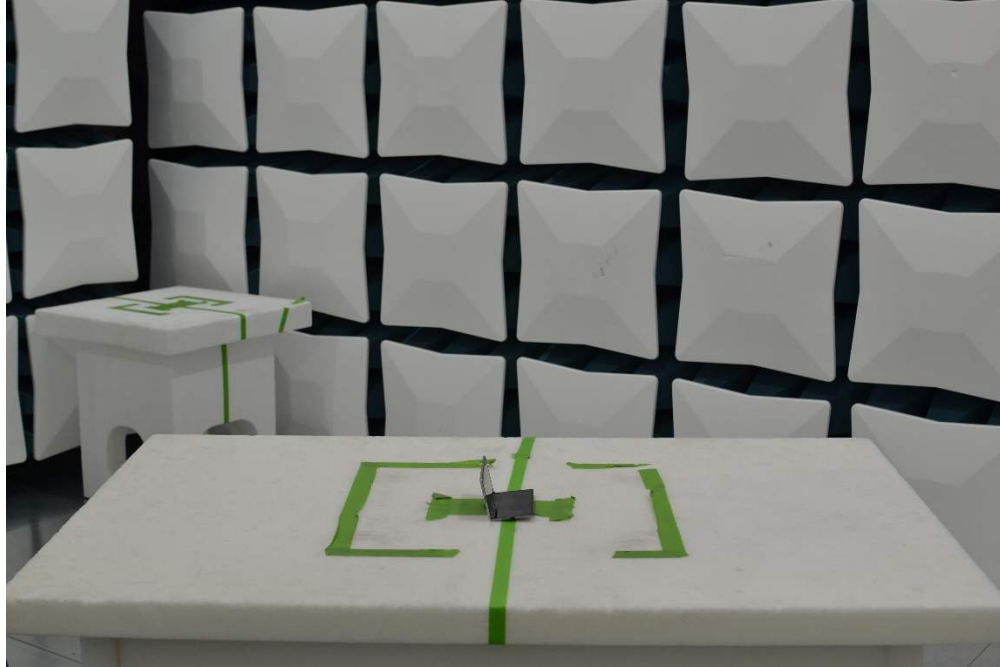
Figure 13. Test Setup – X Position – 30MHz-18GHz – Half Open
