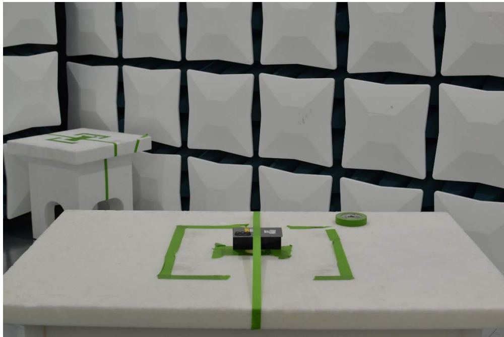
Figure 16. Test Setup – Y Position – 30MHz-18GHz – Half Open
