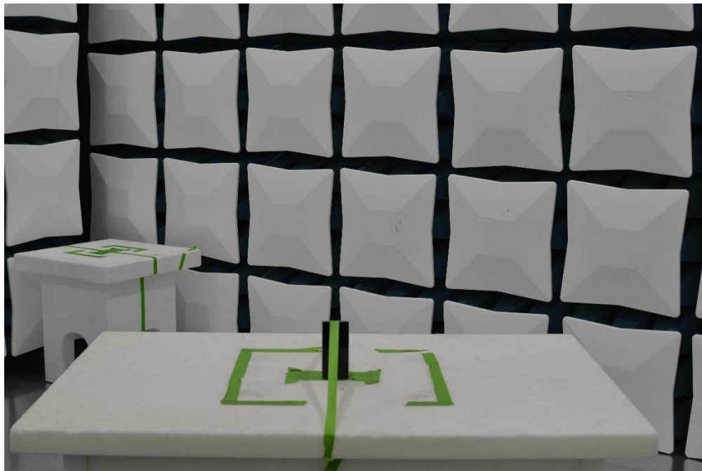
Figure 20. Test Setup – Z Position – 30MHz-18GHz – Closed
