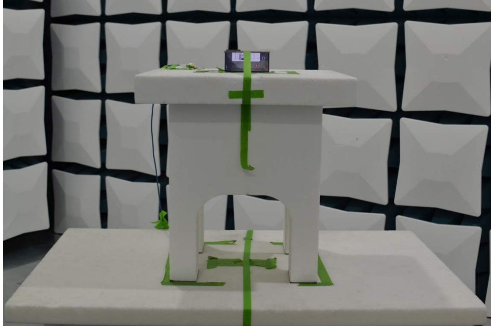
Figure 5. Test Setup – Y Position – 1GHz-40GHz – Half Open
