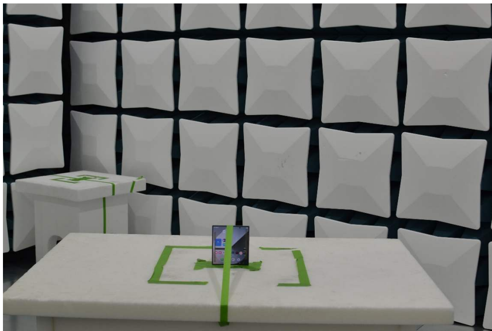
Figure 18. Test Setup – Z Position – 30MHz-18GHz – Open
