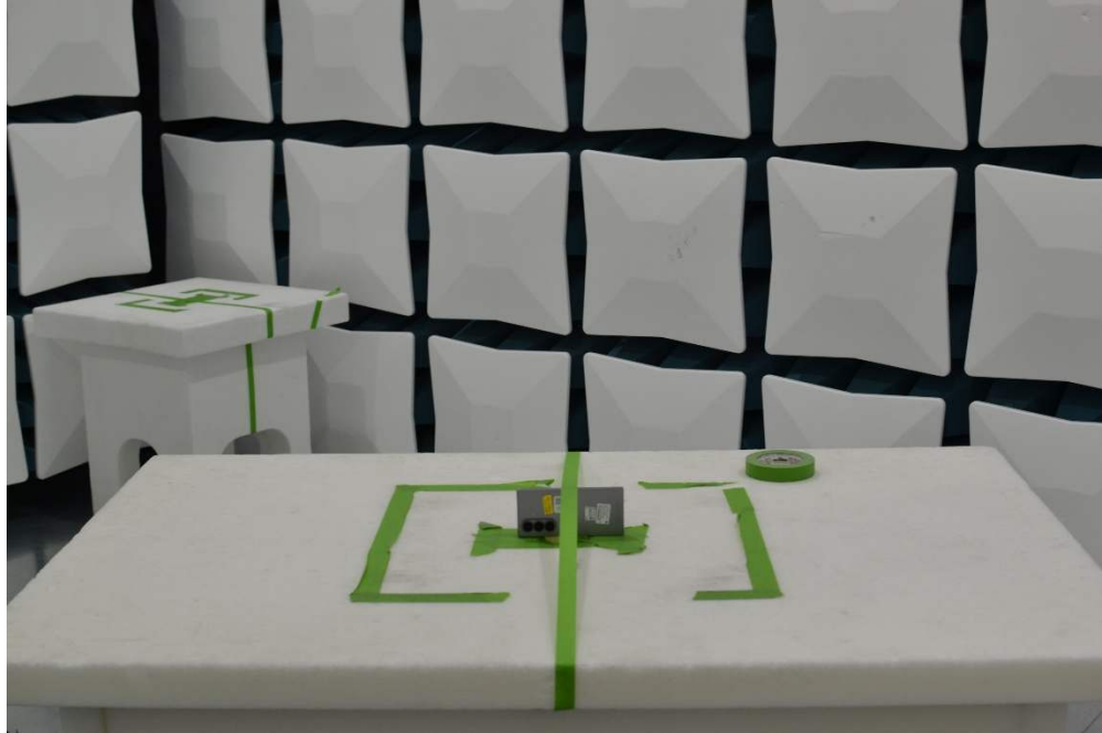
Figure 17. Test Setup – Y Position – 30MHz-18GHz – Closed
