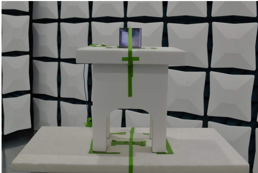
Figure 4. Test Setup – Y Position – 1GHz-40GHz – Open
