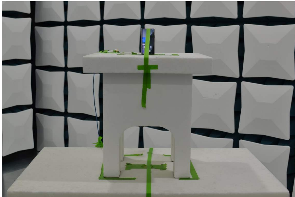
Figure 8. Test Setup – Z Position – 1GHz-40GHz – Half Open
