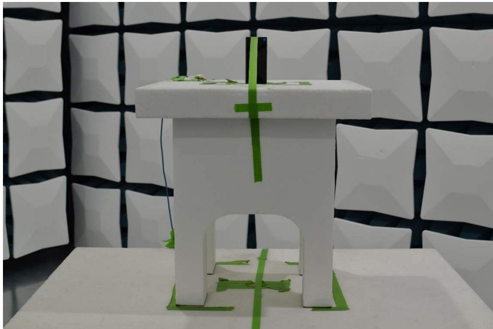
Figure 6. Test Setup – Y Position – 1GHz-40GHz – Closed
