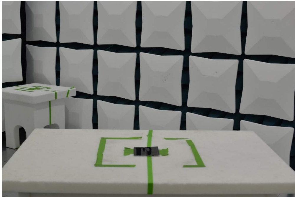
Figure 12. Test Setup – X Position – 30MHz-18GHz – Open
