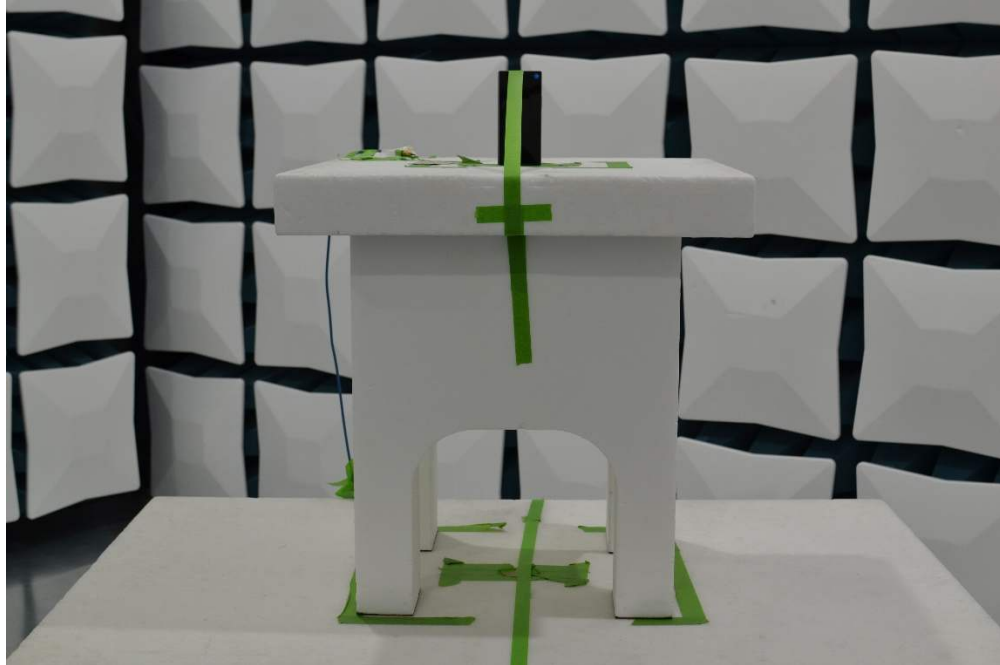
Figure 9. Test Setup – Z Position – 1GHz-40GHz – Closed
