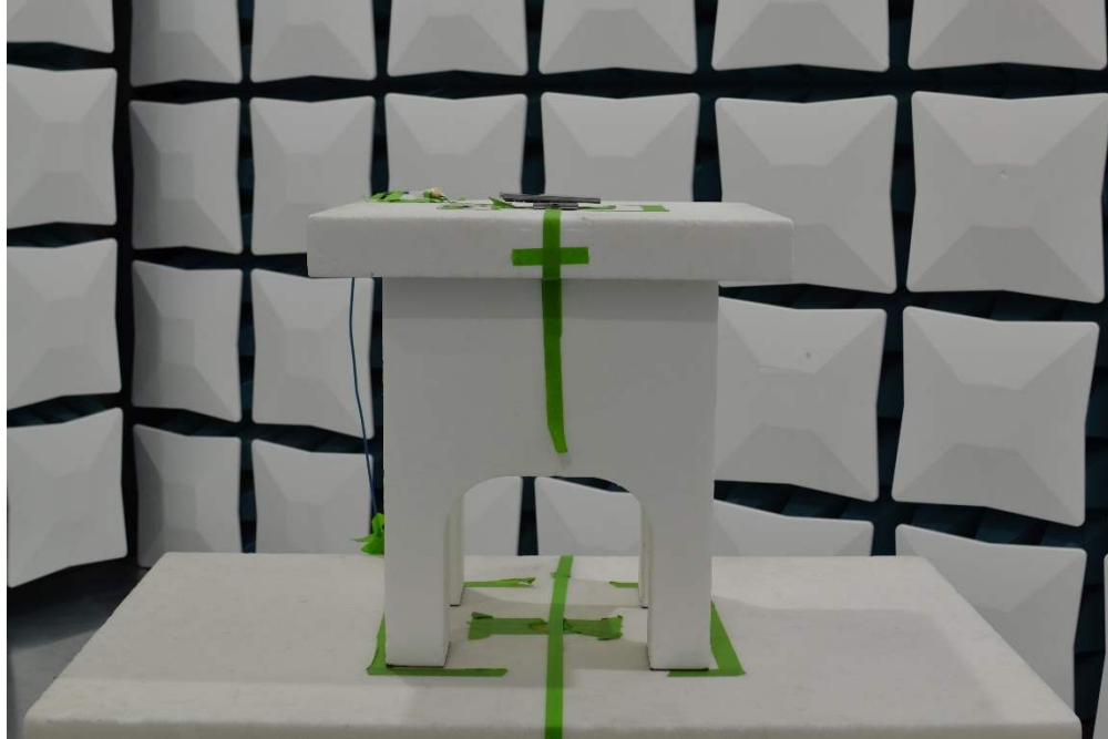
Figure 11. Test Setup – WPT
