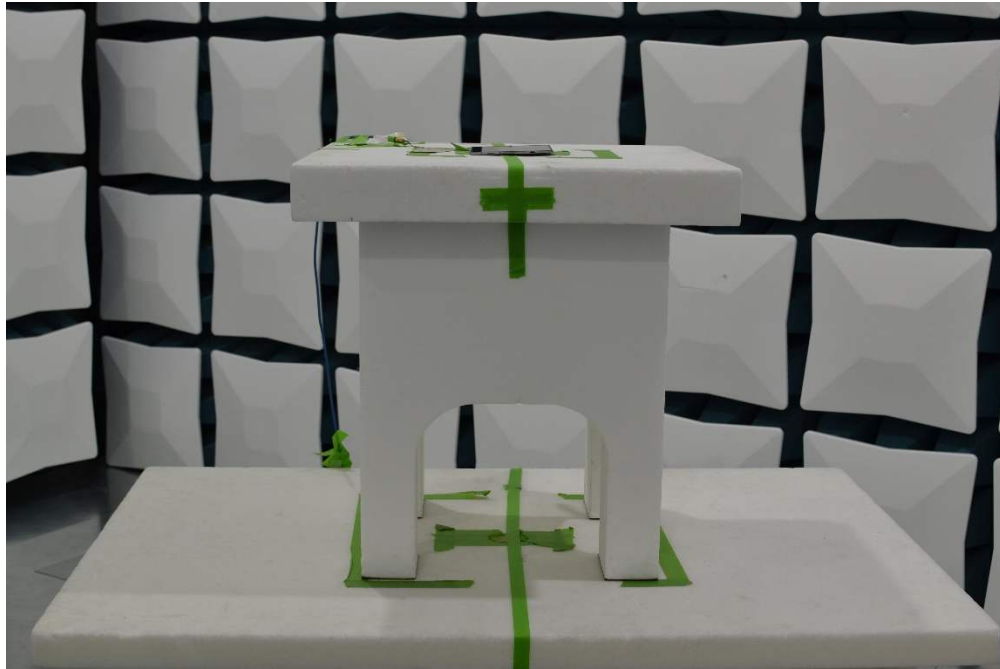
Figure 1. Test Setup – X Position – 1GHz-40GHz – Open
