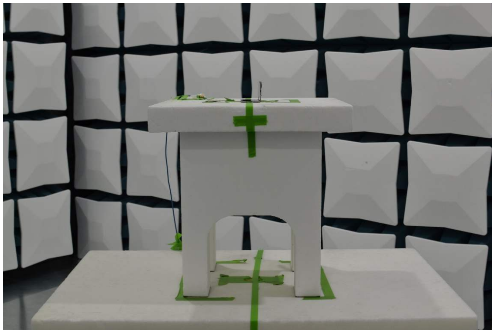
Figure 2. Test Setup – X Position – 1GHz-40GHz – Half Open
