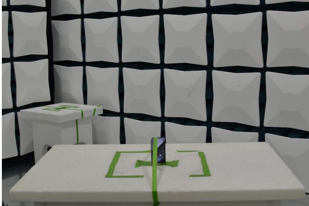
Figure 19. Test Setup – Z Position – 30MHz-18GHz – Half-Open
