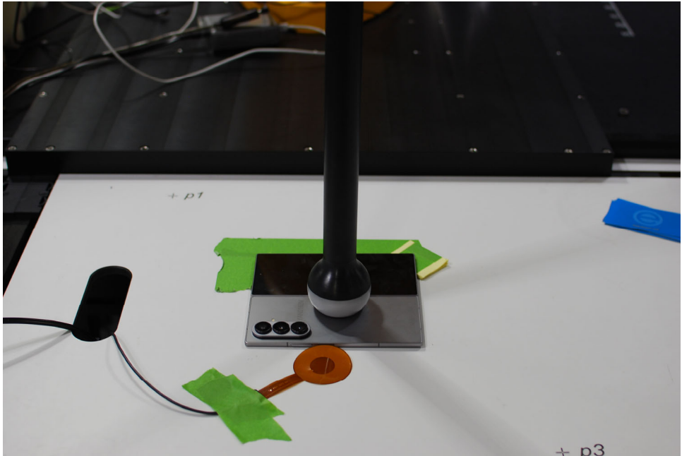
Test Setup Photo 7 Standby (Ping) Signal, Folder Open, Back Side, 0mm
