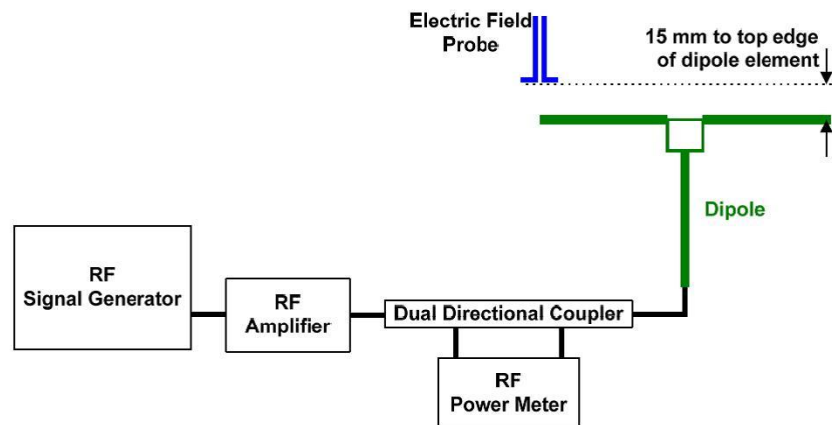
Setup diagram
