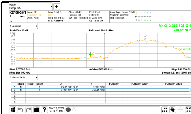
1 Channel Band-edge
