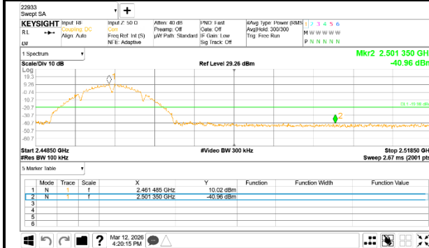
11 Channel Band-edge
