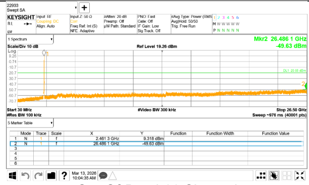
Out-Of-Band 11 Channel
