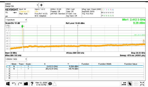
Out-Of-Band 1 Channel
