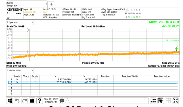
Out-Of-Band 6 Channel
