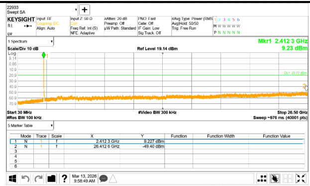
Out-Of-Band 1 Channel
