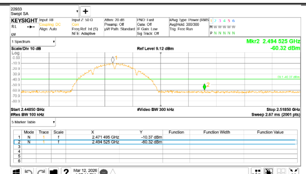
13 Channel Band-edge
