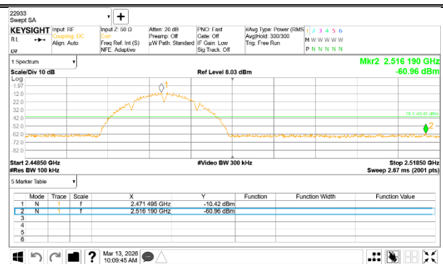
13 Channel Band-edge
