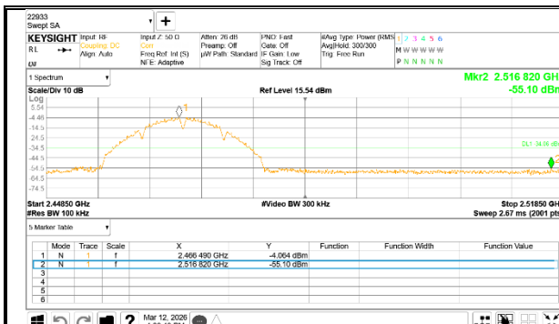
12 Channel Band-edge
