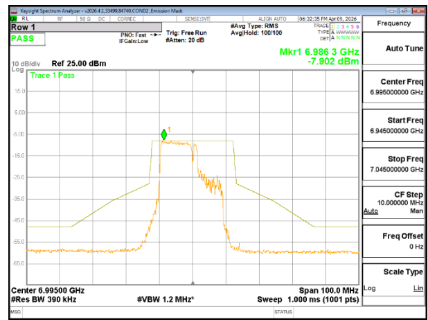
6995 MHz CHAIN 1
