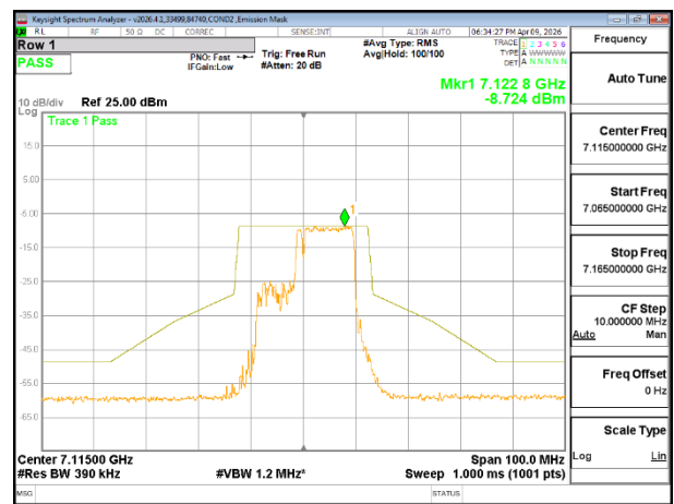
7115 MHz CHAIN 1
