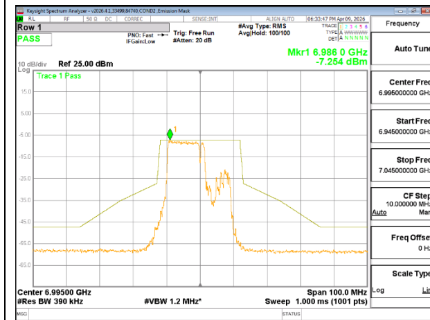
6995 MHz CHAIN 0
