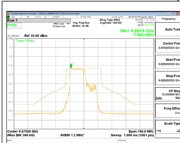
6875 MHz CHAIN 0
