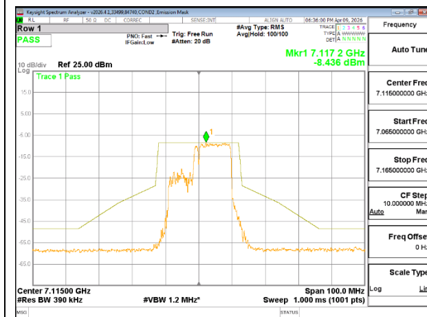
7115 MHz CHAIN 0
