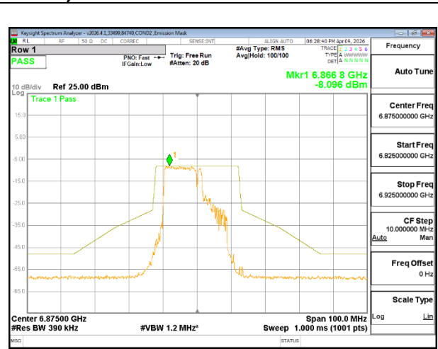
6875 MHz CHAIN 1
