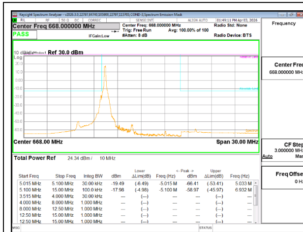
5G NR n71 10MHz BPSK Low Channel RB1-1
