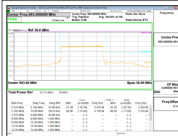
5G NR n71 10MHz BPSK Mid Channel RB50-0
