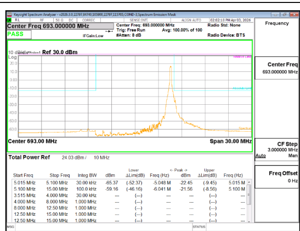
5G NR n71 10MHz BPSK High Channel RB1-50
