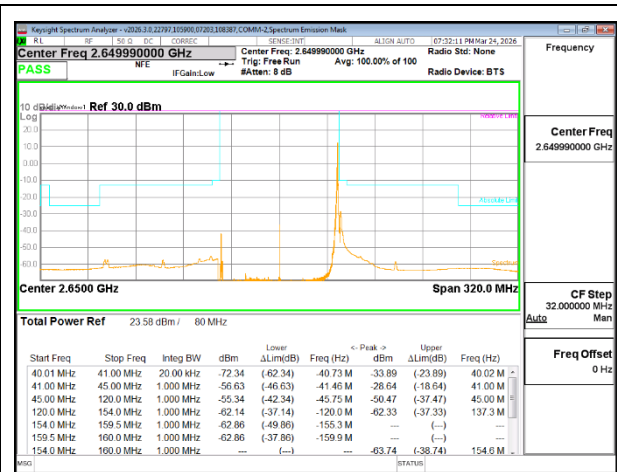
5G NR n41 80MHz BPSK High Channel RB1-215
