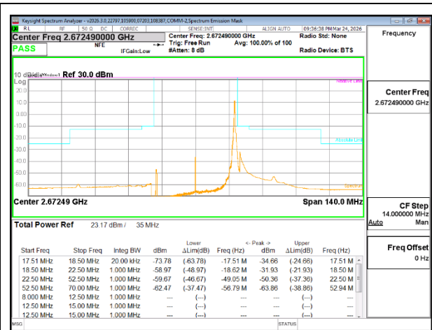
5G NR n41 35MHz BPSK High Channel RB1-90
