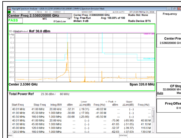
5G NR n41 80MHz BPSK Low Channel RB1-1
