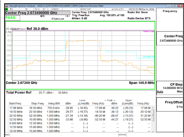
5G NR n41 35MHz BPSK High Channel RB90-0
