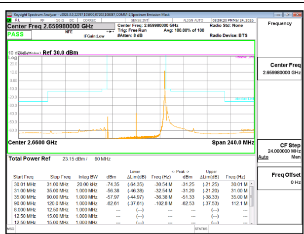
5G NR n41 60MHz BPSK High Channel RB1-160
