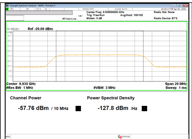
MINIMUM PASSING INCUMBENT SIGNAL POWER
