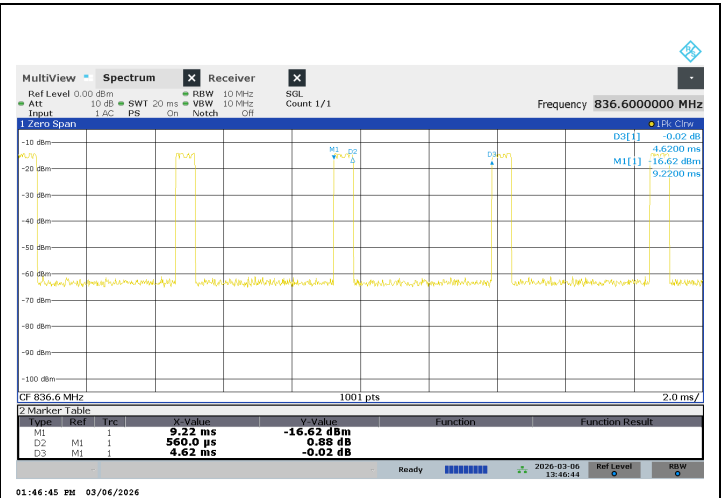
DUTY CYCLE GSM850 – EGPRS
