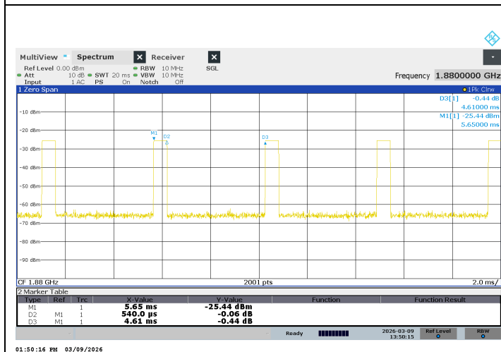
DUTY CYCLE GSM1900 – GPRS
