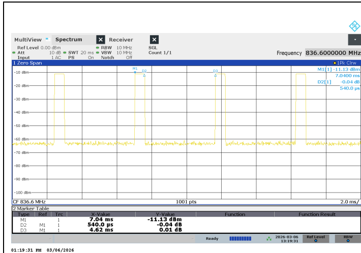
DUTY CYCLE GSM850 – GPRS
