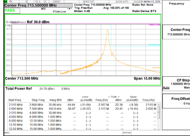
LTE B12 5MHz QPSK High Channel RB1-24
