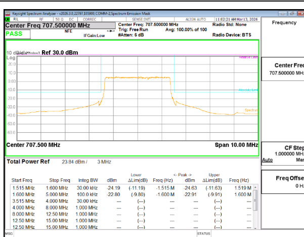
LTE B12 3MHz QPSK Mid Channel RB15-0
