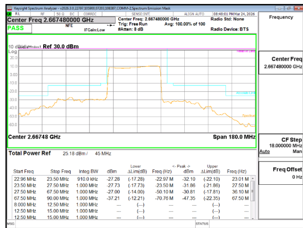
5G NR n41 45MHz BPSK High Channel RB108-0
