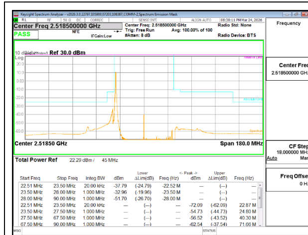
5G NR n41 45MHz BPSK Low Channel RB1-1
