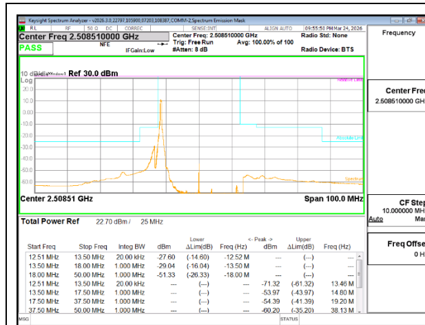
5G NR n41 25MHz BPSK Low Channel RB1-1
