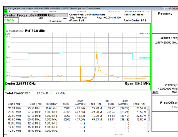
5G NR n41 45MHz BPSK High Channel RB1-117
