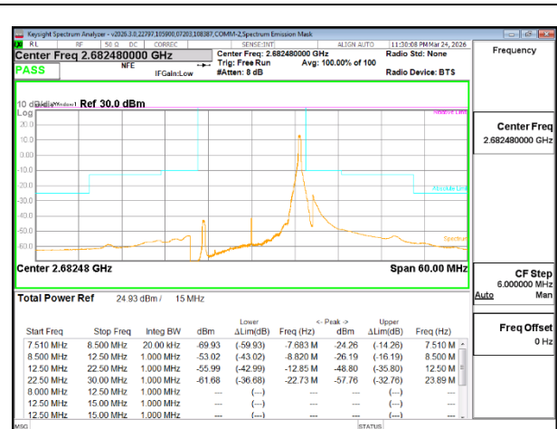
5G NR n41 15MHz BPSK High Channel RB1-36
