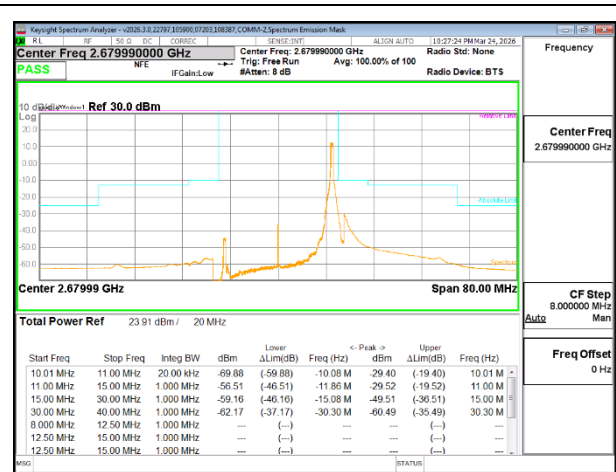
5G NR n41 20MHz BPSK High Channel RB1-49
