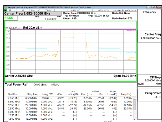
5G NR n41 15MHz BPSK High Channel RB36-0
