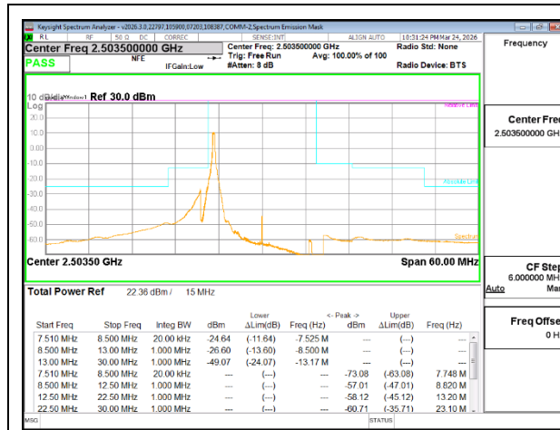
5G NR n41 15MHz BPSK Low Channel RB1-1
