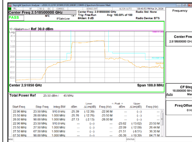
5G NR n41 45MHz BPSK Low Channel RB108-0
