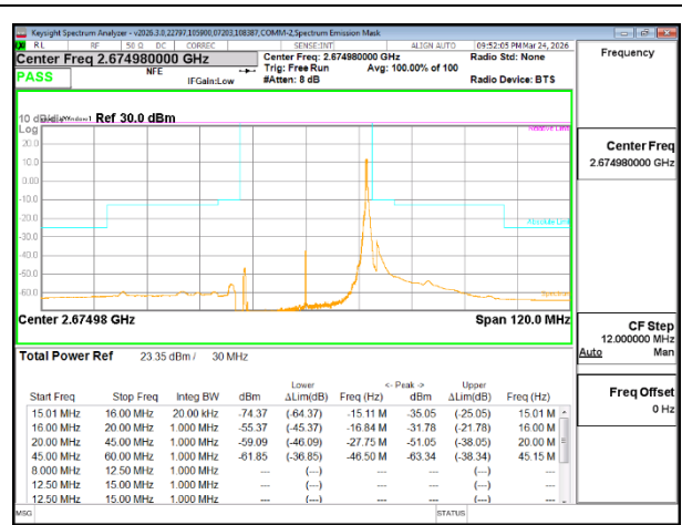
5G NR n41 30MHz BPSK High Channel RB1-76
