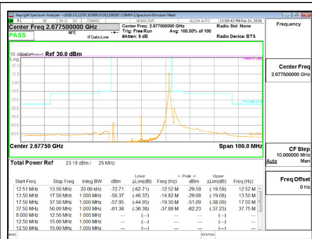
5G NR n41 25MHz BPSK High Channel RB1-63
