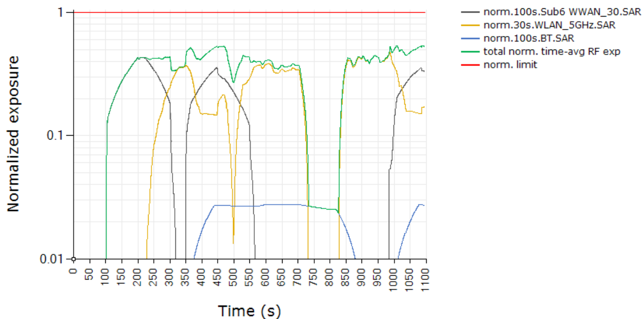
Total Normalized Time-averaged RF Exposure Tech: WLAN, Band 5GHz / Tech: LTE, Band 30 / Tech: BT
