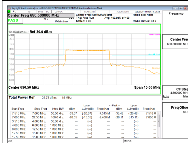
LTE B71 15MHz QPSK Mid Channel RB75-0
