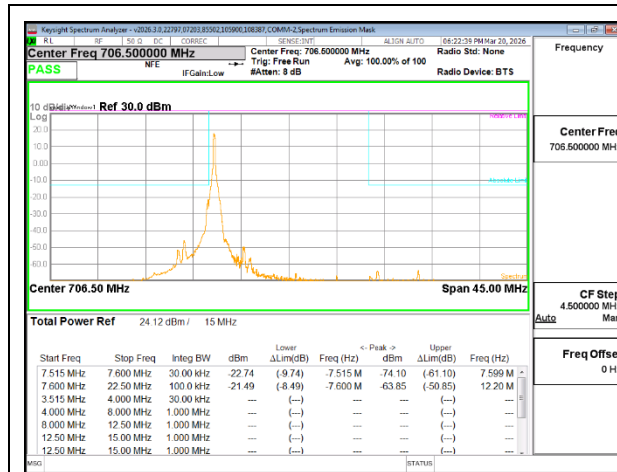
5G NR n12 15MHz BPSK Low Channel RB1-1
