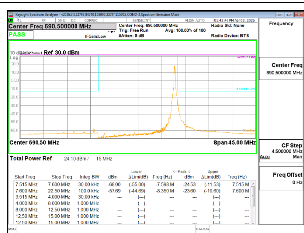
5G NR n71 15MHz BPSK High Channel RB1-77
