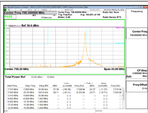
5G NR n12 15MHz BPSK High Channel RB1-77
