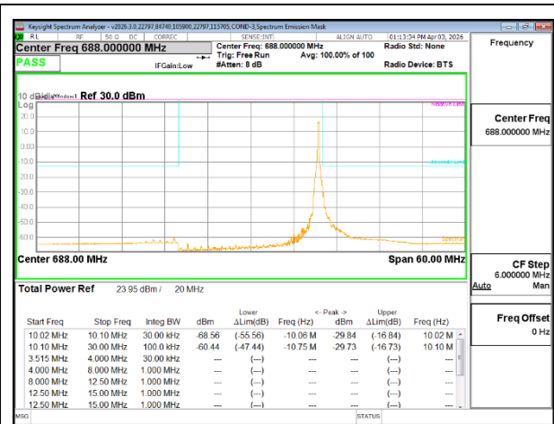
5G NR n71 20MHz BPSK High Channel RB1-104
