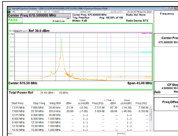
5G NR n71 15MHz BPSK Low Channel RB1-1
