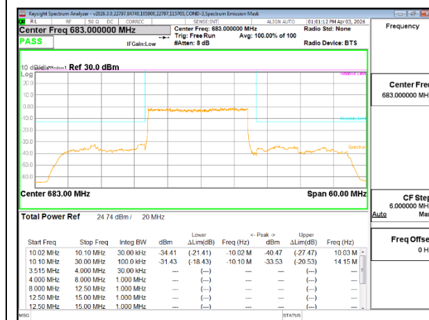
5G NR n71 20MHz BPSK Mid Channel RB100-0
