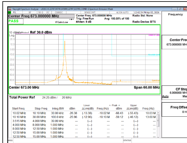
5G NR n71 20MHz BPSK Low Channel RB1-1
