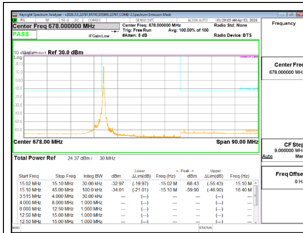
5G NR n71 30MHz BPSK Low Channel RB1-1
