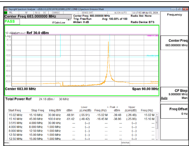
5G NR n71 30MHz BPSK High Channel RB1-158
