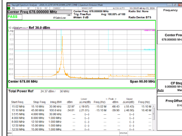
5G NR n71 30MHz BPSK Low Channel RB160-0
