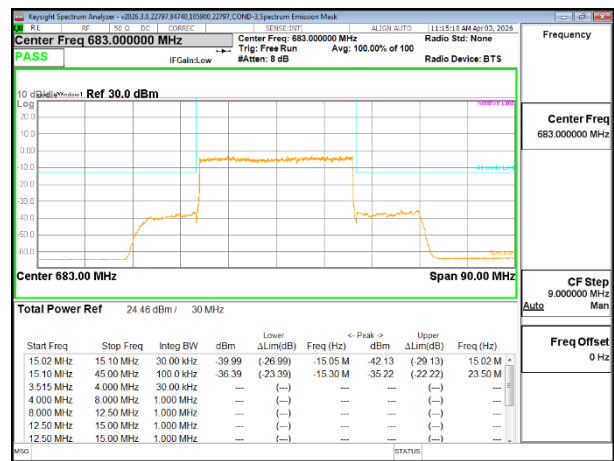
5G NR n71 30MHz BPSK High Channel RB160-0
