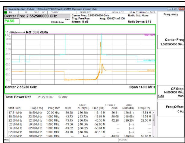
5G NR n7 35MHz BPSK High Channel RB1-186
