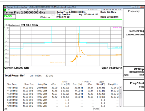
5G NR n7 20MHz BPSK High Channel RB1-104
