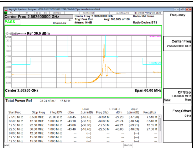
5G NR n7 15MHz BPSK High Channel RB1-77
