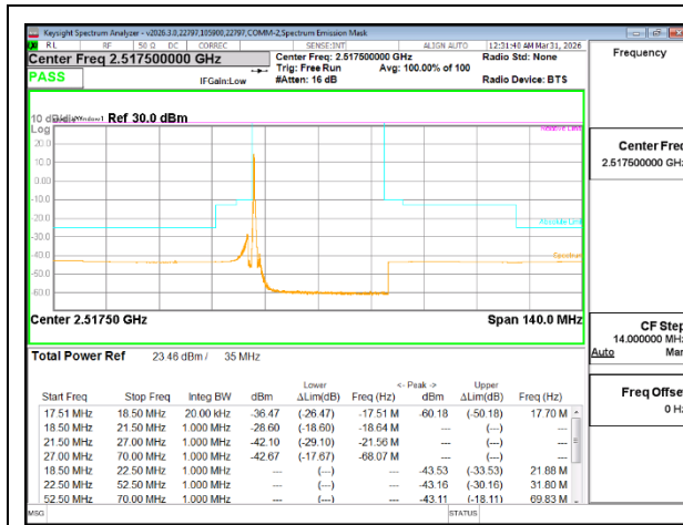
5G NR n7 35MHz BPSK Low Channel RB1-1
