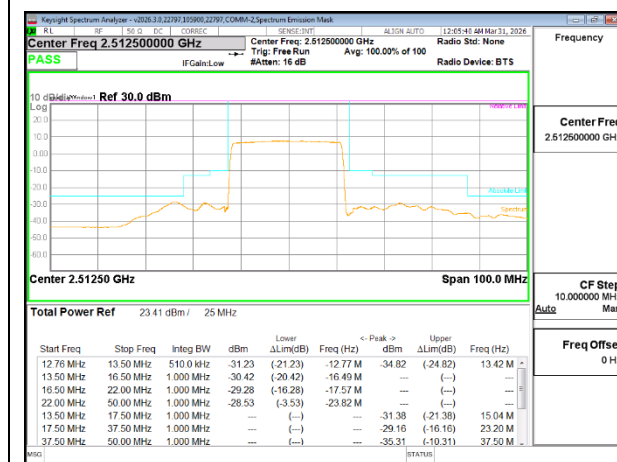
5G NR n7 25MHz BPSK Low Channel RB1-1
