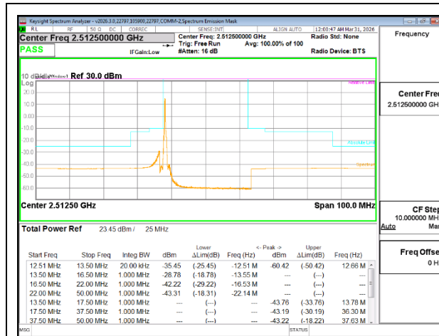
5G NR n7 25MHz BPSK Low Channel RB1-1
