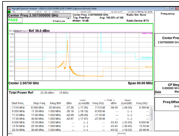
5G NR n7 15MHz BPSK Low Channel RB1-1
