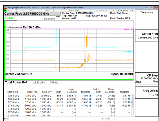
5G NR n7 25MHz BPSK High Channel RB1-131
