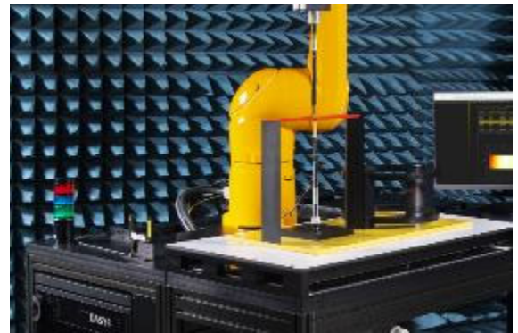
Figure 4.2 DASY8 with Module HAC
