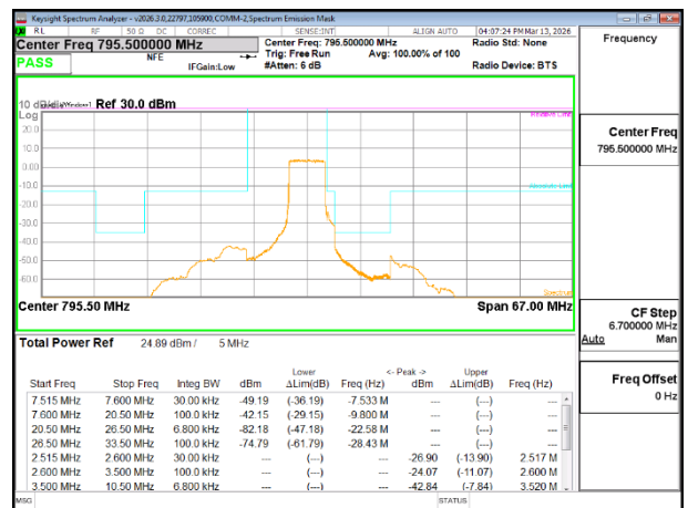
LTE B14 5MHz QPSK High Channel RB25-0
