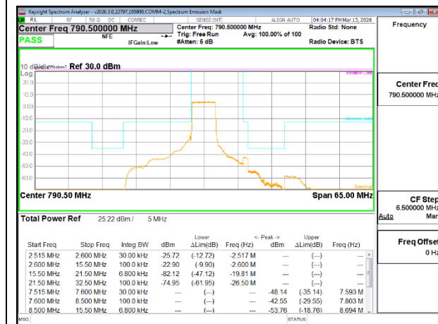
LTE B14 5MHz QPSK Low Channel RB25-0
