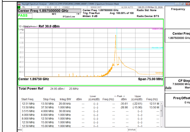
5G NR N2 25MHz QPSK High Channel RB1-132
