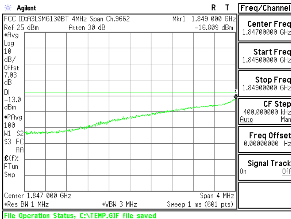
Plot 6-54. 4MHz Span Plot (PCS WCDMA Mode - Ch.9262(DL9662))
