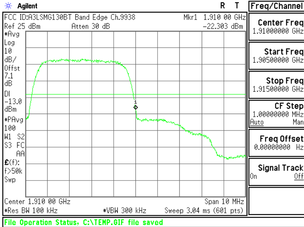
Plot 6-55. Band Edge Plot (PCS WCDMA Mode - Ch.9538(DL9938))
