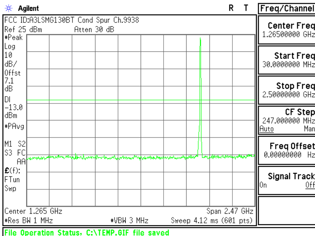
Plot 6-37. Conducted Spurious Plot (PCS WCDMA Mode - Ch.9538(DL9938))
