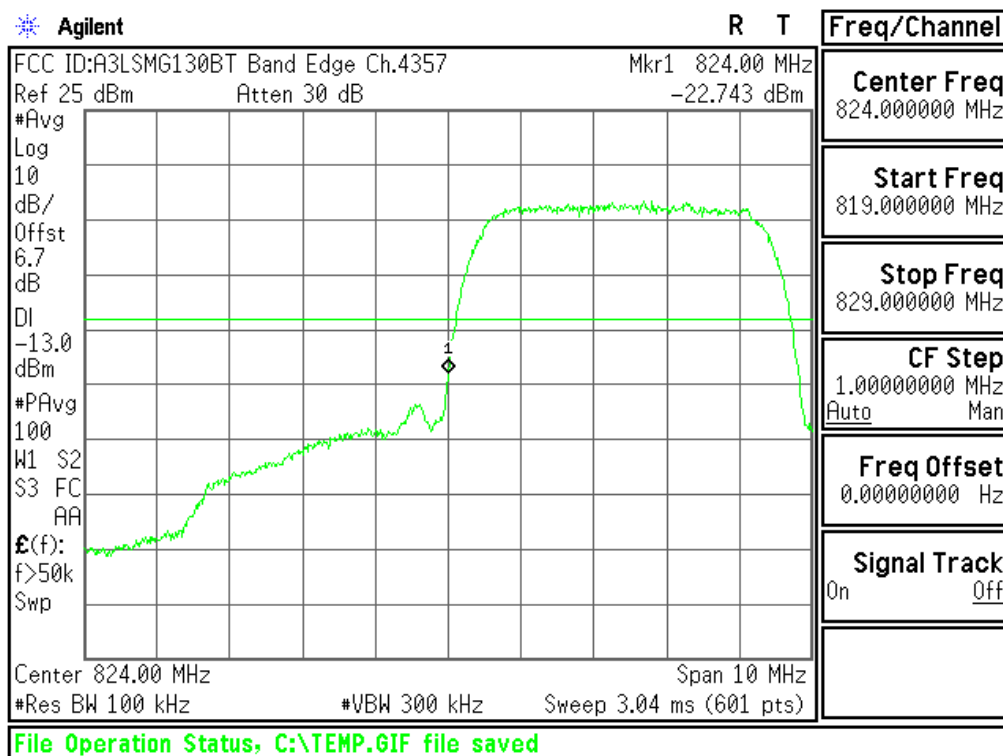
Plot 6-49. Band Edge Plot (Cellular WCDMA Mode - Ch.4132(DL4357))
