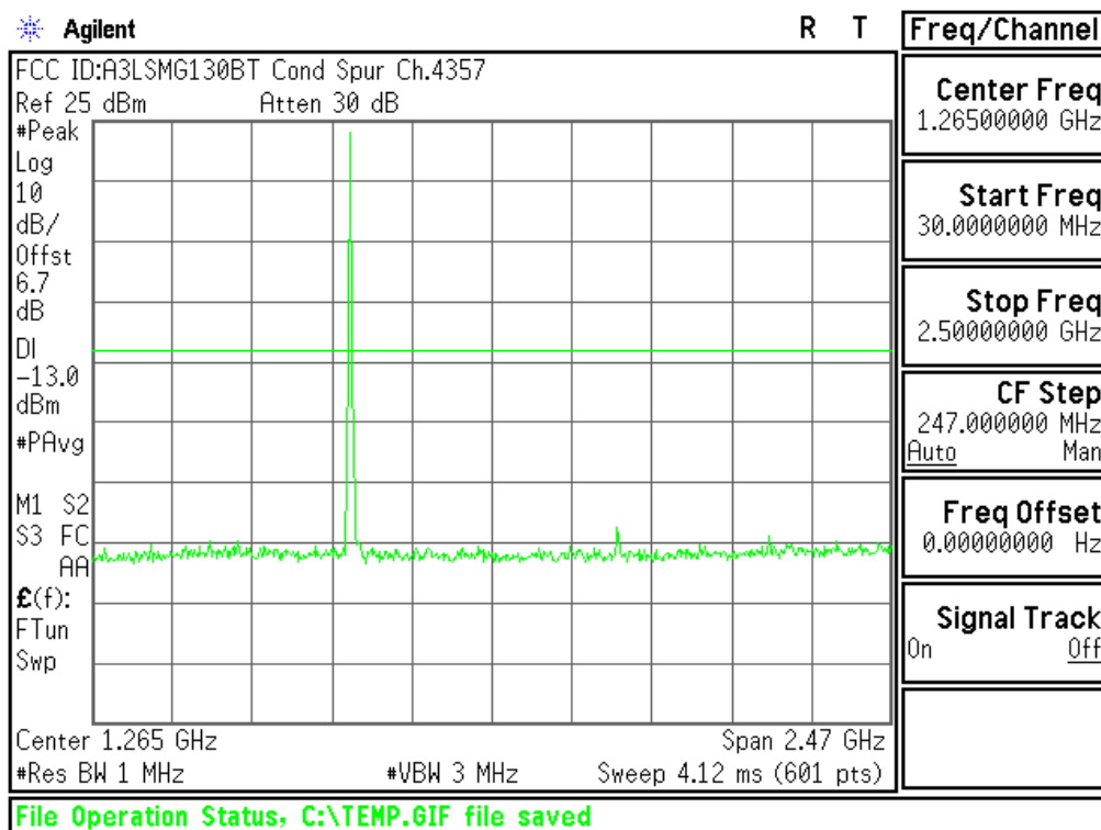
Plot 6-17. Conducted Spurious Plot (Cellular WCDMA Mode - Ch.4132(DL4357))
