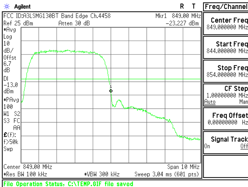
Plot 6-51. Band Edge Plot (Cellular WCDMA Mode - Ch.4233(DL4458))
