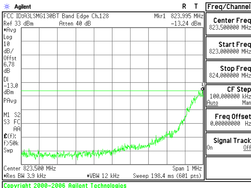
Plot 6-42. Band Edge Plot (Cellular GSM Mode – Ch.128)
