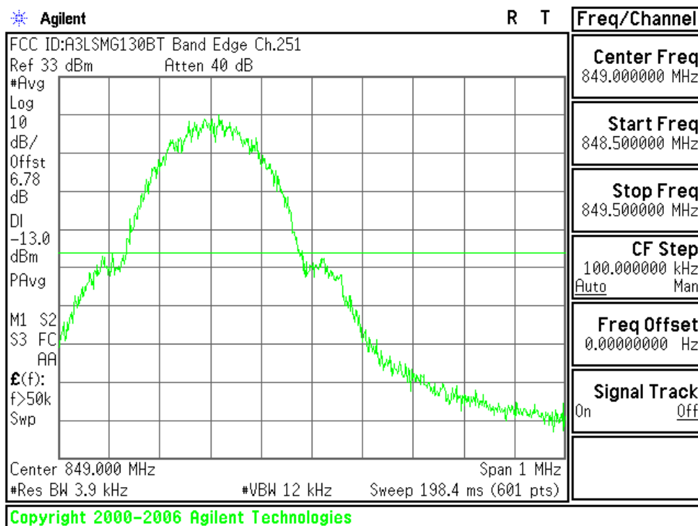
Plot 6-43. Band Edge Plot (Cellular GSM Mode – Ch.251)
