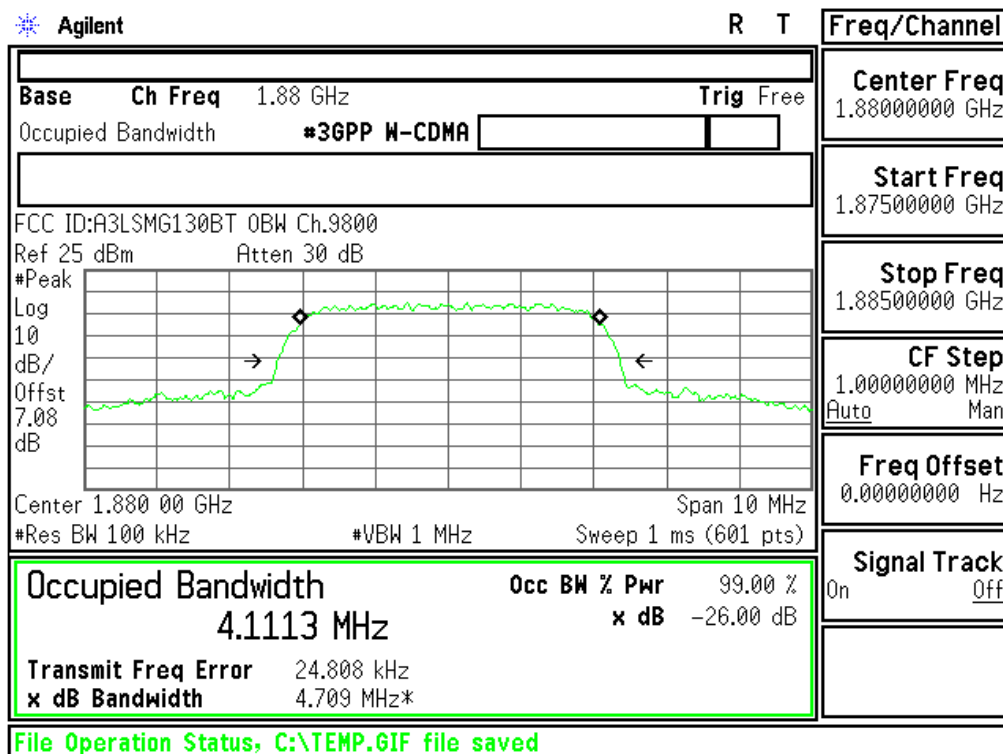
Plot 6-4. Occupied Bandwidth Plot (PCS WCDMA Mode - Ch.9400(DL9800))
