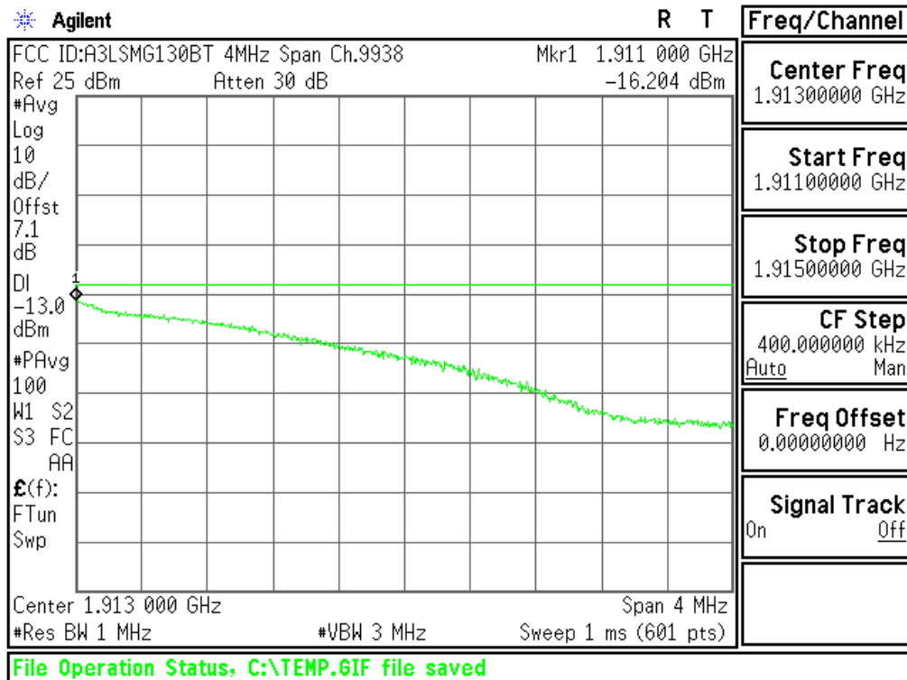
Plot 6-56. 4MHz Span Plot (PCS WCDMA Mode - Ch.9538(DL9938))
