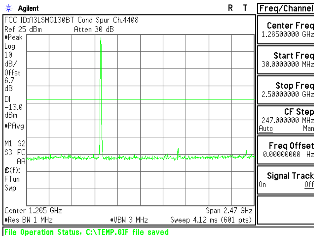
Plot 6-21. Conducted Spurious Plot (Cellular WCDMA Mode - Ch.4183(DL4408))
