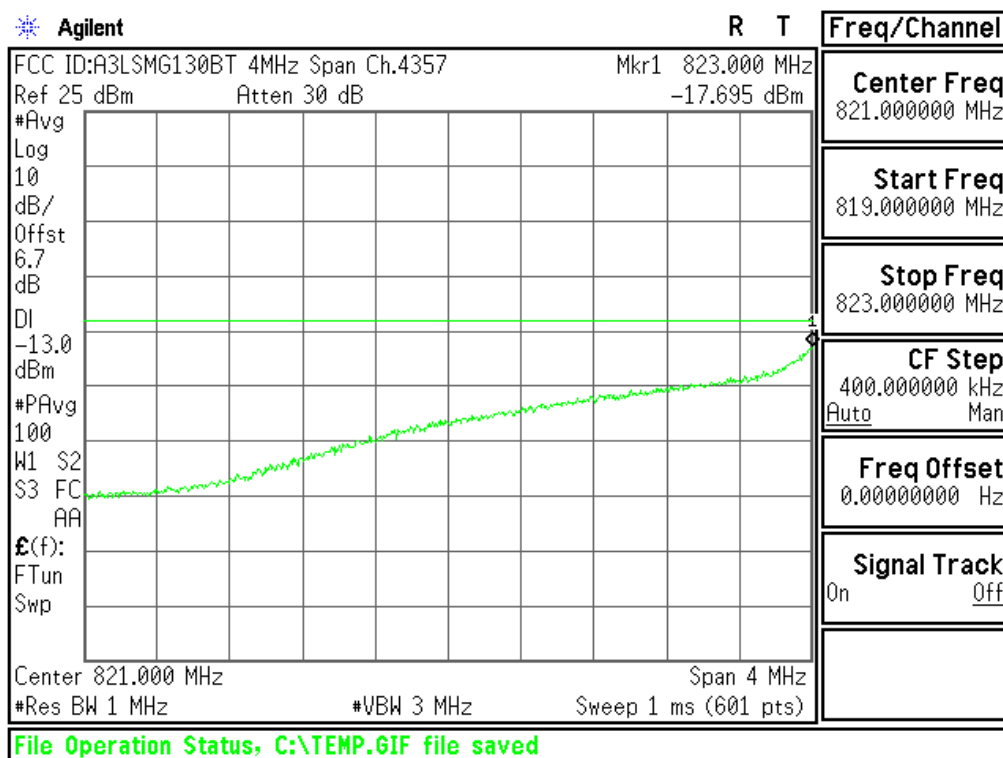
Plot 6-50. 4MHz Span Plot (Cellular WCDMA Mode - Ch.4132(DL4357))
