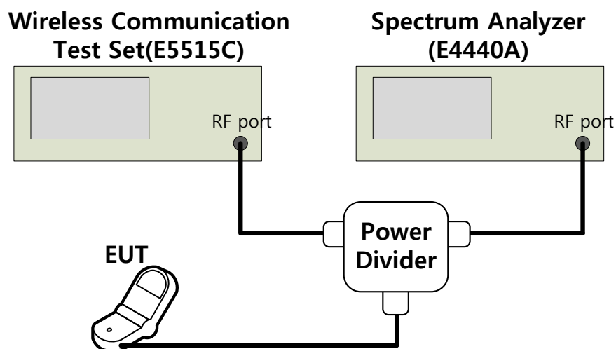
Figure 6-5. Test Instruments & Measurement Setup
