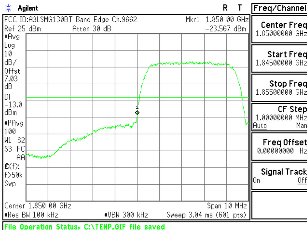
Plot 6-53. Band Edge Plot (PCS WCDMA Mode - Ch.9262(DL9662))
