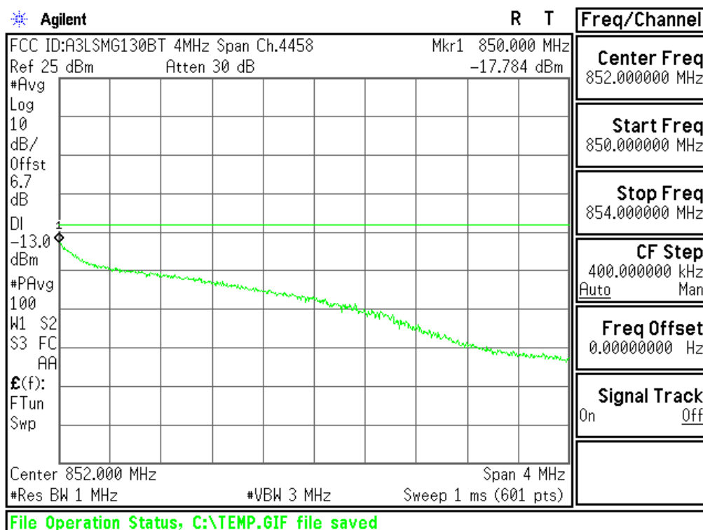
Plot 6-52. 4MHz Span Plot (Cellular WCDMA Mode - Ch.4233(DL4458))
