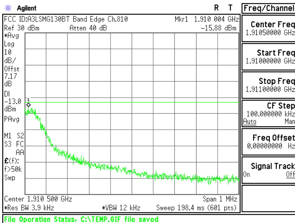
Plot 6-48. Band Edge Plot (PCS GSM Mode – Ch.810)
