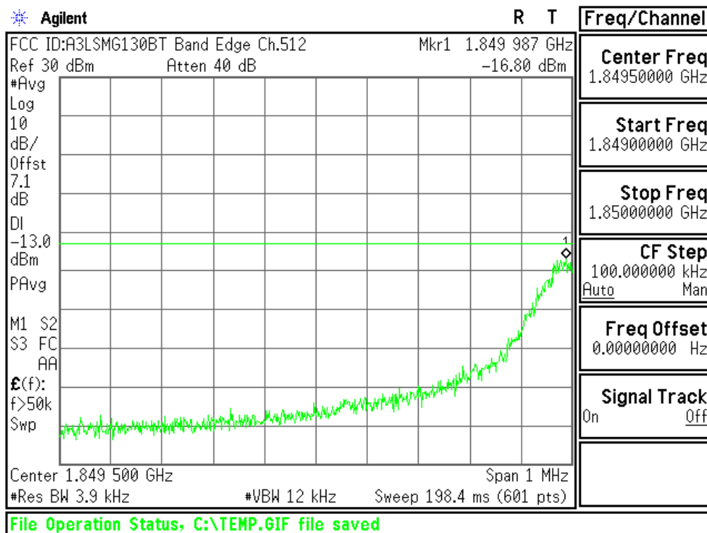
Plot 6-46. Band Edge Plot (PCS GSM Mode – Ch.512)
