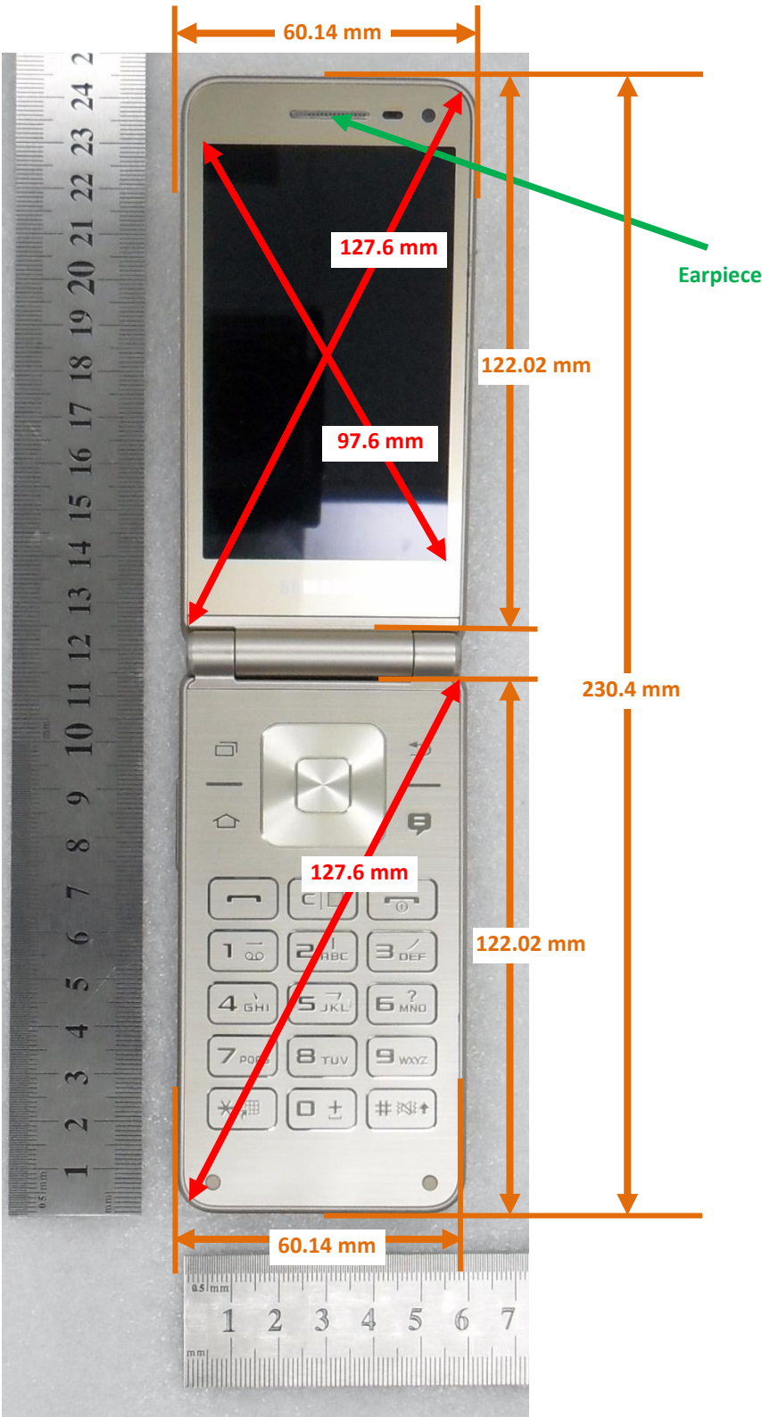
Overall Dimensions 1
