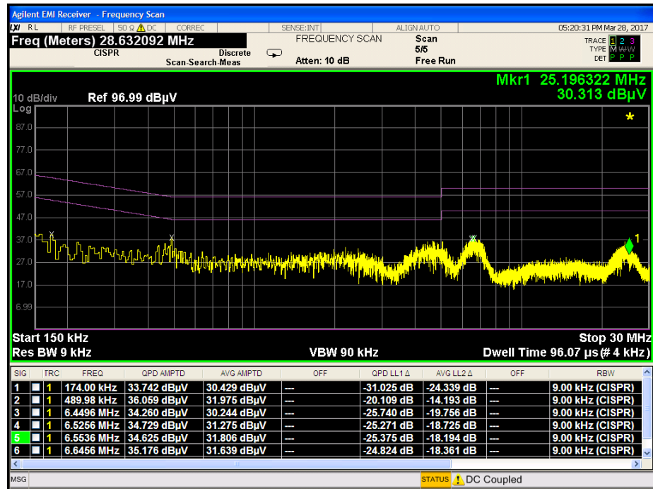
Plot 7-93. Line Conducted Plot with 802.11a UNII Band 2A (L1)
