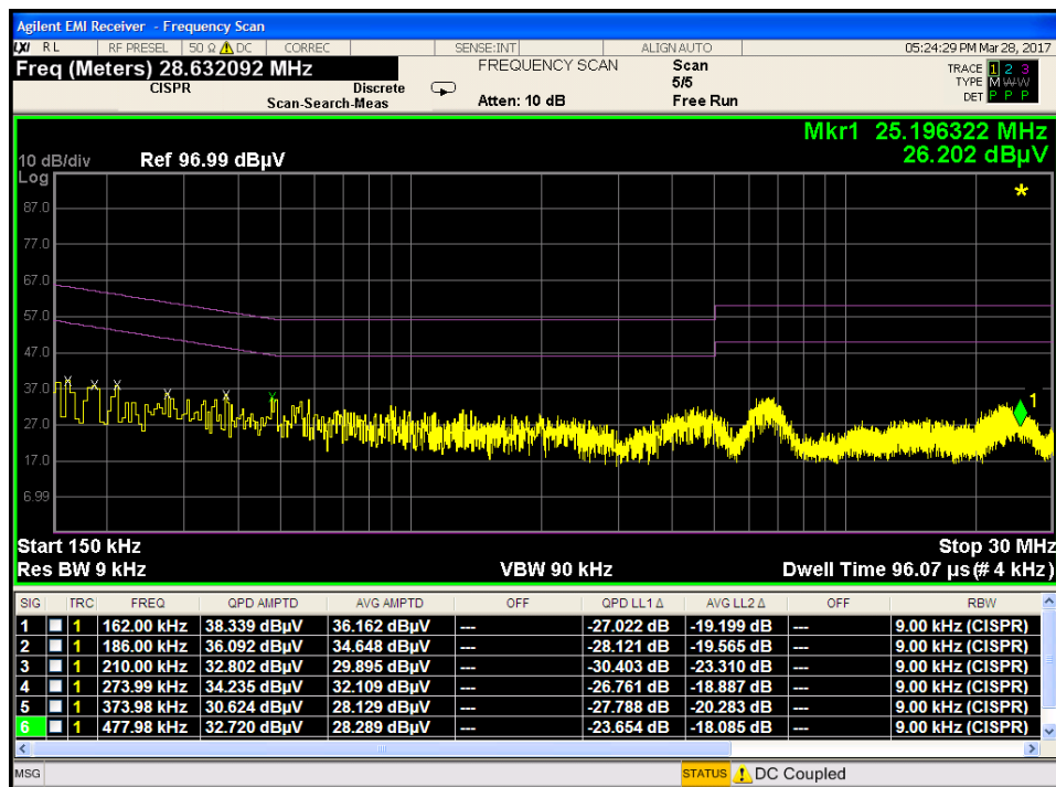
Plot 7-94. Line Conducted Plot with 802.11a UNII Band 2A (N)
