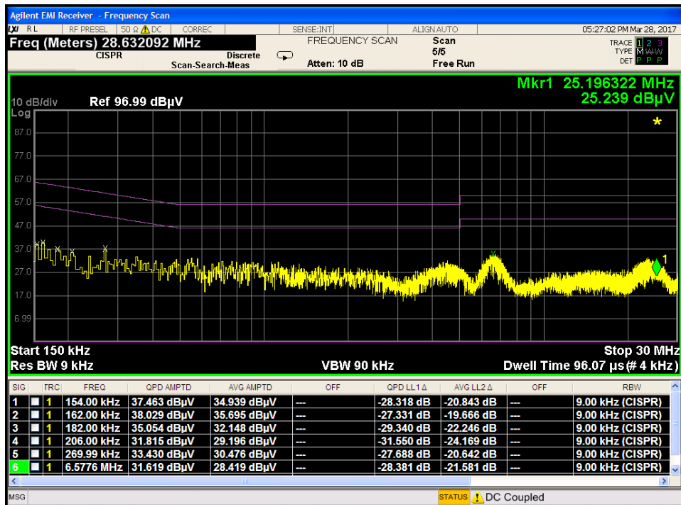
Plot 7-96. Line Conducted Plot with 802.11a UNII Band 2C (N)
