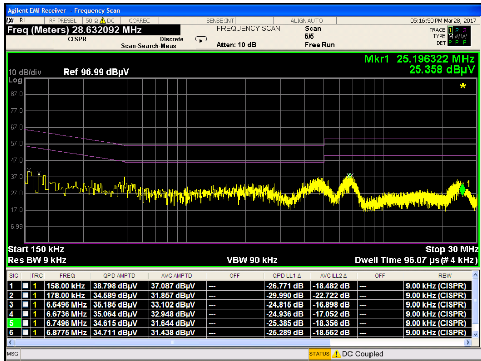
Plot 7-91. Line Conducted Plot with 802.11a UNII Band 1 (L1)
