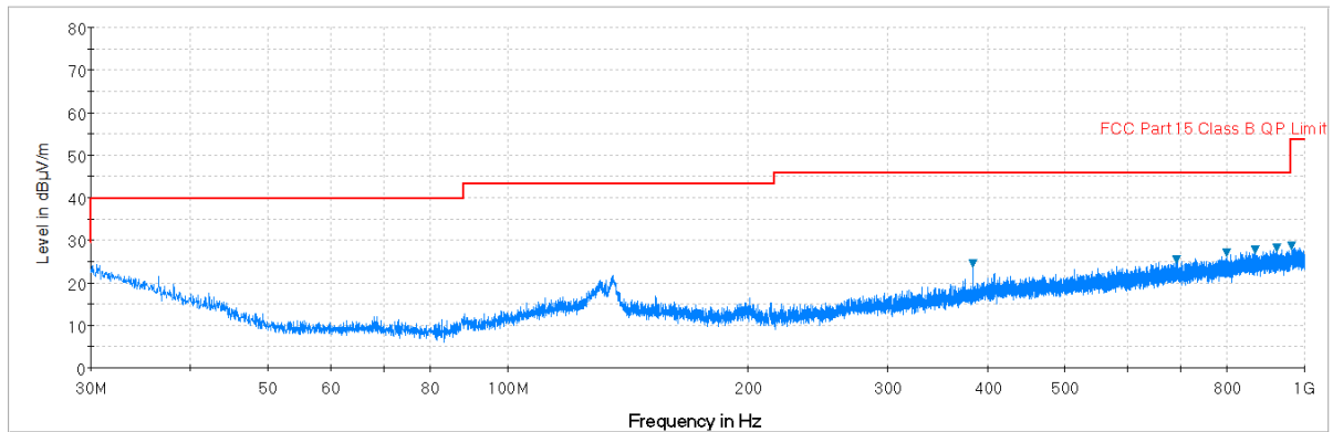
Plot 7-90. Radiated Spurious Plot below 1GHz (802.11a – U3 Ch. 157, Ant. Pol. V)
