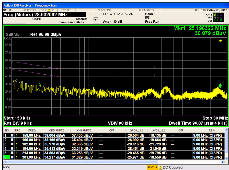
Plot 7-92. Line Conducted Plot with 802.11a UNII Band 1 (N)
