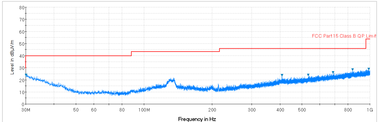
Plot 7-89. Radiated Spurious Plot below 1GHz (802.11a – U3 Ch. 157, Ant. Pol. H)
