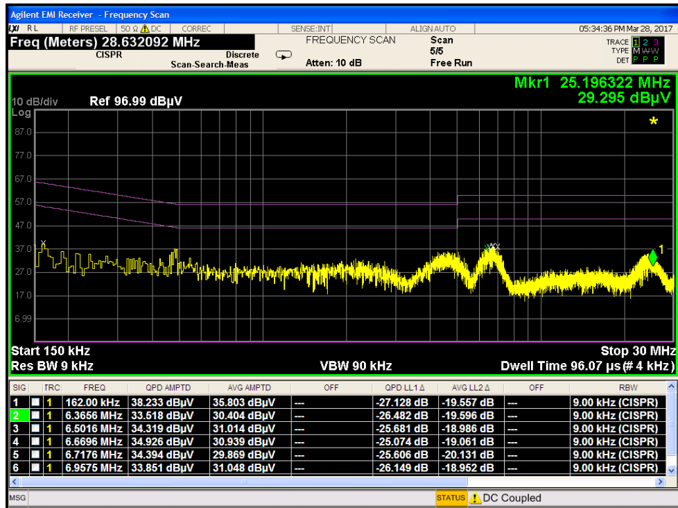
Plot 7-97. Line Conducted Plot with 802.11a UNII Band 3 (L1)
