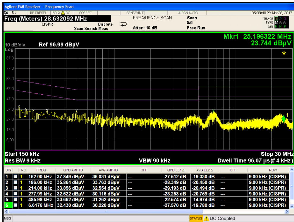
Plot 7-98. Line Conducted Plot with 802.11a UNII Band 3 (N)
