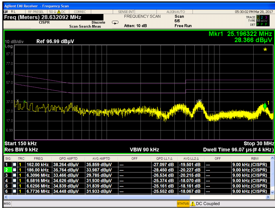
Plot 7-95. Line Conducted Plot with 802.11a UNII Band 2C (L1)
