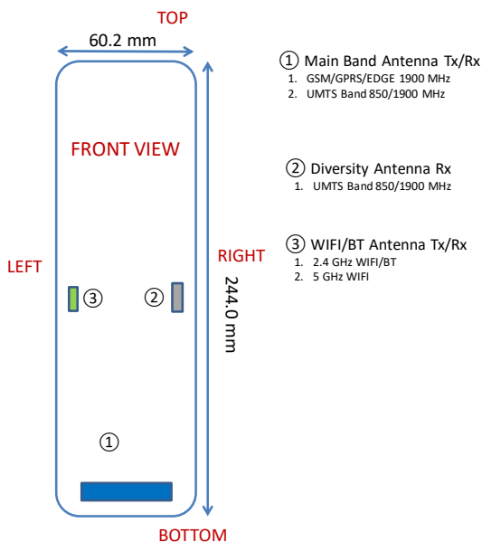
Figure F-2 DUT Closed Antenna Locations
