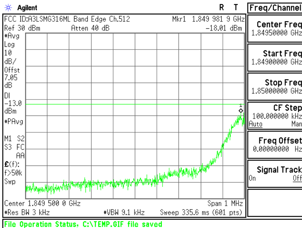
Plot 6-58. Lower Band Edge Plot (PCS GSM Mode – Ch.512)
