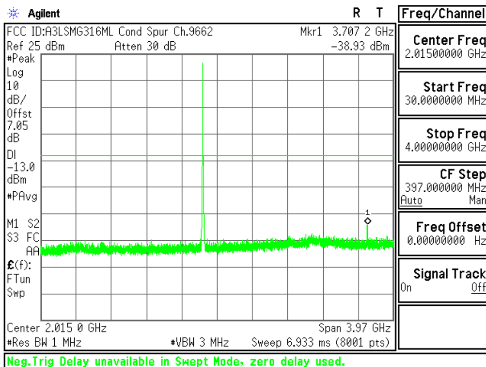
Plot 6-38. Conducted Spurious Plot (PCS WCDMA Mode - Ch.9262(DL9662))
