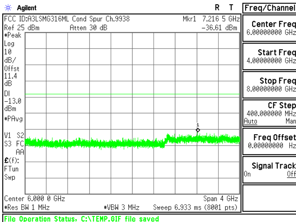
Plot 6-49. Conducted Spurious Plot (PCS WCDMA Mode - Ch.9538(DL9938))
