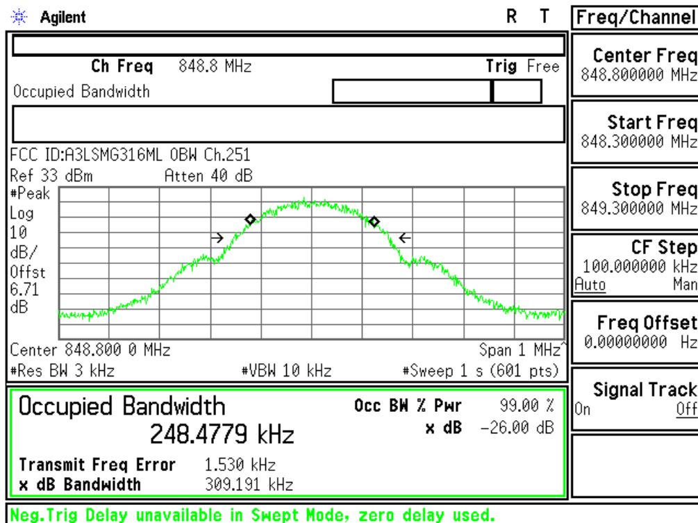
Plot 6-1. Occupied Bandwidth Plot (Cellular GSM Mode - Ch.251)
