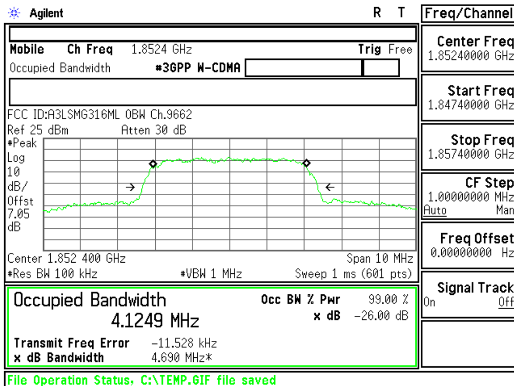
Plot 6-4. Occupied Bandwidth Plot (PCS WCDMA Mode - Ch.9262(DL9662))
