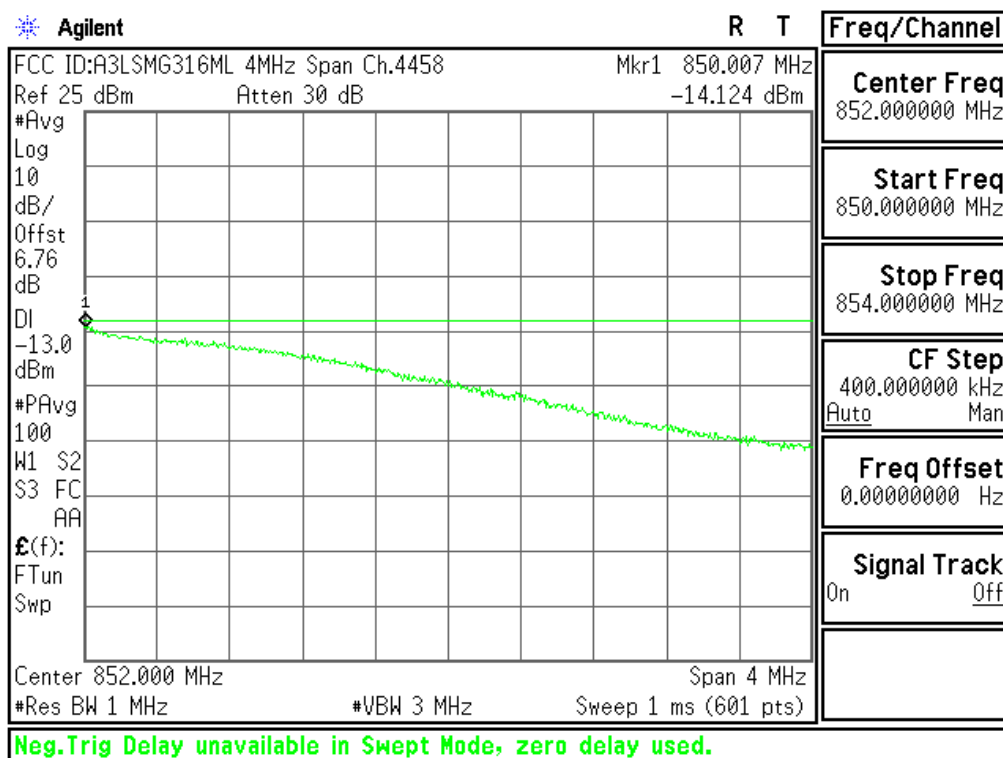
Plot 6-64. Extended Upper Band Edge Plot (Cellular WCDMA Mode - Ch.4233(DL4458))
