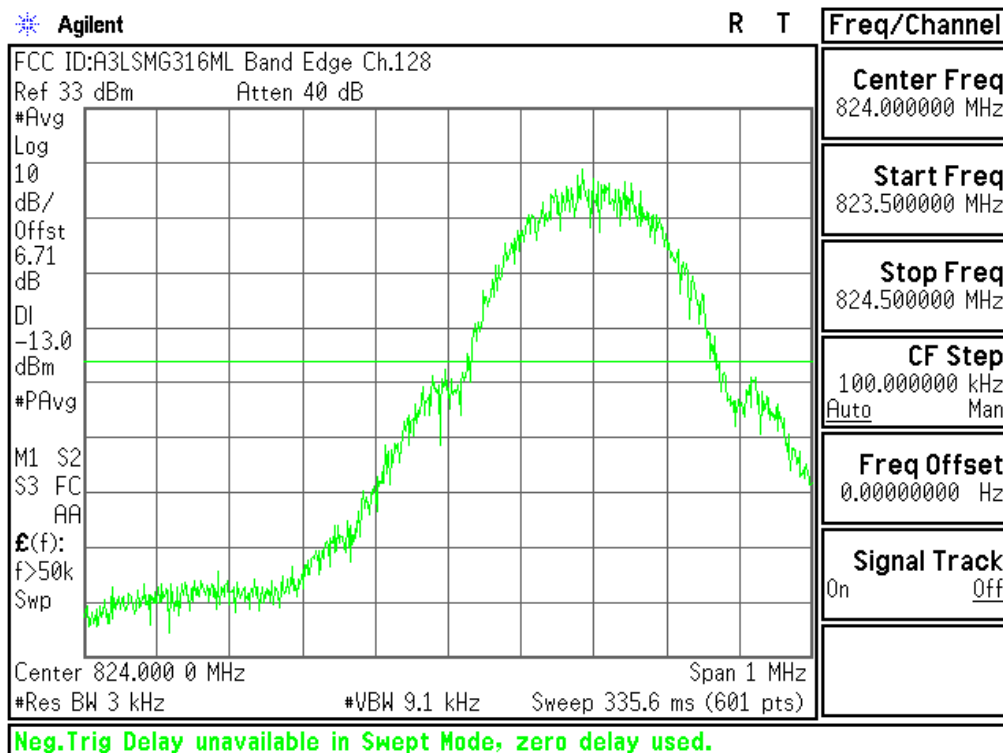
Plot 6-53. Lower Band Edge Plot (Cellular GSM Mode – Ch.128)
