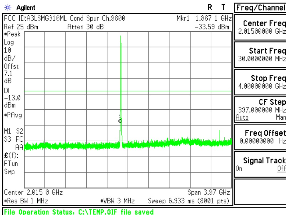
Plot 6-43. Conducted Spurious Plot (PCS WCDMA Mode - Ch.9400(DL9800))
