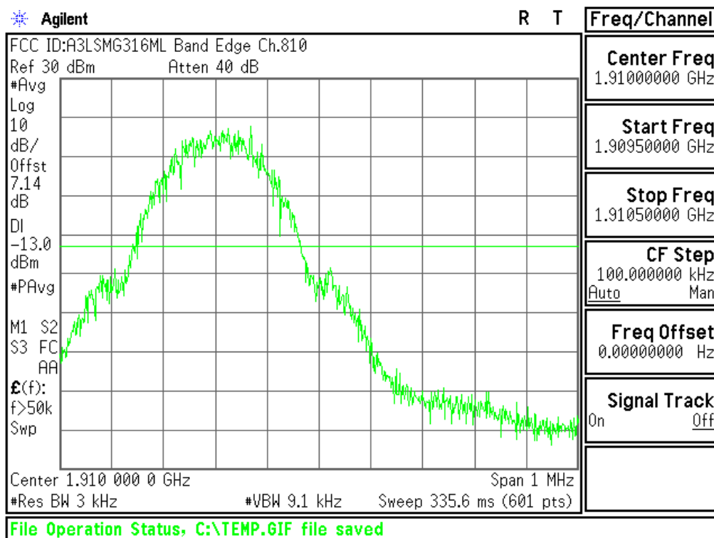
Plot 6-59. Upper Band Edge Plot (PCS GSM Mode – Ch.810)
