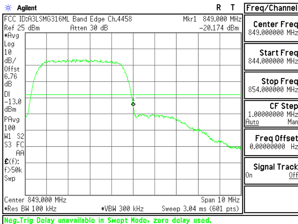
Plot 6-63. Upper Band Edge Plot (Cellular WCDMA Mode - Ch.4233(DL4458))
