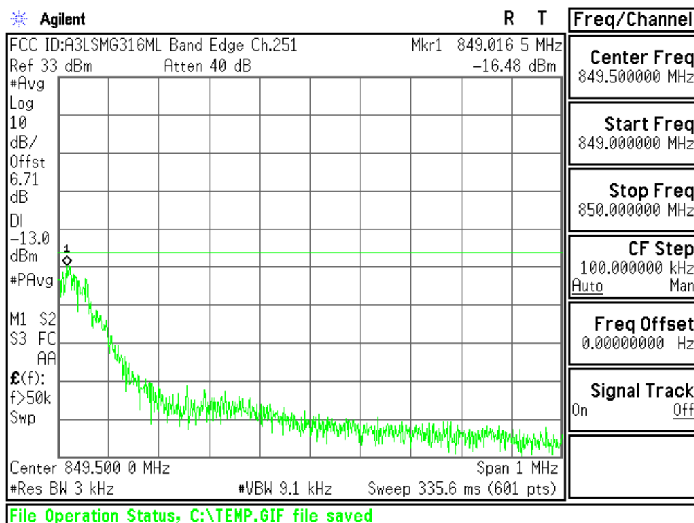
Plot 6-56. Upper Band Edge Plot (Cellular GSM Mode – Ch.251)
