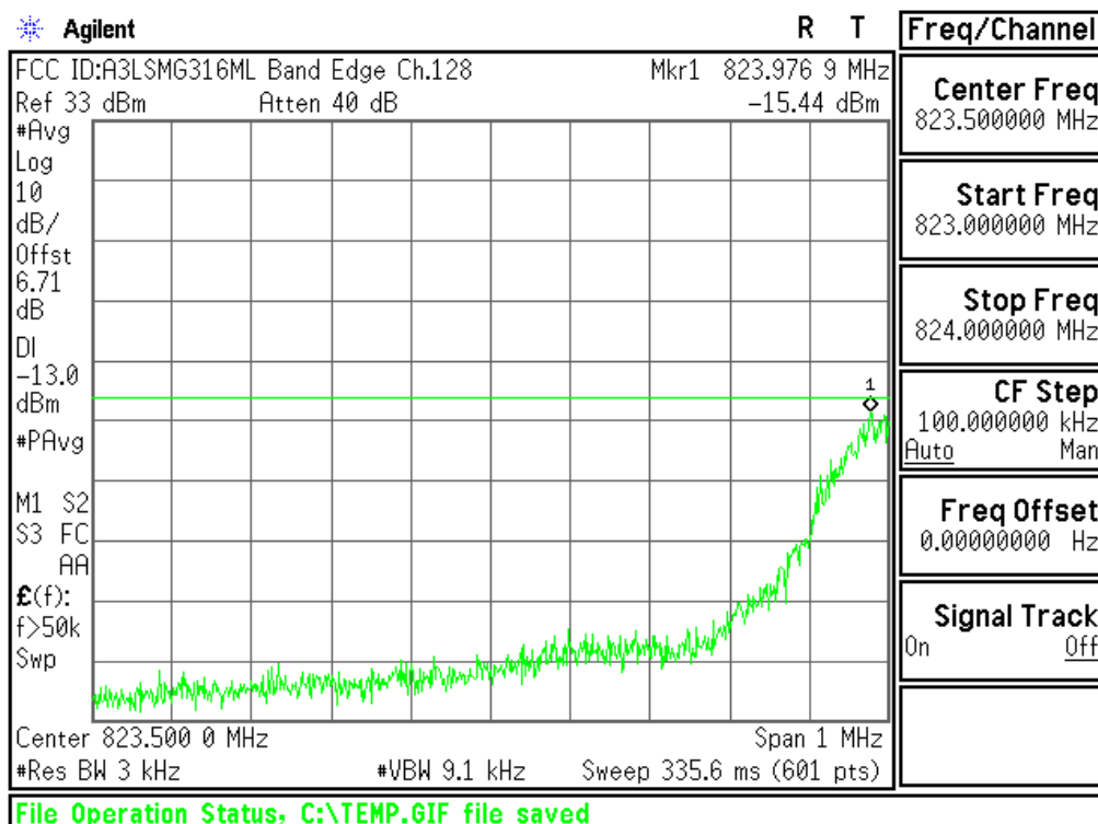
Plot 6-54. Lower Band Edge Plot (Cellular GSM Mode – Ch.128)
