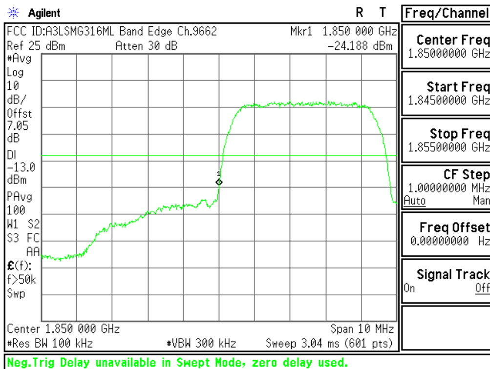
Plot 6-65. Lower Band Edge Plot (PCS WCDMA Mode - Ch.9262(DL9662))
