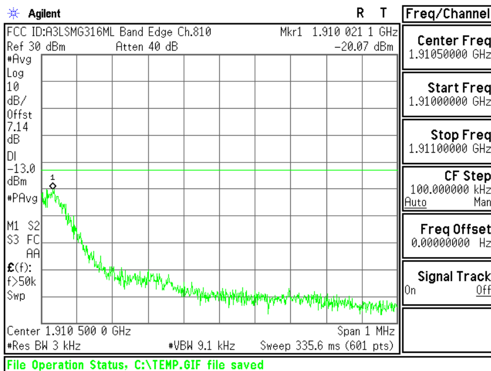
Plot 6-60. Upper Band Edge Plot (PCS GSM Mode – Ch.810)
