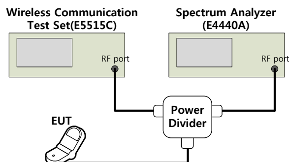
Figure 6-4. Test Instruments & Measurement Setup
