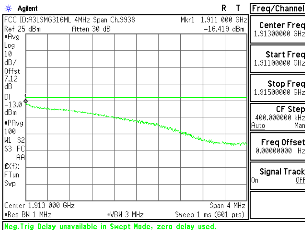
Plot 6-68. Extended Upper Band Edge Plot (PCS WCDMA Mode - Ch.9538(DL9938))
