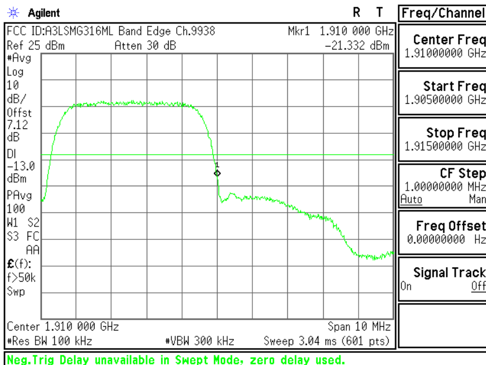
Plot 6-67. Upper Band Edge Plot (PCS WCDMA Mode - Ch.9538(DL9938))
