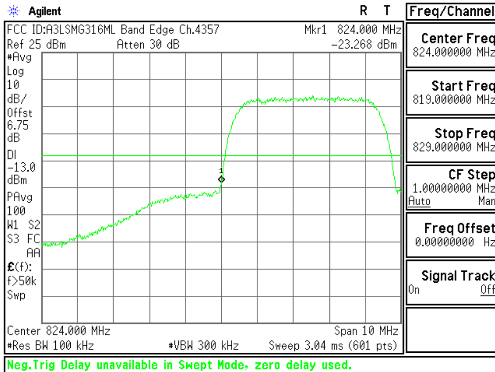
Plot 6-61. Lower Band Edge Plot (Cellular WCDMA Mode - Ch.4132(DL4357))
