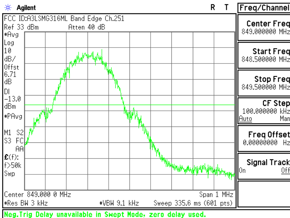
Plot 6-55. Upper Band Edge Plot (Cellular GSM Mode – Ch.251)
