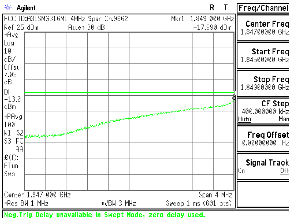
Plot 6-66. Extended Lower Band Edge Plot (PCS WCDMA Mode - Ch.9262(DL9662))
