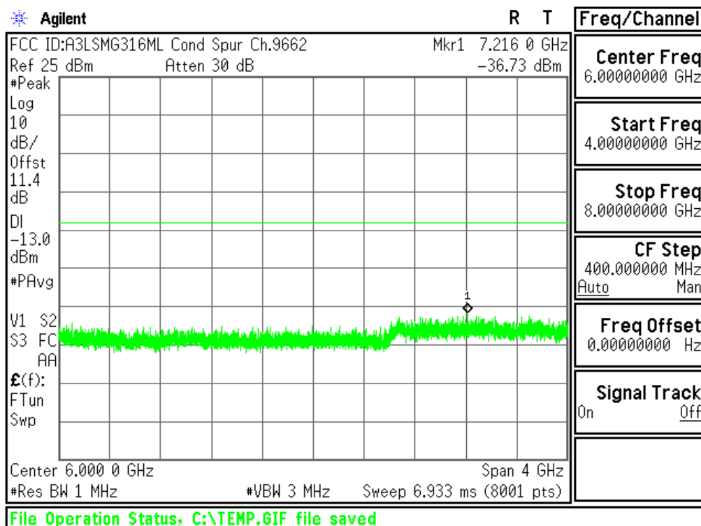
Plot 6-39. Conducted Spurious Plot (PCS WCDMA Mode - Ch.9262(DL9662))
