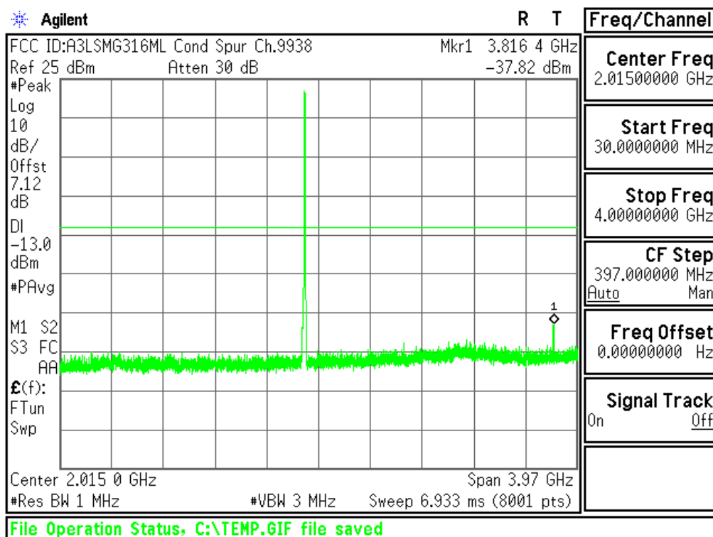
Plot 6-48. Conducted Spurious Plot (PCS WCDMA Mode - Ch.9538(DL9938))
