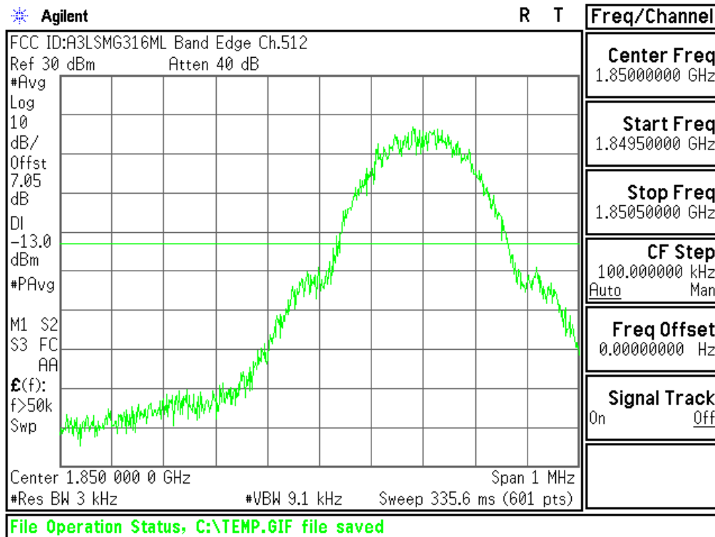
Plot 6-57. Lower Band Edge Plot (PCS GSM Mode – Ch.512)
