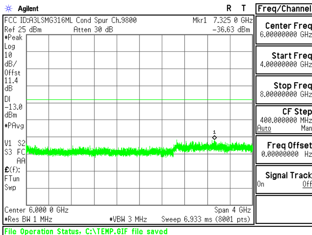
Plot 6-44. Conducted Spurious Plot (PCS WCDMA Mode - Ch.9400(DL9800))
