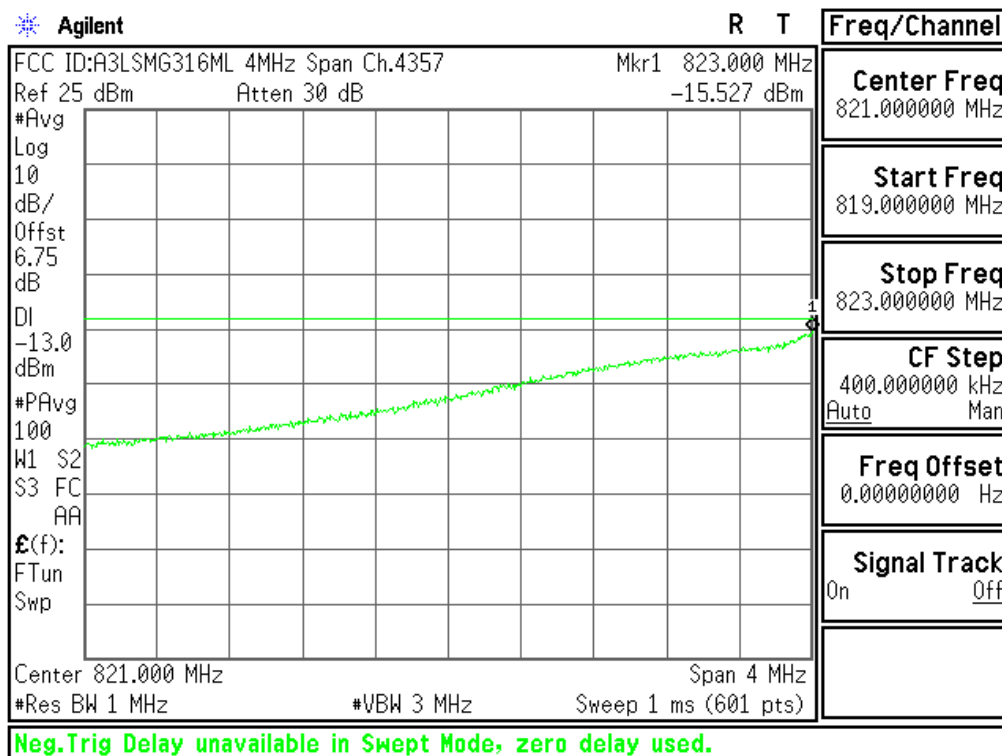
Plot 6-62. Extended Lower Band Edge Plot (Cellular WCDMA Mode - Ch.4132(DL4357))
