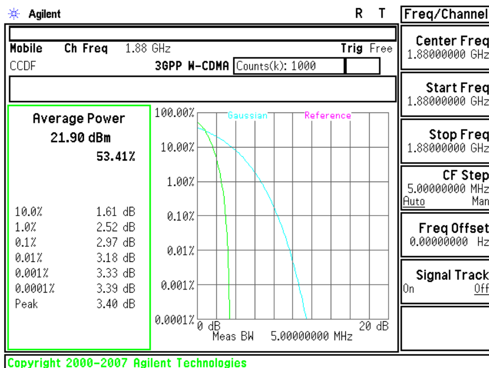
Plot 6-70. Peak-Average Ratio Plot (PCS WCDMA Mode - Ch.9400(DL9800))
