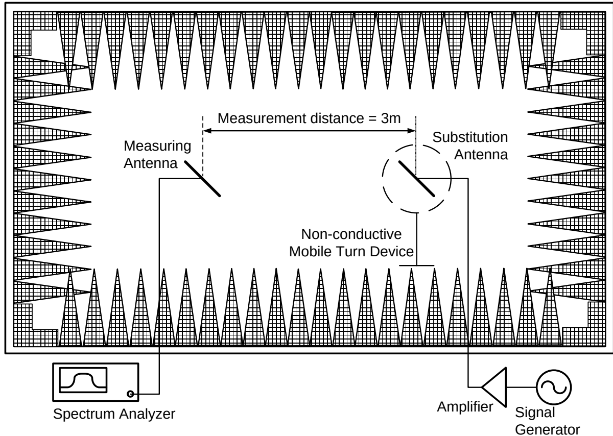
Figure 6-7. Test Instruments & Measurement Setup
