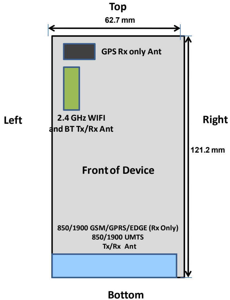
Figure 1-1 DUT Antenna Locations
