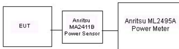
Figure 8-2 Power Measurement Setup
