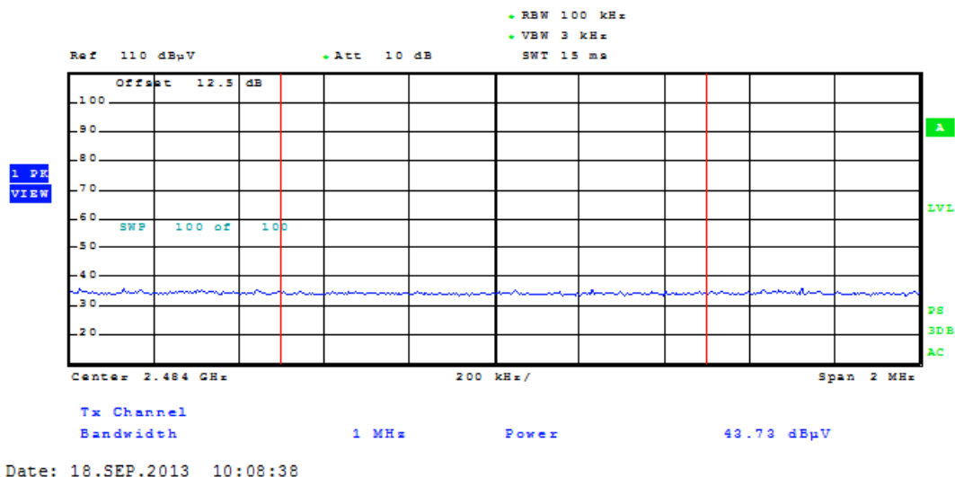
Plot 6-18. Radiated Restricted Upper Band Edge Measurement (Average)
