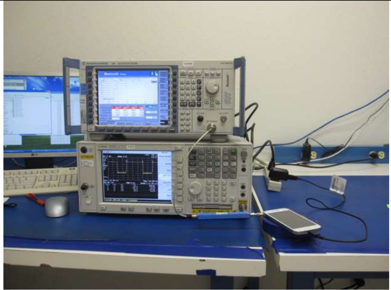
ANTENNA PORT CONDUCTED PHOTO
