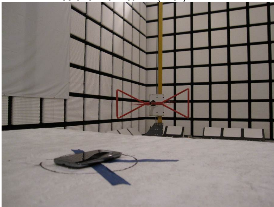
RADIATED EMISSIONS ABOVE 30 MHz (BACK)
