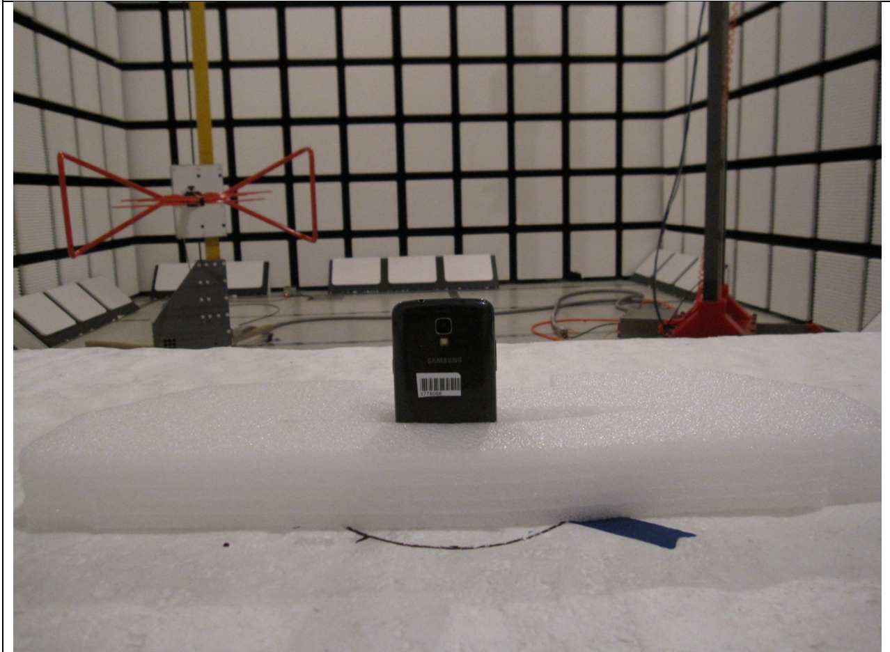
Z-AXIS BACK PHOTO
