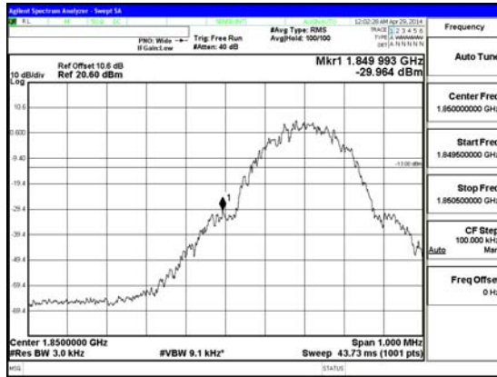
Band GSM1900 GPRS CBE Low channel
