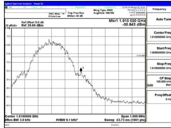
Band GSM1900 GPRS CBE High channel
