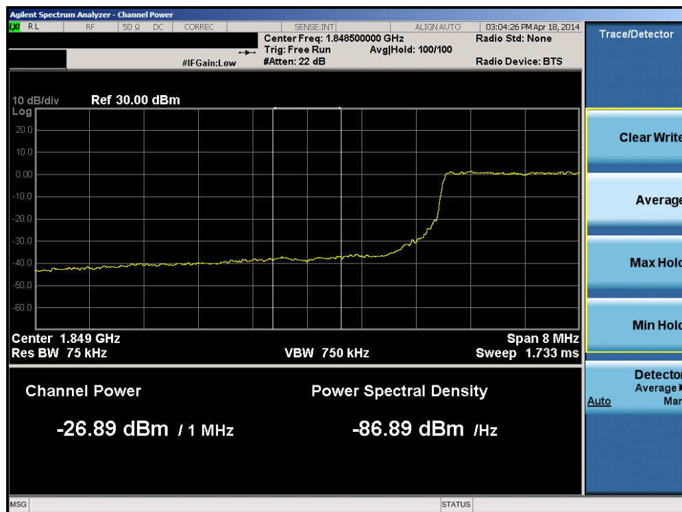
Plot 6-196. Lower Extended Band Edge Plot (Band 2 – 10.0MHz QPSK – RB Size 50)
