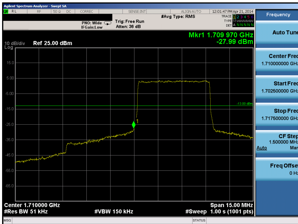
Plot 6-167. Lower Band Edge Plot (Band 4 – 5.0MHz QPSK – RB Size 25)
