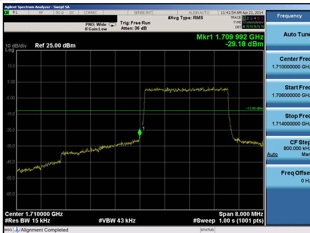
Plot 6-163. Lower Band Edge Plot (Band 4 – 3.0MHz QPSK – RB Size 15)
