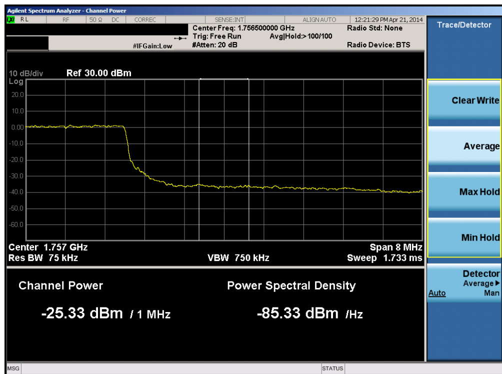
Plot 6-174. Upper Extended Band Edge Plot (Band 4 – 10.0MHz QPSK – RB Size 50)
