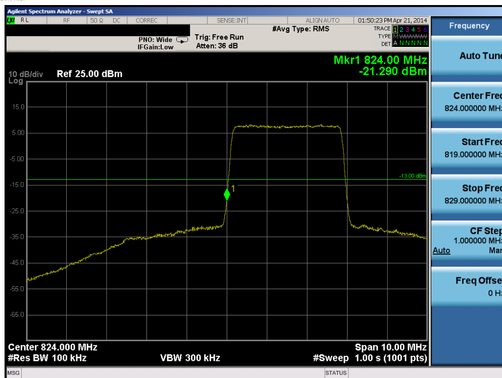
Plot 6-153. Lower Band Edge Plot (Band 5 – 3.0MHz QPSK – RB Size 15)
