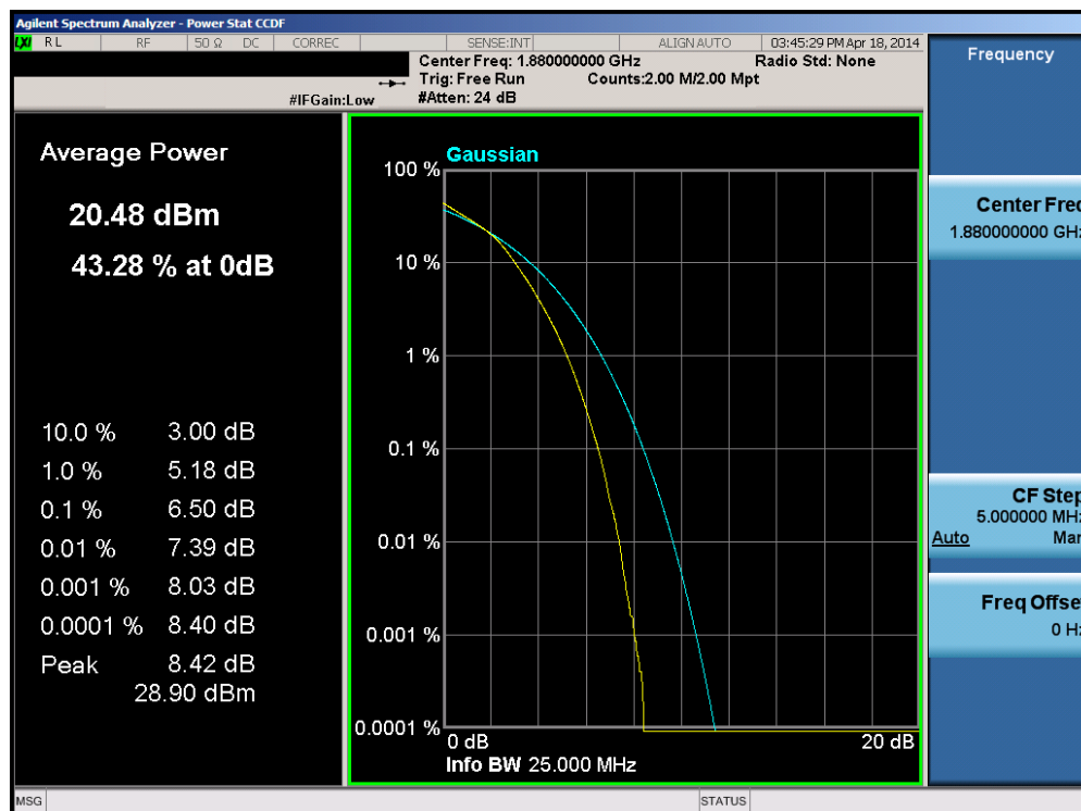
Plot 6-230. PAR Plot (Band 2 – 20.0MHz 16-QAM – RB Size 100)
