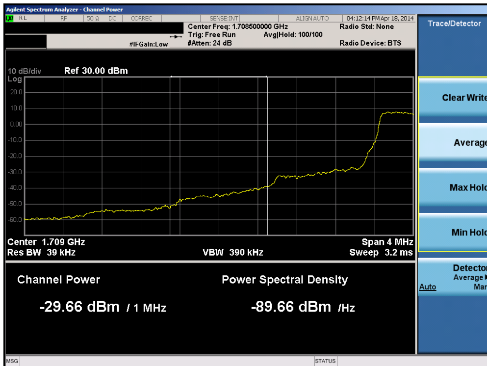
Plot 6-160. Lower Extended Band Edge Plot (Band 4 – 1.4MHz QPSK – RB Size 6)
