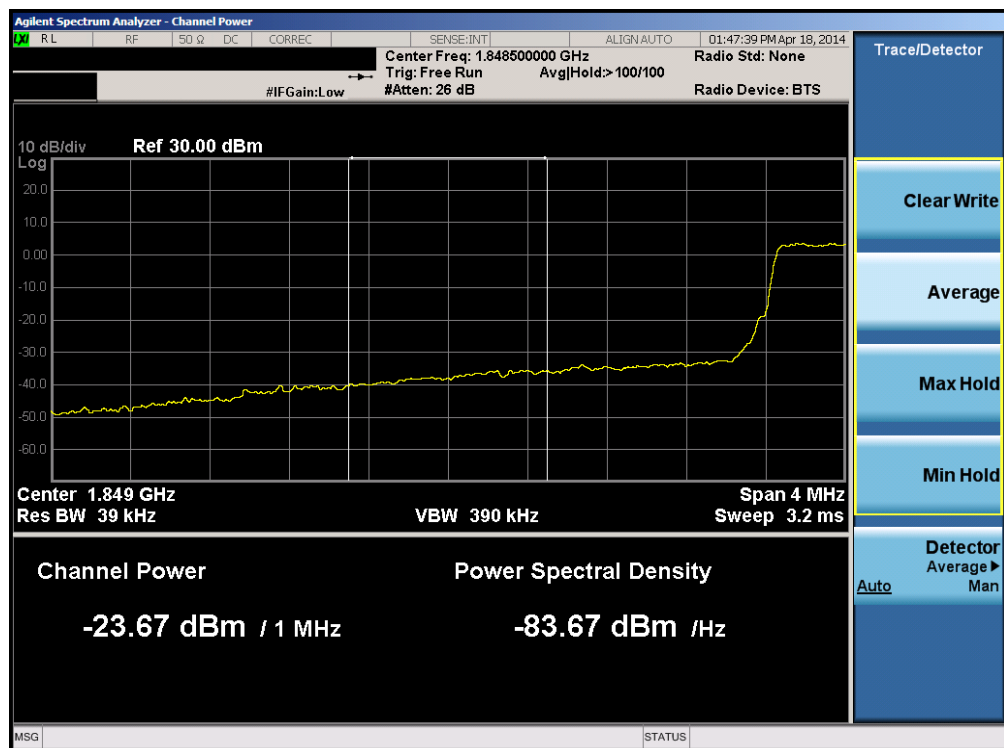
Plot 6-188. Lower Extended Band Edge Plot (Band 2 – 3.0MHz QPSK – RB Size 15)
