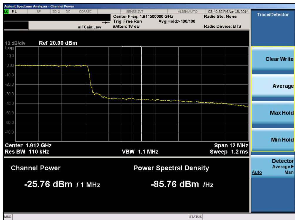
Plot 6-202. Upper Extended Band Edge Plot (Band 2 – 15.0MHz QPSK – RB Size 75)
