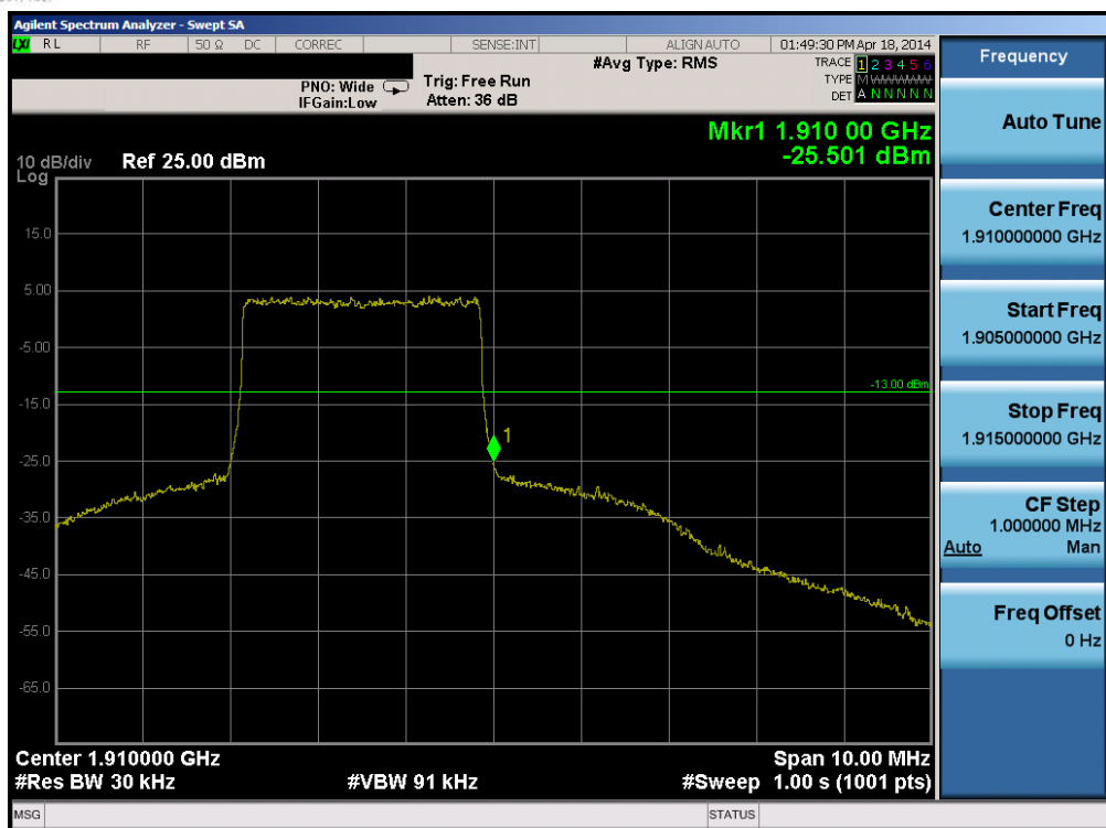
Plot 6-189. Upper Band Edge Plot (Band 2 – 3.0MHz QPSK – RB Size 15)
