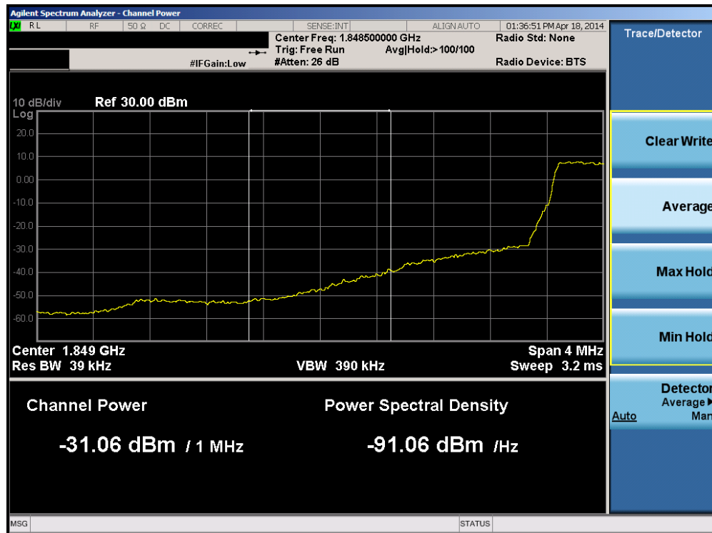
Plot 6-184. Lower Extended Band Edge Plot (Band 2 – 1.4MHz QPSK – RB Size 6)
