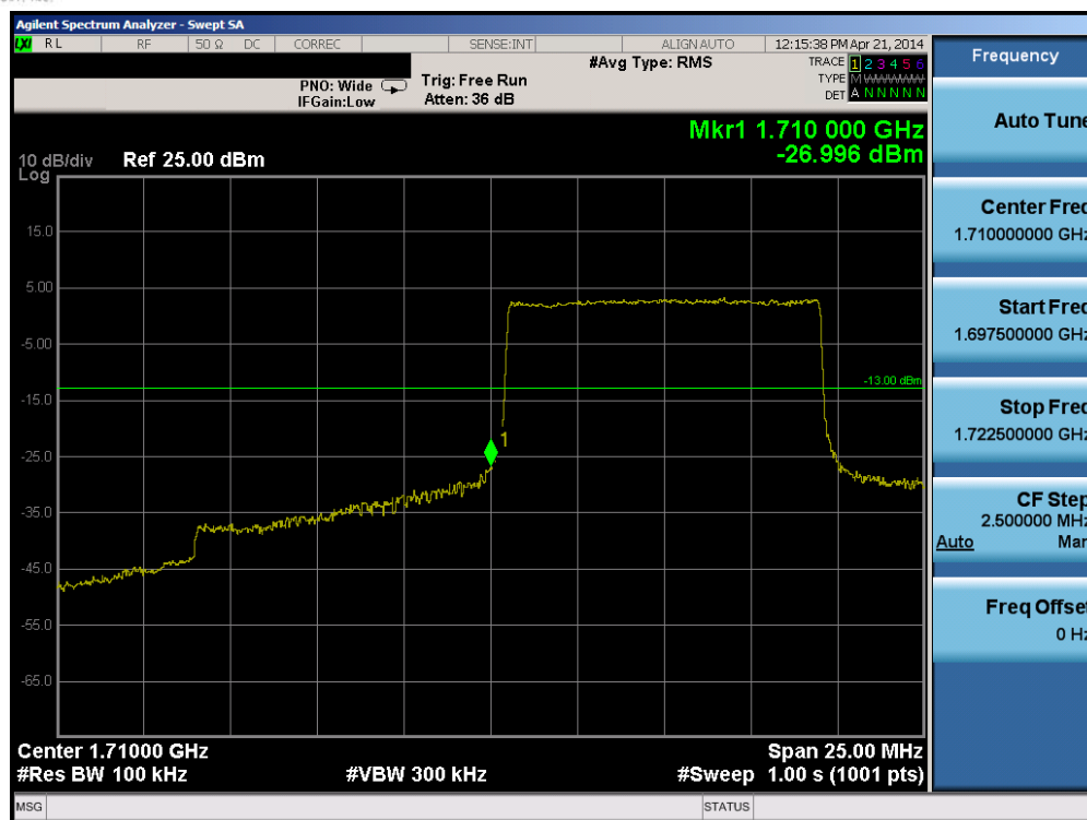
Plot 6-171. Lower Band Edge Plot (Band 4 – 10.0MHz QPSK – RB Size 50)
