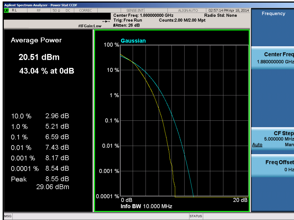
Plot 6-226. PAR Plot (Band 2 – 10.0MHz 16-QAM – RB Size 50)
