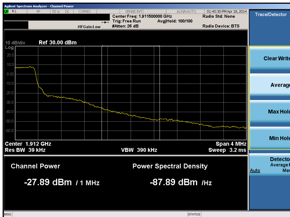
Plot 6-186. Upper Extended Band Edge Plot (Band 2 – 1.4MHz QPSK – RB Size 6)
