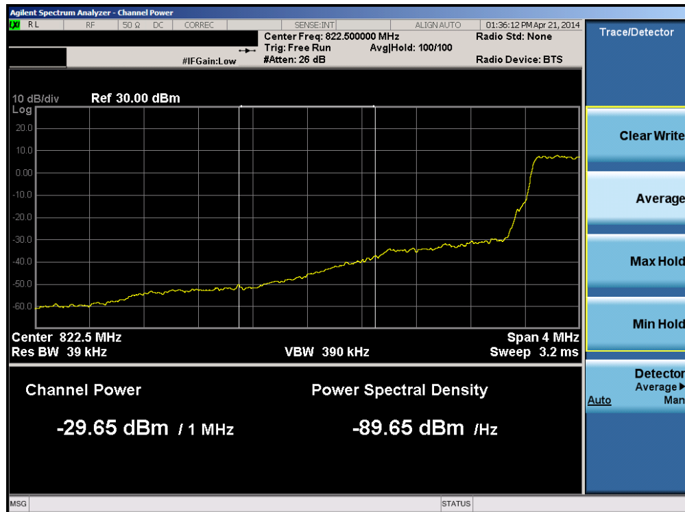
Plot 6-150. Lower Extended Band Edge Plot (Band 5 – 1.4MHz QPSK – RB Size 6)
