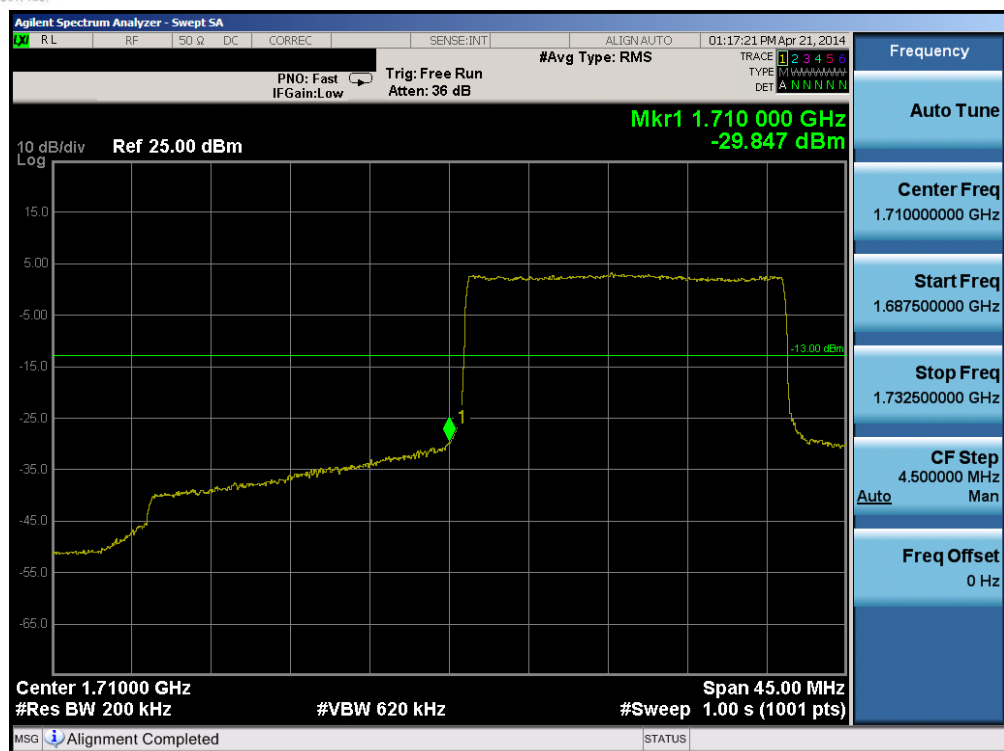
Plot 6-179. Lower Band Edge Plot (Band 4 – 20.0MHz QPSK – RB Size 100)
