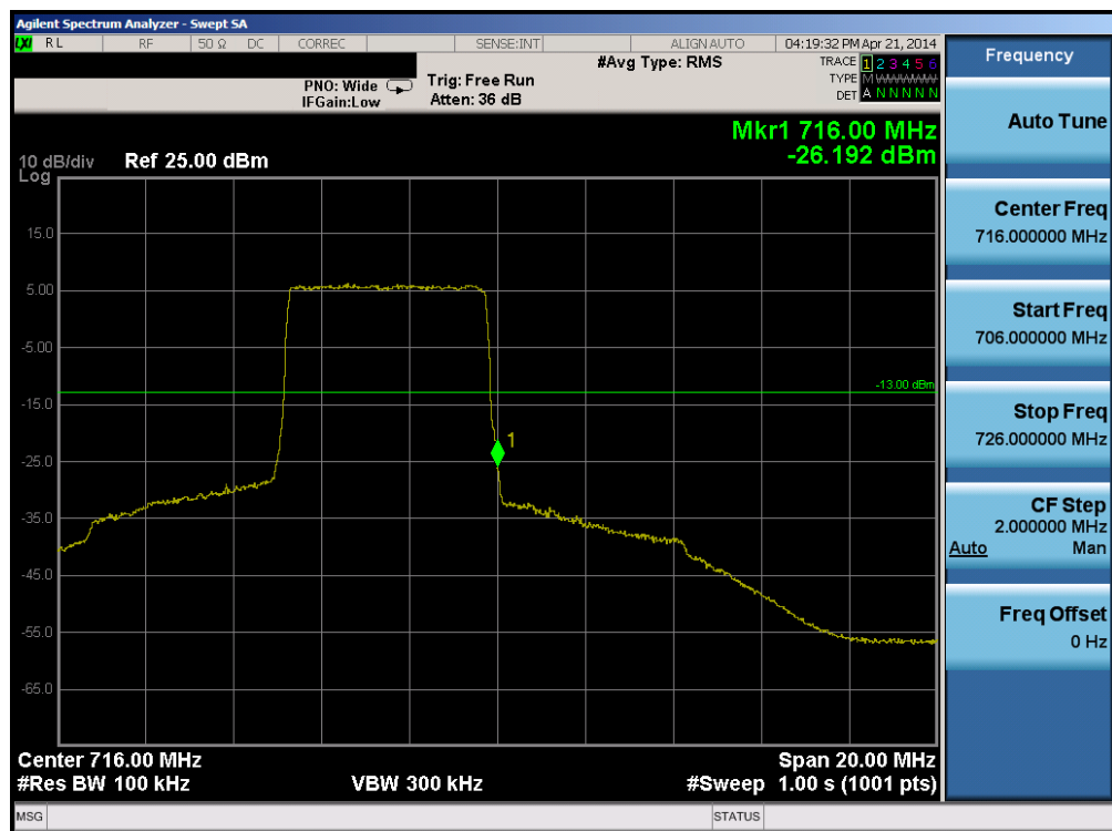
Plot 6-146. Upper Band Edge Plot (Band 17 – 5.0MHz QPSK – RB Size 25)
