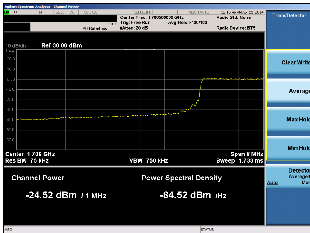
Plot 6-172. Lower Extended Band Edge Plot (Band 4 – 10.0MHz QPSK – RB Size 50)
