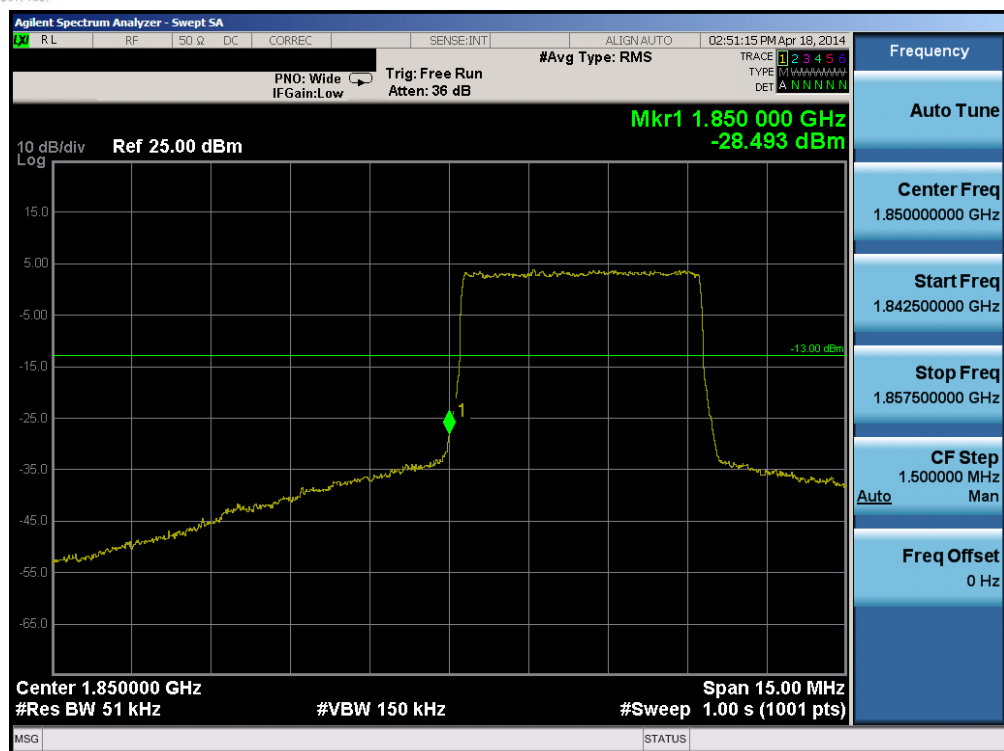
Plot 6-191. Lower Band Edge Plot (Band 2 – 5.0MHz QPSK – RB Size 25)
