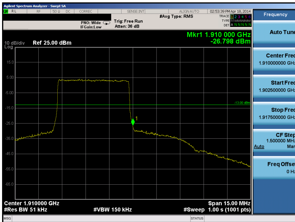
Plot 6-193. Upper Band Edge Plot (Band 2 – 5.0MHz QPSK – RB Size 25)
