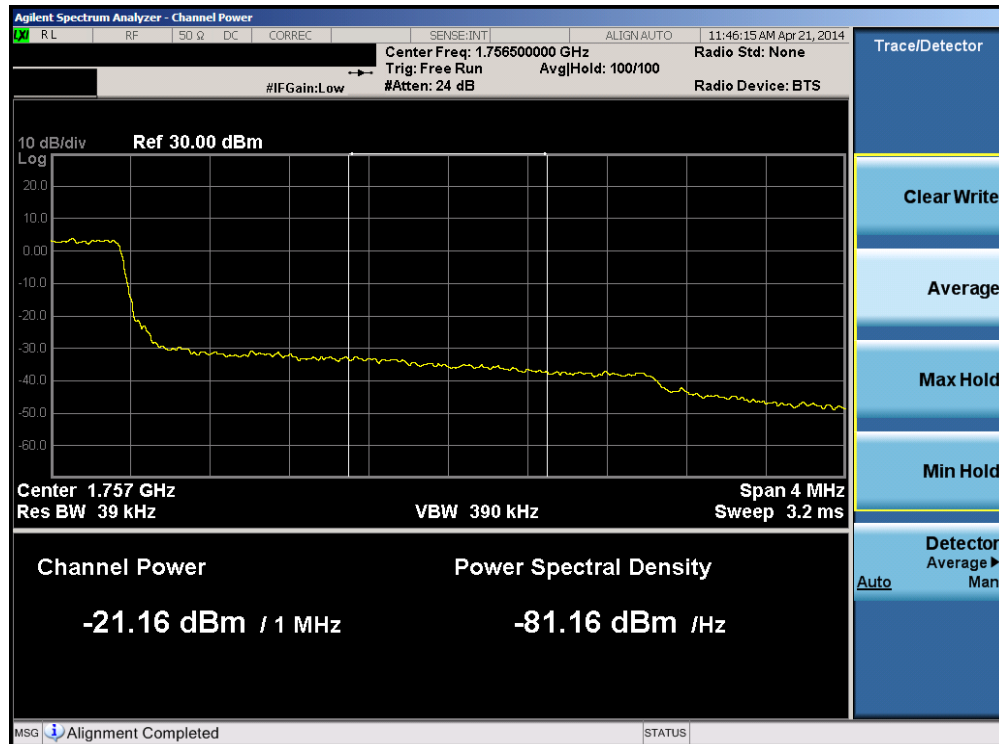
Plot 6-166. Upper Extended Band Edge Plot (Band 4 – 3.0MHz QPSK – RB Size 15)
