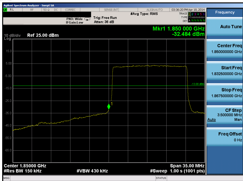
Plot 6-199. Lower Band Edge Plot (Band 2 – 15.0MHz QPSK – RB Size 75)
