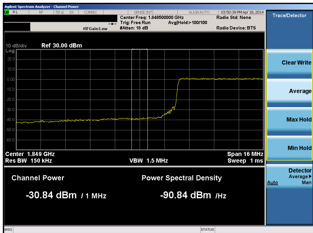
Plot 6-204. Lower Extended Band Edge Plot (Band 2 – 20.0MHz QPSK – RB Size 100)
