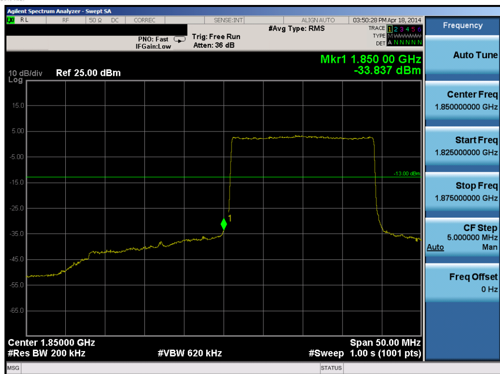
Plot 6-203. Lower Band Edge Plot (Band 2 – 20.0MHz QPSK – RB Size 100)
