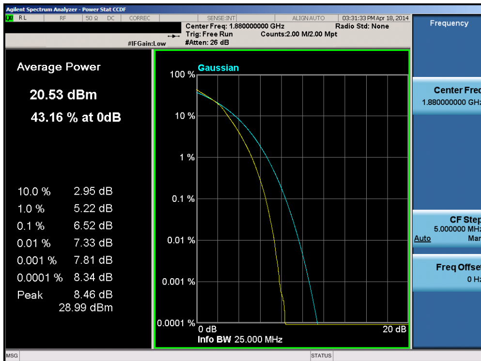
Plot 6-228. PAR Plot (Band 2 – 15.0MHz 16-QAM – RB Size 75)
