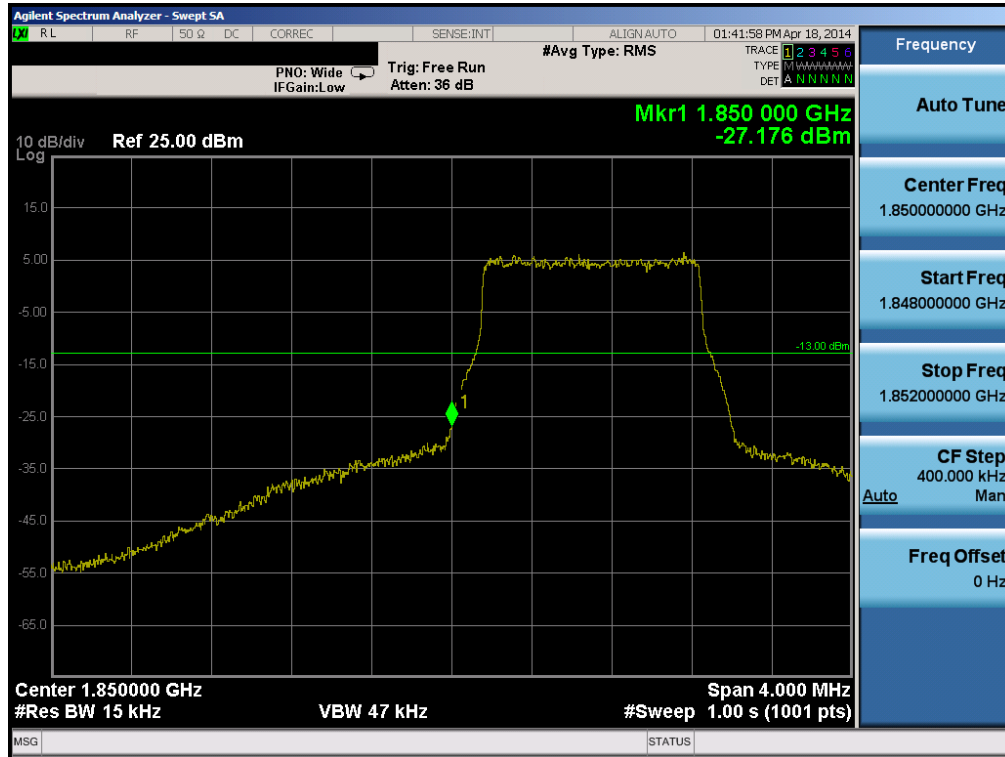
Plot 6-183. Lower Band Edge Plot (Band 2 – 1.4MHz QPSK – RB Size 6)
