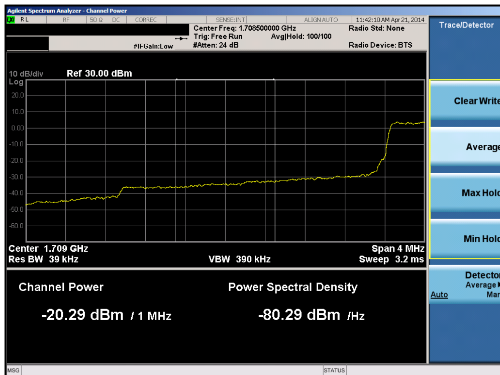
Plot 6-164. Lower Extended Band Edge Plot (Band 4 – 3.0MHz QPSK – RB Size 15)
