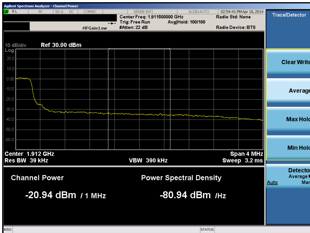
Plot 6-194. Upper Extended Band Edge Plot (Band 2 – 5.0MHz QPSK – RB Size 25)
