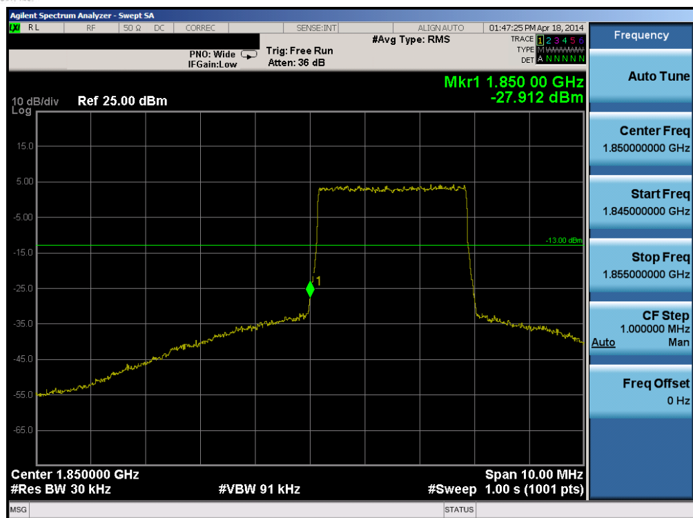
Plot 6-187. Lower Band Edge Plot (Band 2 – 3.0MHz QPSK – RB Size 15)
