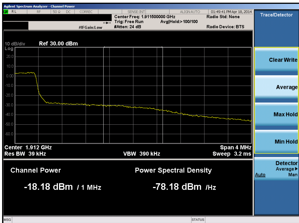
Plot 6-190. Upper Extended Band Edge Plot (Band 2 – 3.0MHz QPSK – RB Size 15)
