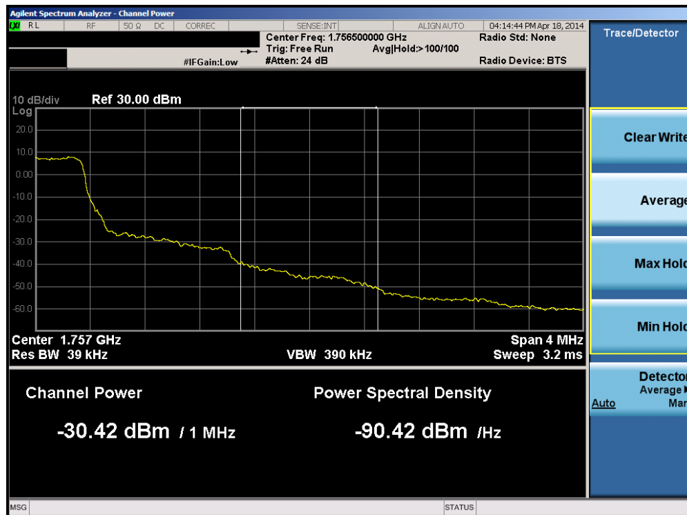
Plot 6-162. Upper Extended Band Edge Plot (Band 4 – 1.4MHz QPSK – RB Size 6)
