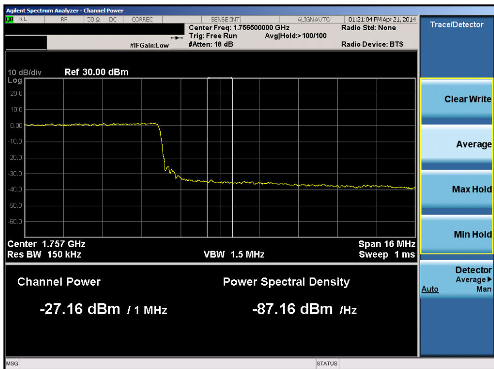
Plot 6-182. Upper Extended Band Edge Plot (Band 4 – 20.0MHz QPSK – RB Size 100)
