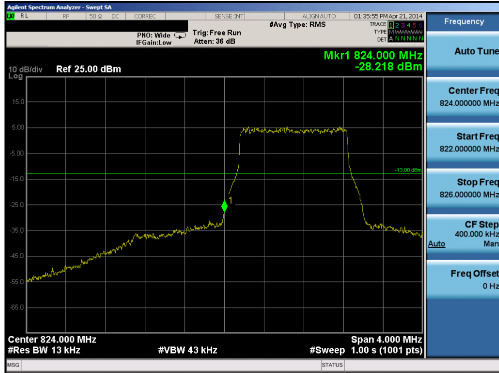
Plot 6-149. Lower Band Edge Plot (Band 5 – 1.4MHz QPSK – RB Size 6)
