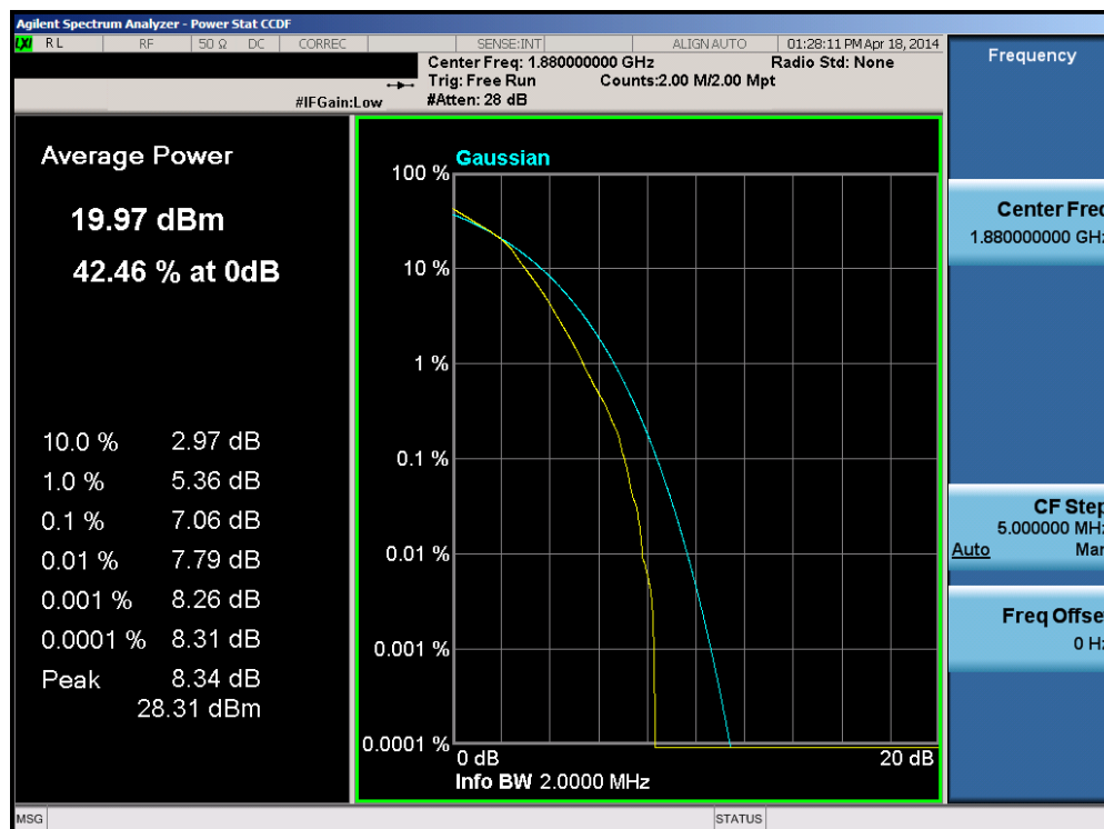
Plot 6-220. PAR Plot (Band 2 – 1.4MHz 16-QAM – RB Size 6)
