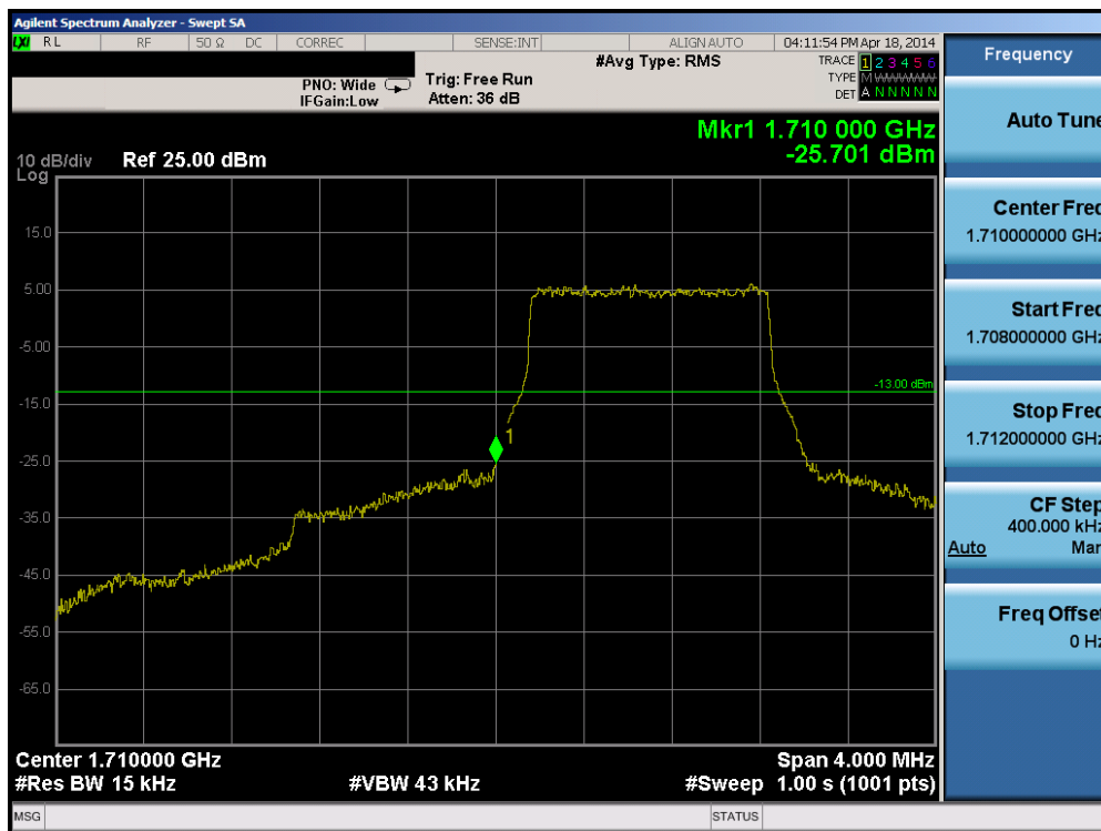
Plot 6-159. Lower Band Edge Plot (Band 4 – 1.4MHz QPSK – RB Size 6)
