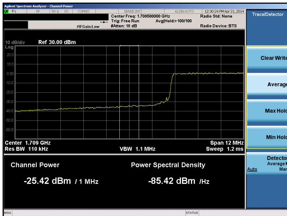
Plot 6-176. Lower Extended Band Edge Plot (Band 4 – 15.0MHz QPSK – RB Size 75)
