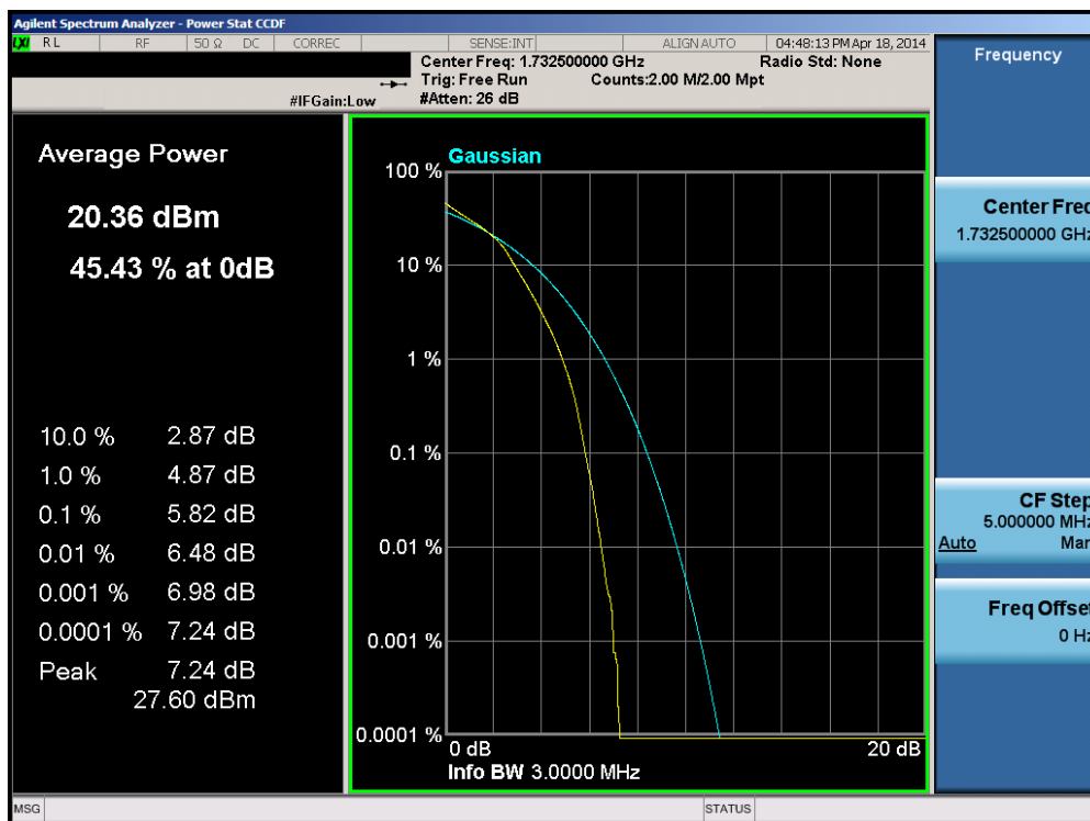
Plot 6-210. PAR Plot (Band 4 – 3.0MHz 16-QAM – RB Size 15)
