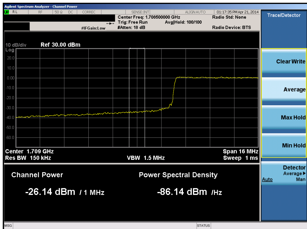
Plot 6-180. Lower Extended Band Edge Plot (Band 4 – 20.0MHz QPSK – RB Size 100)
