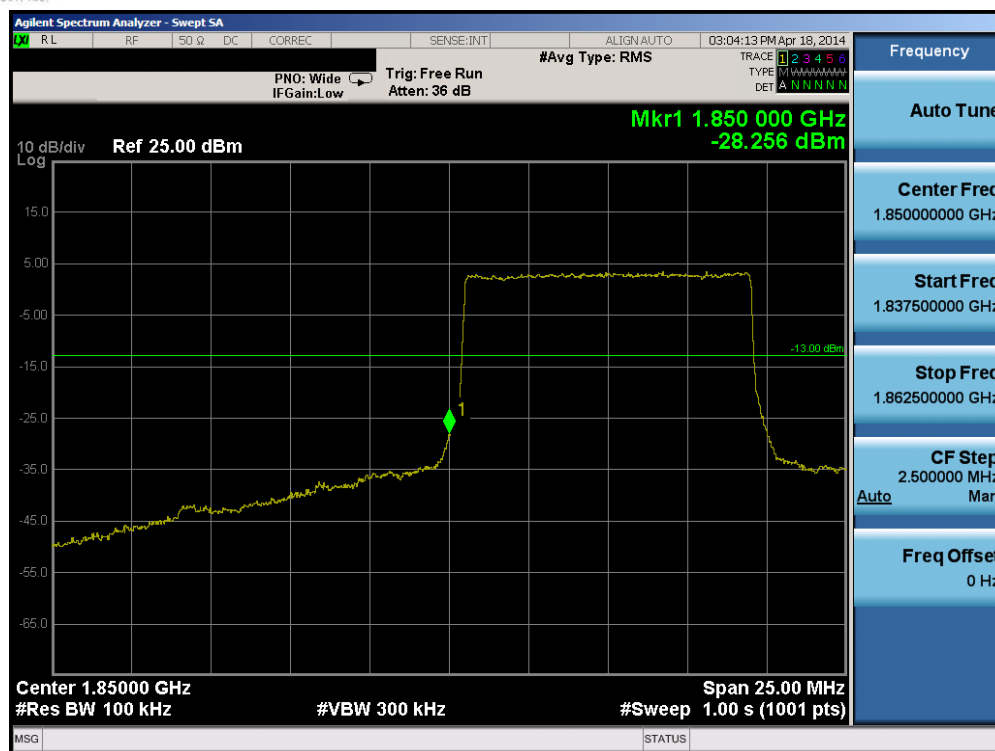
Plot 6-195. Lower Band Edge Plot (Band 2 – 10.0MHz QPSK – RB Size 50)
