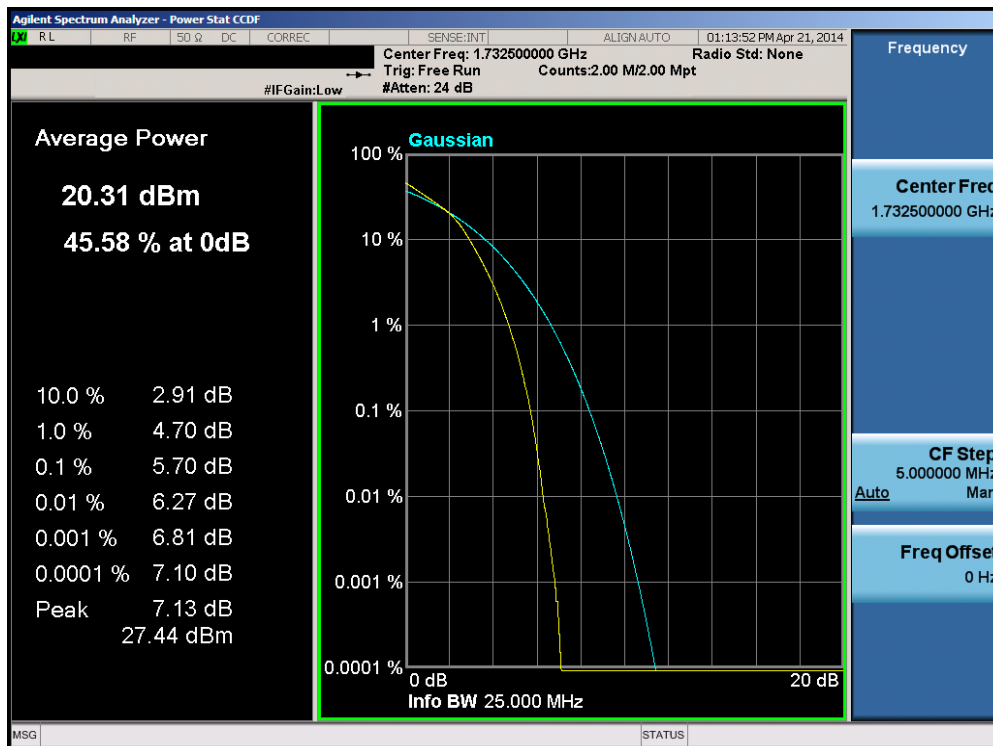
Plot 6-218. PAR Plot (Band 4 – 20.0MHz 16-QAM – RB Size 100)
