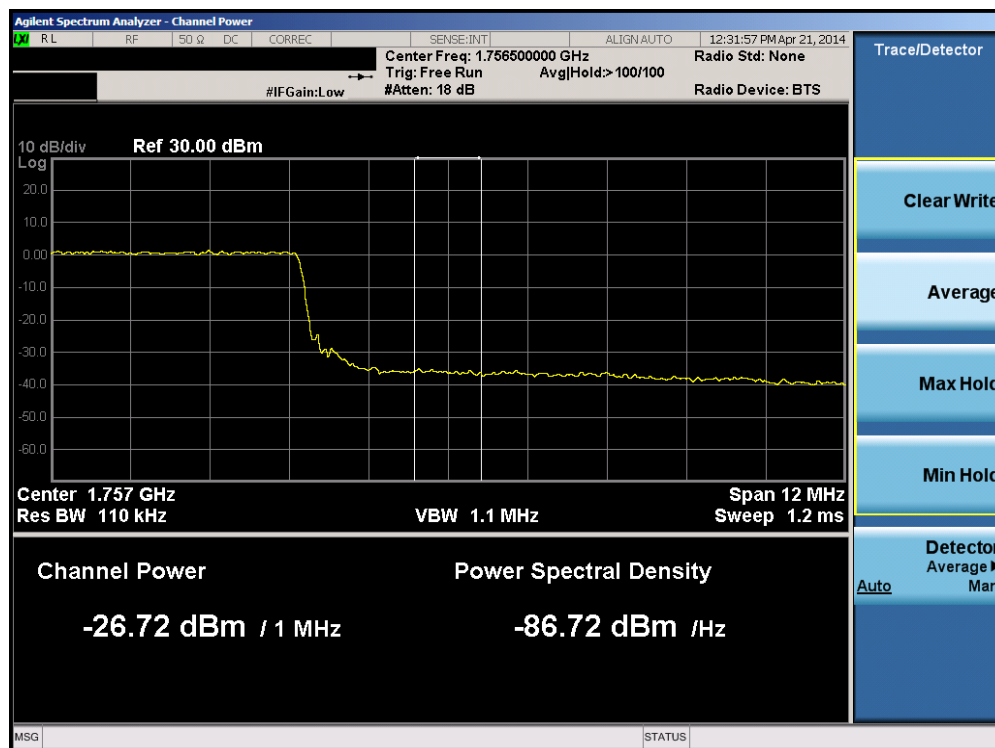
Plot 6-178. Upper Extended Band Edge Plot (Band 4 – 15.0MHz QPSK – RB Size 75)
