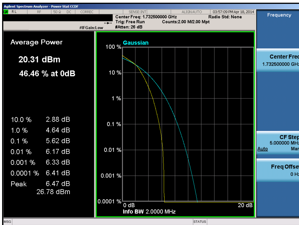
Plot 6-208. PAR Plot (Band 4 – 1.4MHz 16-QAM – RB Size 6)
