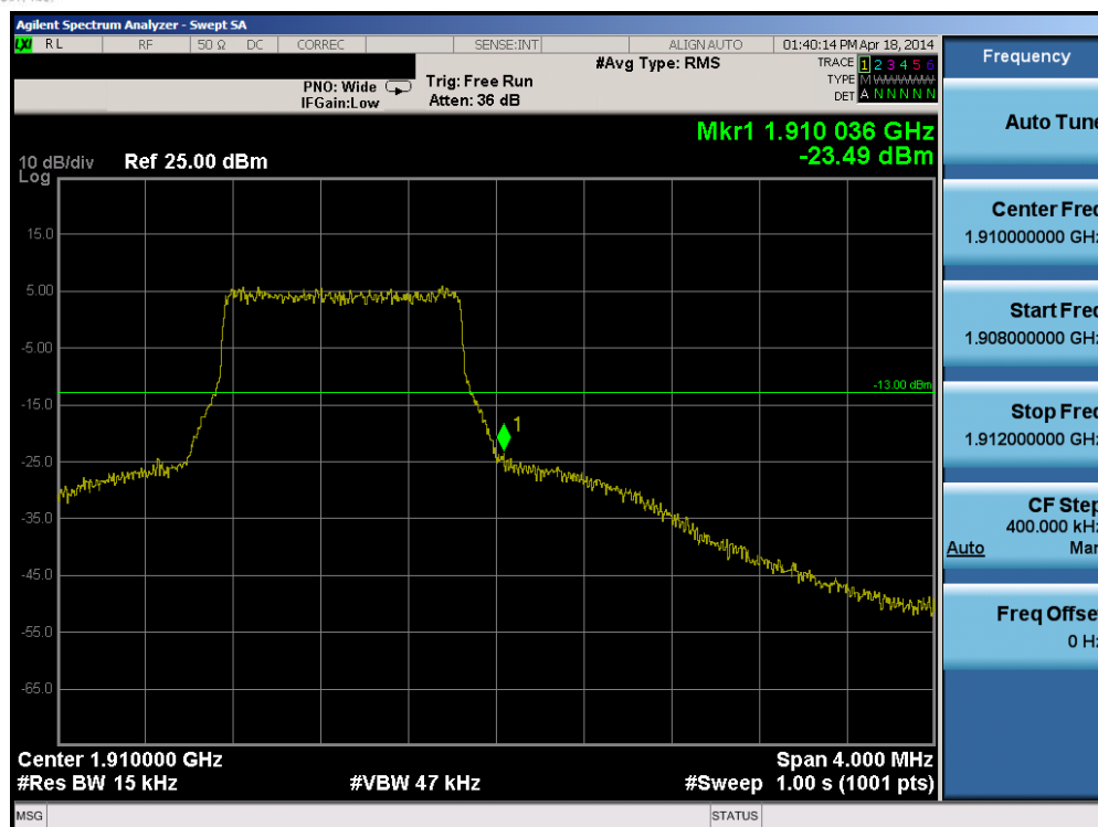
Plot 6-185. Upper Band Edge Plot (Band 2 – 1.4MHz QPSK – RB Size 6)
