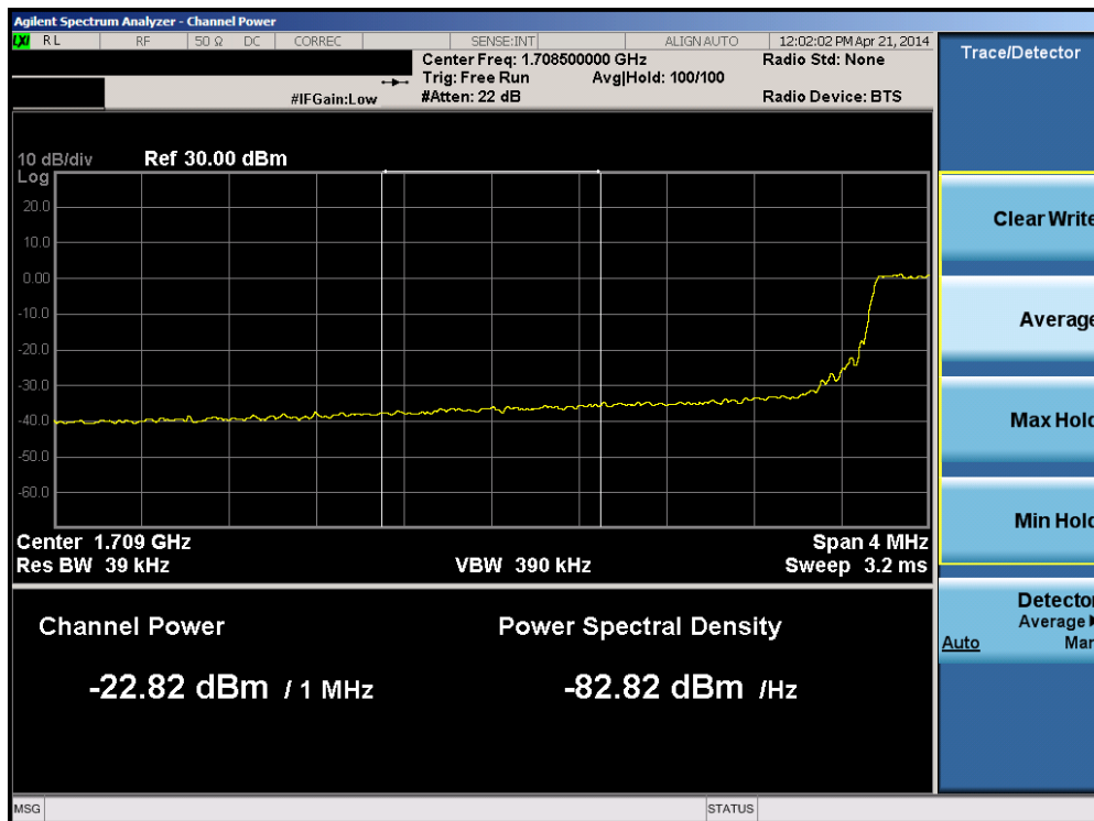
Plot 6-168. Lower Extended Band Edge Plot (Band 4 – 5.0MHz QPSK – RB Size 25)
