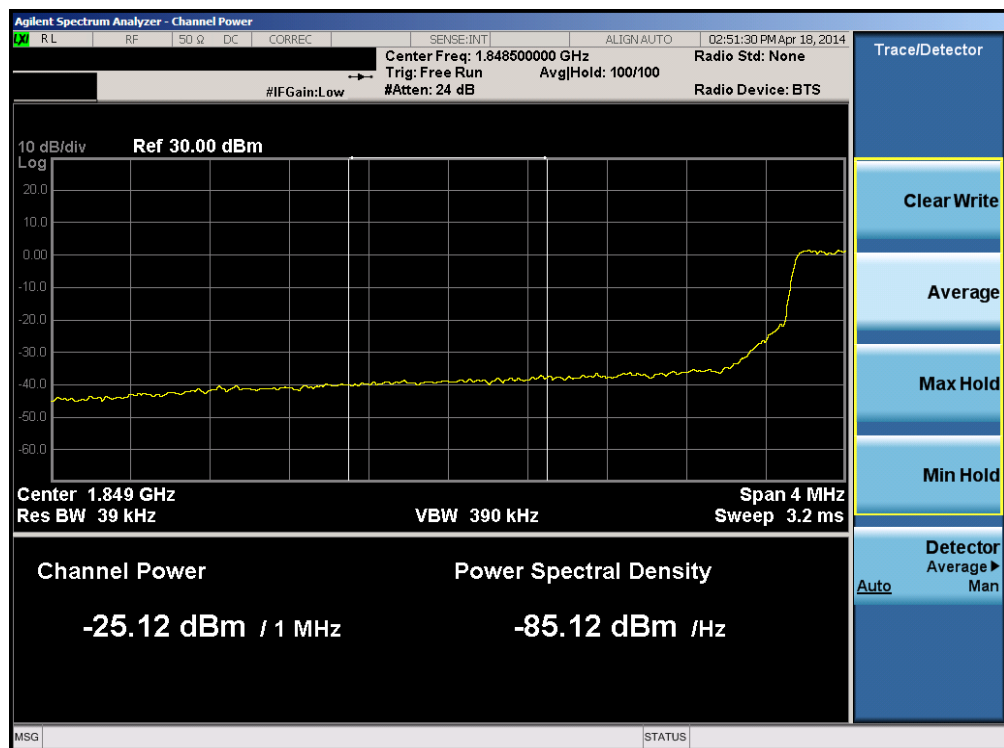
Plot 6-192. Lower Extended Band Edge Plot (Band 2 – 5.0MHz QPSK – RB Size 25)
