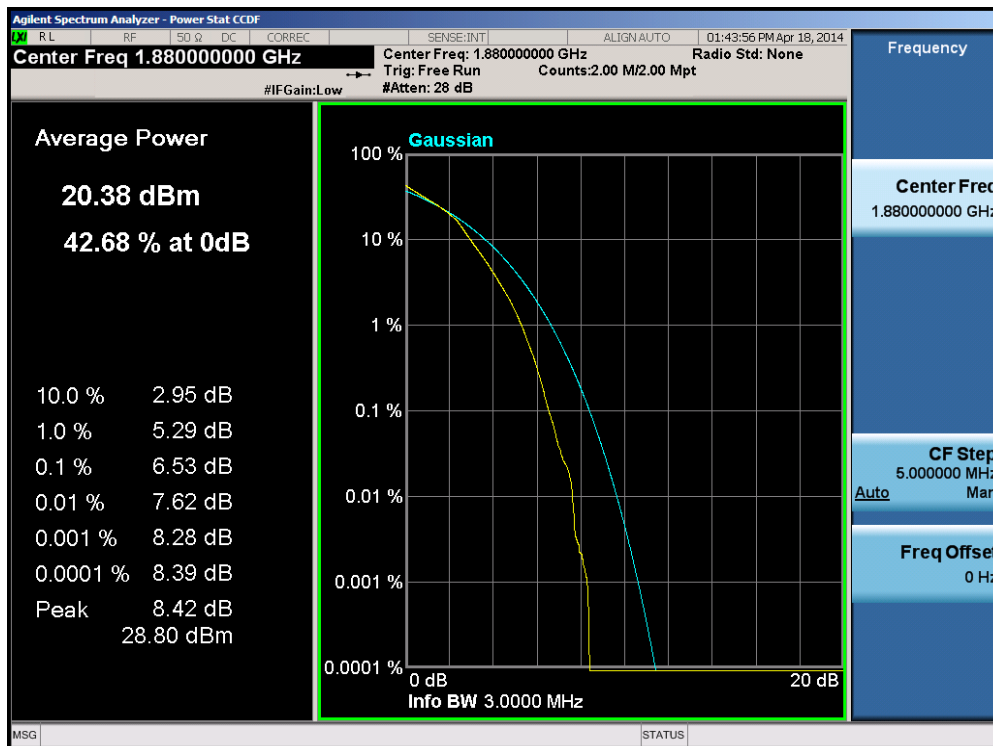
Plot 6-222. PAR Plot (Band 2 – 3.0MHz 16-QAM – RB Size 15)
