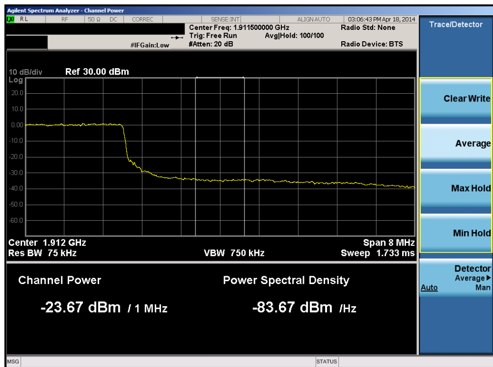
Plot 6-198. Upper Extended Band Edge Plot (Band 2 – 10.0MHz QPSK – RB Size 50)
