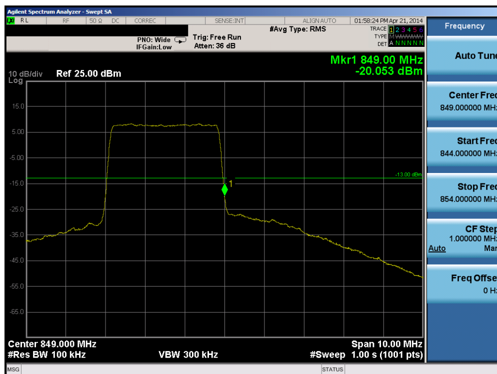
Plot 6-154. Upper Band Edge Plot (Band 5 – 3.0MHz QPSK – RB Size 15)
