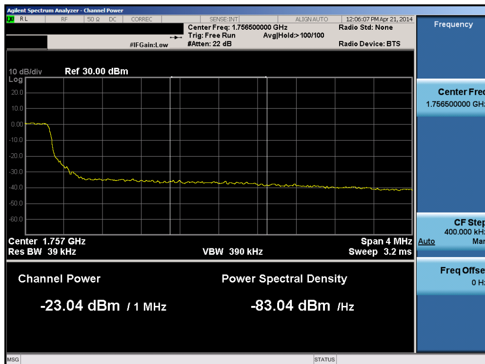
Plot 6-170. Upper Extended Band Edge Plot (Band 4 – 5.0MHz QPSK – RB Size 25)
