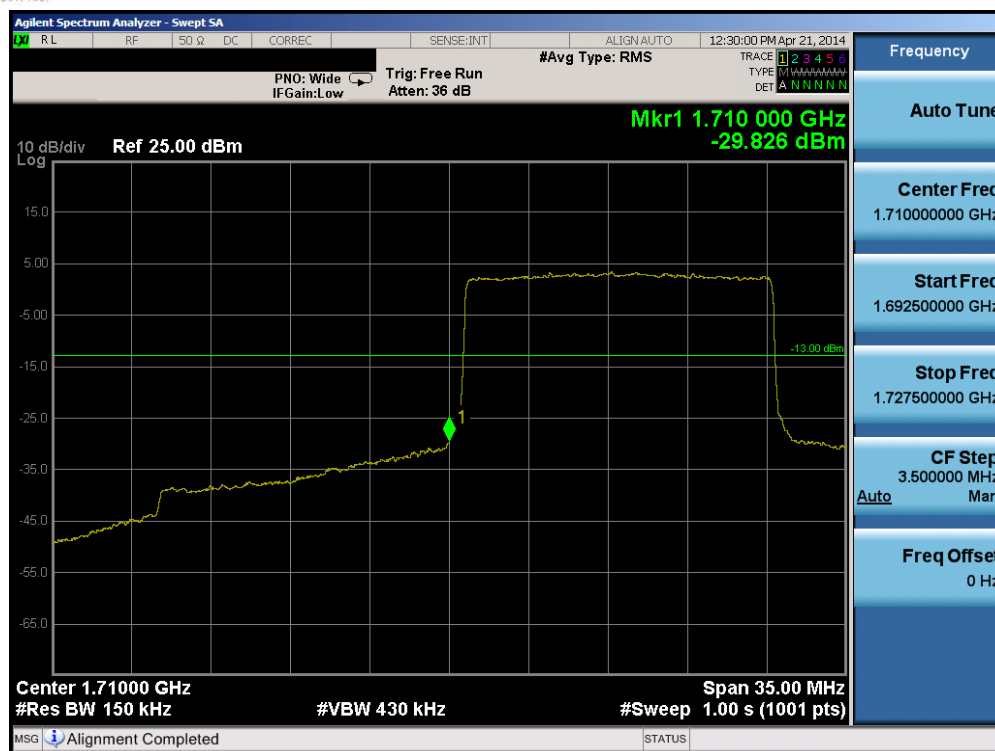
Plot 6-175. Lower Band Edge Plot (Band 4 – 15.0MHz QPSK – RB Size 75)
