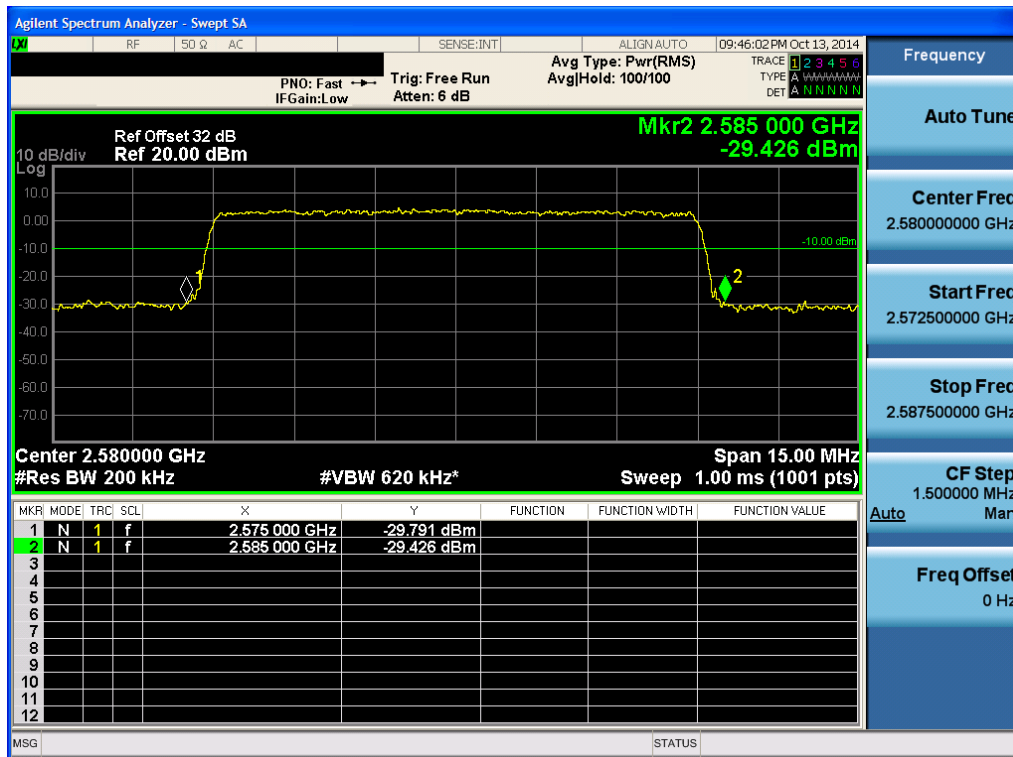
Lower Plot (10 MHz Ch.40490 QPSK -RB size 50)-1
