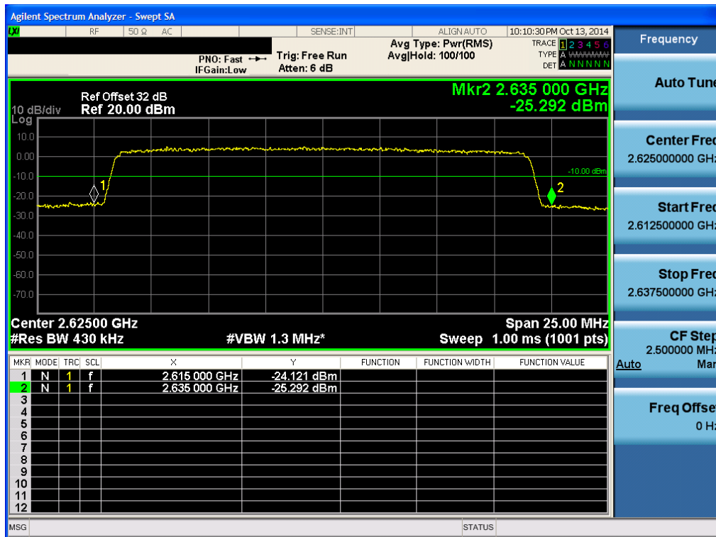
High Plot (20 MHz Ch.40940 QPSK -RB size 100)-5
