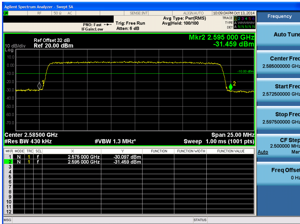
Lower Plot (20 MHz Ch.40540 QPSK -RB size 100)-1
