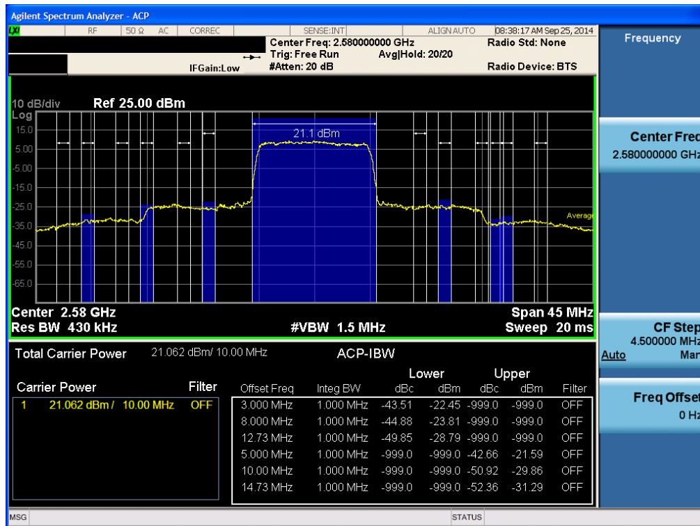
Lower ACP Plot (10 MHz Ch.40490 QPSK -RB size 50)-2
