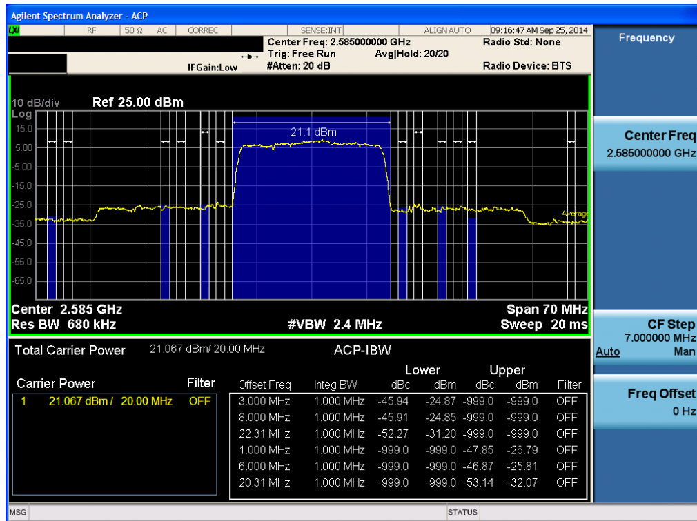
Lower ACP Plot (20 MHz Ch.40540 QPSK -RB size 100)-2
