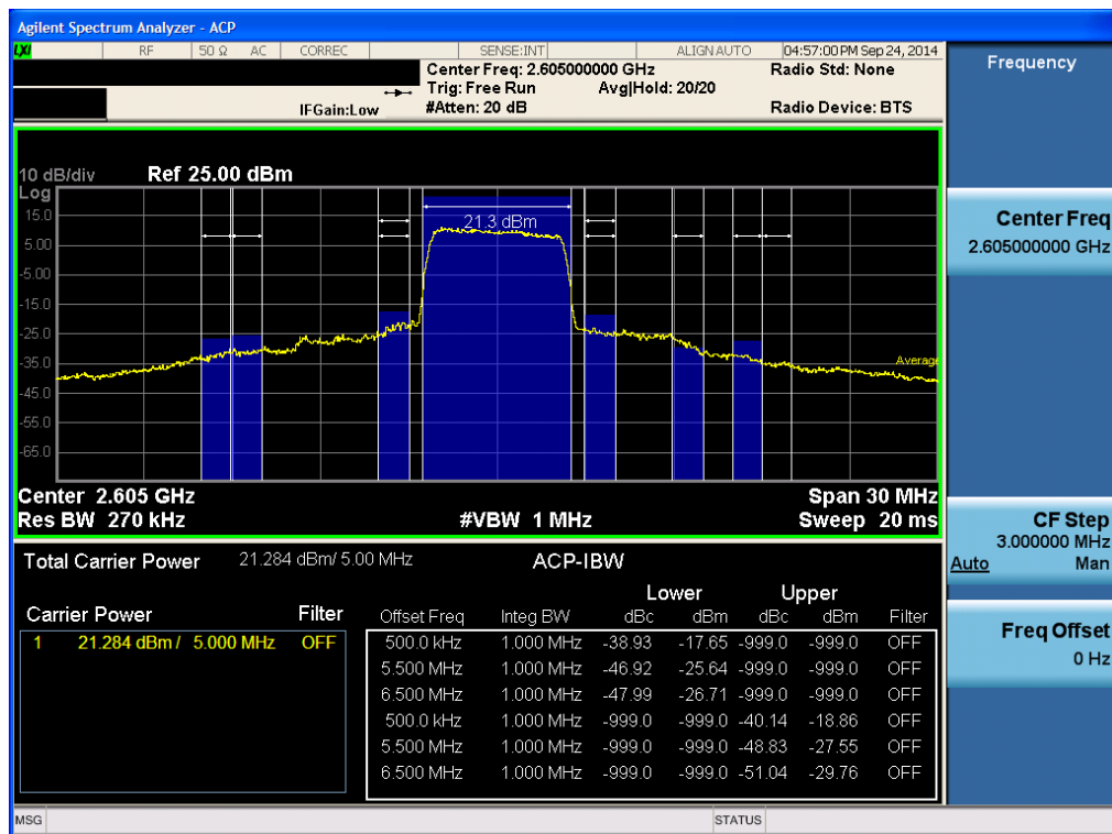
Middle ACP Plot (5 MHz Ch.40740 QPSK -RB size 25)-4
