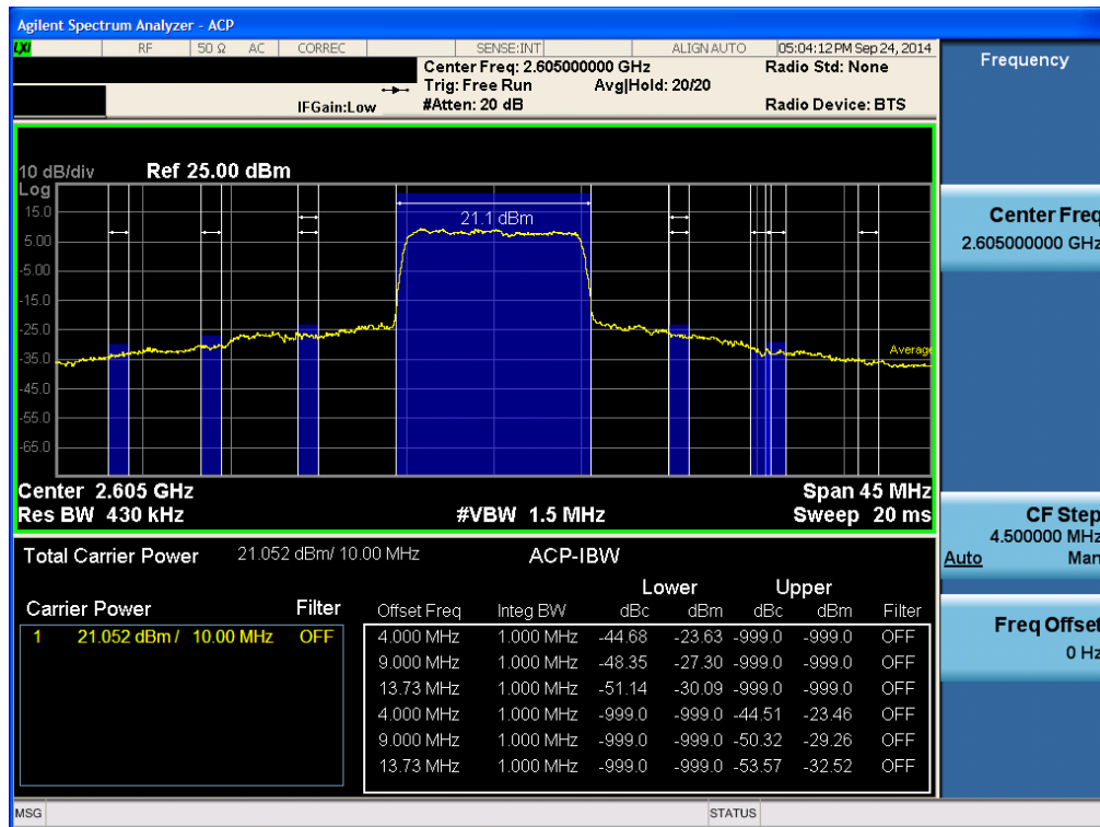
Middle ACP Plot (10 MHz Ch.40740 QPSK -RB size 50)-4
