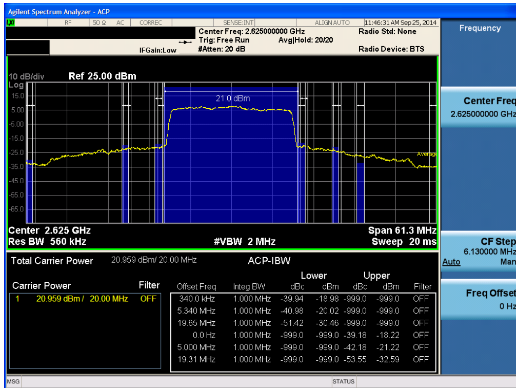
High ACP Plot (20 MHz Ch.40940 QPSK -RB size 100)-6
