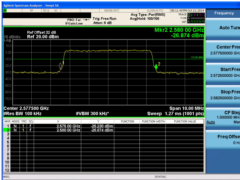
Lower Plot (5 MHz Ch.40465 QPSK -RB size 25)-1
