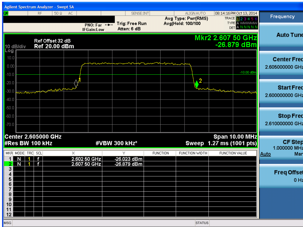
Middle Plot (5 MHz Ch.40740 QPSK -RB size 25)-3
