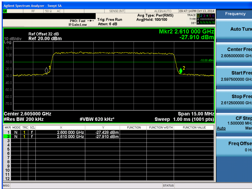
Middle Plot (10 MHz Ch.40740 QPSK -RB size 50)-3
