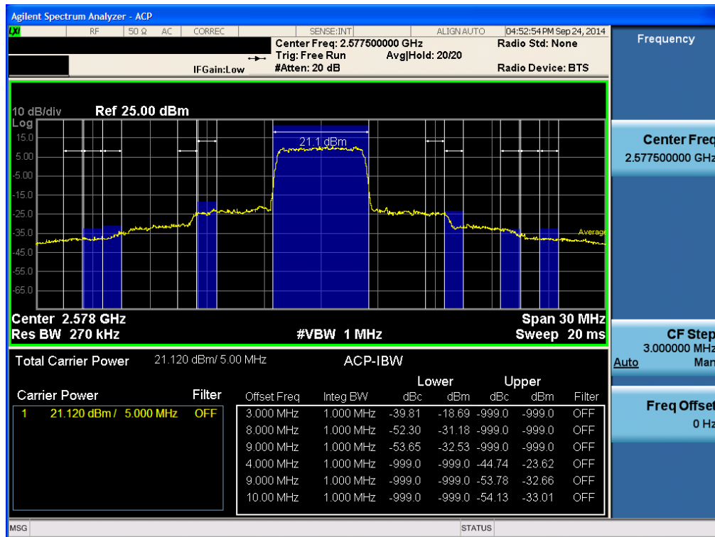
Lower ACP Plot (5 MHz Ch.40465 QPSK -RB size 25)-2
