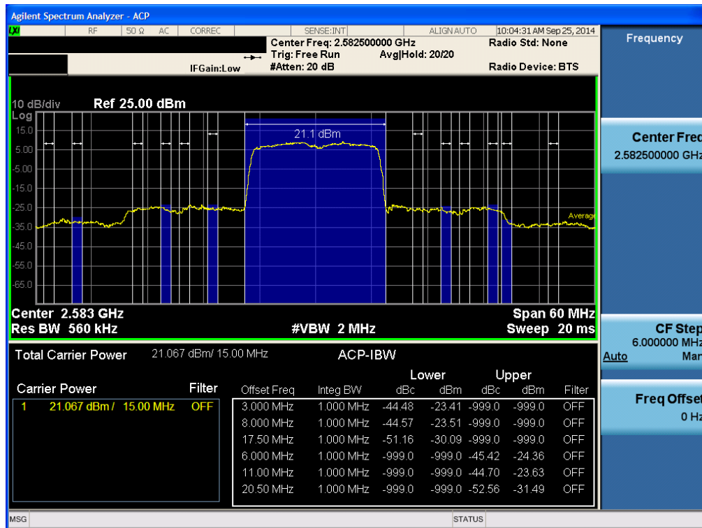
Lower ACP Plot (15 MHz Ch.40515 QPSK -RB size 75)-2
