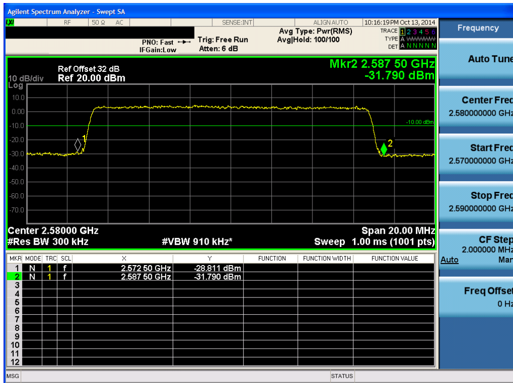
Lower Plot (15 MHz Ch.40515 QPSK -RB size 75)-1
