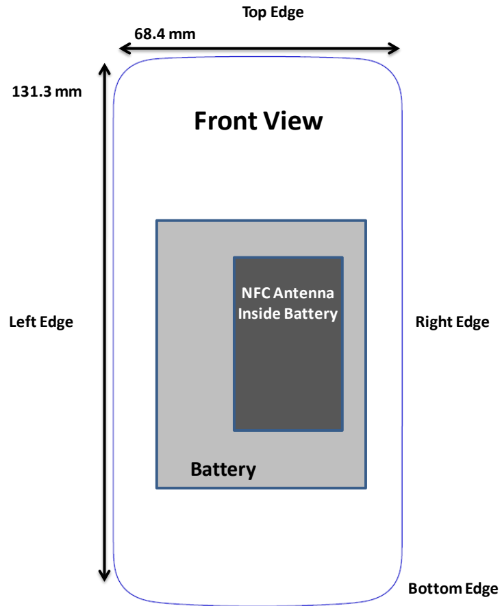
Figure 1-2 NFC Antenna Locations
