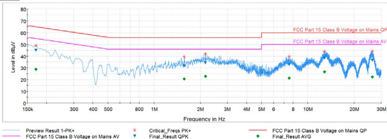
Plot 6-44. Line-Conducted Test Plot (L1)
