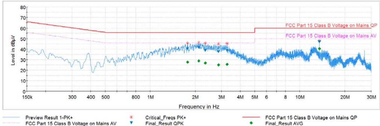
Plot 8-2. Line-Conducted Test Plot (N)
