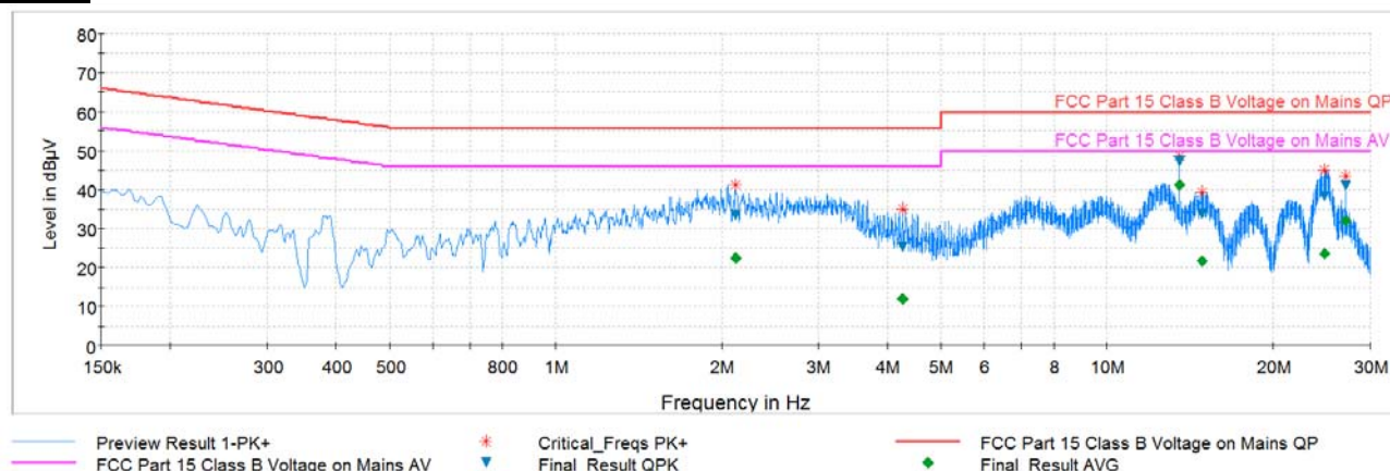
Plot 8-1. Line-Conducted Test Plot (L1)
